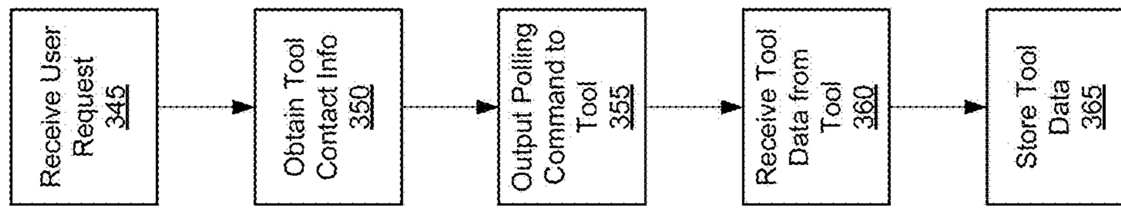
Tool Polling
