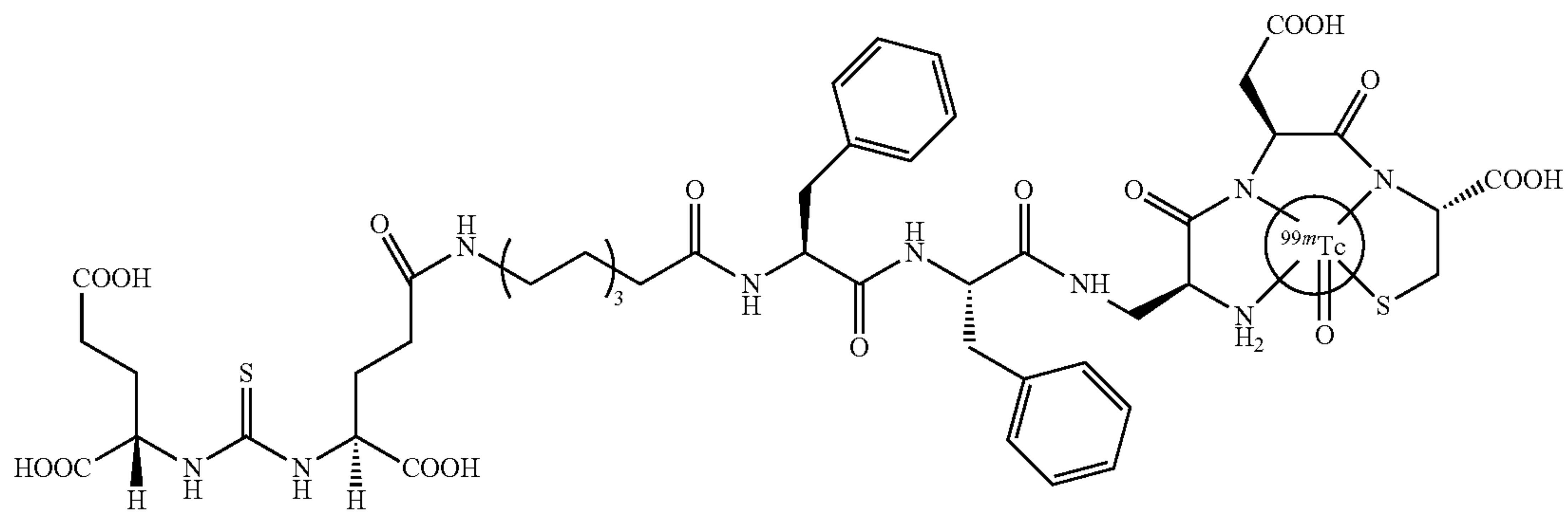
anti-VC6
