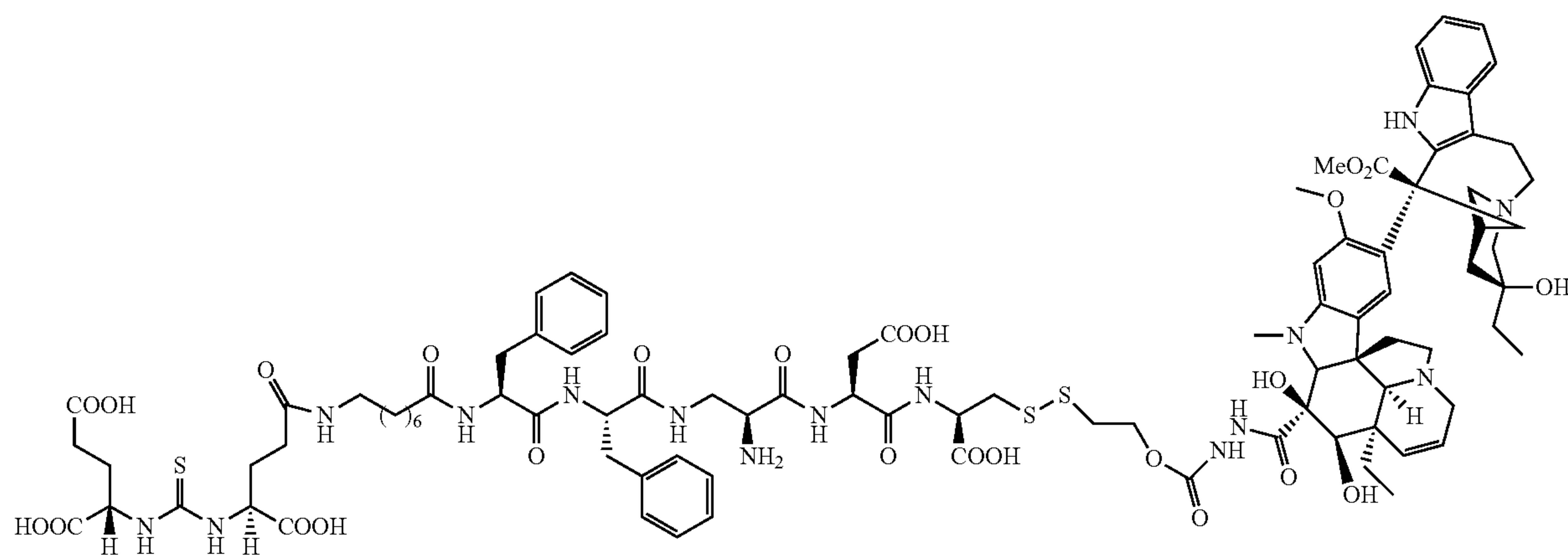
(31 atom linker, Desacetylvinblastinhydrazone)
