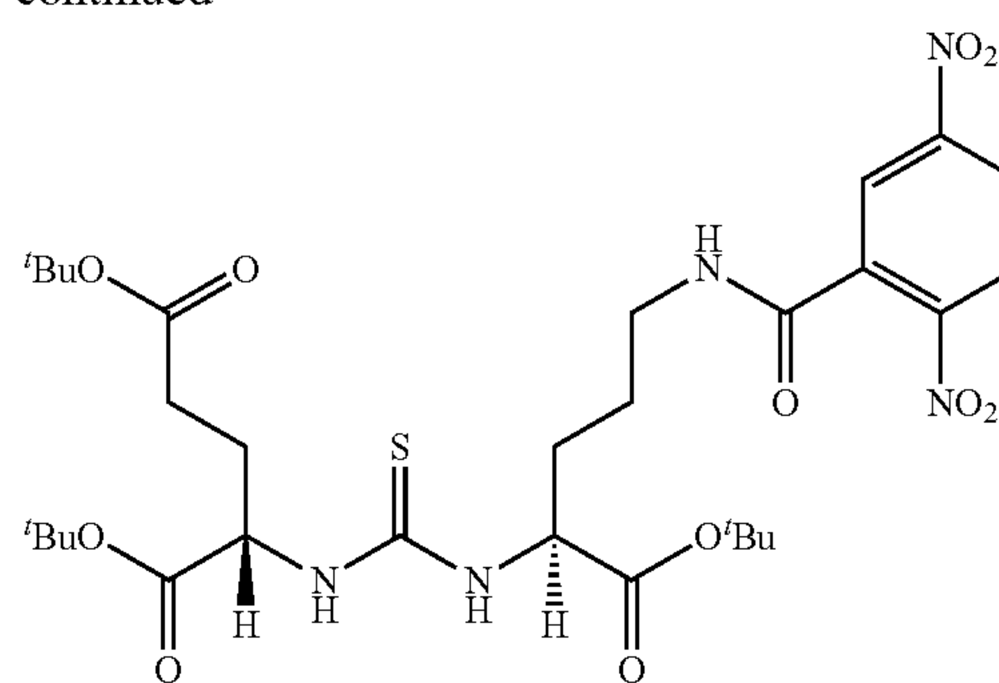
(0 atom linker, PET precursor)
