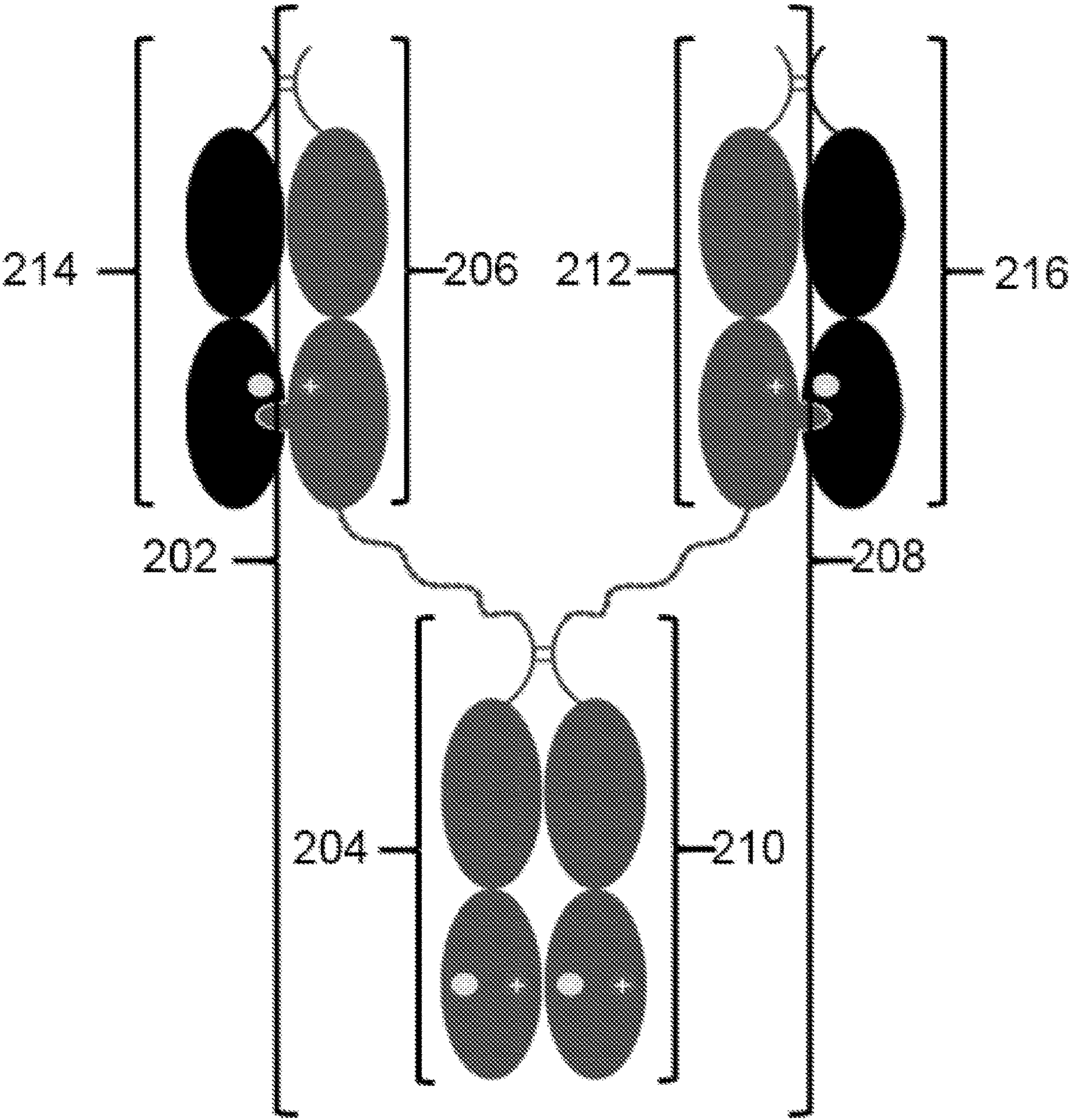
FIG. 2 (Fc construct 4)
