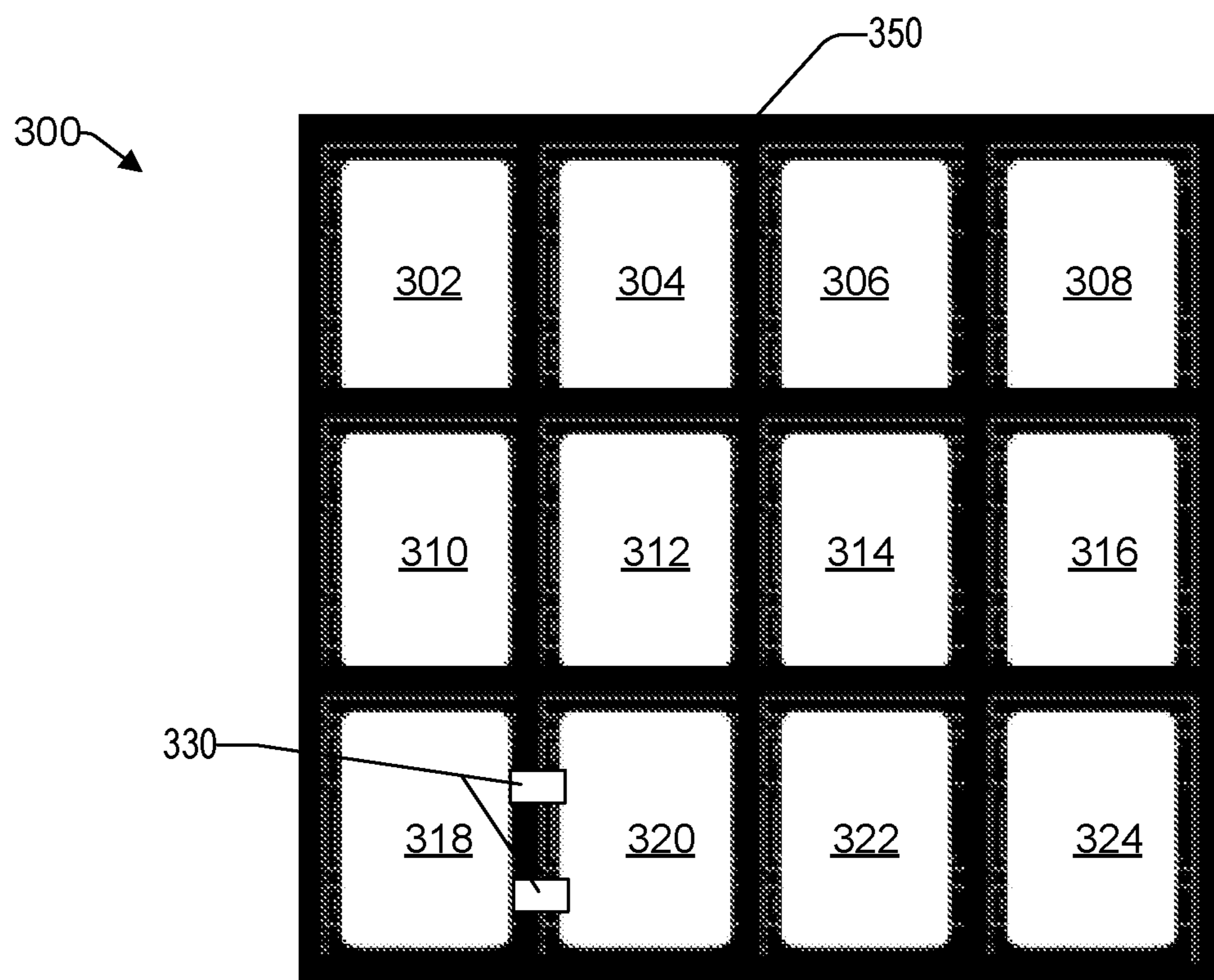
MULTICHIP CONFIGURATION
