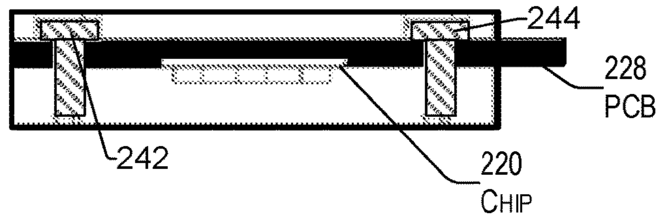
CROSS SECTION OF A PACKAGE
