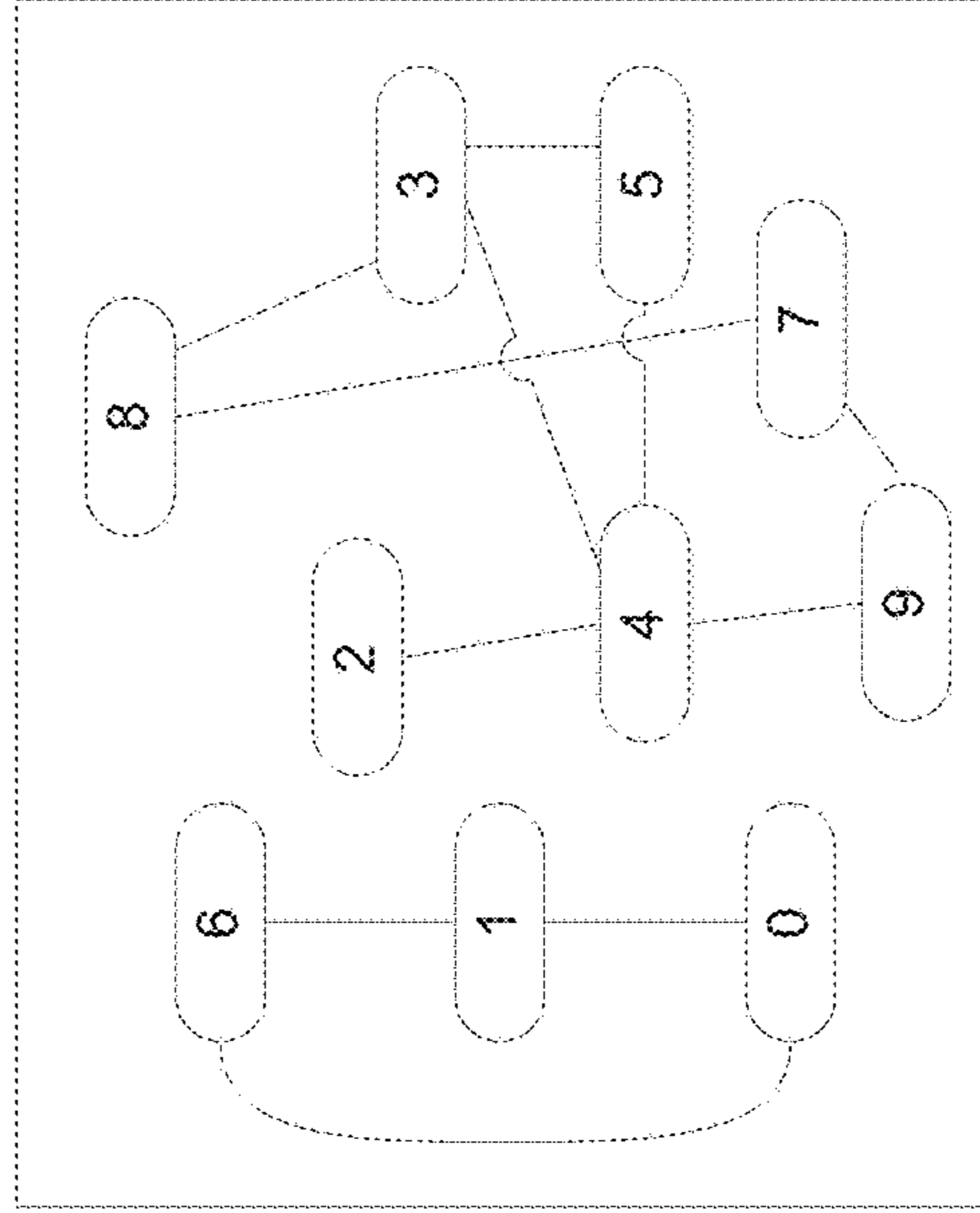
704 Example Clusters
