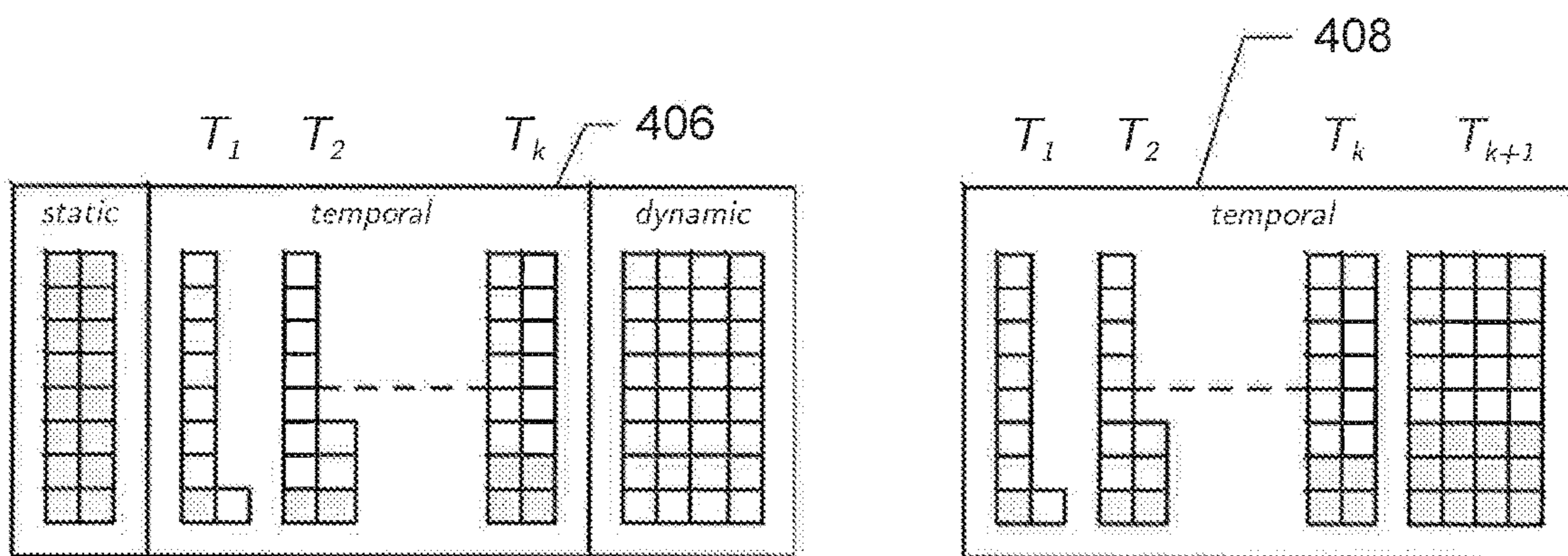
STD using Temporal SDC with variable sizes
