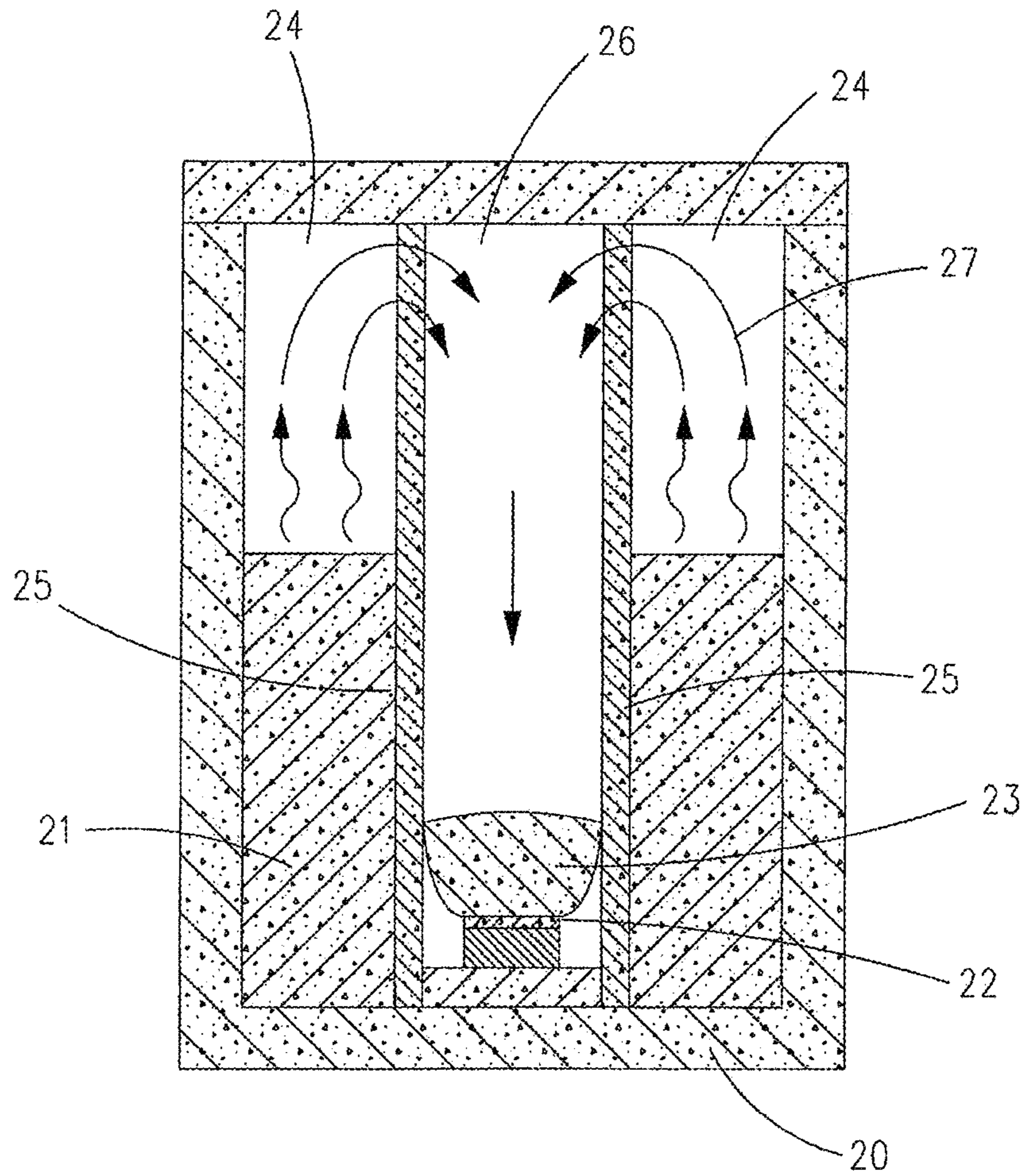
FIG. 2 (PRIOR ART)
