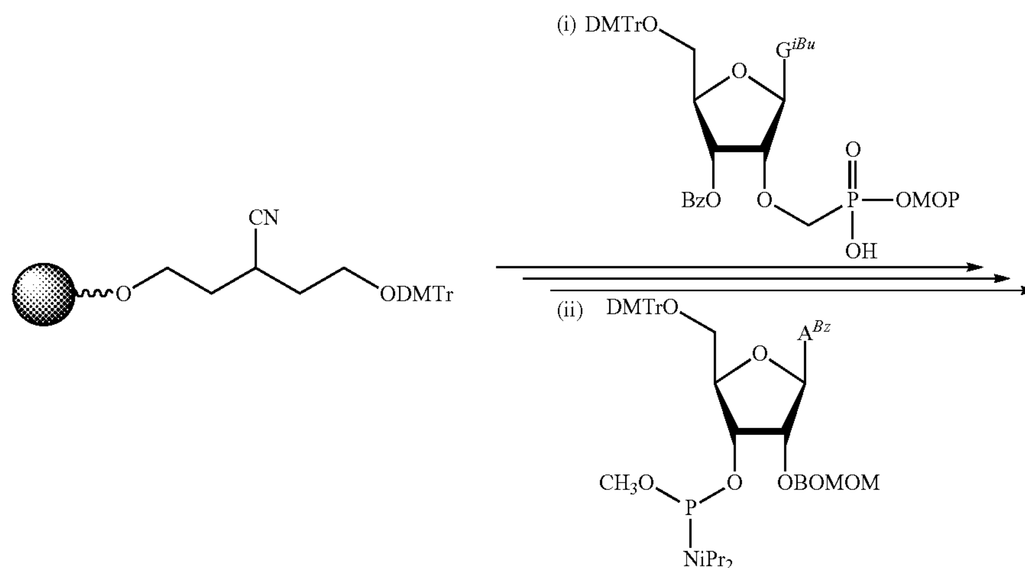
Scheme 3. Exemplary synthesis of CDN derived from nucleoside-2'- and 3'-methylphosphonates.
