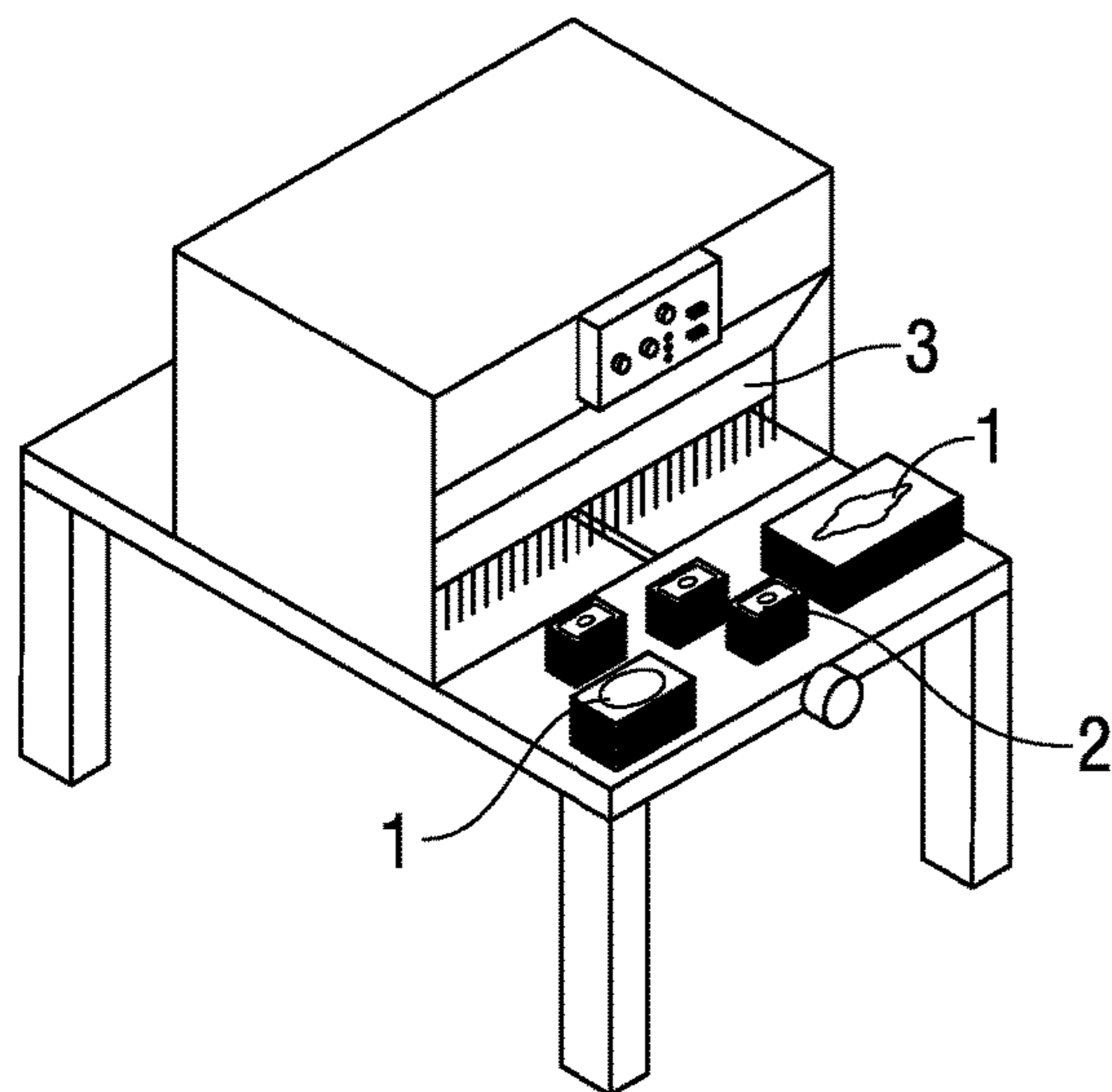
FIG. 9 Prior Art
