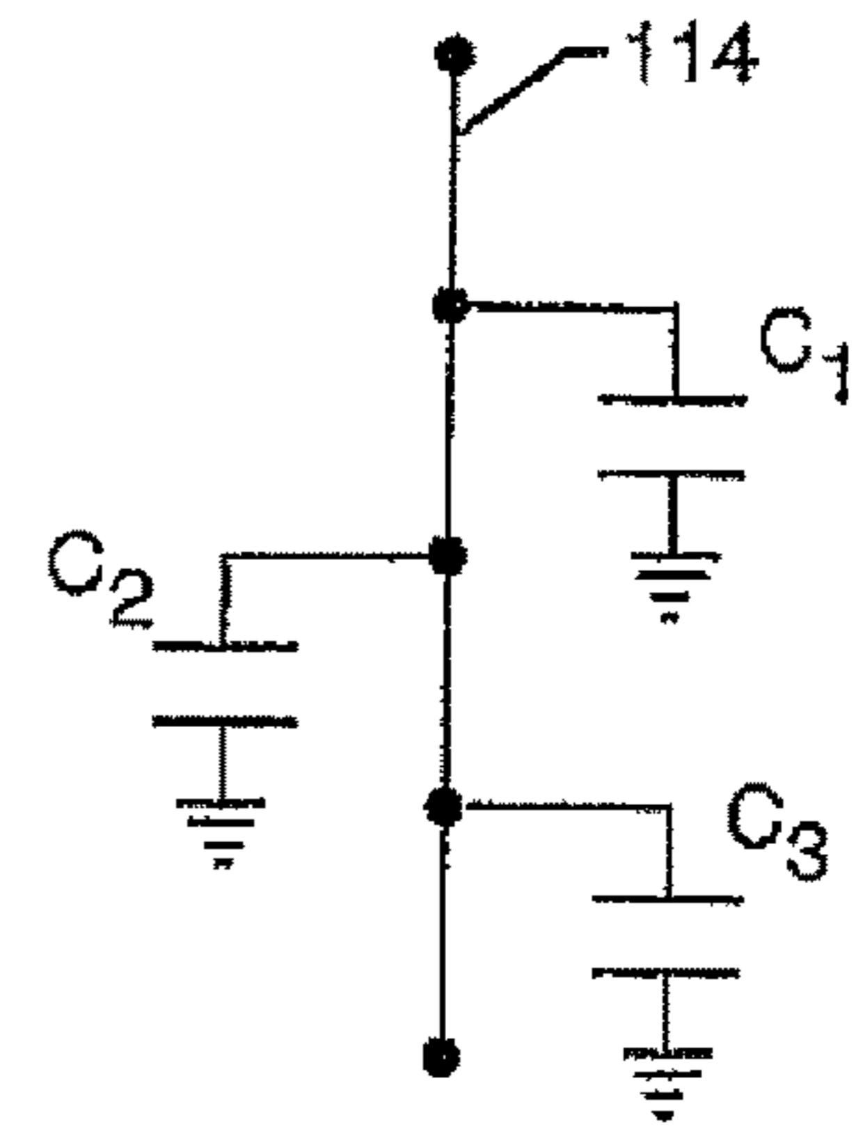
FIG. 20 PRIOR ART
