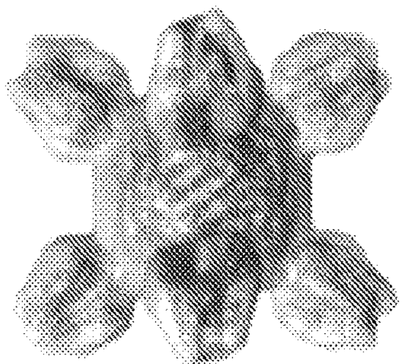
H1-SS-np model fit into cryo-EM map
