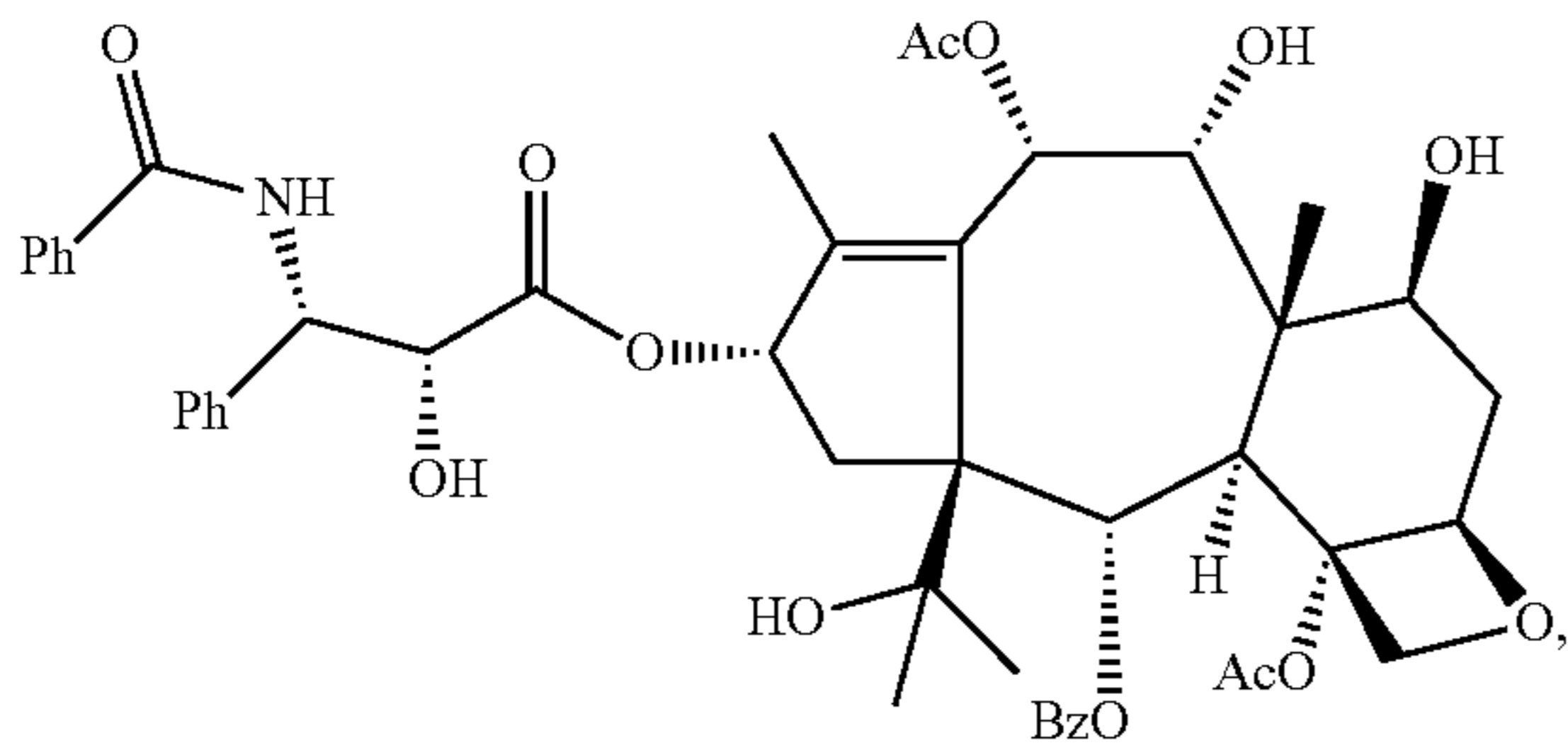
Formula (22a)
