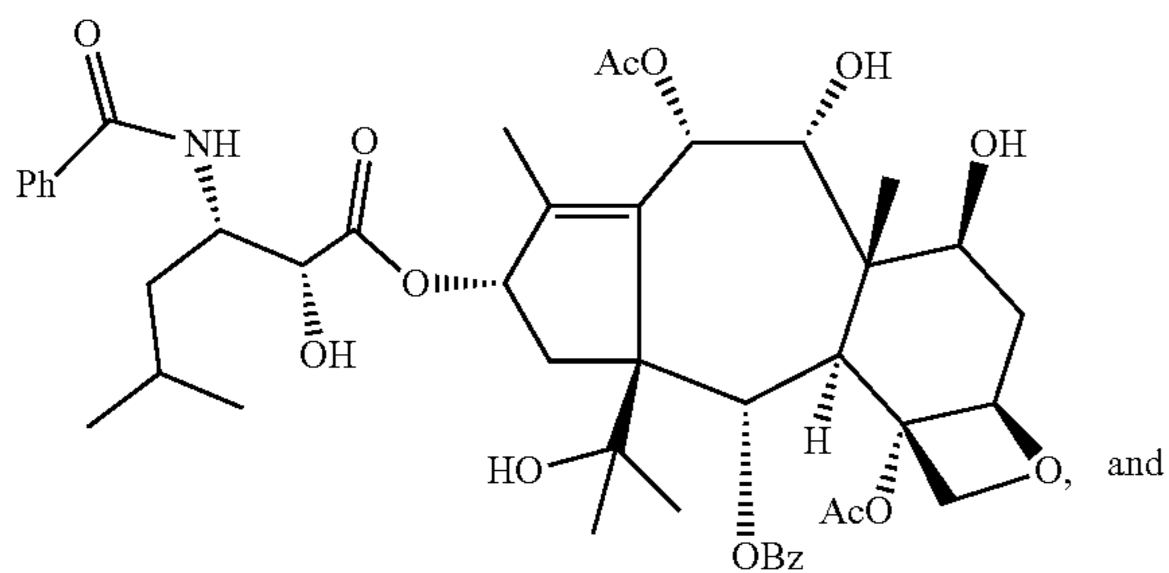
Formula (27 & 28)
