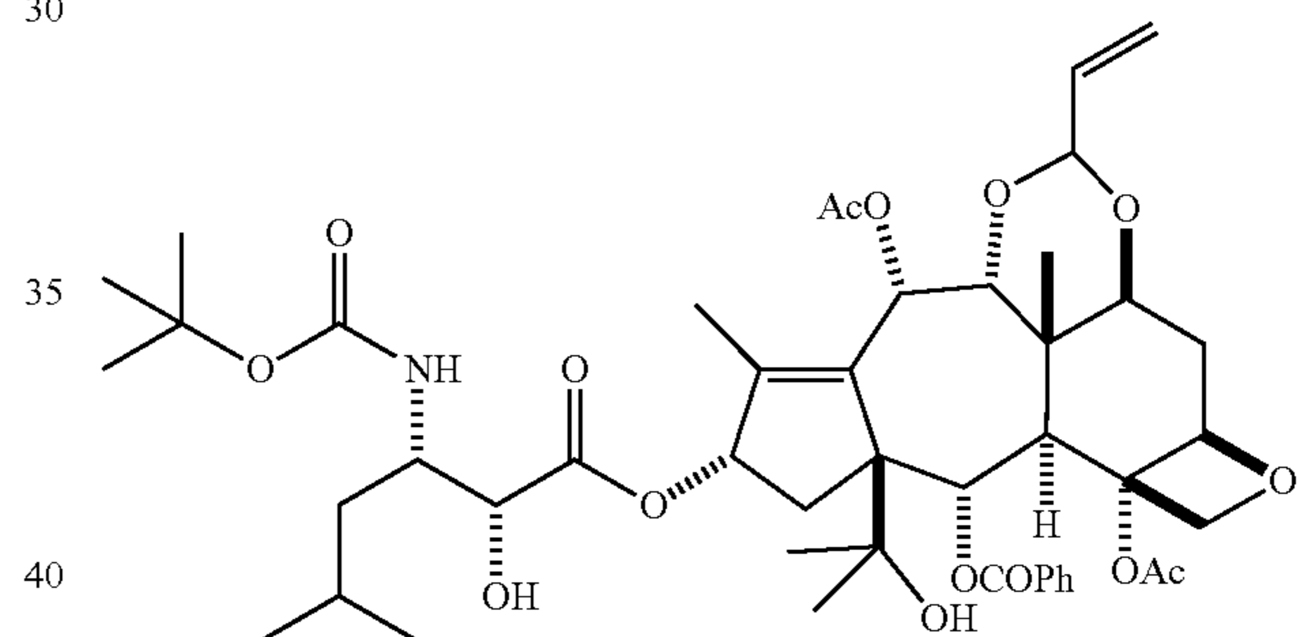
Formula (3)
