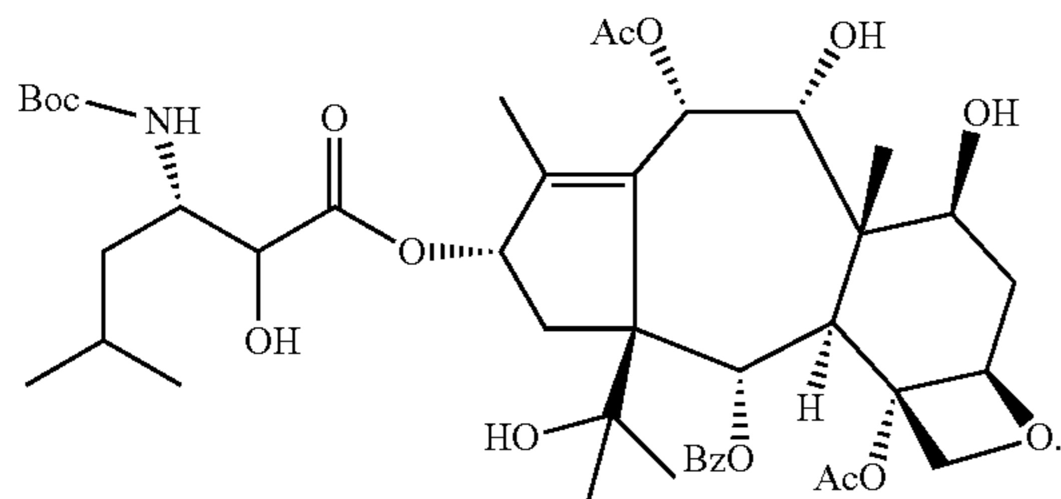
Formula (27 & 28)
