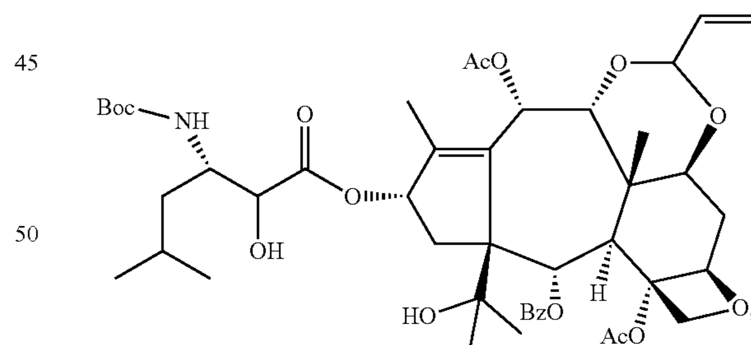
Formula (3)
