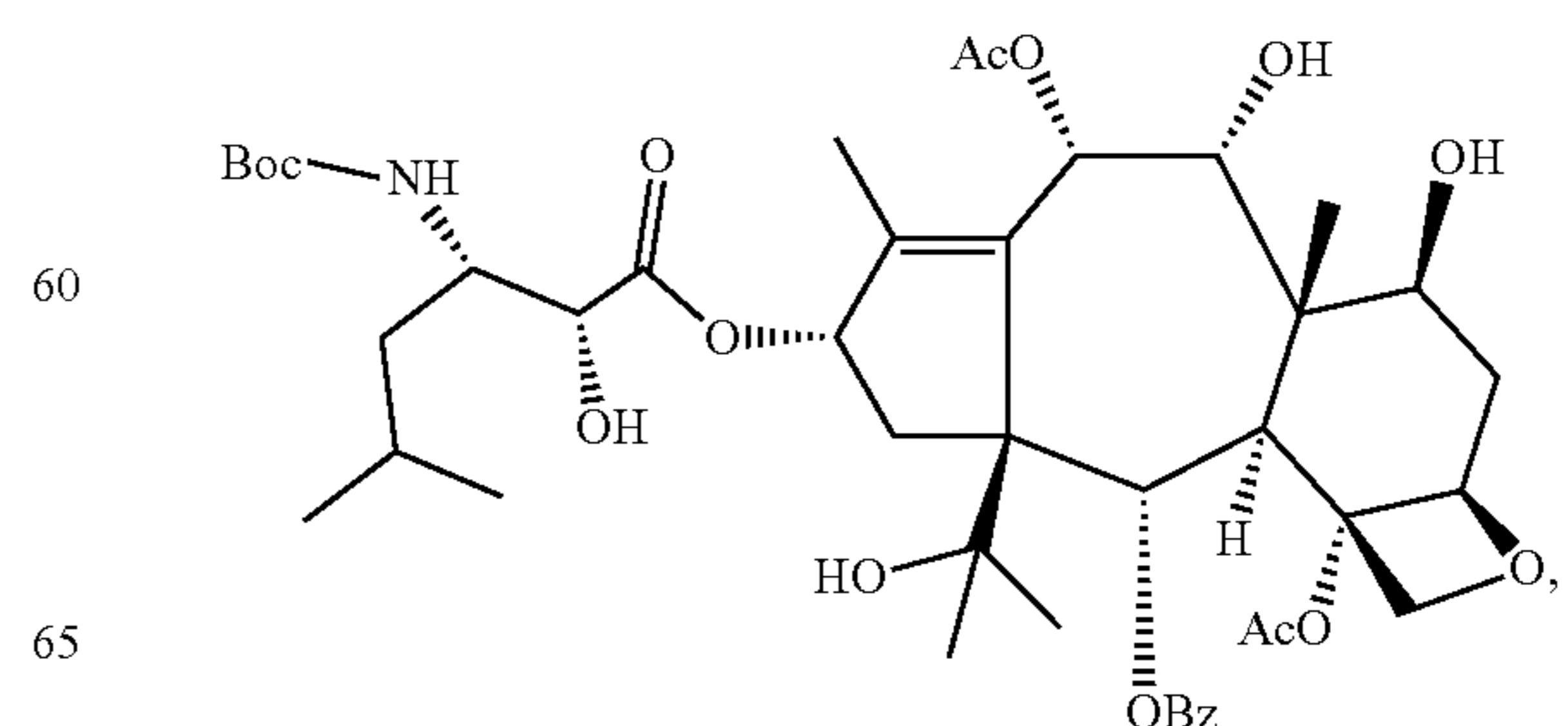
Formula (13)
