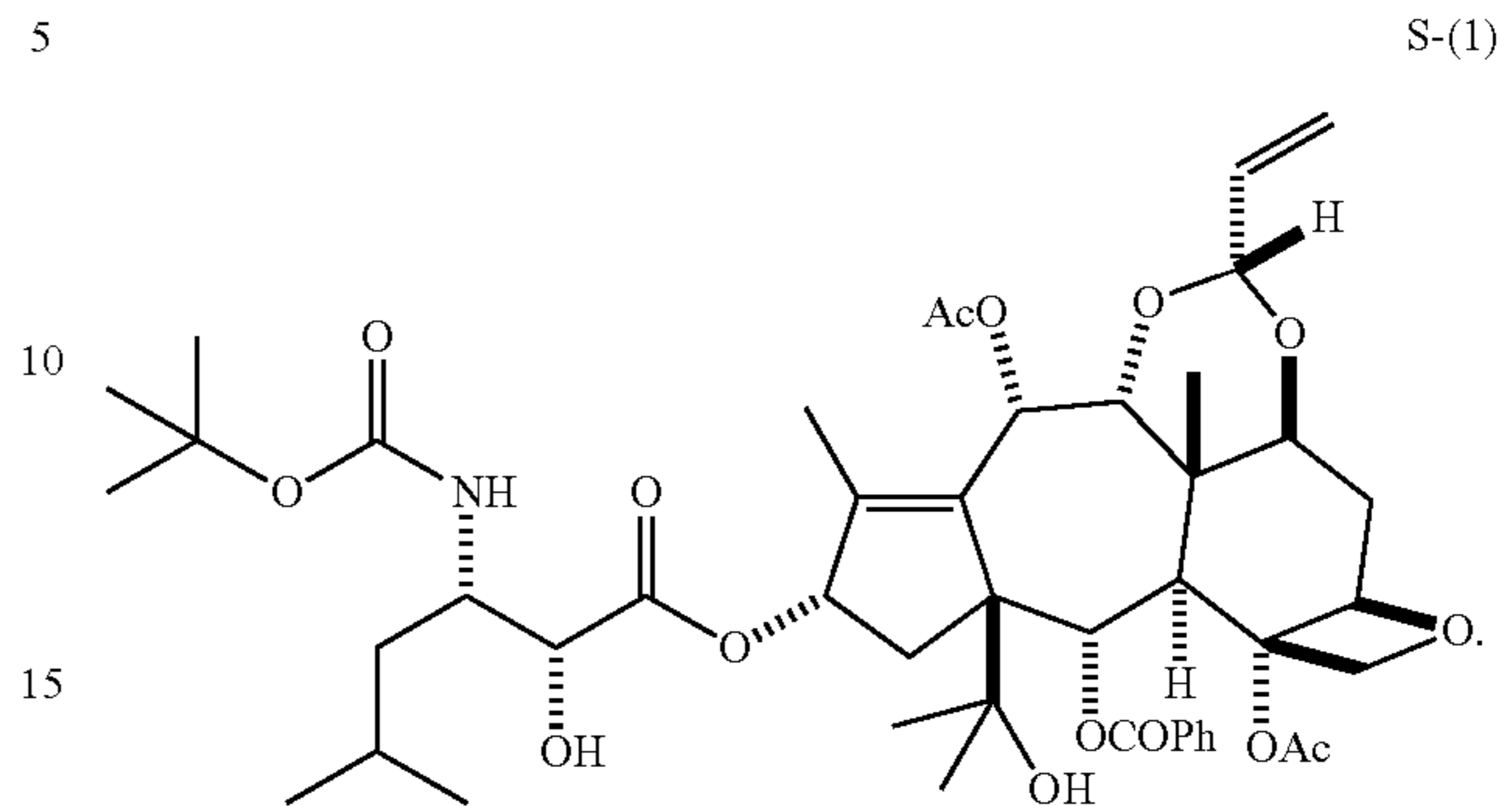
Formula (22a)
