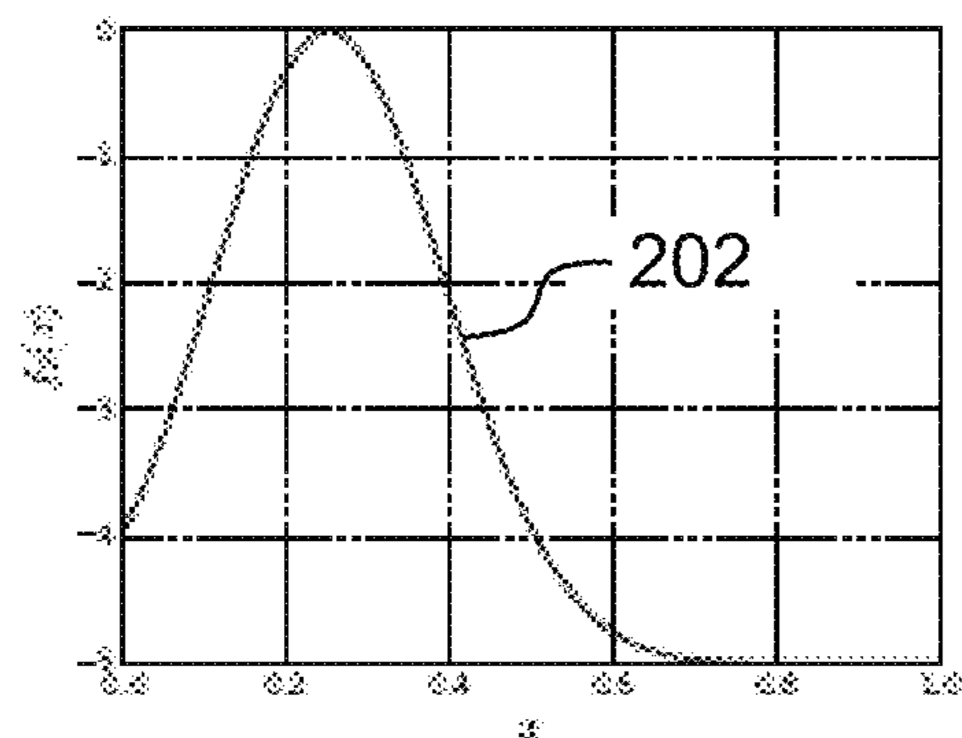
(c) f_2(x) = 5 \exp(-25(x - 0.25)^2) - 5
