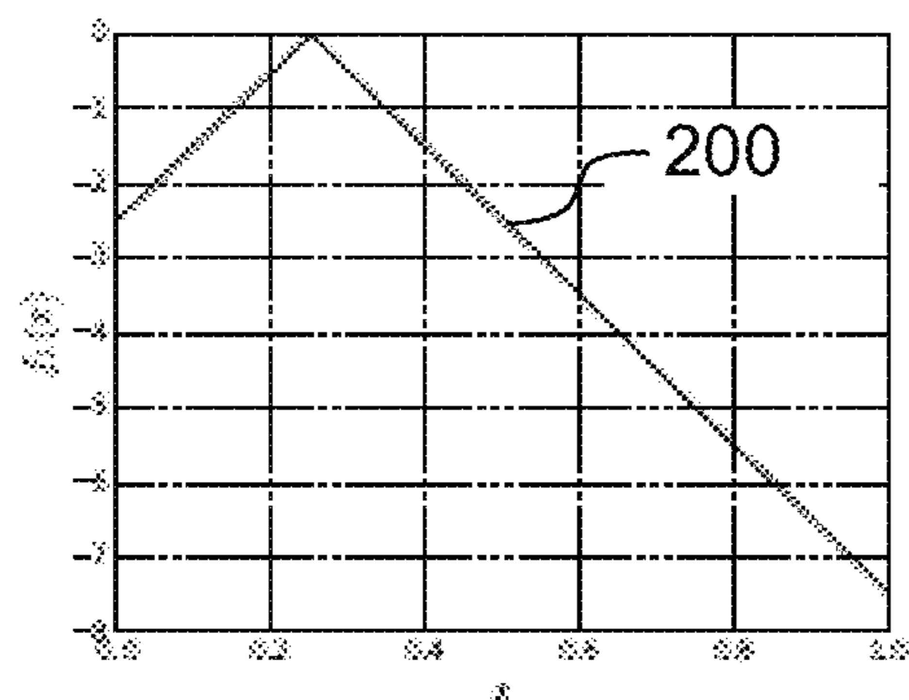
(a) f_1(x) = -\sqrt{100(x - 0.25)^2}
