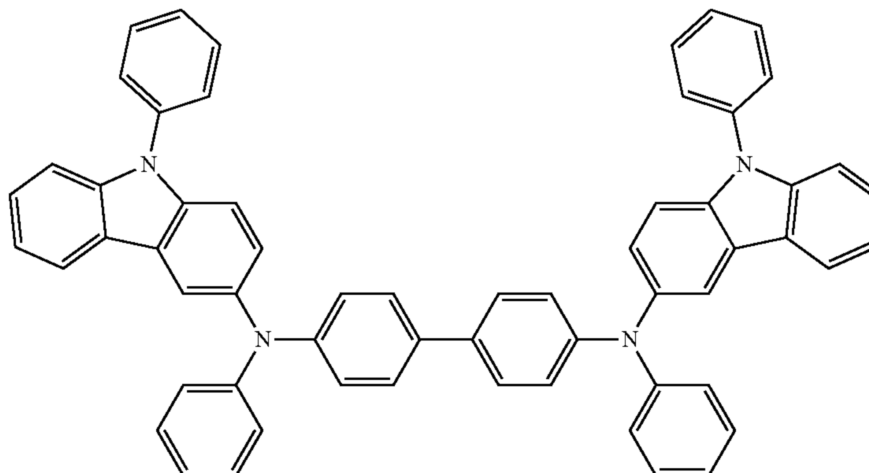
N 4 ,N 4' -diphenyl-N 4 ,N 4' -bis(9-phenyl-9H-carbazol-3-yl)-[1,1'-biphenyl]-4,4'-diamine
