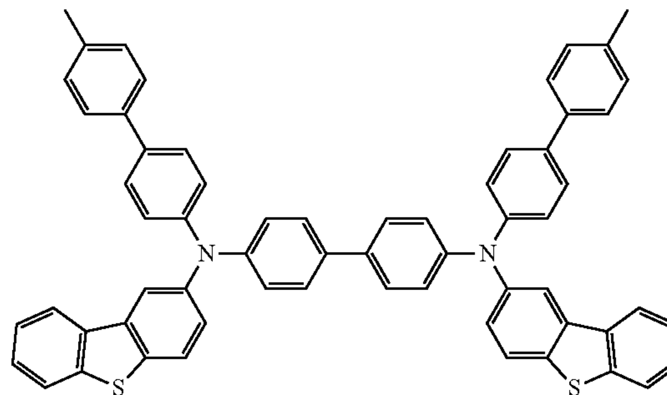
N 4 ,N 4' -bis(dibenzo[b,d]thiophen-2-yl)-N 4 ,N 4' -bis(4'-methyl-[1,1'-biphenyl]-4-yl)-[1,1'-biphenyl]-4,4'-diamine
