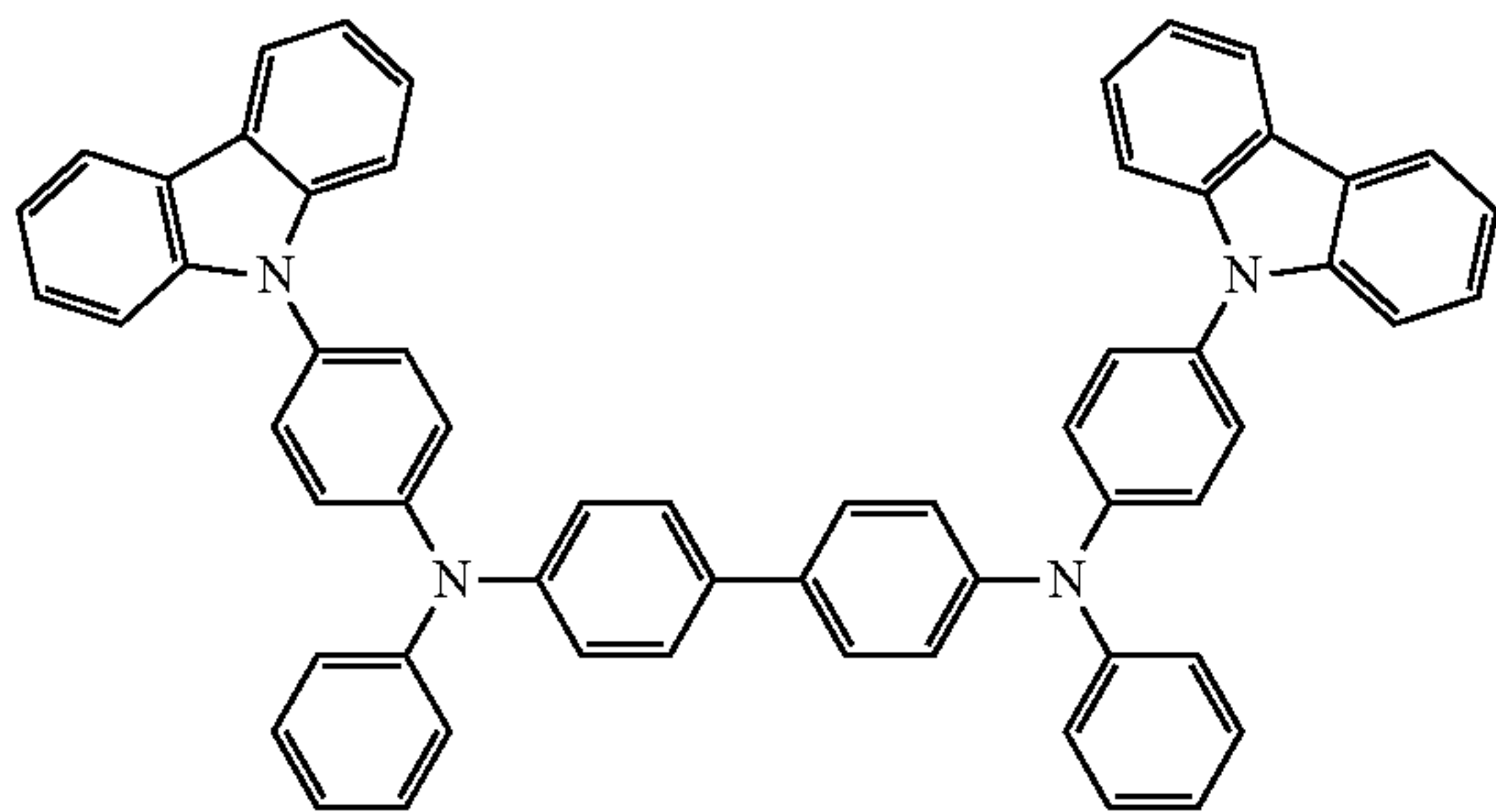
N^4, N^{4'} -bis(4-(9H-carbazol-9-yl)phenyl)- N^4, N^{4'} -diphenyl-[1,1'-biphenyl]-4,4'-diamine
