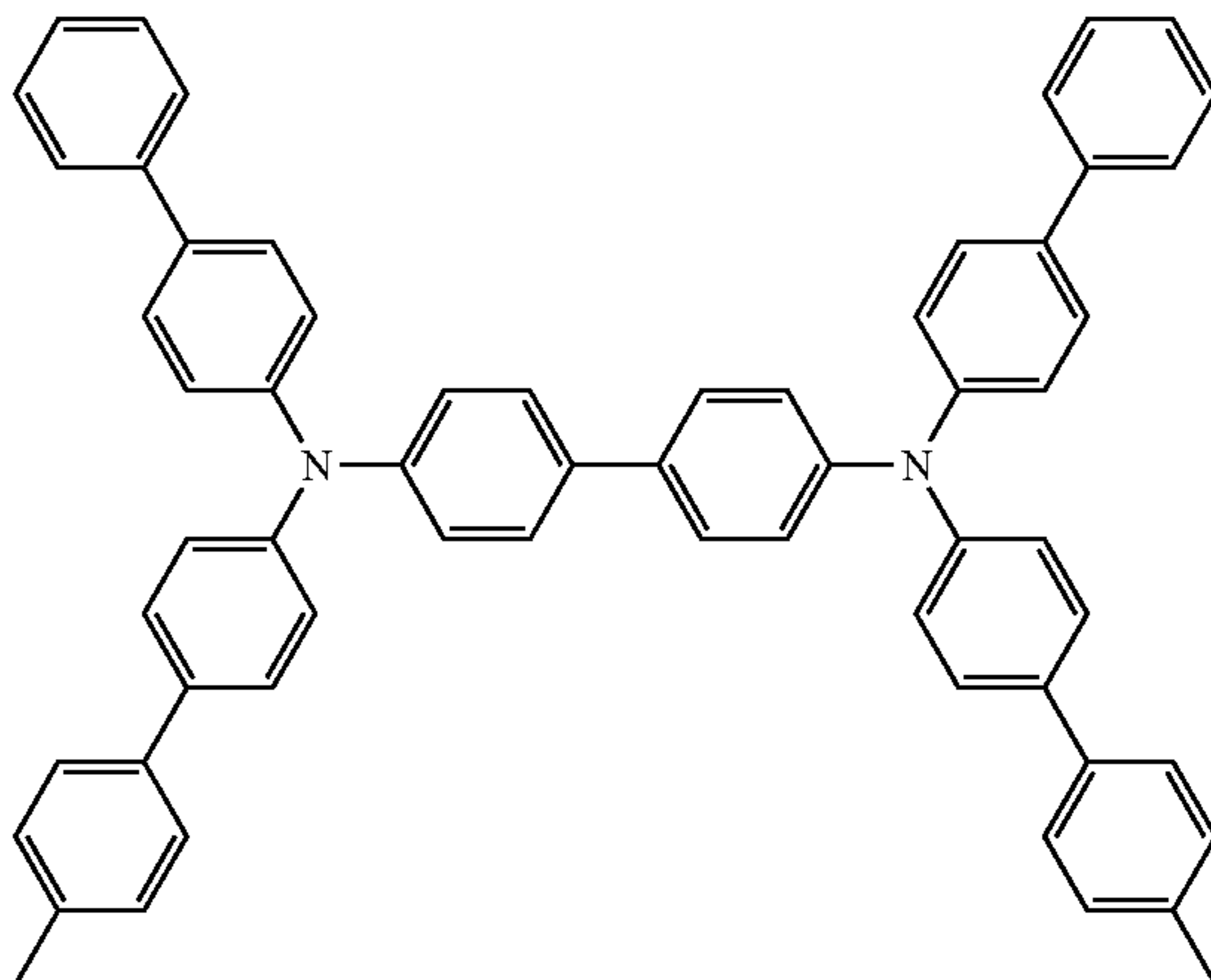
N^4, N^{4'} -di([1,1'-biphenyl]-4-yl)- N^4, N^{4'} -bis(4'-methyl-[1,1'-biphenyl]-4-yl)-[1,1'-biphenyl]-4,4'-diamine
