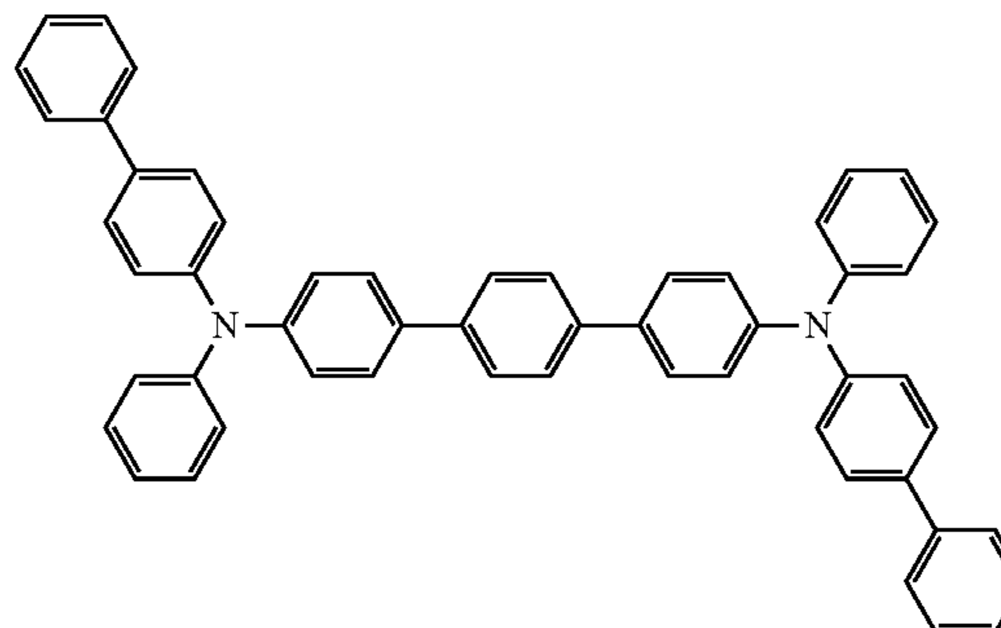
N^4, N^{4''} -di([1,1'-biphenyl]-4-yl)- N^{4'}, N^{4''} -diphenyl-[1,1':4',1''-terphenyl]-4,4''-diamine
