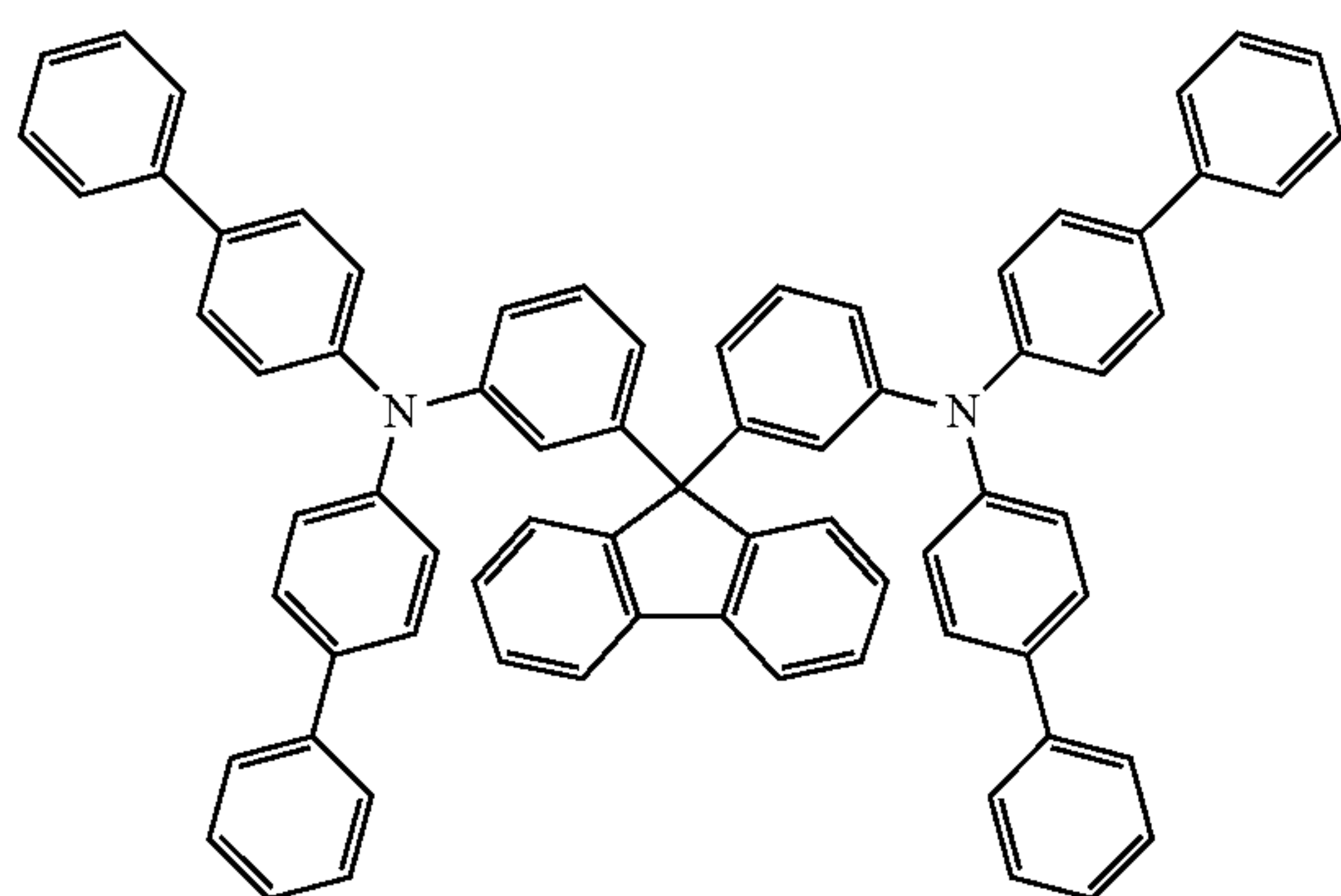
N,N'-((9H-fluorene-9,9-diyl)bis(3,1-phenylene))bis(N-[1,1'-biphenyl]-4-yl)-[1,1'-biphenyl]-4-amine
