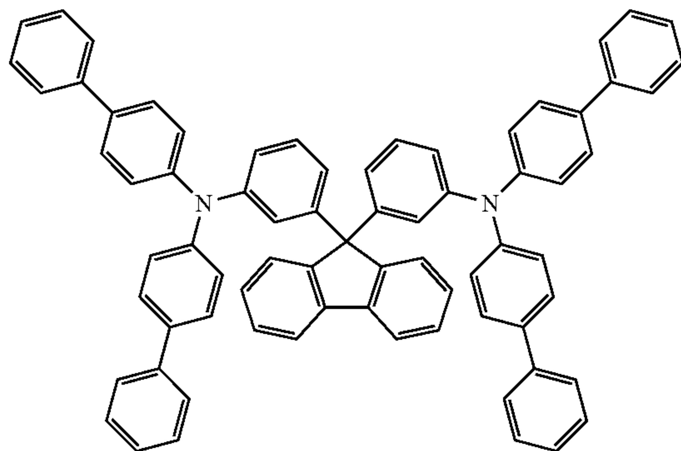
N,N'-((9H-fluorene-9,9-diyl)bis(3,1-phenylene))bis(N-[1,1'-biphenyl]-4-yl)-[1,1'-biphenyl]-4-amine)
