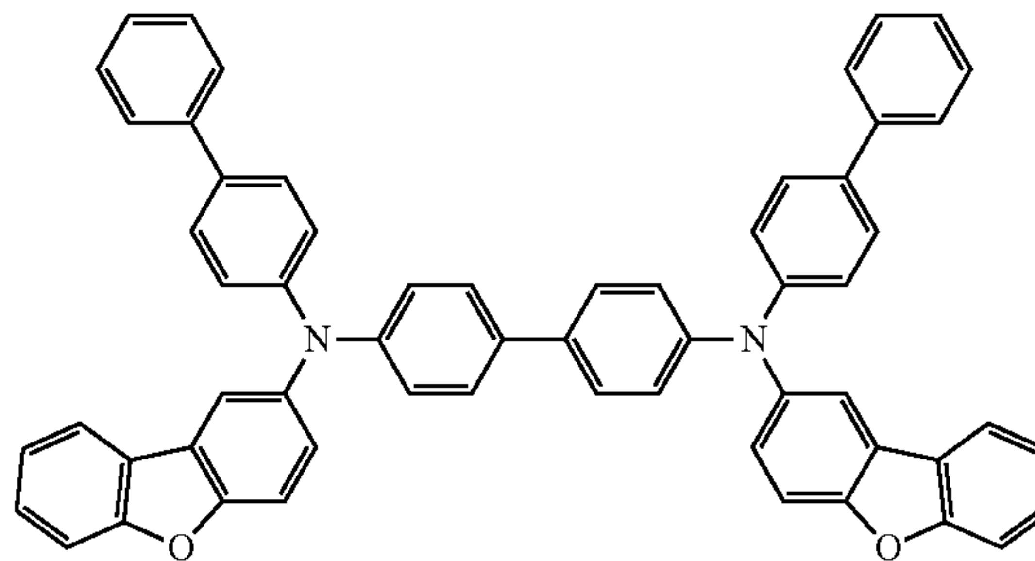
N^4, N^{4'} -di([1,1'-biphenyl]-4-yl)- N^4, N^{4'} -bis(dibenzo[b,d]furan-2-yl)-[1,1'-biphenyl]-4,4'-diamine
