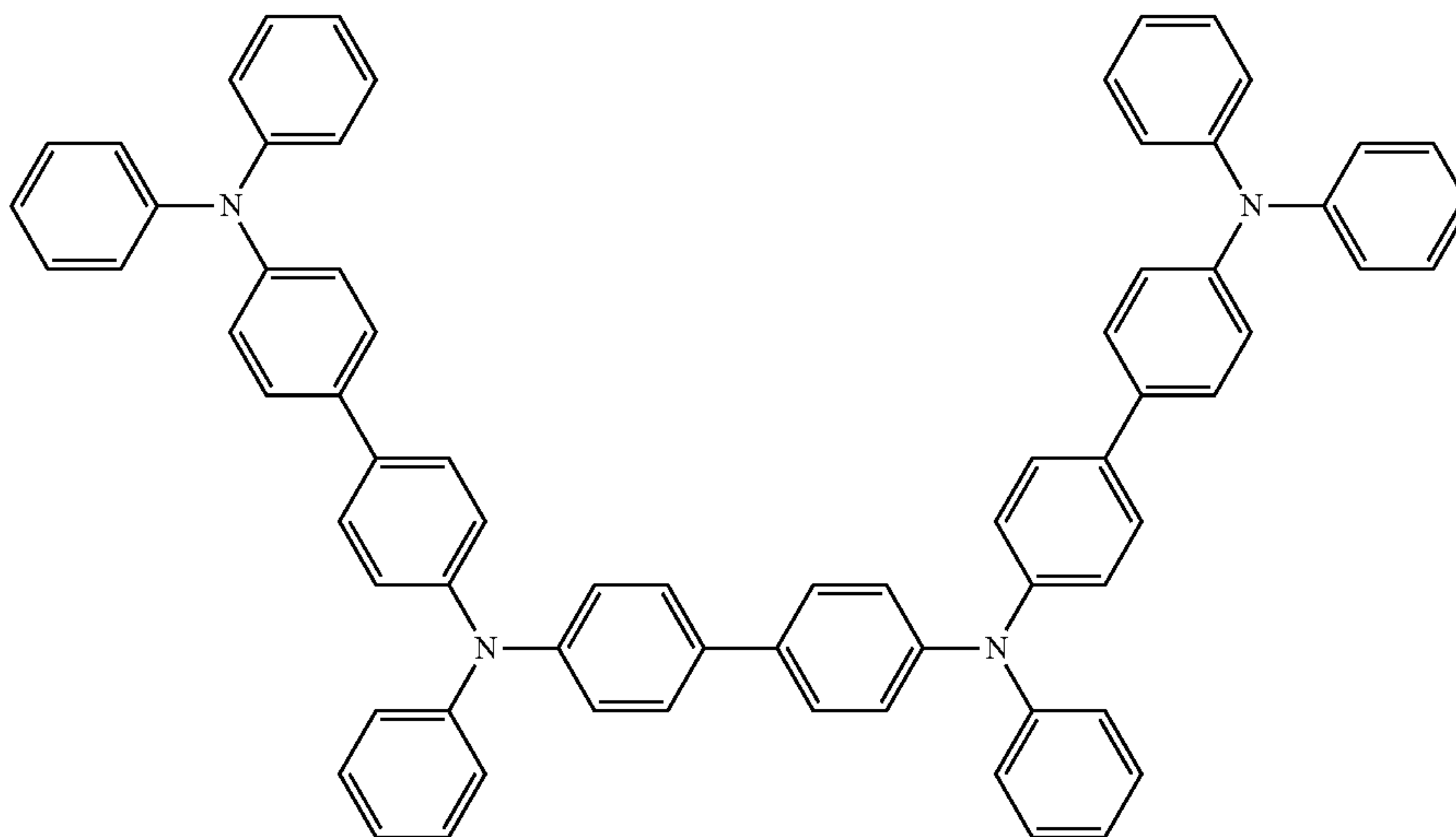
N^4, N^{4'} -([1,1'-biphenyl]-4,4'-diyl)bis( N^4, N^{4'} , N^{4'} -triphenyl-[1,1'-biphenyl]-4,4'-diamine)
