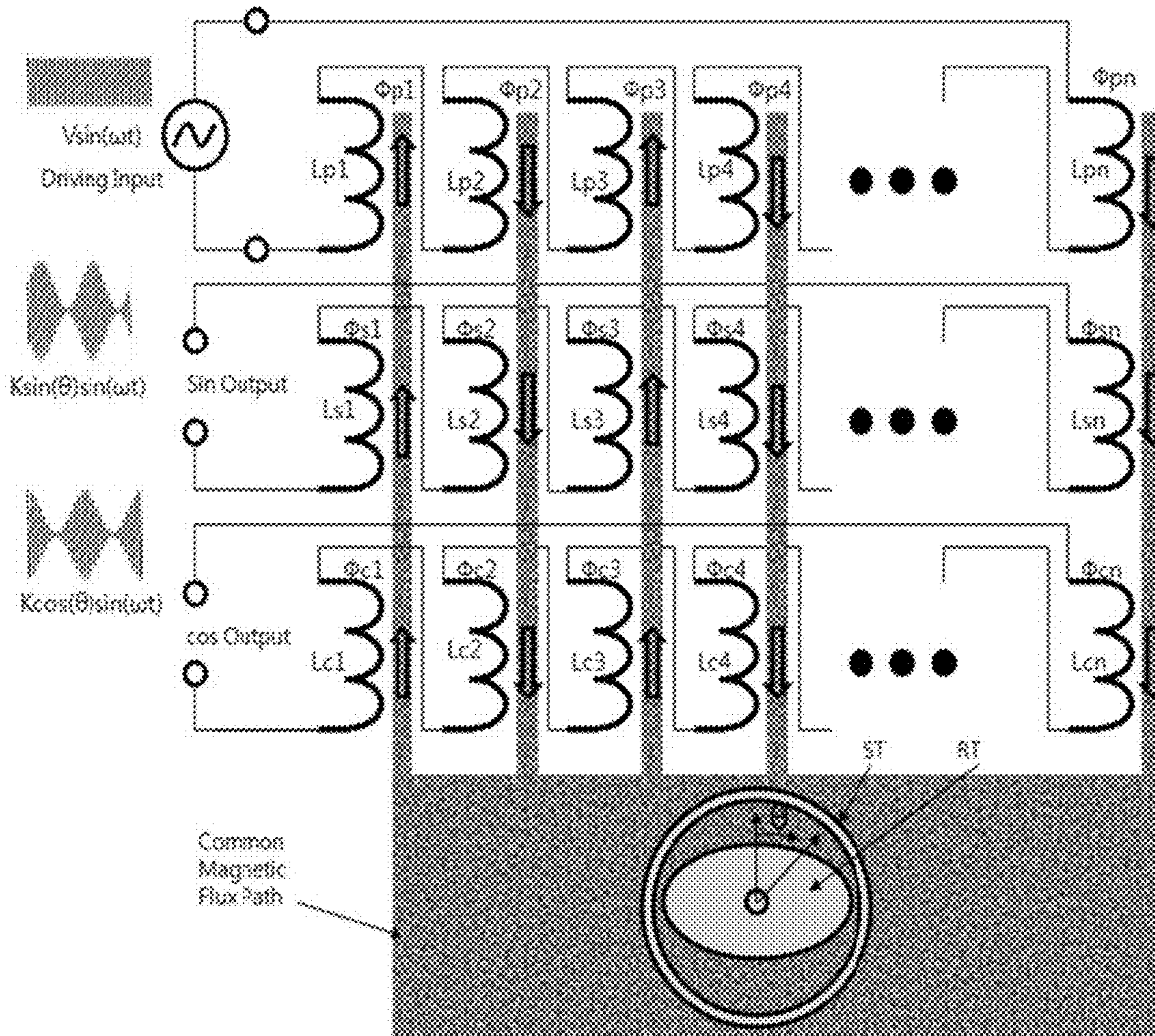
FIG. 2 PRIOR ART
