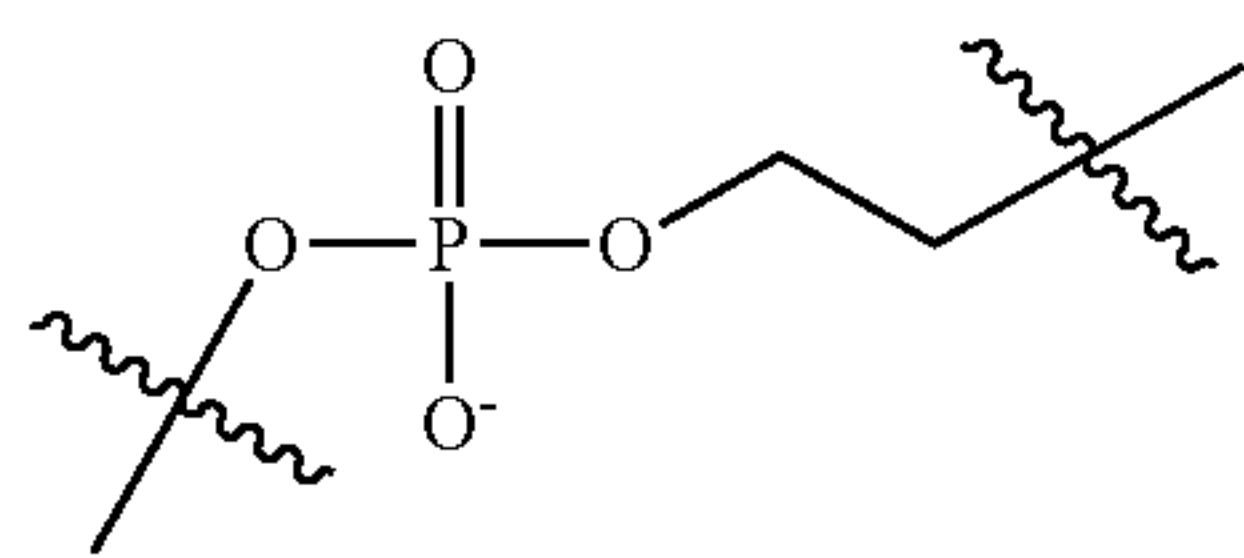
“C linker”
