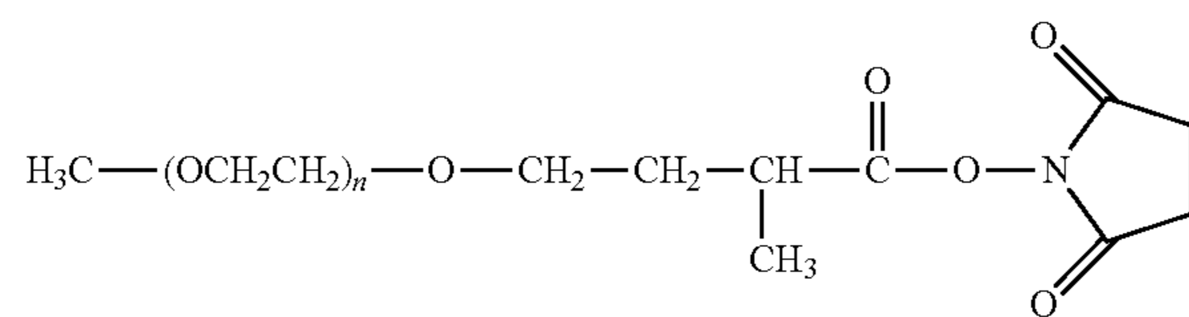
mPEG-Succinimidyl Derivative
