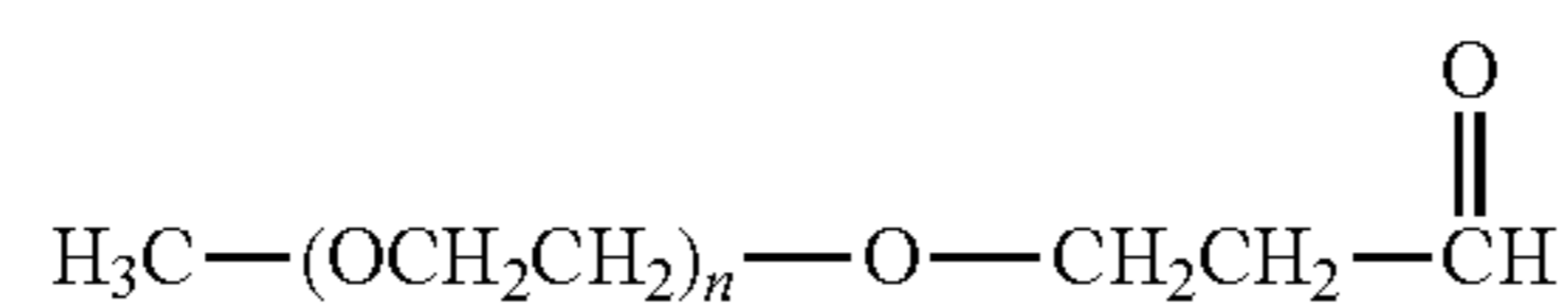
mPEG Propionaldehyde
