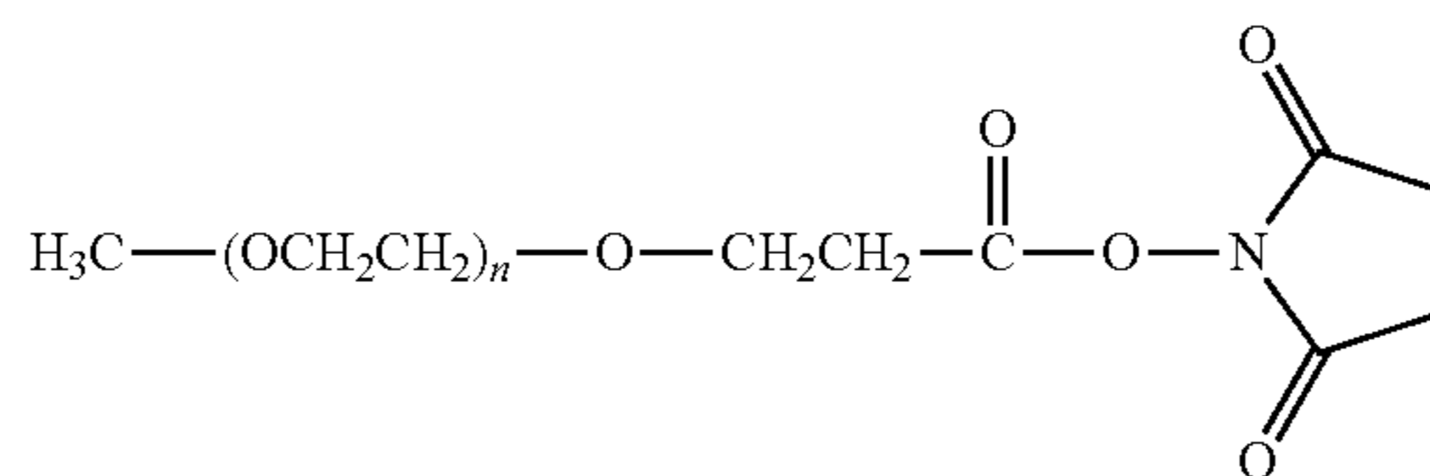
mPEG-Succinimidyl Propionate
