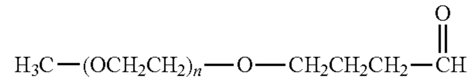
mPEG Butyraldehyde
