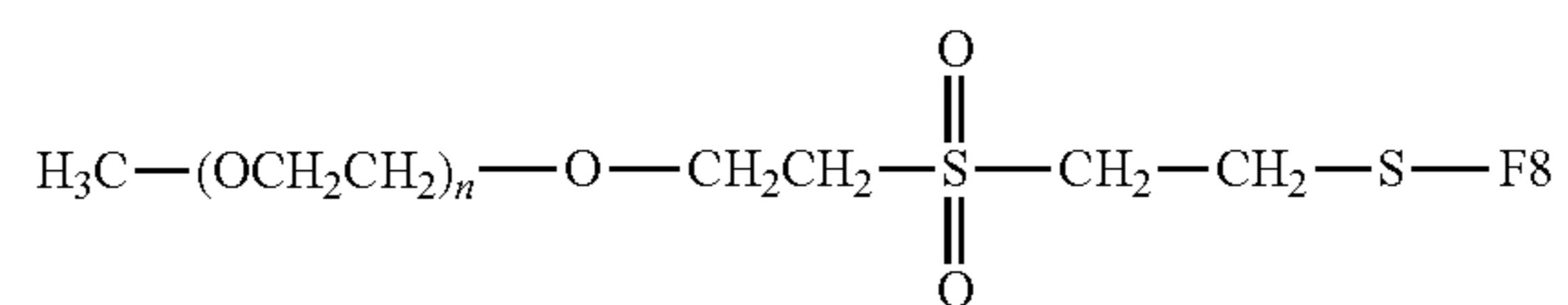
Thioether Linkage
