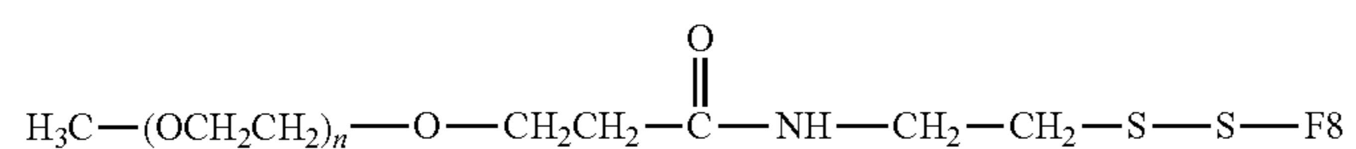
Disulfide Linkage
