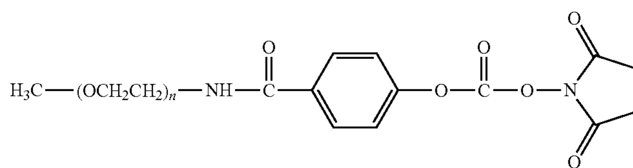
mPEG-Succinimidyl Derivative
