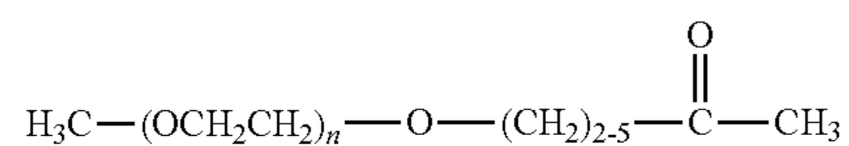
mPEG Methylketone
