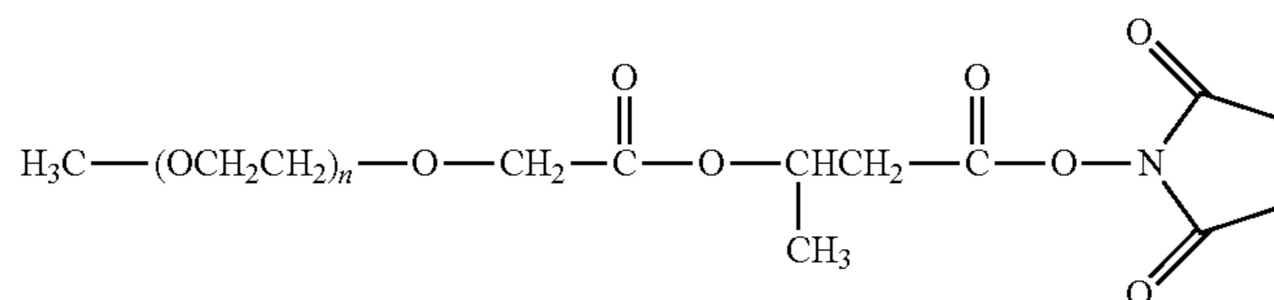
mPEG-Succinimidyl Derivative
