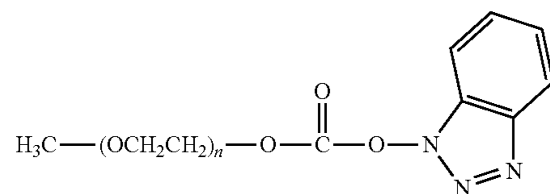
mPEG-Benzotriazole Carbonate
