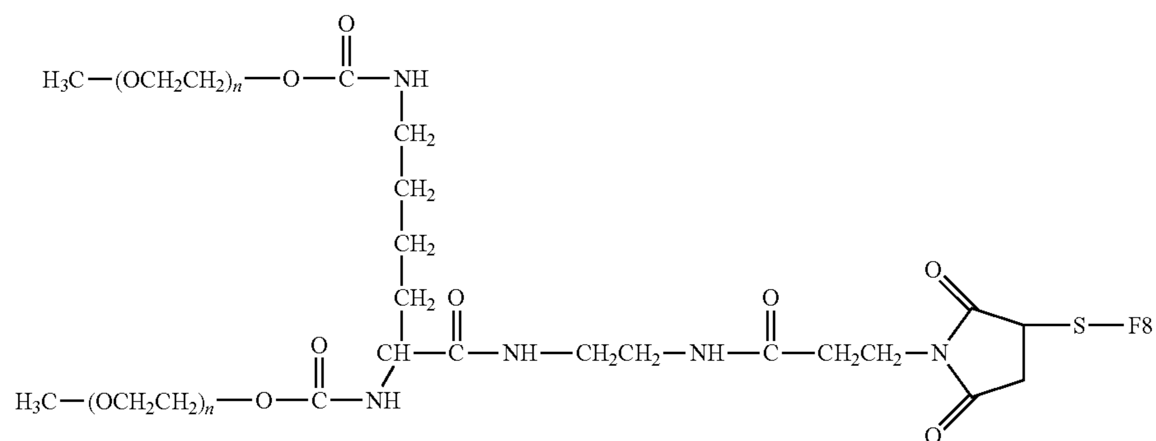
Thioether Linkage
