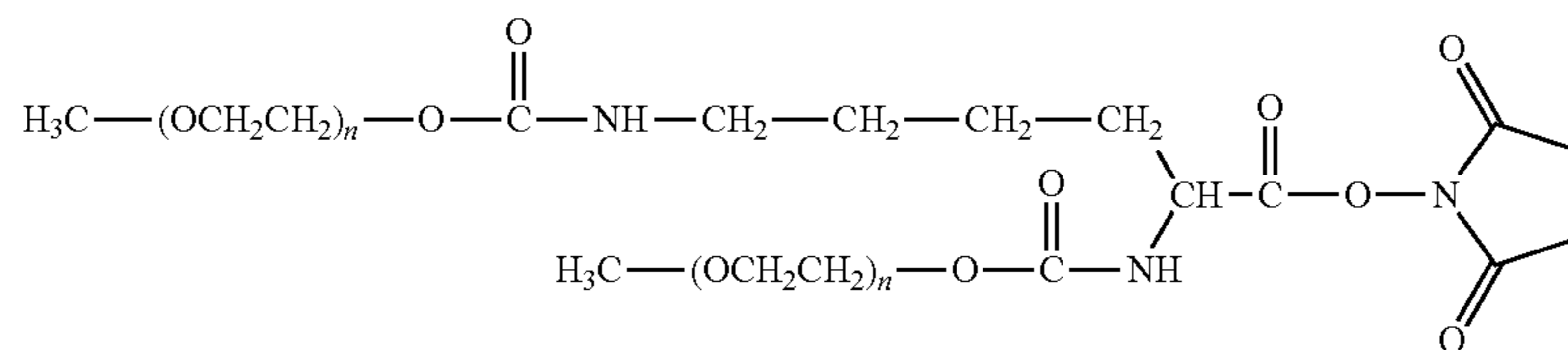
Branched mPEG2-N-Hydroxysuccinimide
