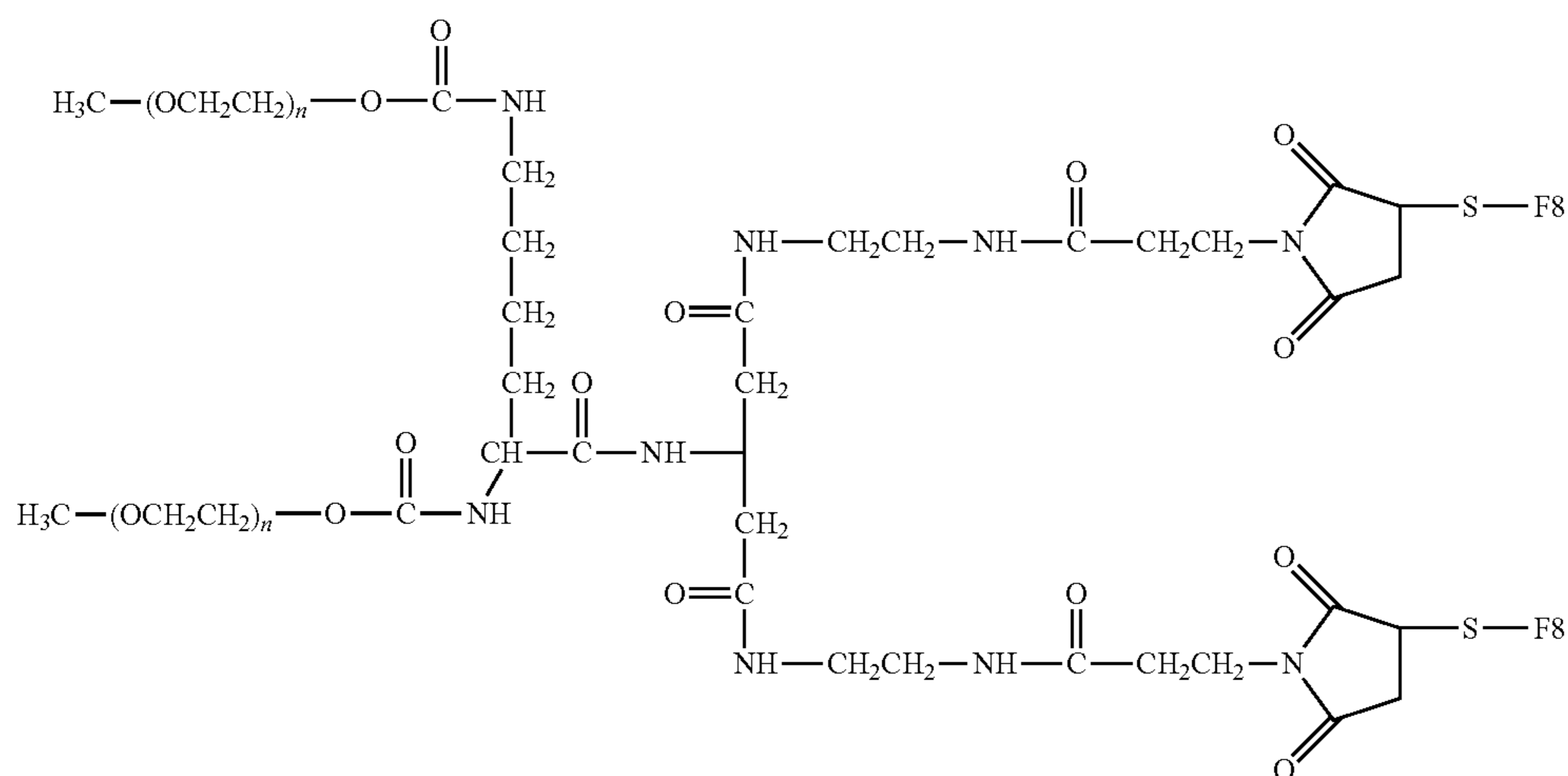
Thioether Linkages
