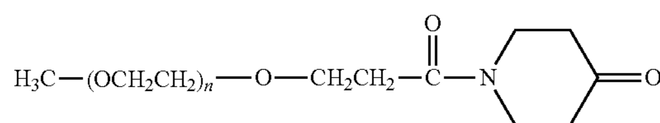
mPEG Piperidone
