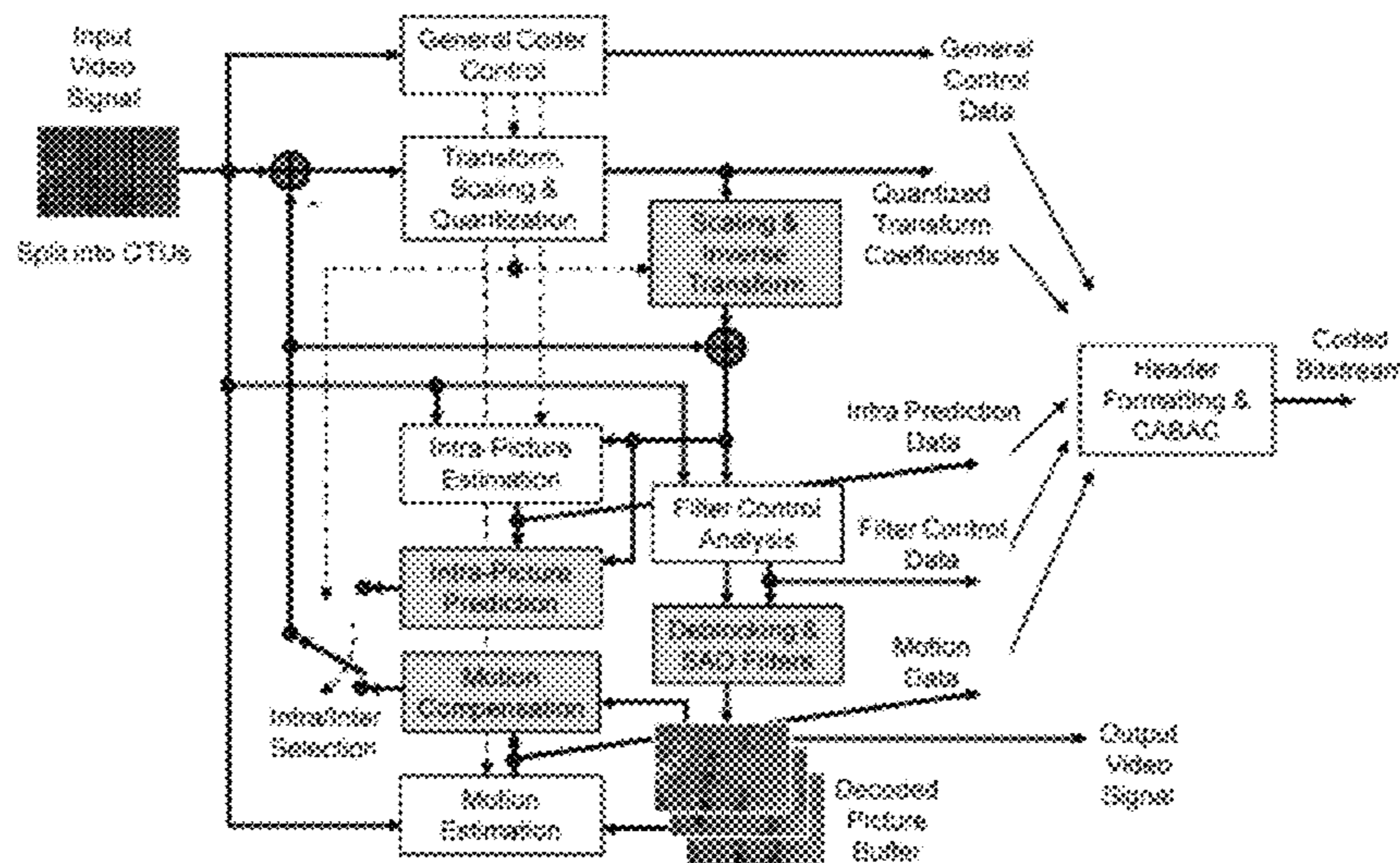
Typical HEVC video encoder with decoder modeling blocks shaded in light gray.
