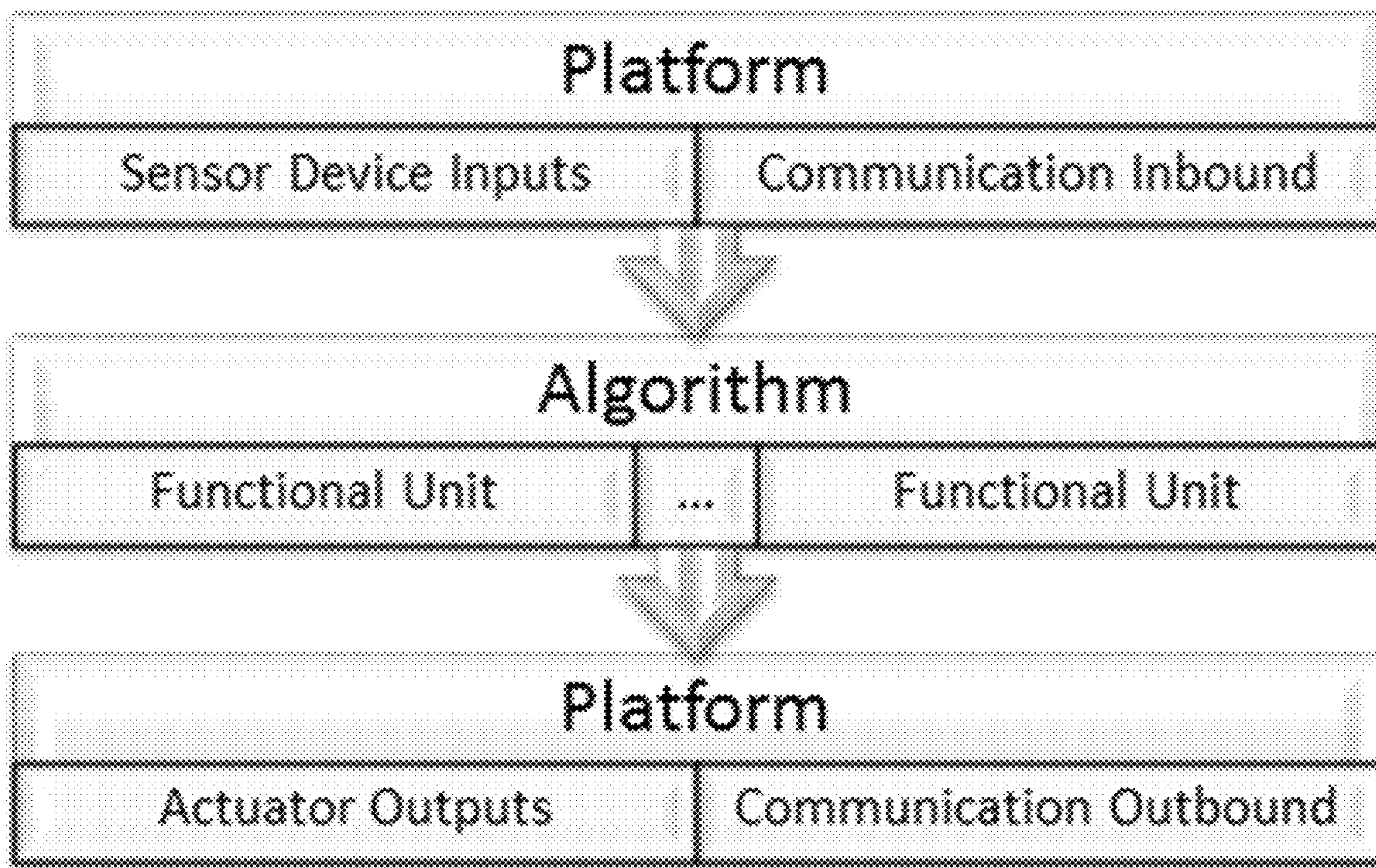
ASL Framework data flow
