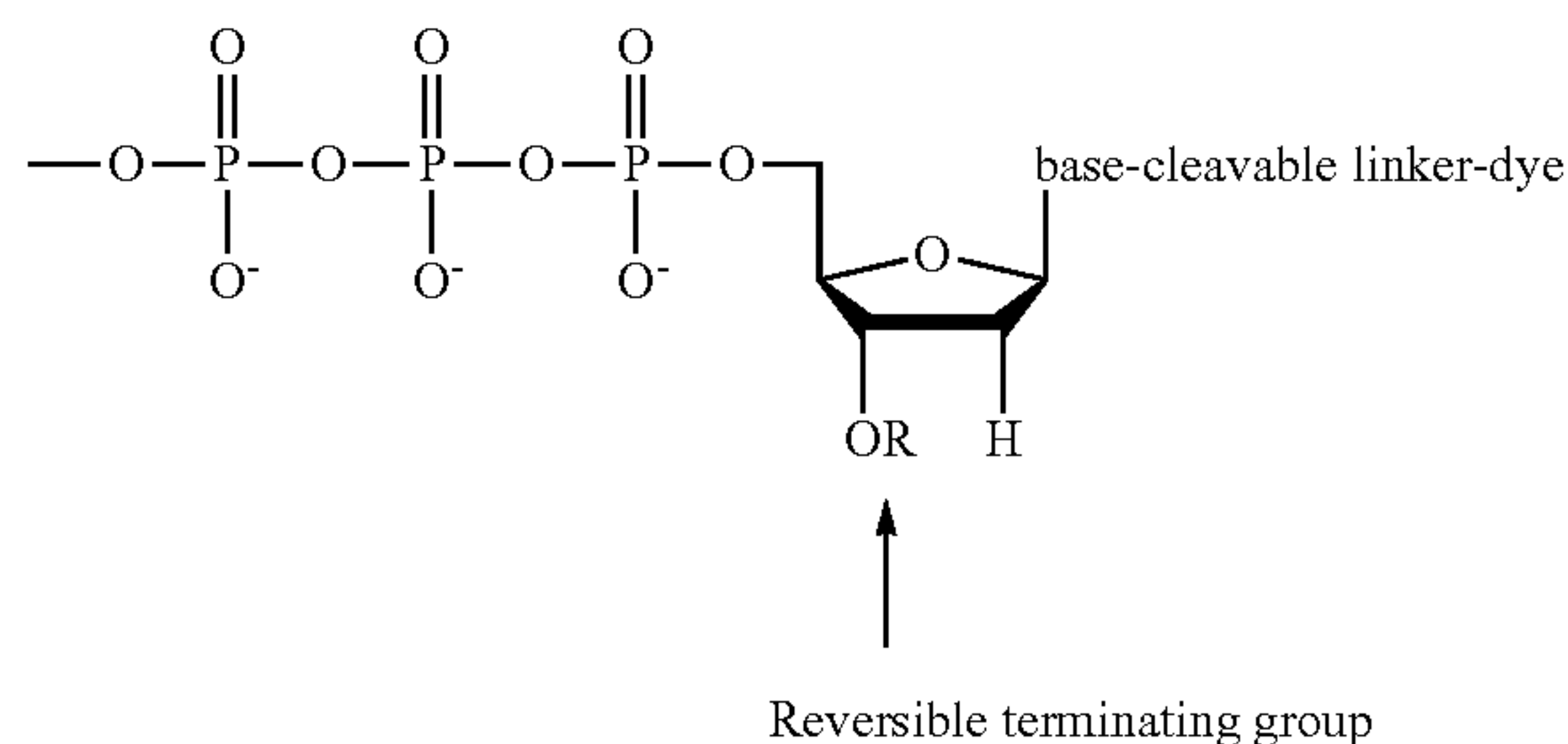
3'-O-blocked reversible terminator
