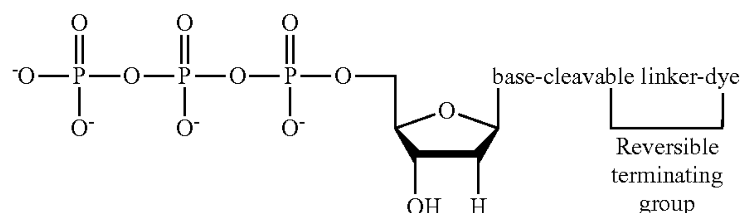
3'-unblocked reversible terminator
