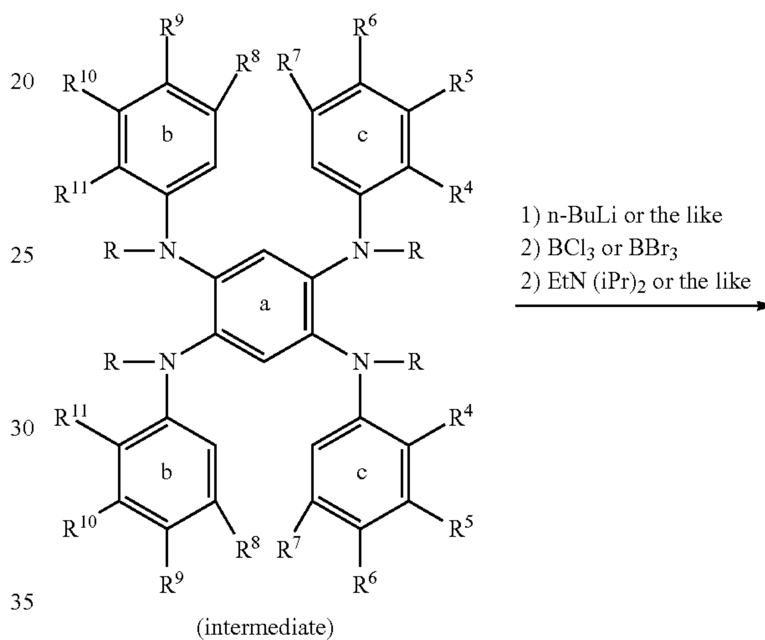
scheme (3)
