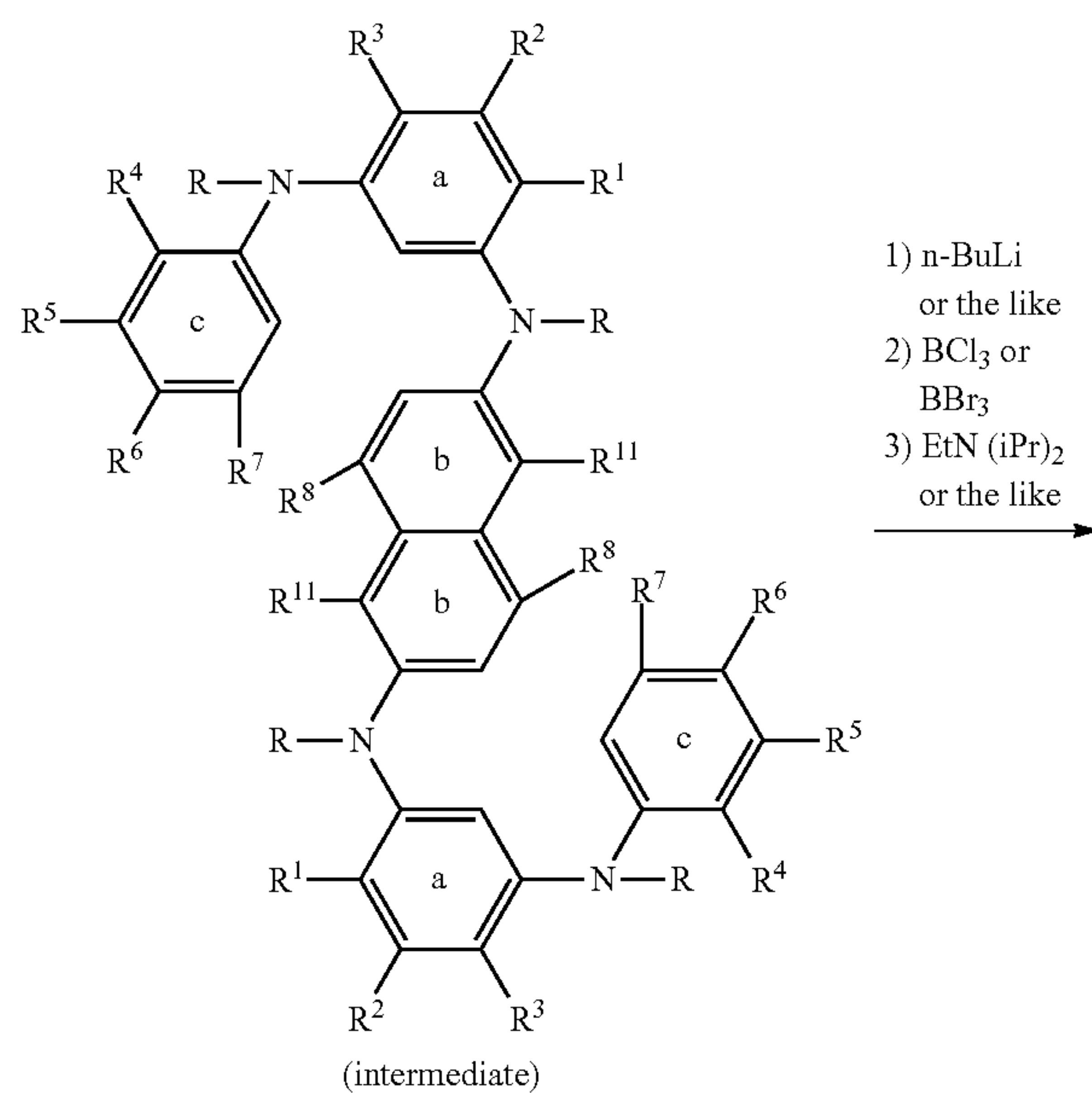
scheme (5)
