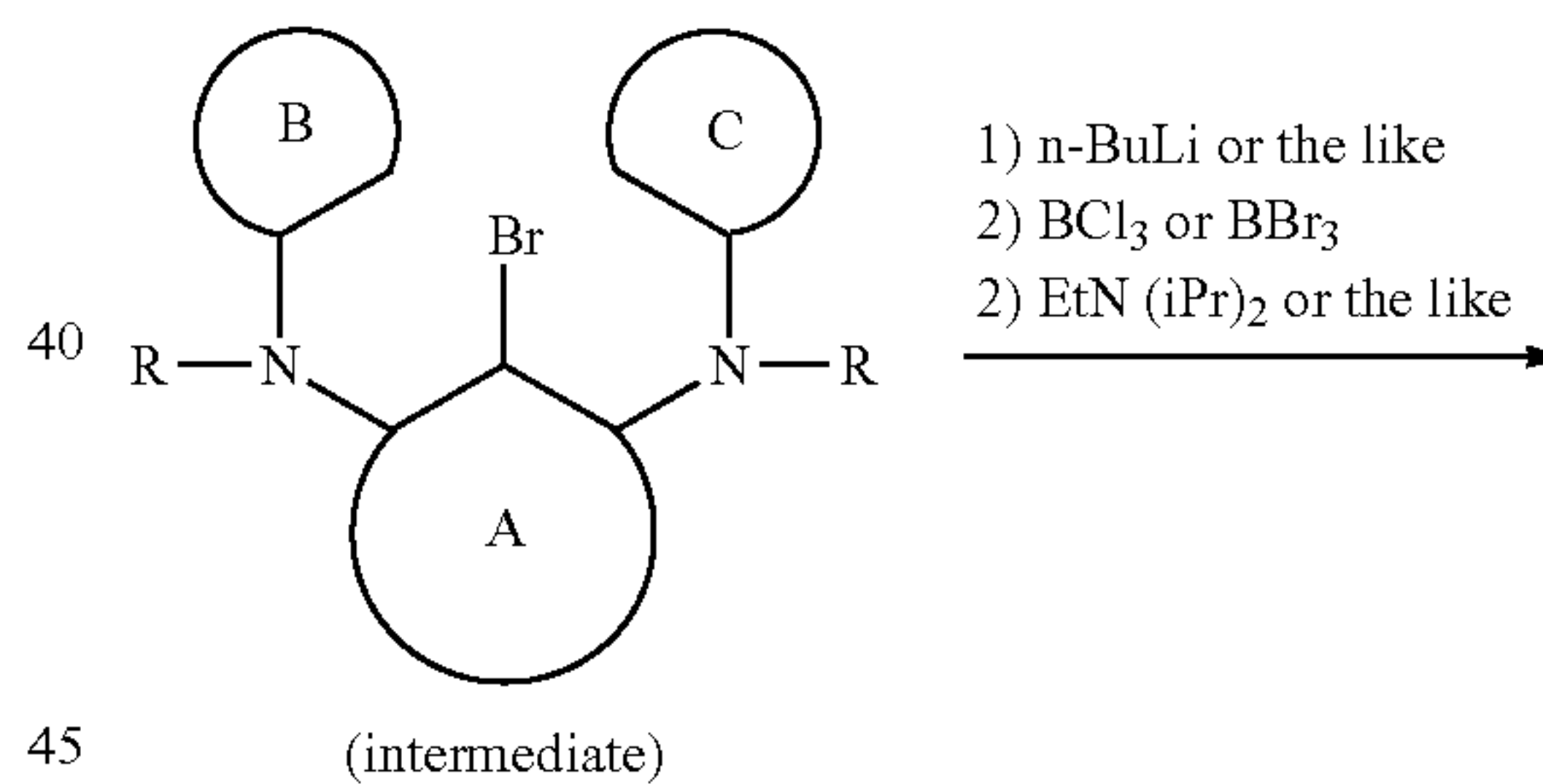
scheme (6)
