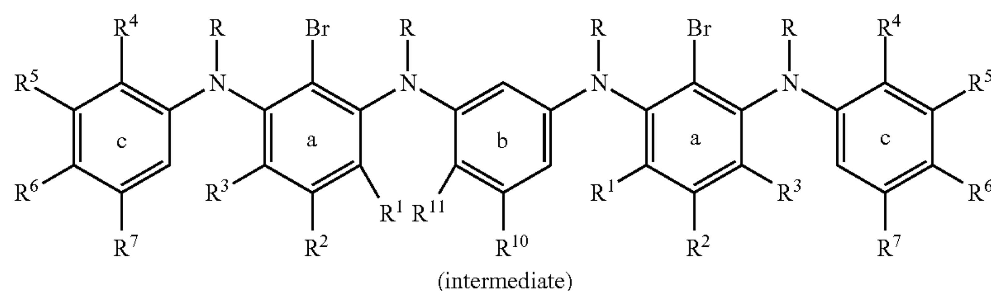
scheme (10)
