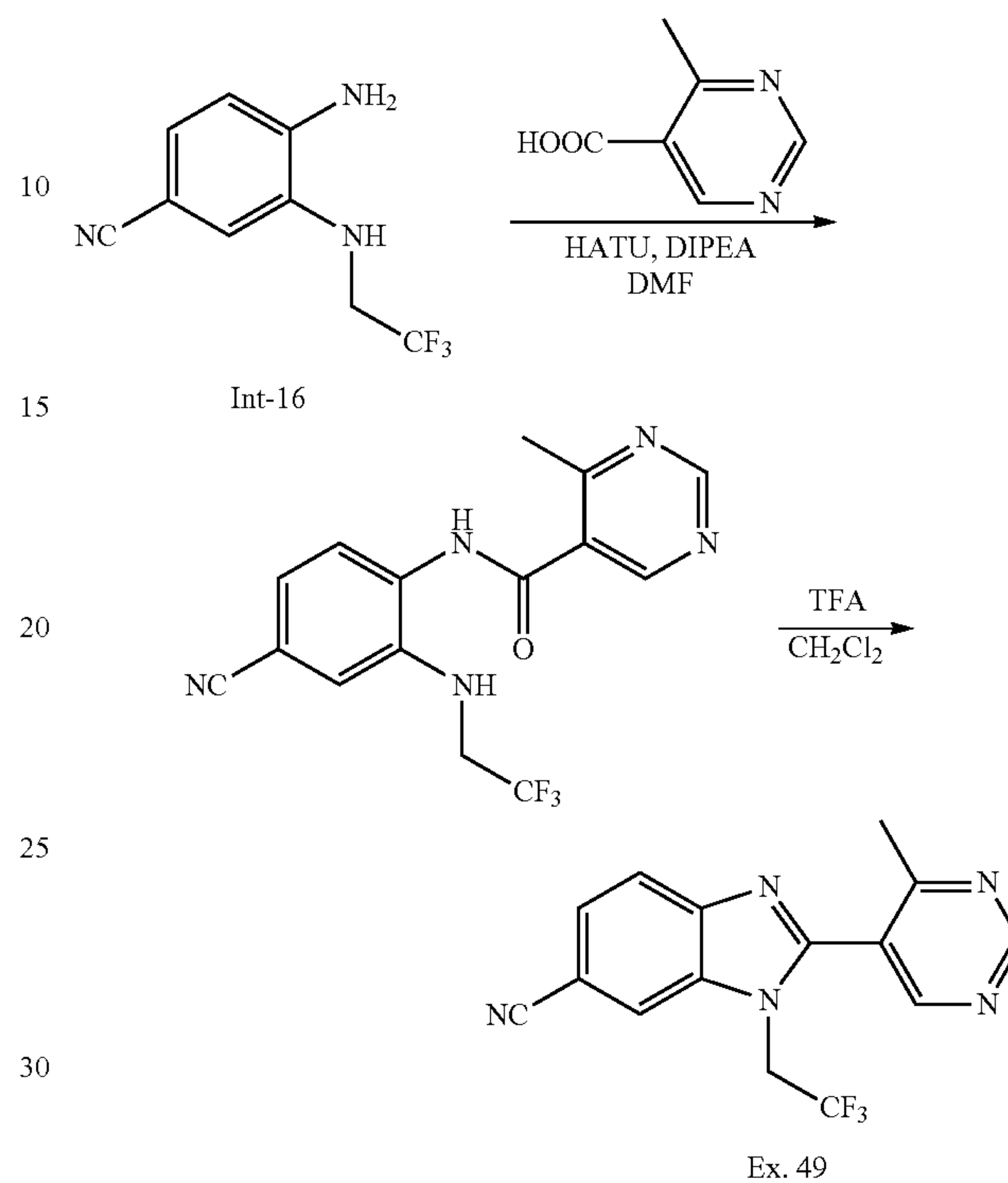
N-(4-Cyano-2-((2,2,2-trifluoroethyl)amino)phenyl)-4-methylpyrimidine-5-carboxamide
