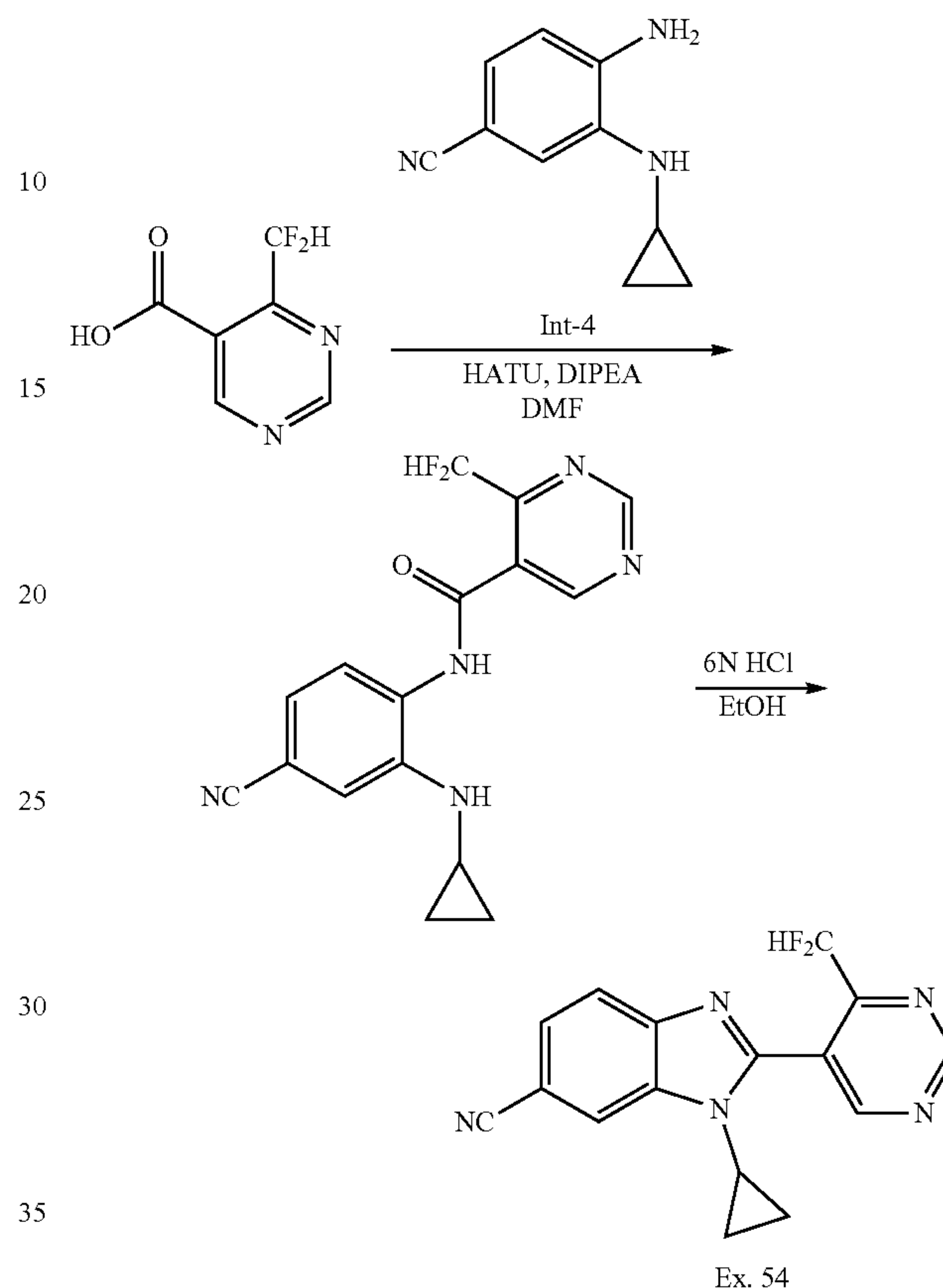
N-(4-Cyano-2-(cyclopropylamino)phenyl)-4-(difluoromethyl)pyrimidine-5-carboxamide
