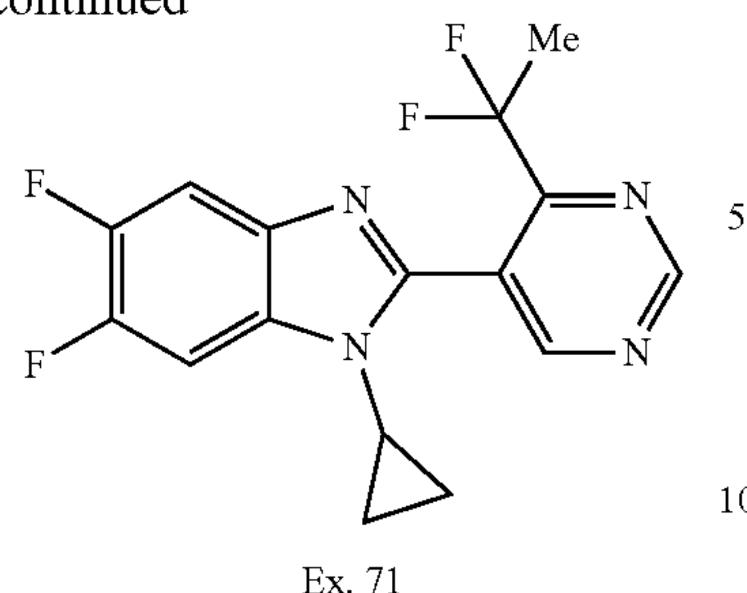
1-Cyclopropyl-2-(4-(1,1-difluoroethyl)pyrimidin-5-yl)-5,6-difluoro-1H-benzo[d]imidazole (Ex. 71)
