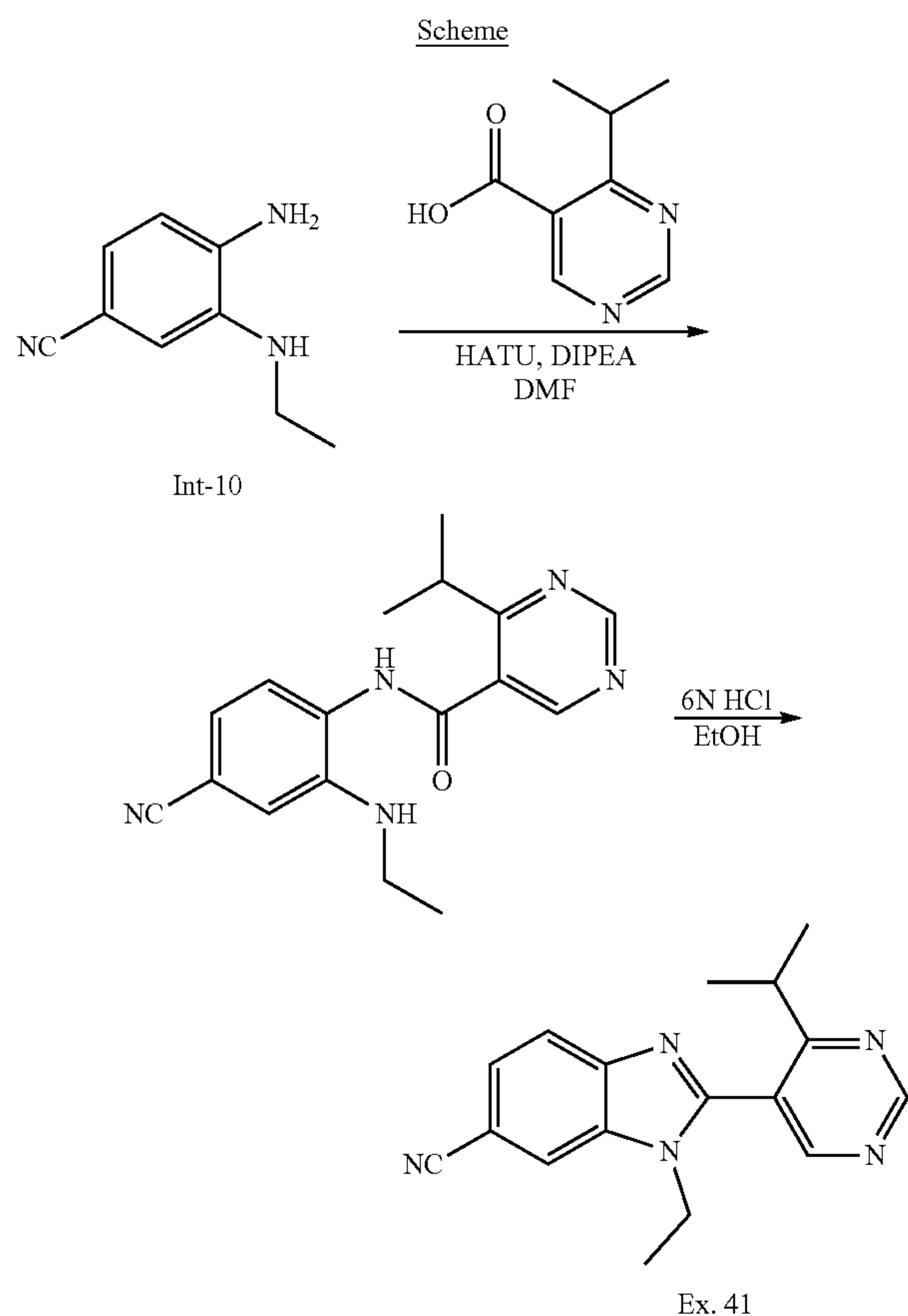
N-(4-Cyano-2-(ethylamino)phenyl)-4-isopropylpyrimidine-5-carboxamide
