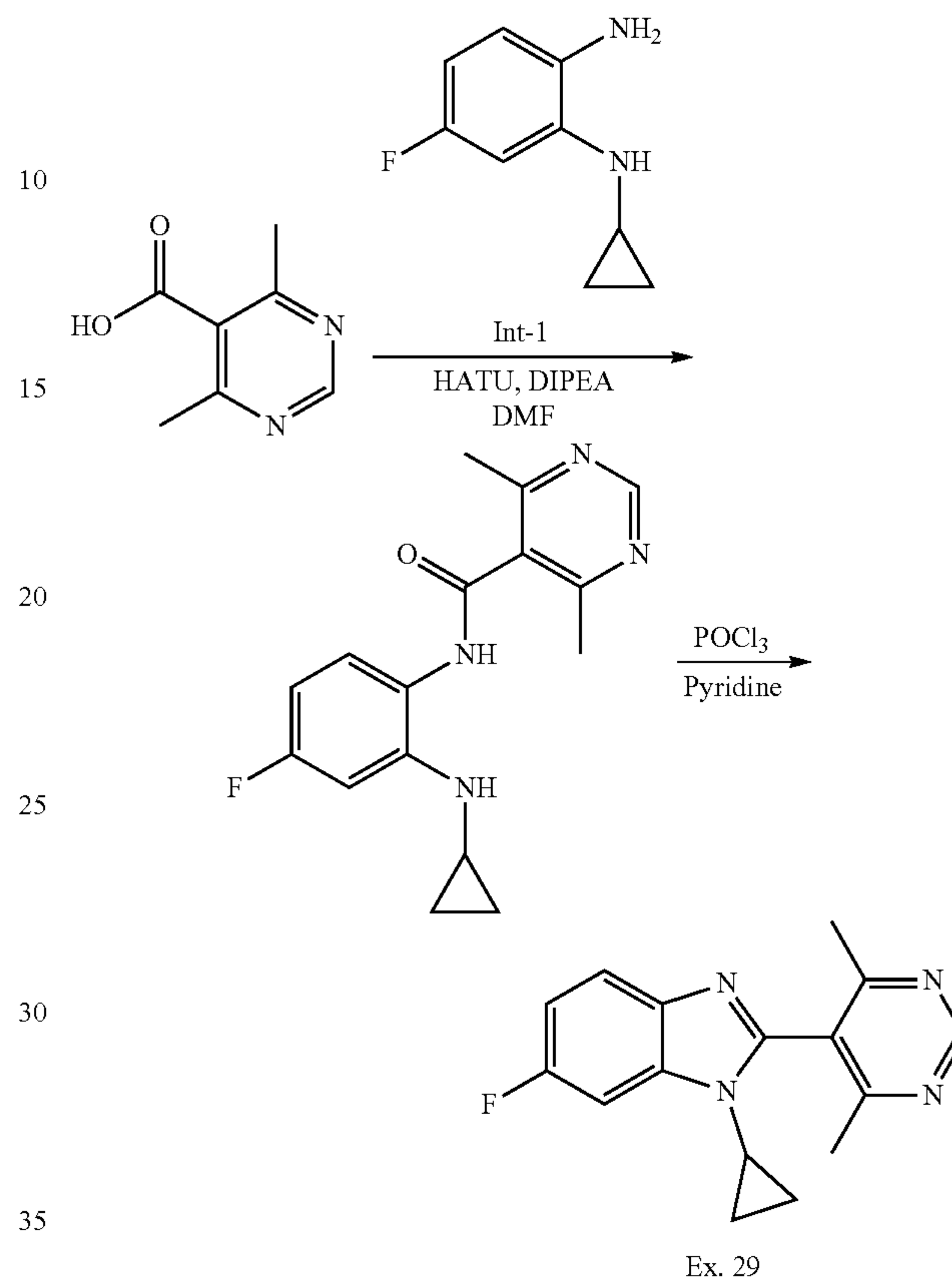
N-(2-(Cyclopropylamino)-4-fluorophenyl)-4,6-dimethylpyrimidine-5-carboxamide
