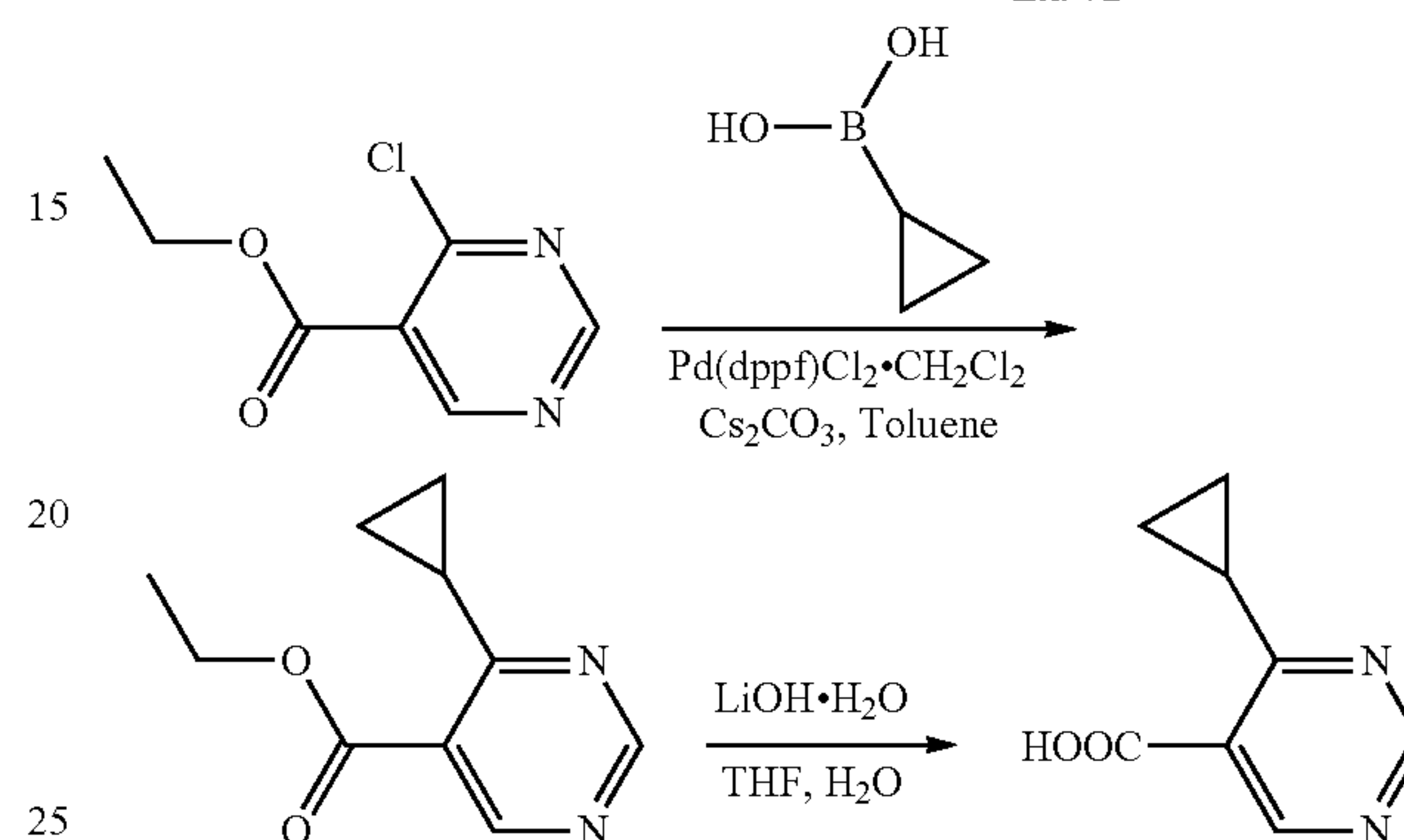
1-Cyclopropyl-2-(4-(1,1-difluoroethyl)pyrimidin-5-yl)-5,6-difluoro-1H-benzo[d]imidazole (Ex. 71)
