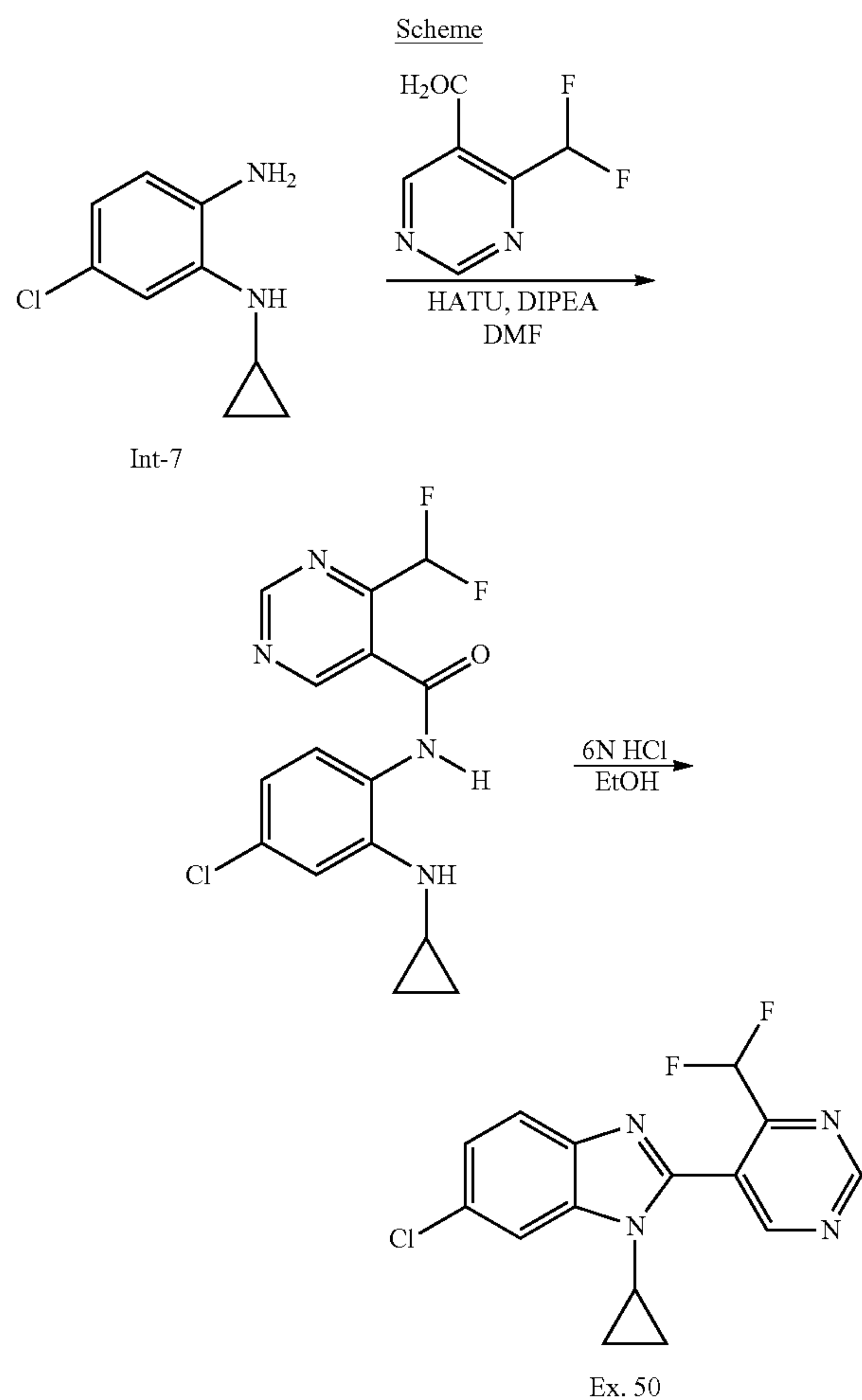
N-(4-Chloro-2-(cyclopropylamino)phenyl)-4-(difluoromethyl)pyrimidine-5-carboxamide
