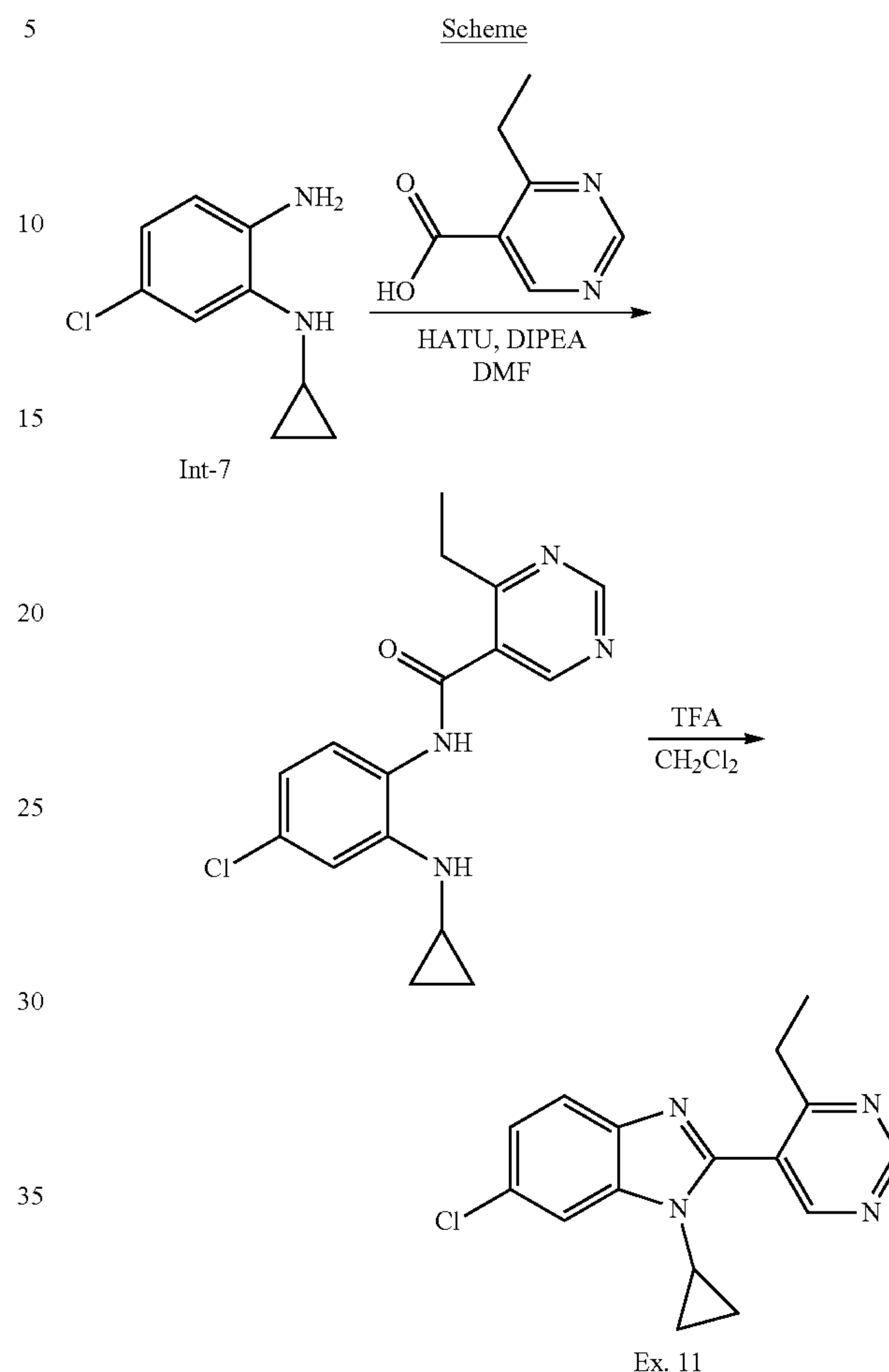
N-(4-Chloro-2-(cyclopropylamino)phenyl)-4-ethylpyrimidine-5-carboxamide
