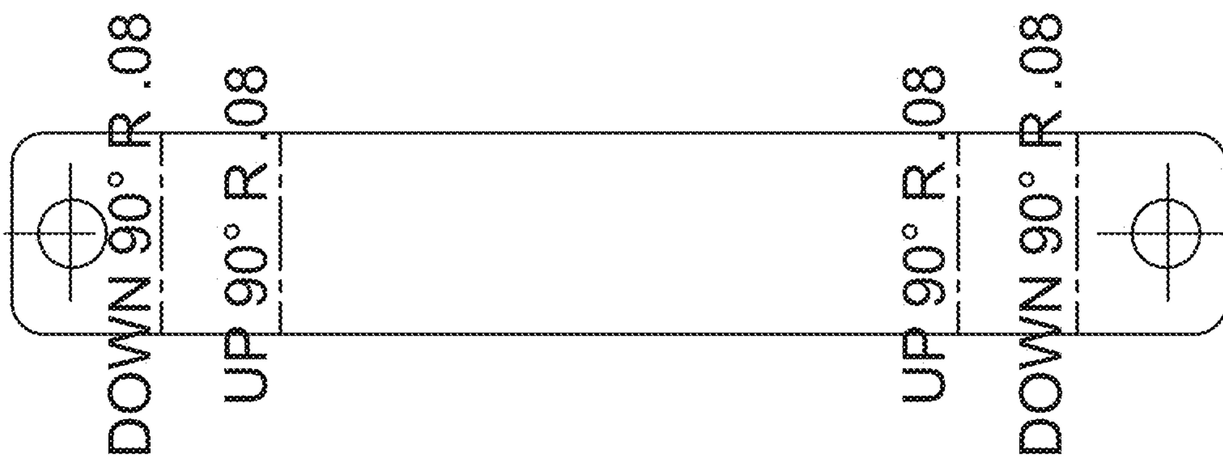
FLAT PATTERN
