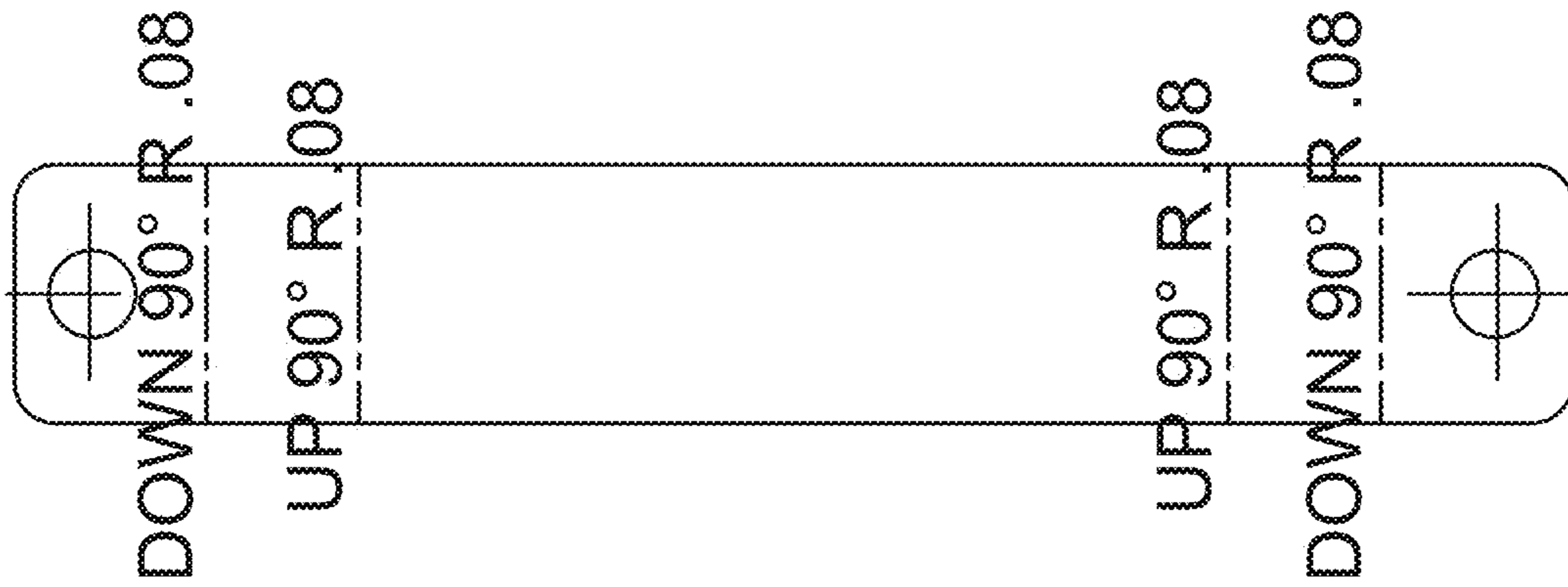
FLAT PATTERN FIG. 9B
