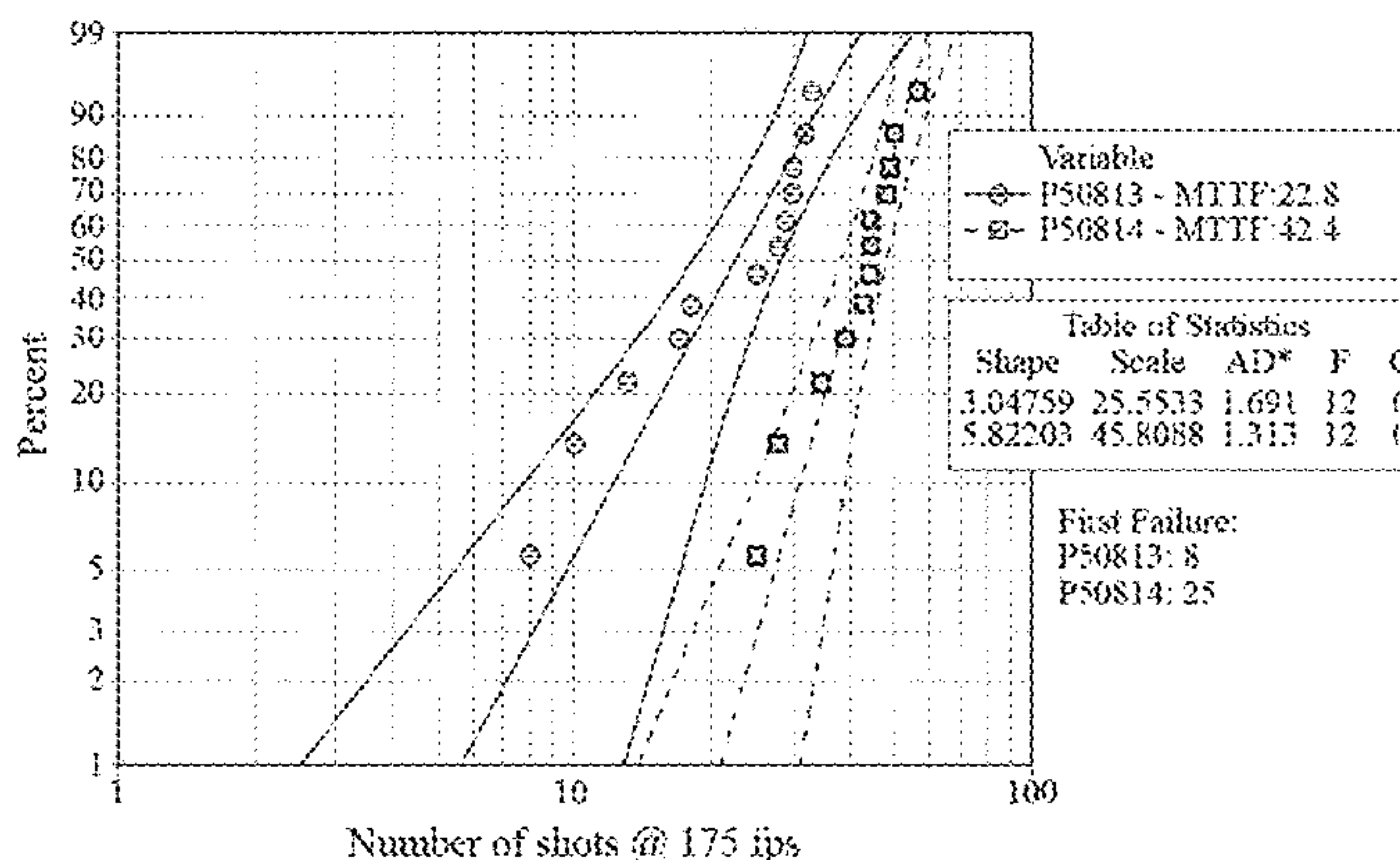
Paraloid Impact Modifier Mantle Failure
