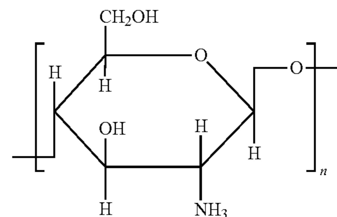
Chemical structure of polysaccharide
