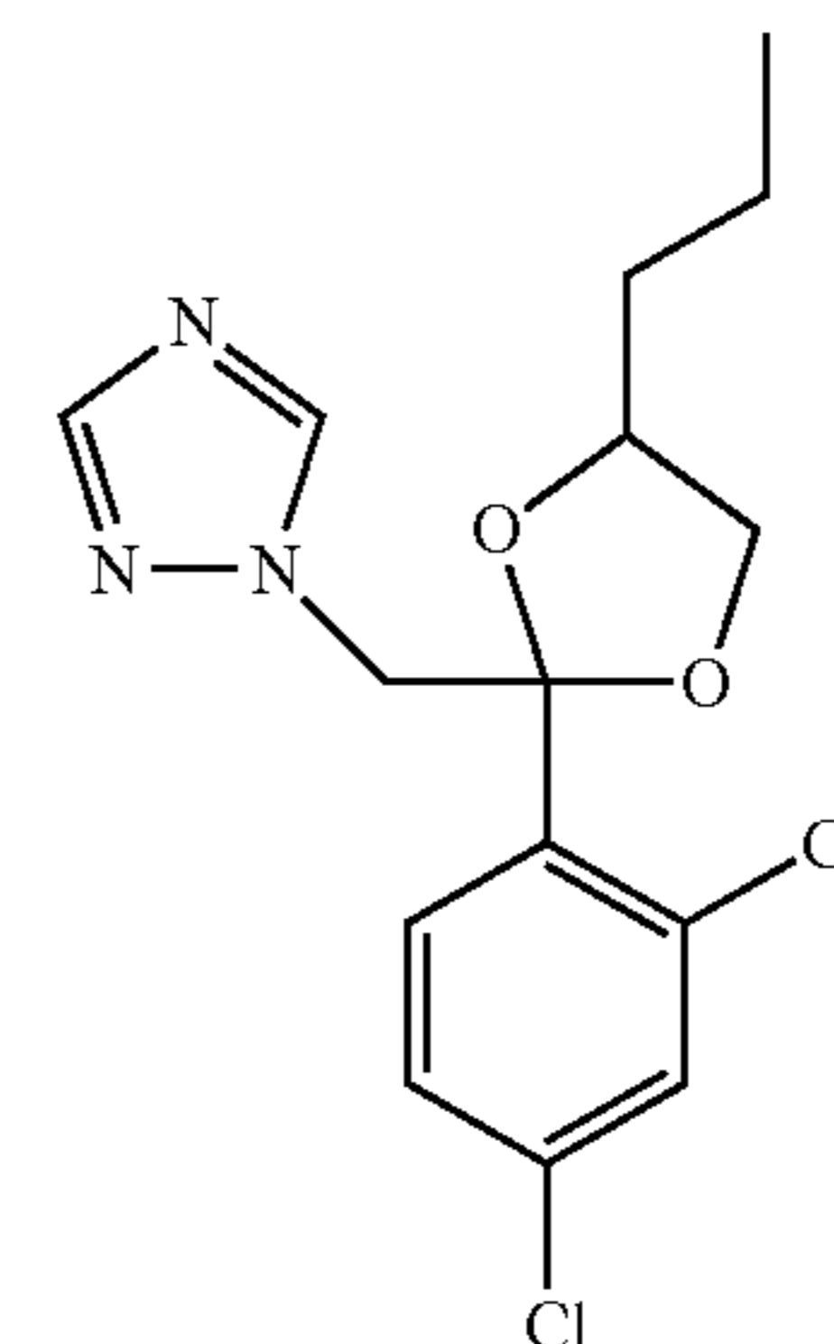
Chemical structure of Propiconazole
