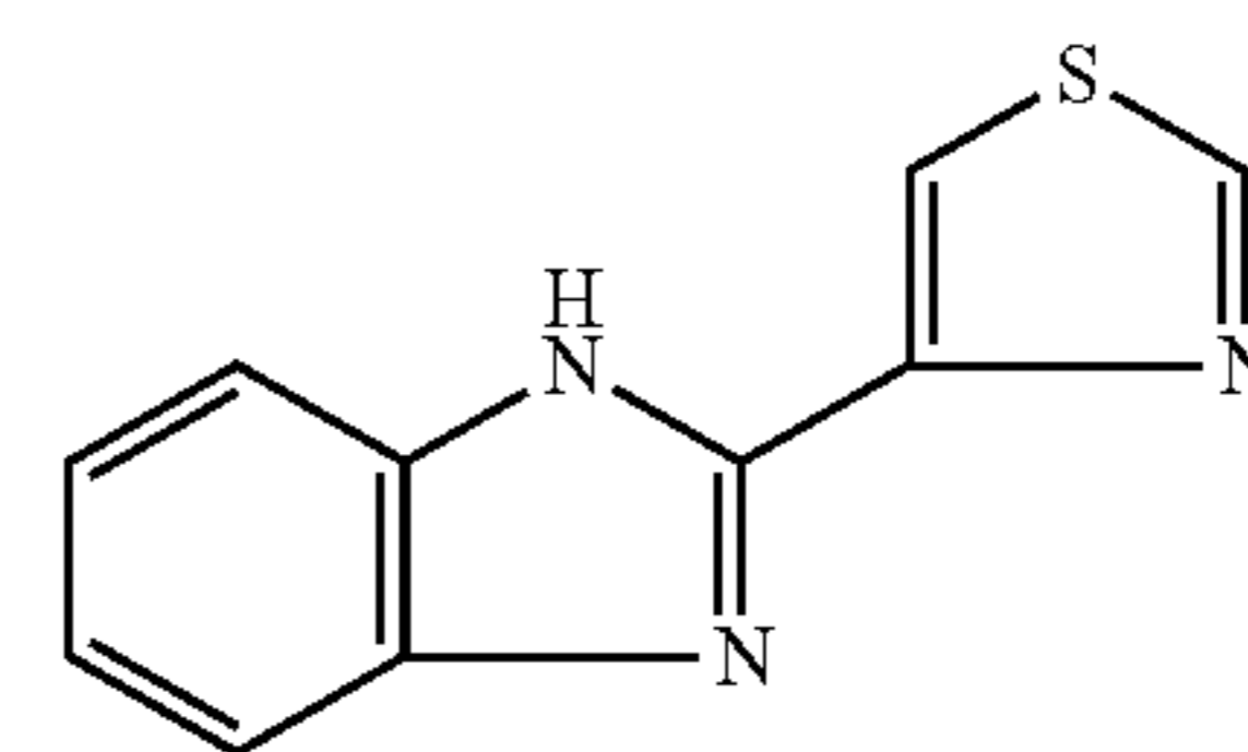
Chemical structure of Thiabendazole
