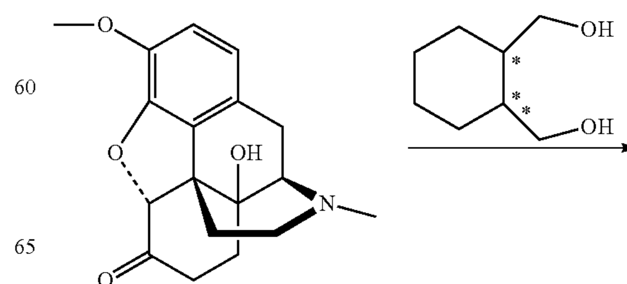
Scheme 3
