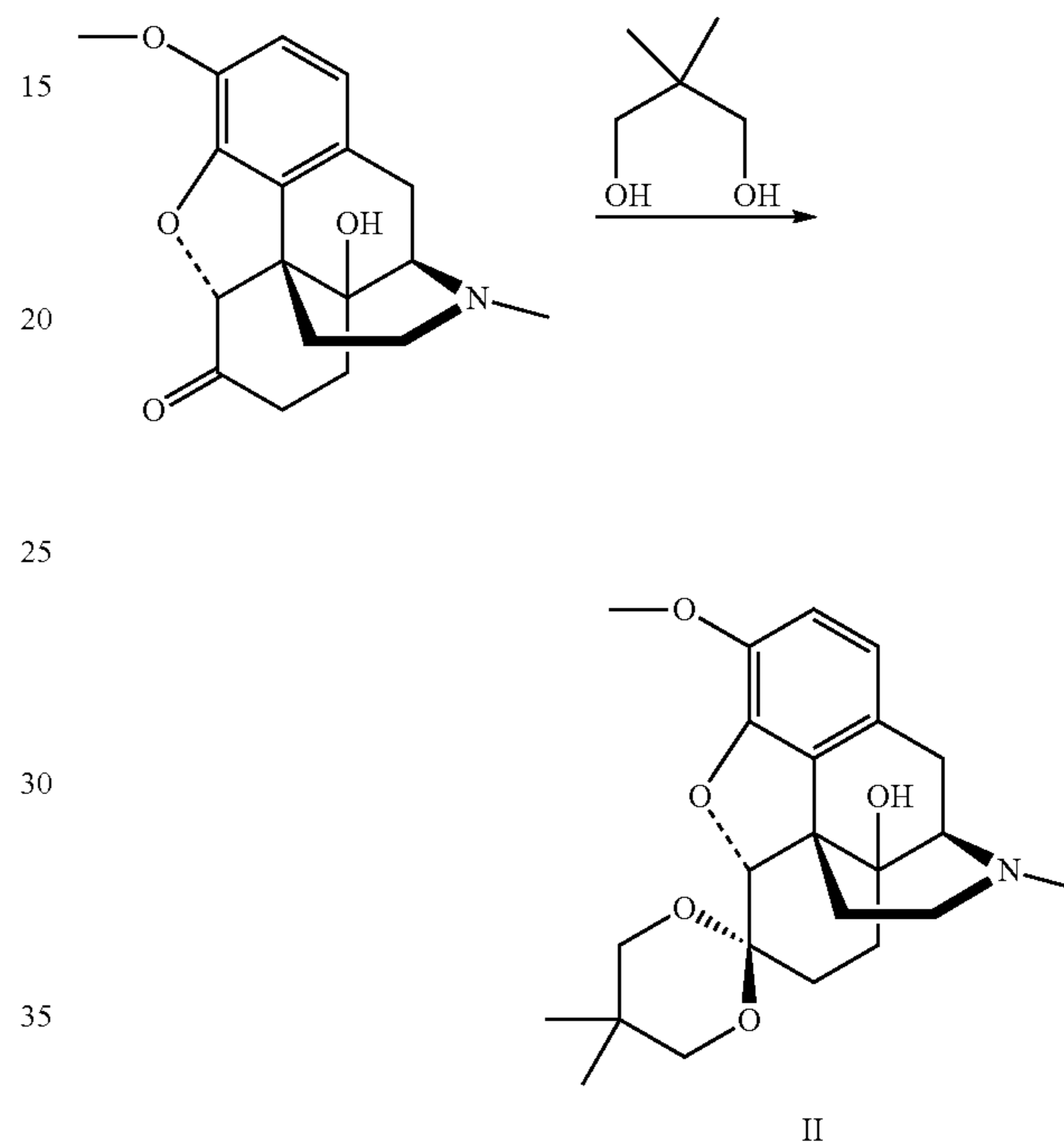
Scheme 2
