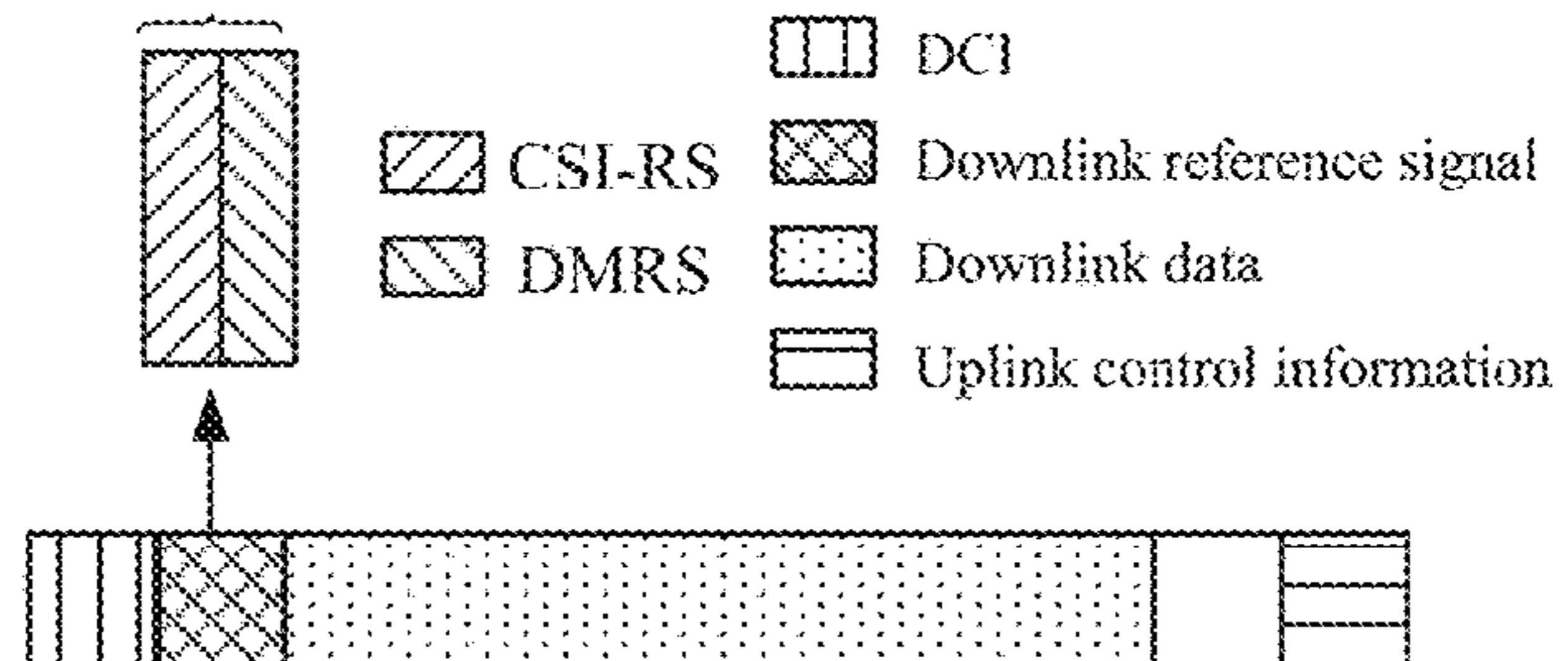
An OFDM symbol
