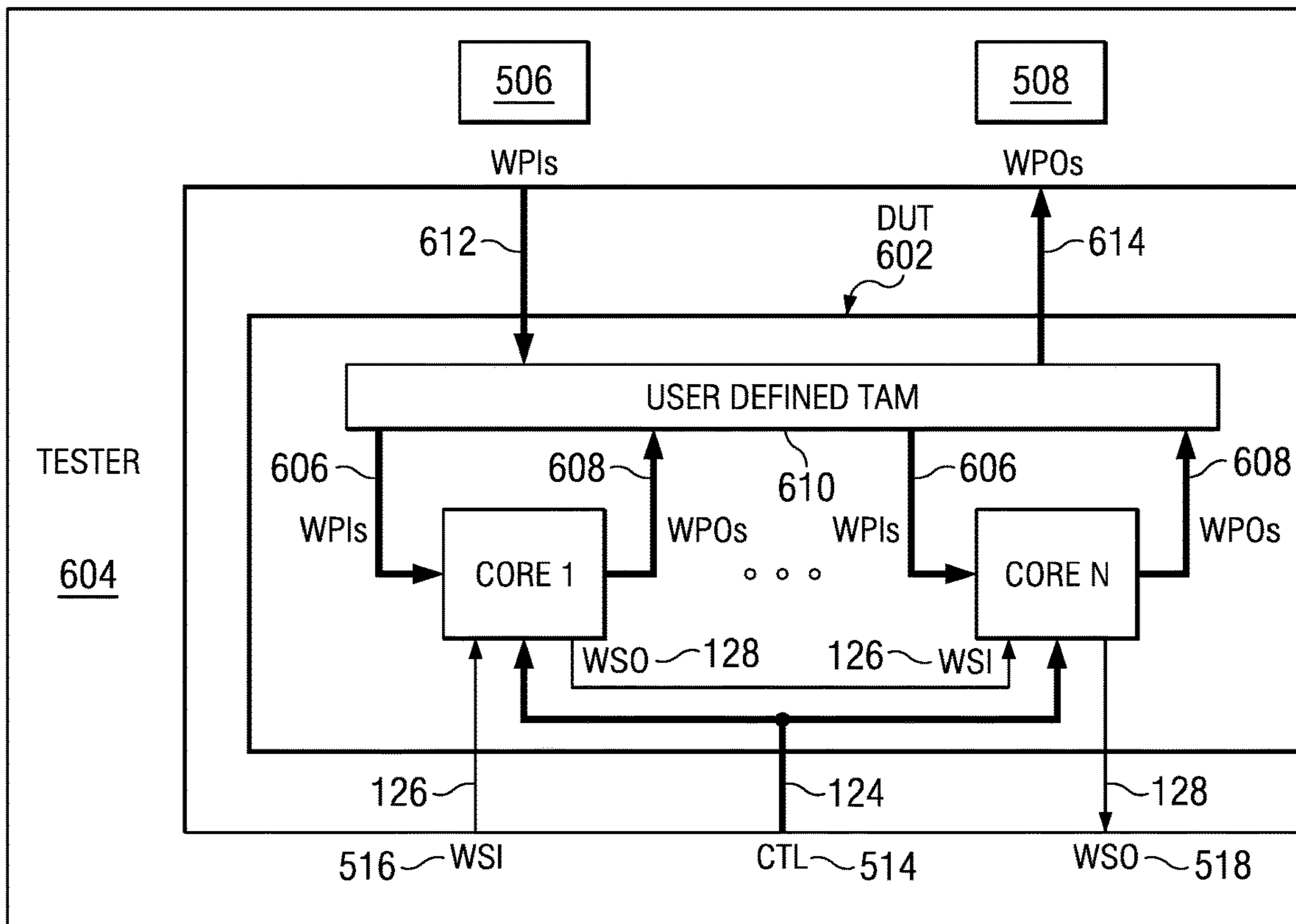
FIG. 6 (PRIOR ART)
