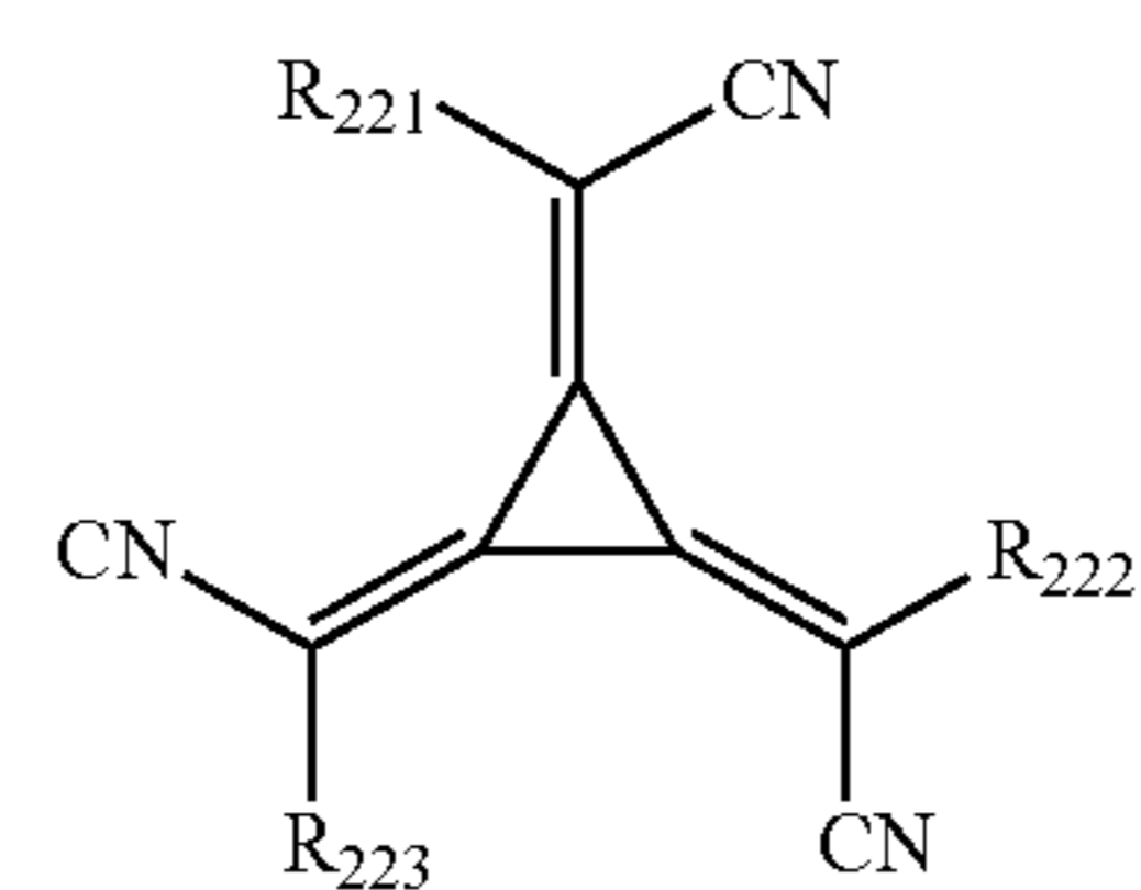
F4-TCNQ
