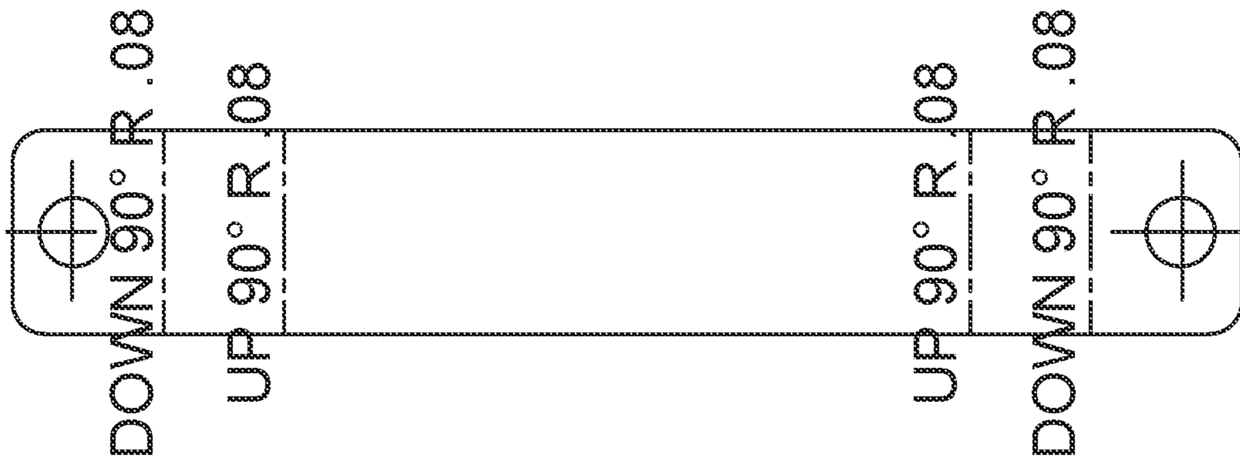
FLAT PATTERN
