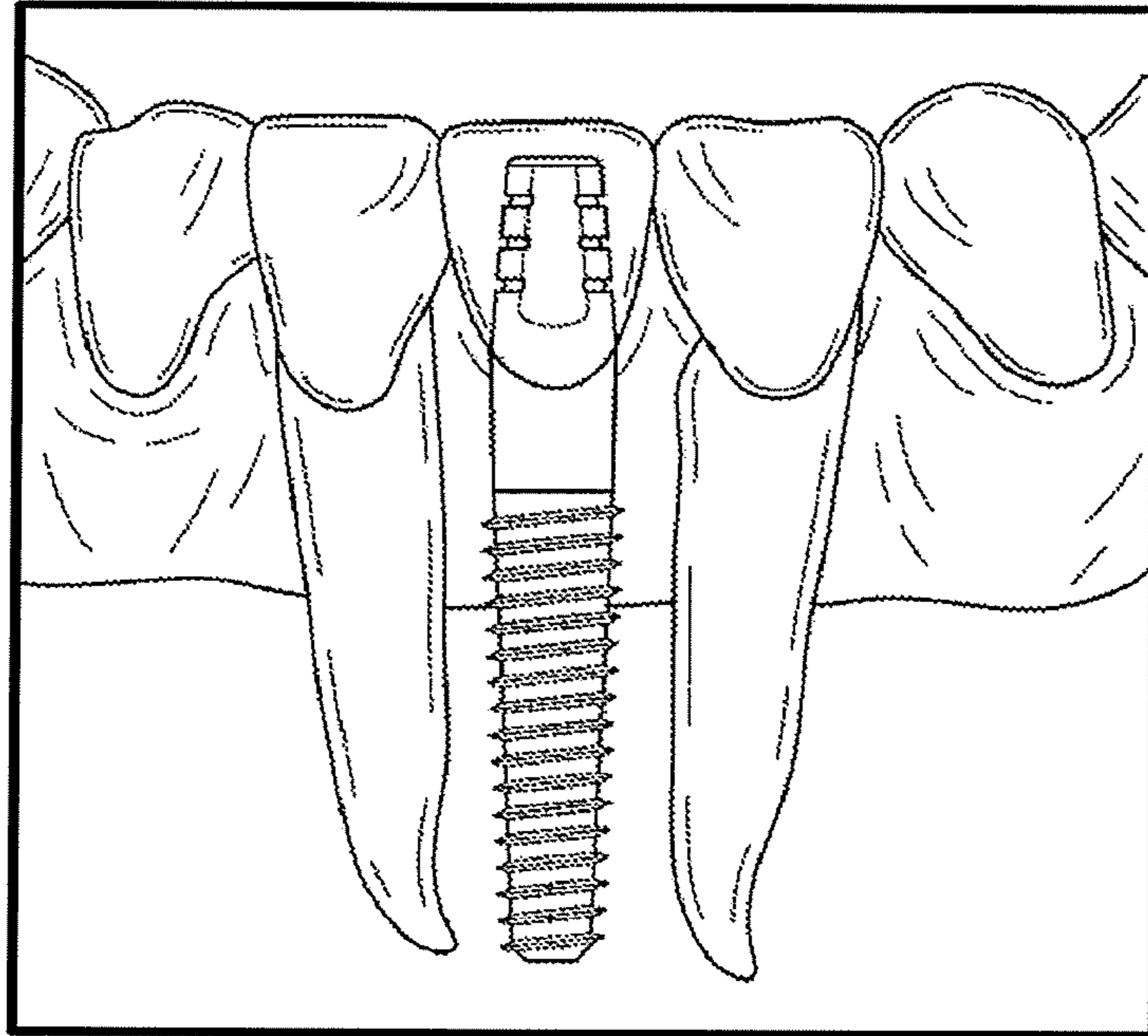
FIG. 1 (Prior Art)
