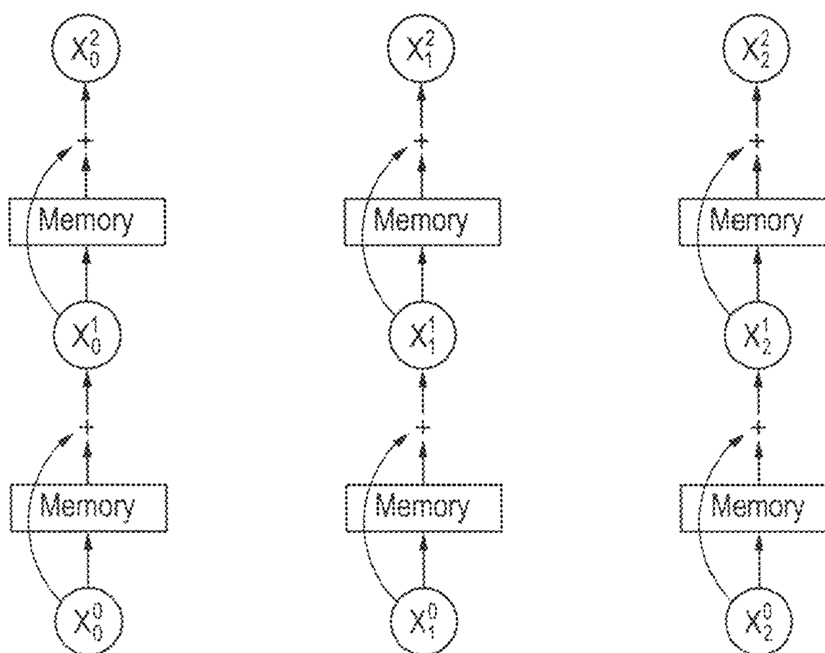
Neural Network
