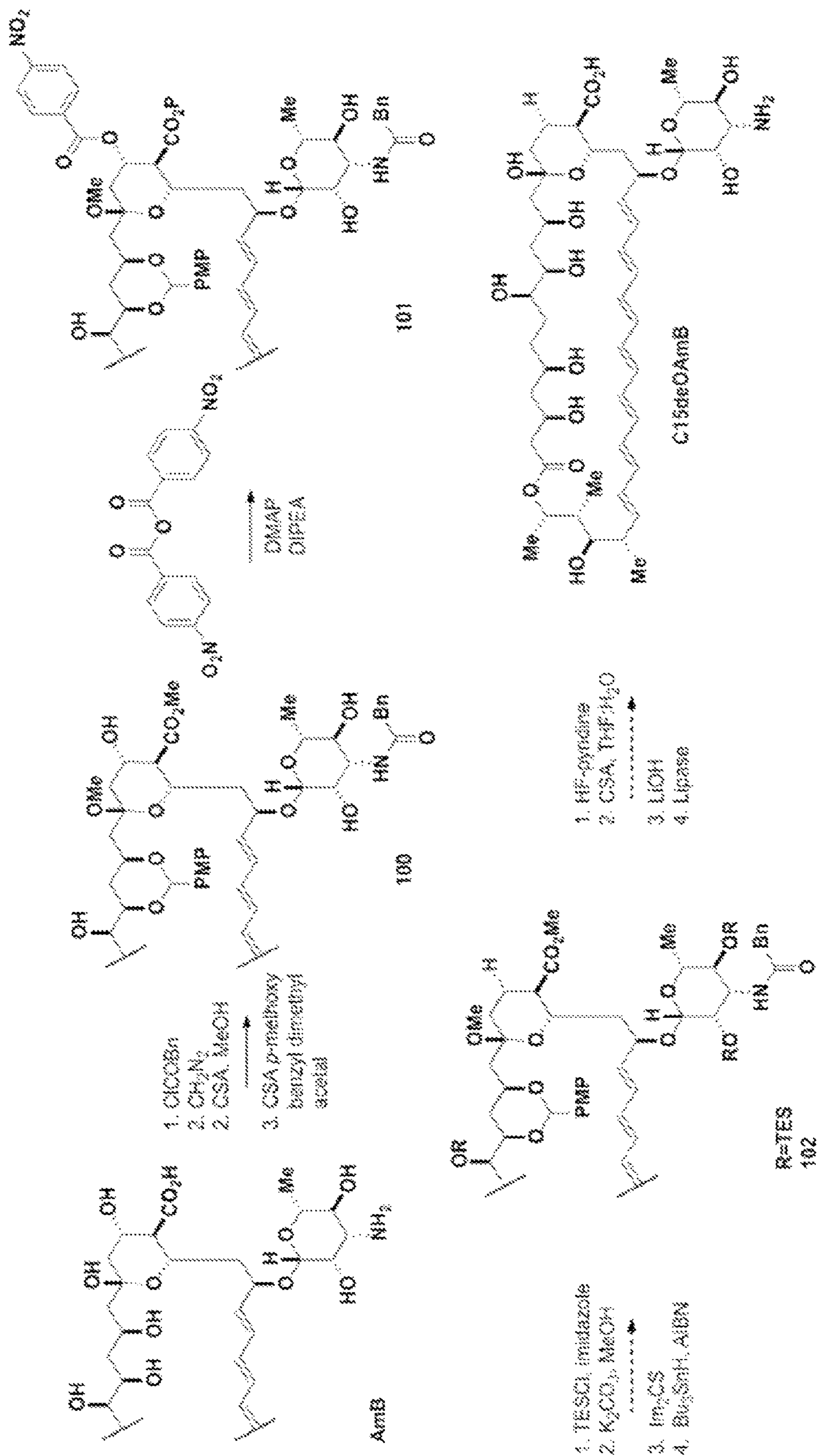
Scheme 25
