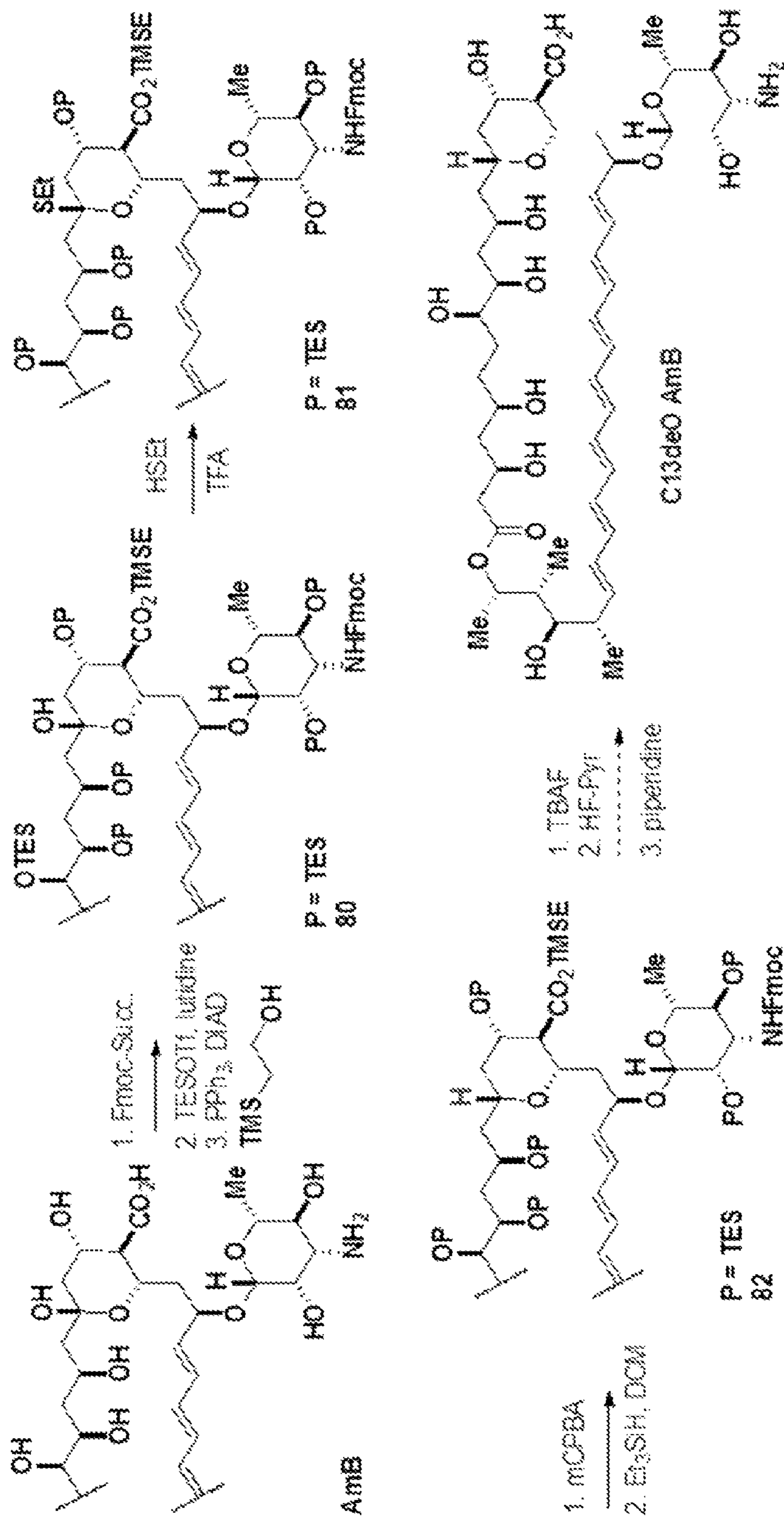
Scheme 21
