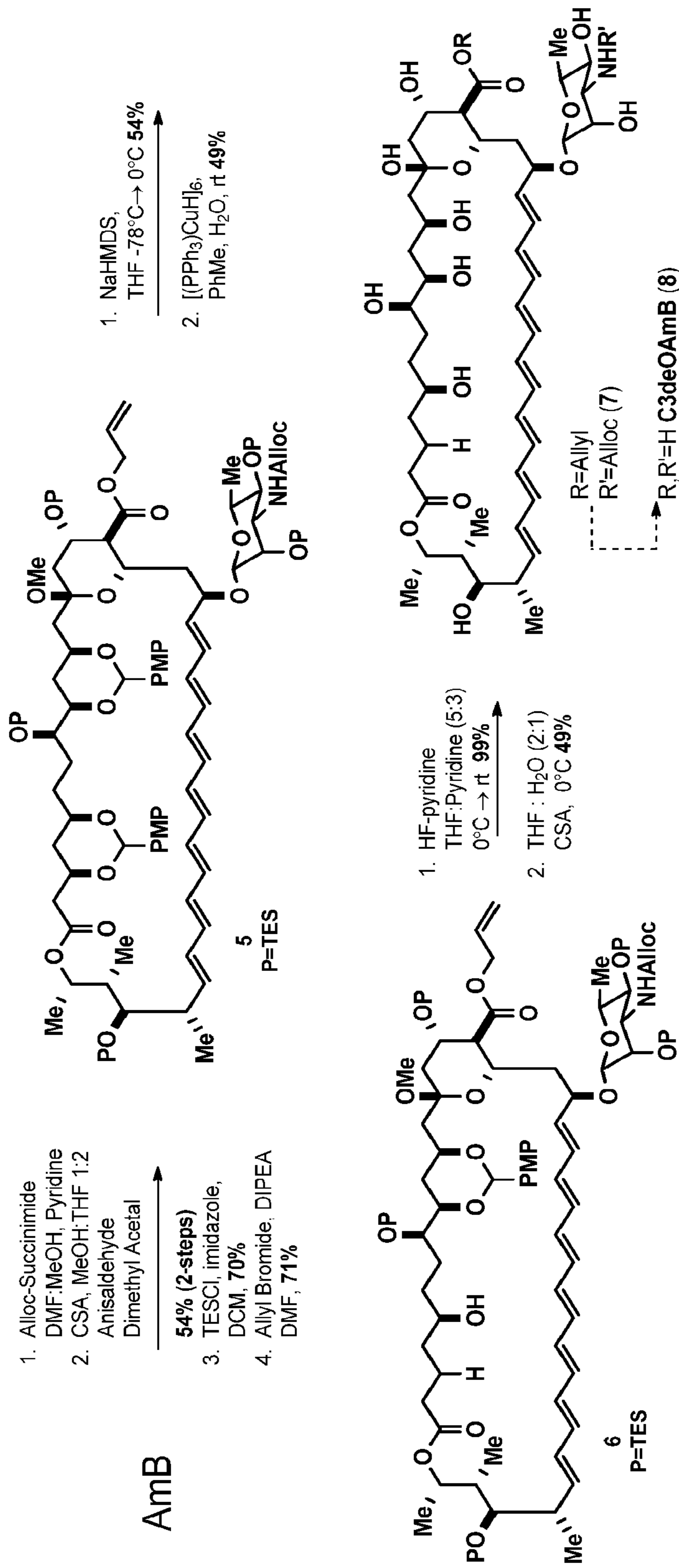
Scheme 3
