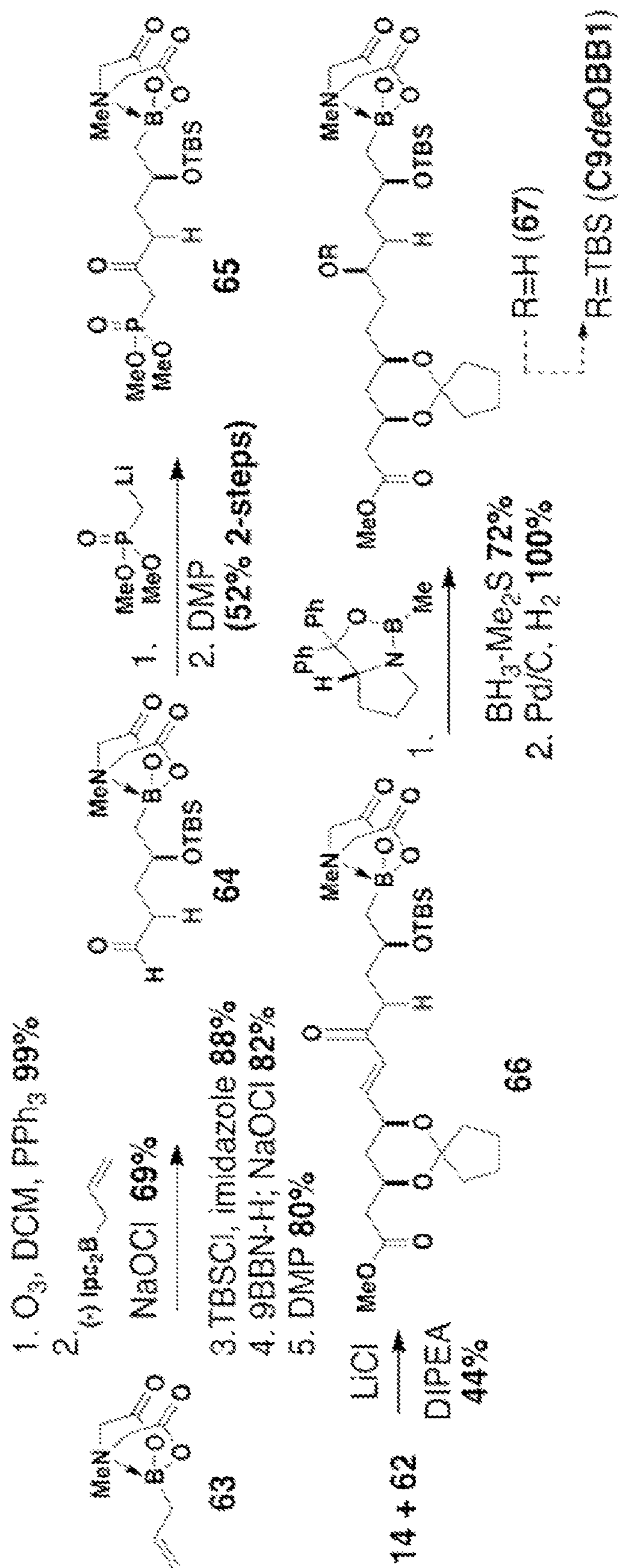
Scheme 17
