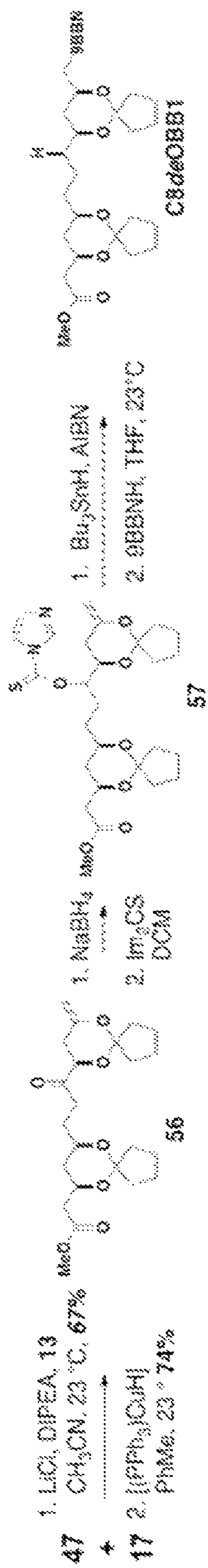
Scheme 15
