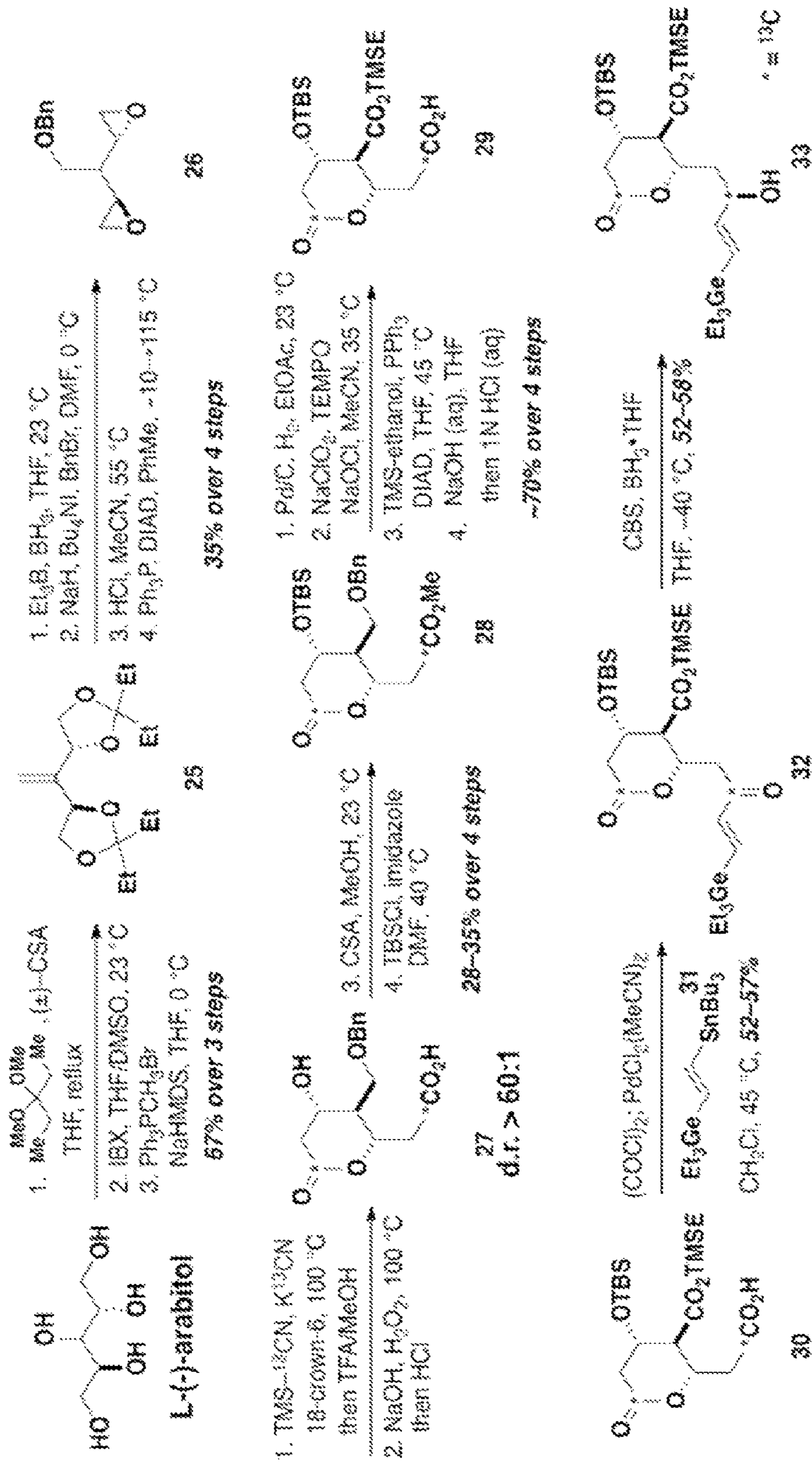
Scheme 9
