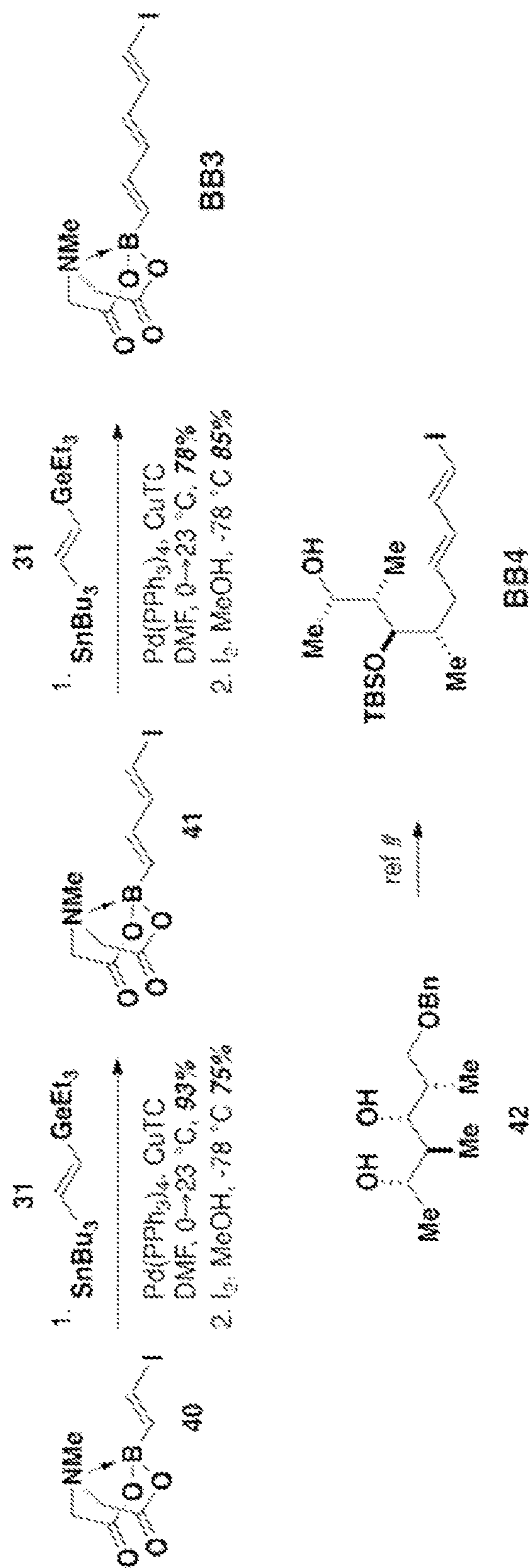
Scheme 11
