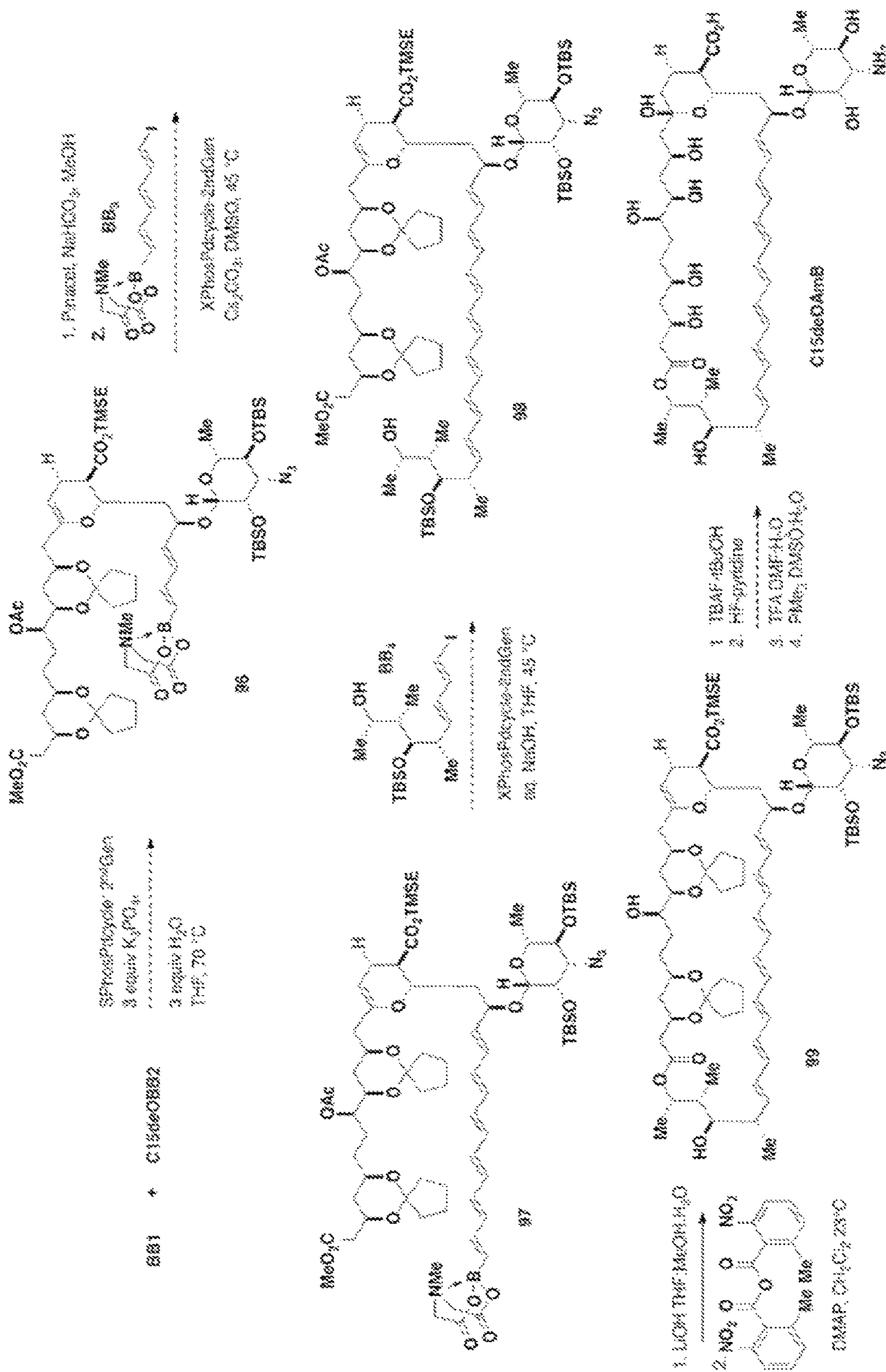
Scheme 24
