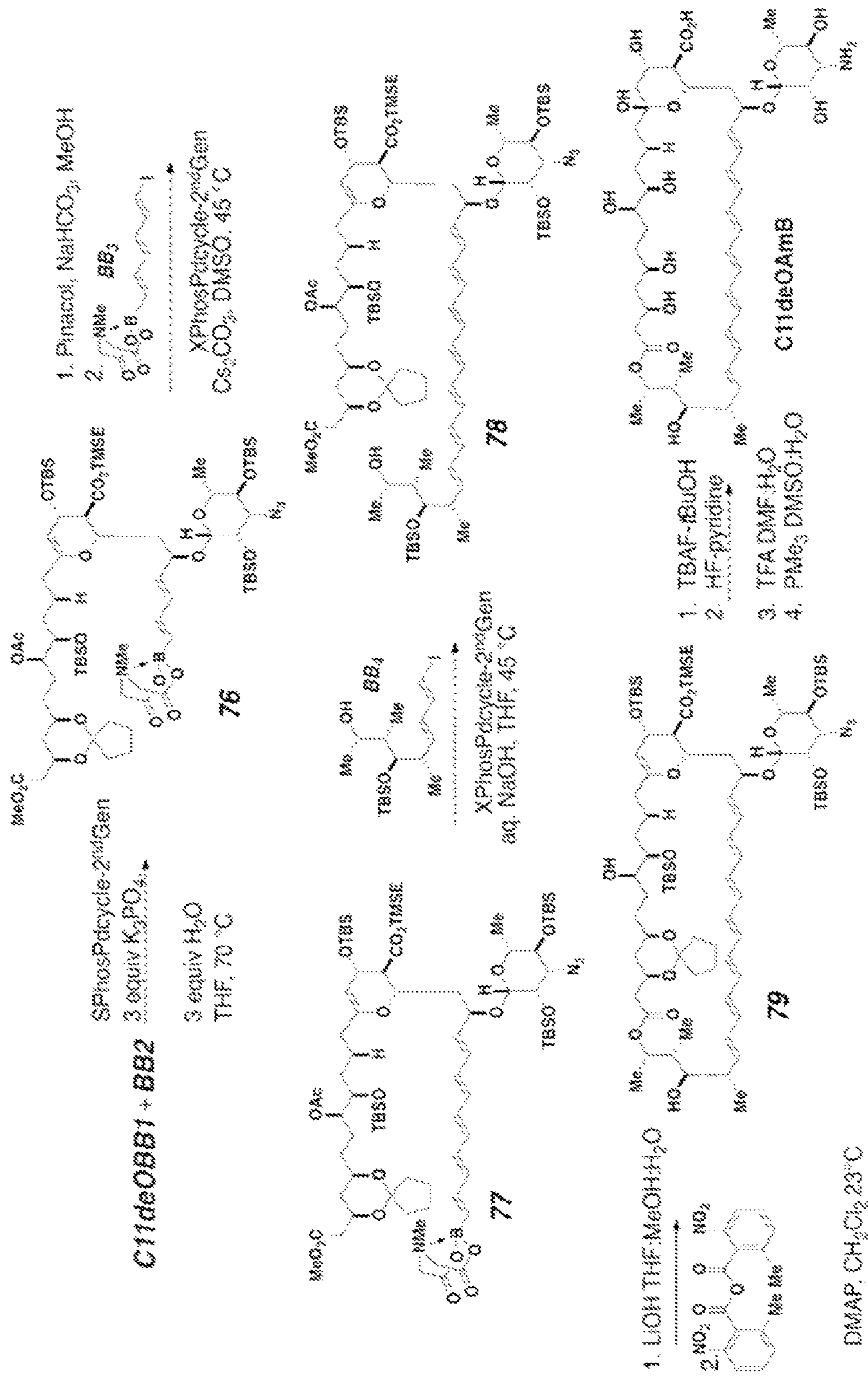
Scheme 20
