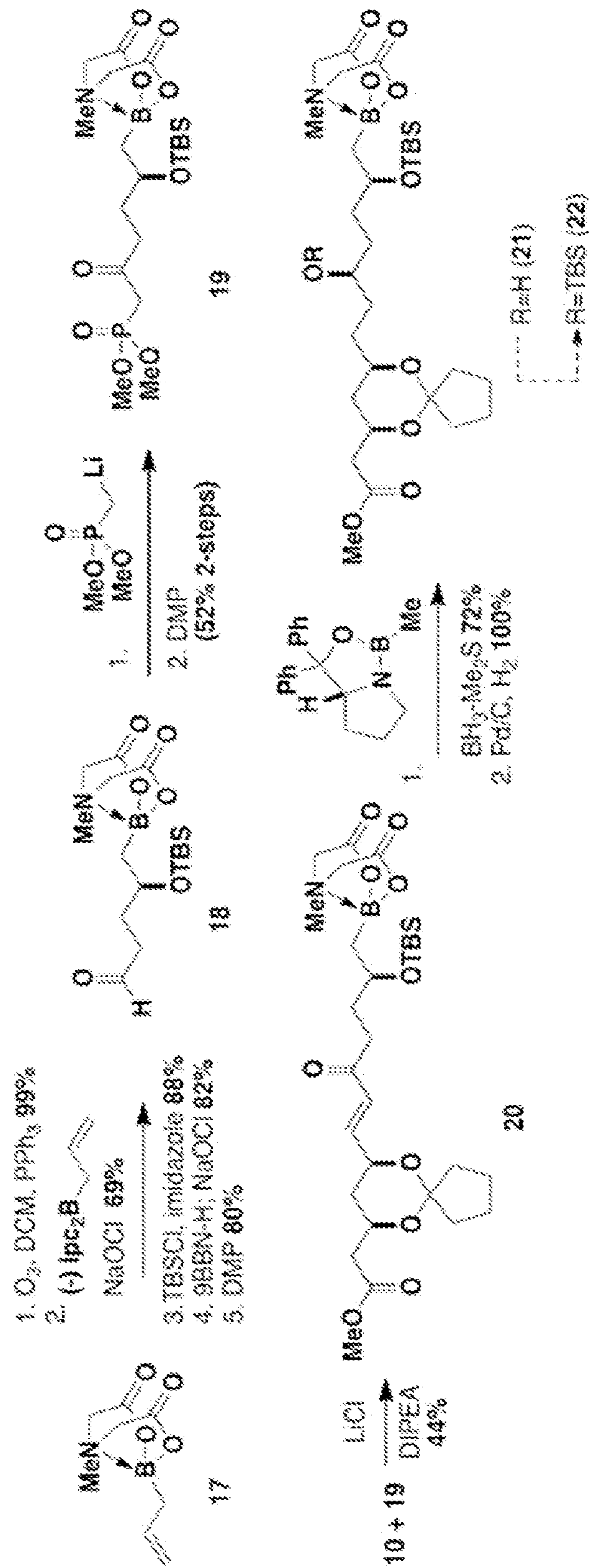
Scheme 5
