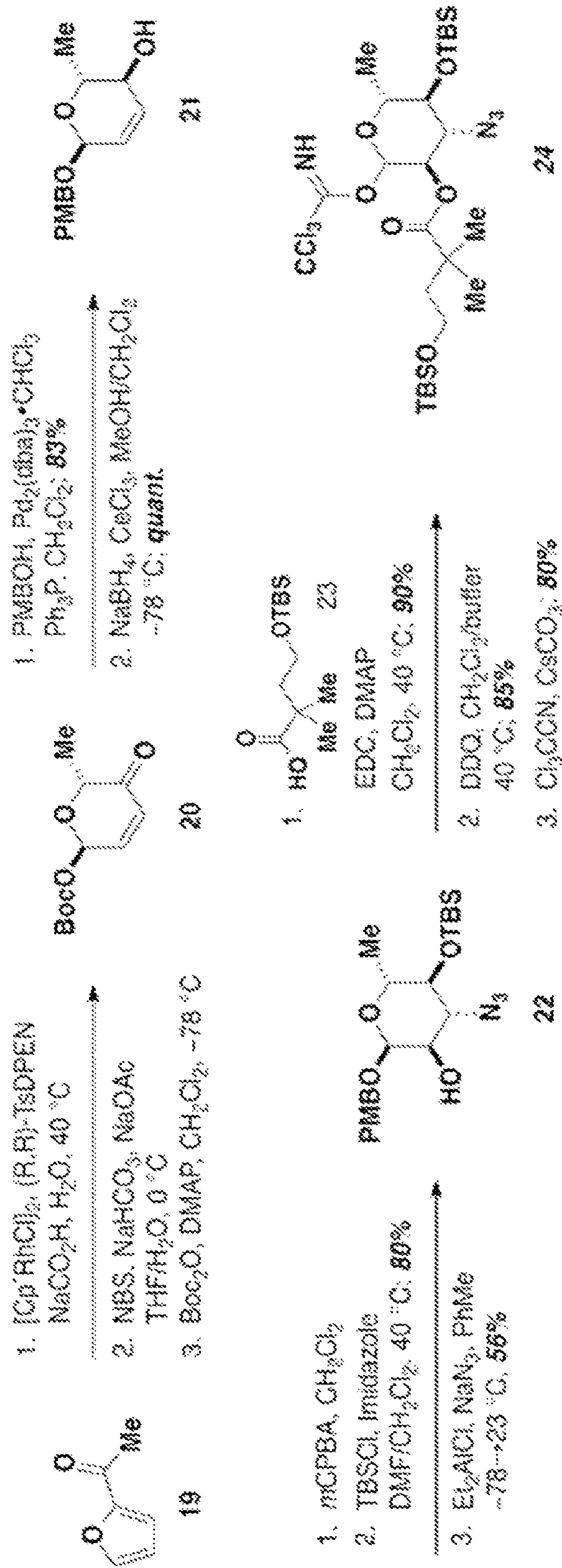
Scheme 8
