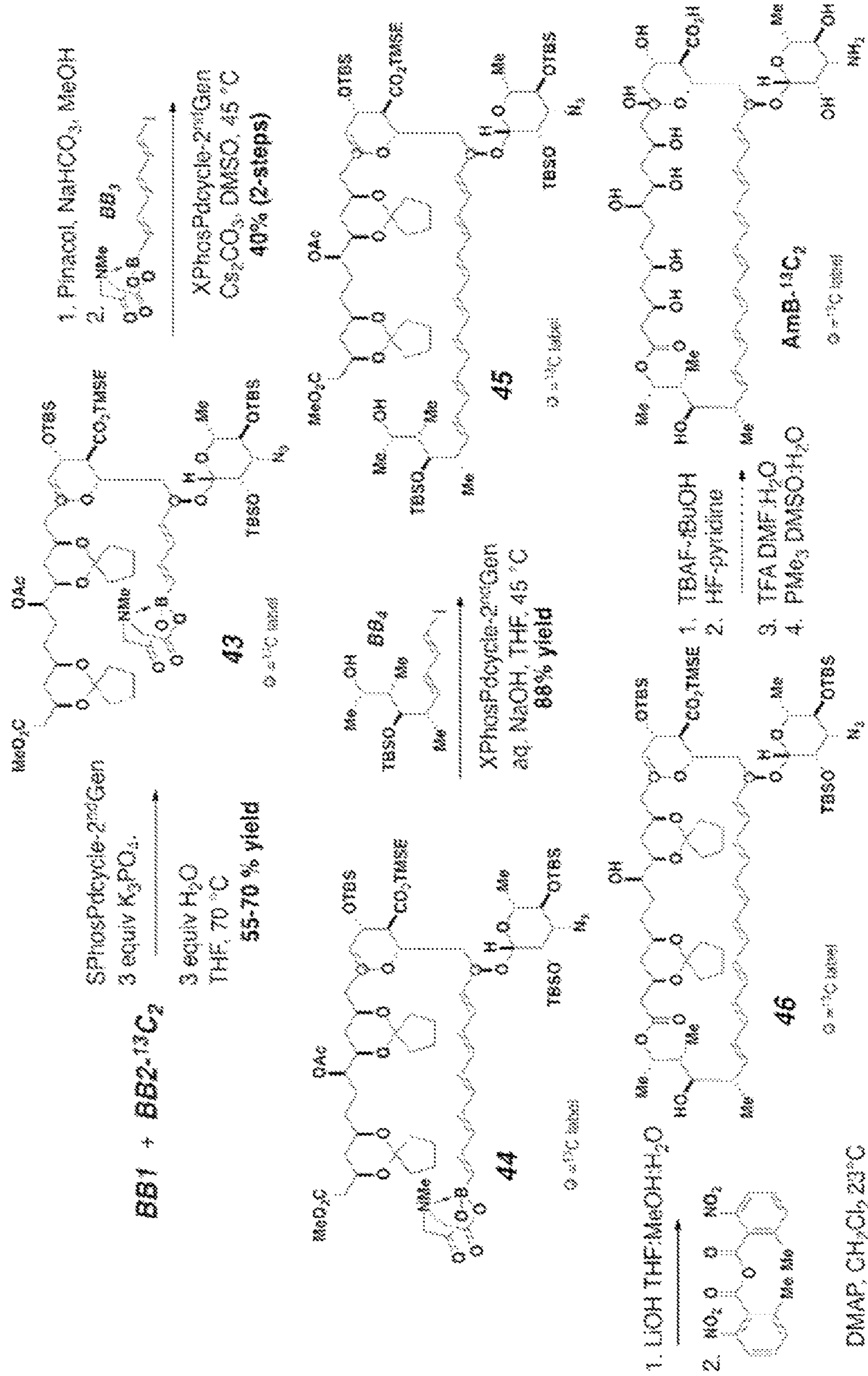
Scheme 12
