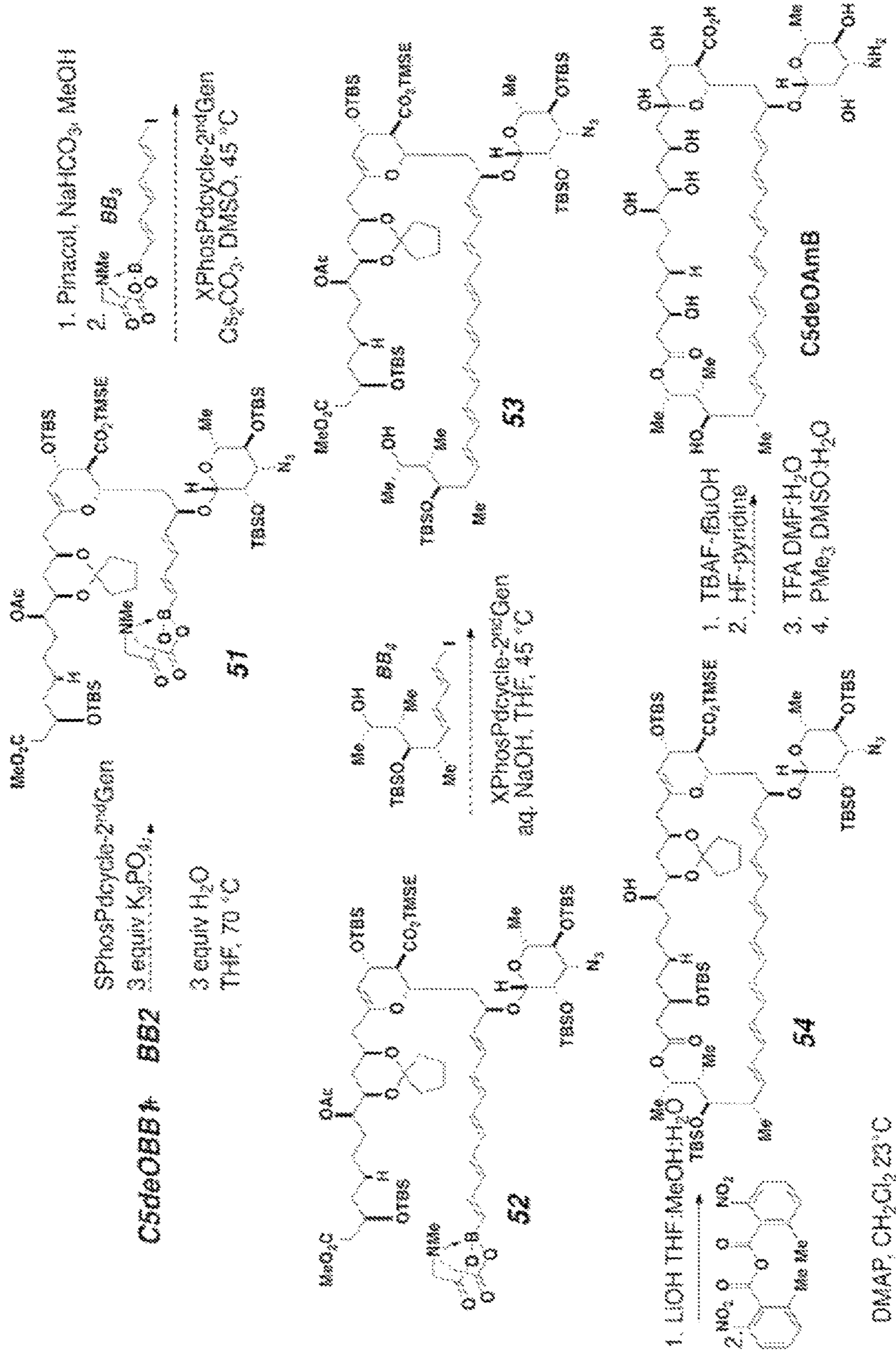
Scheme 14
