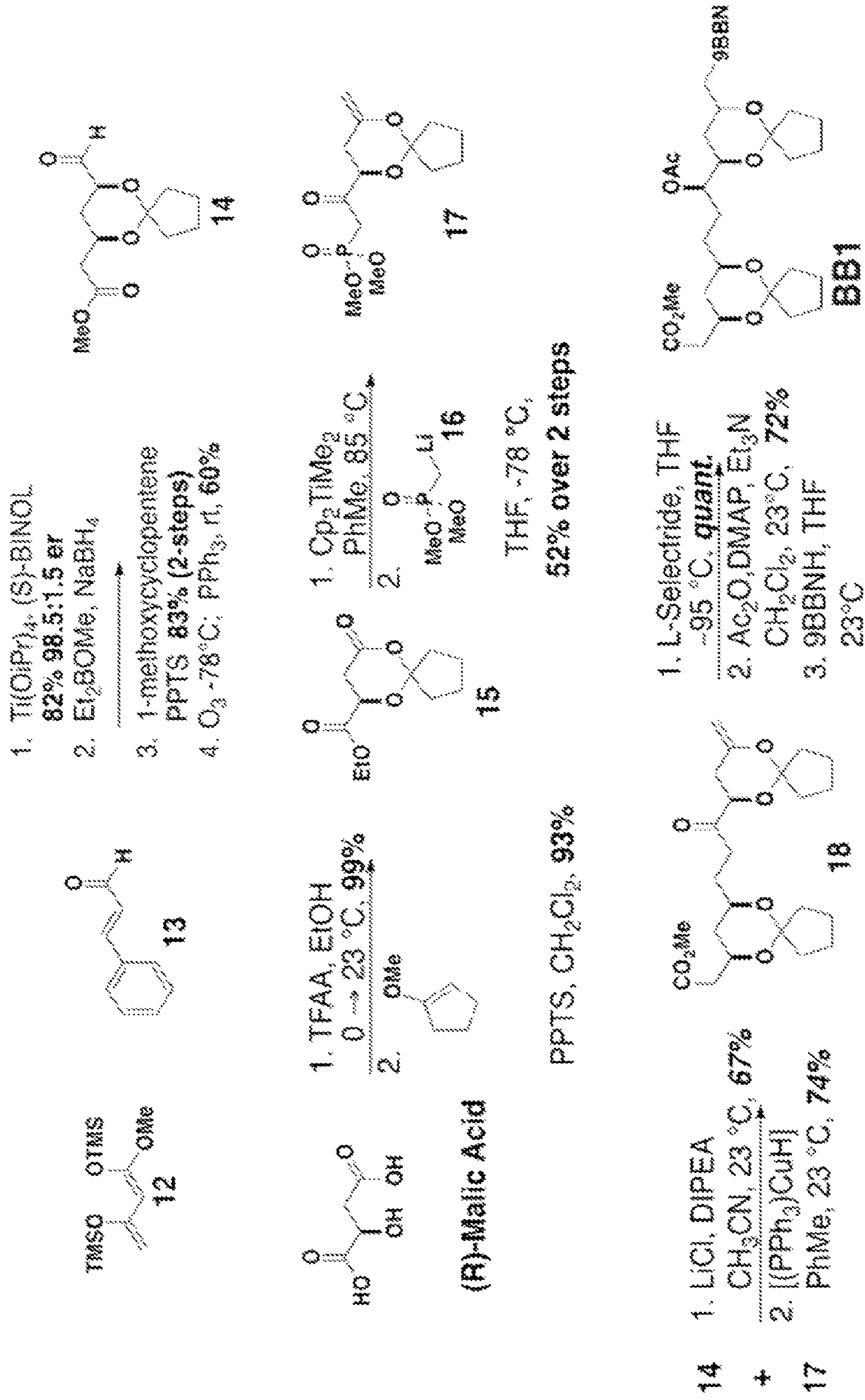
Scheme 7
