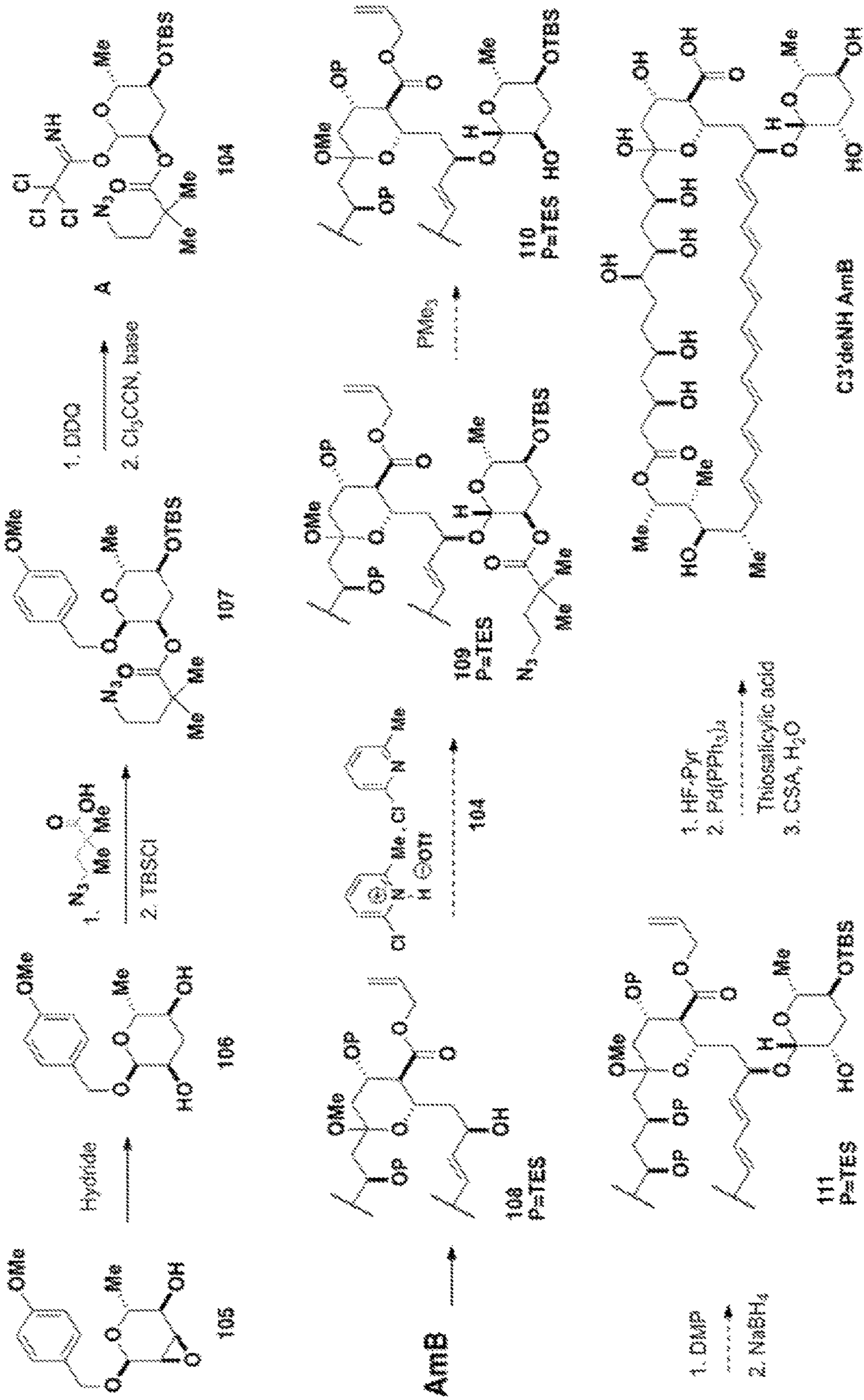
Scheme 26
