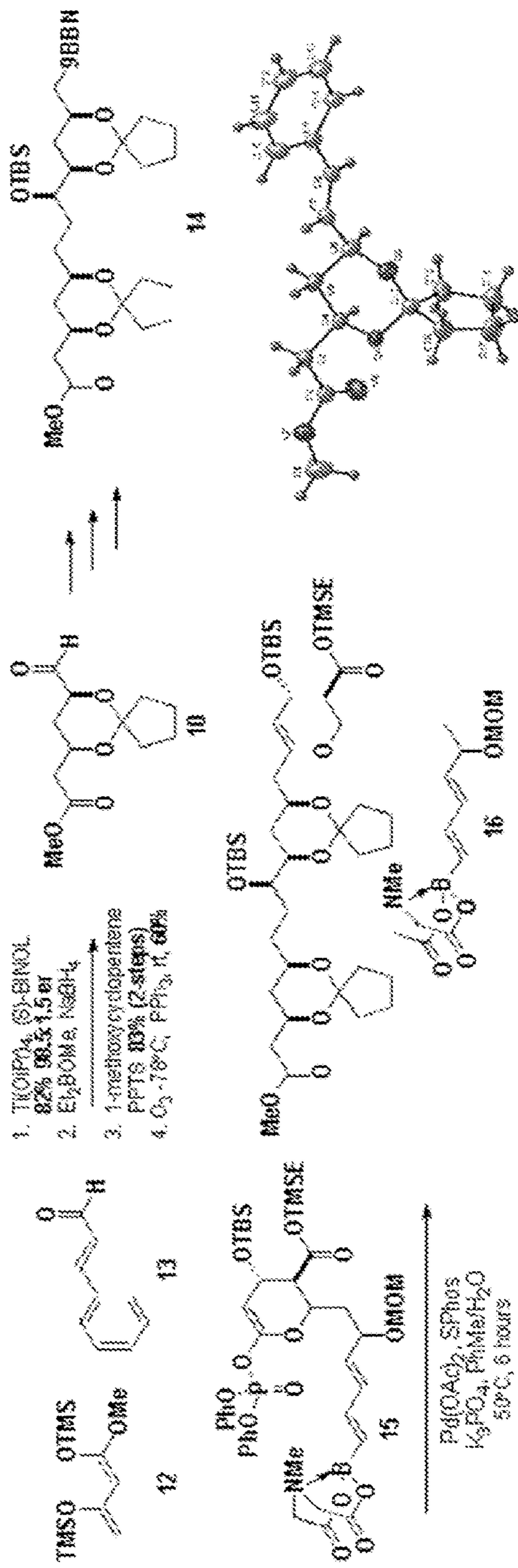
Scheme 4
