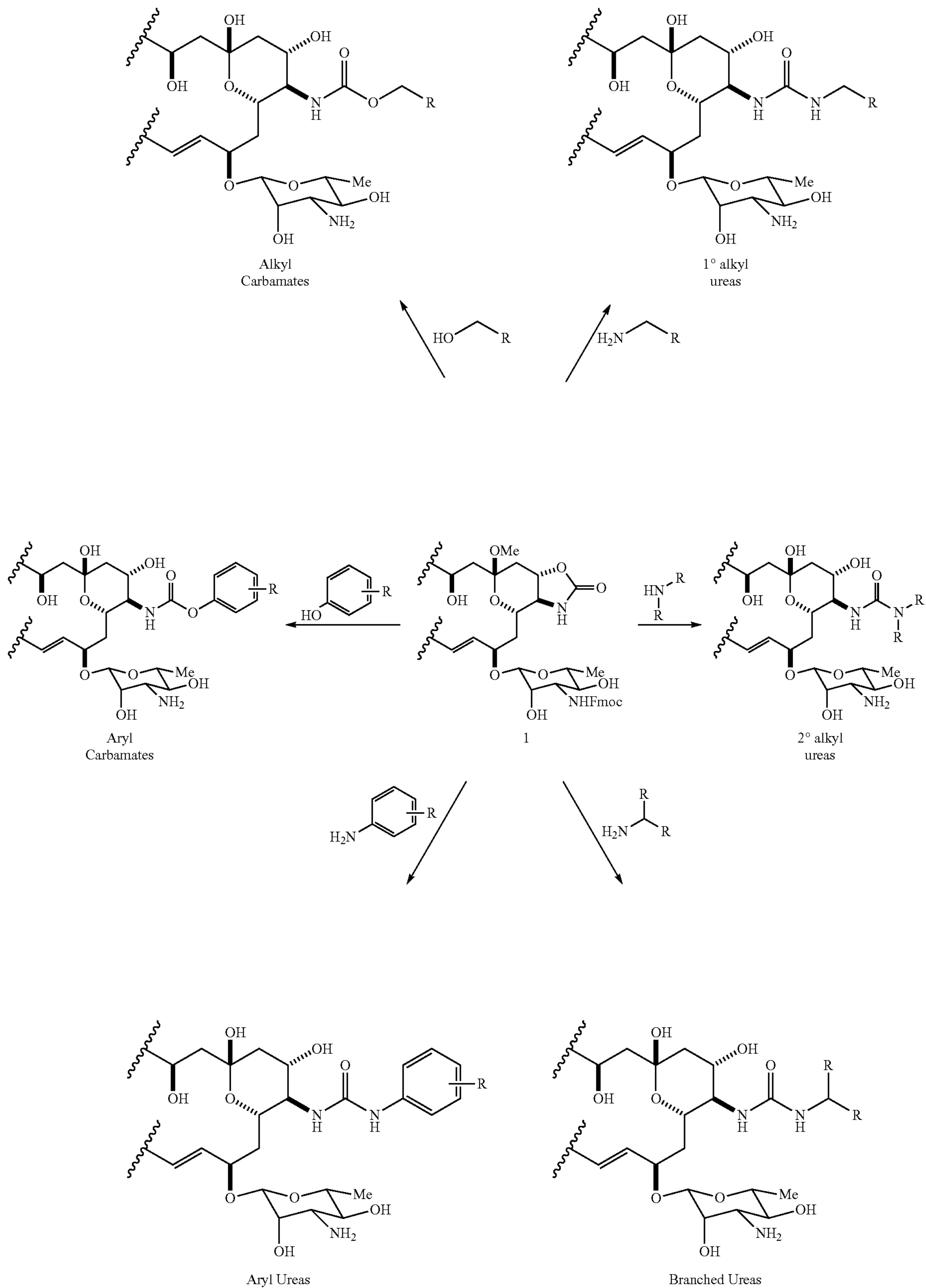
Scheme 2
