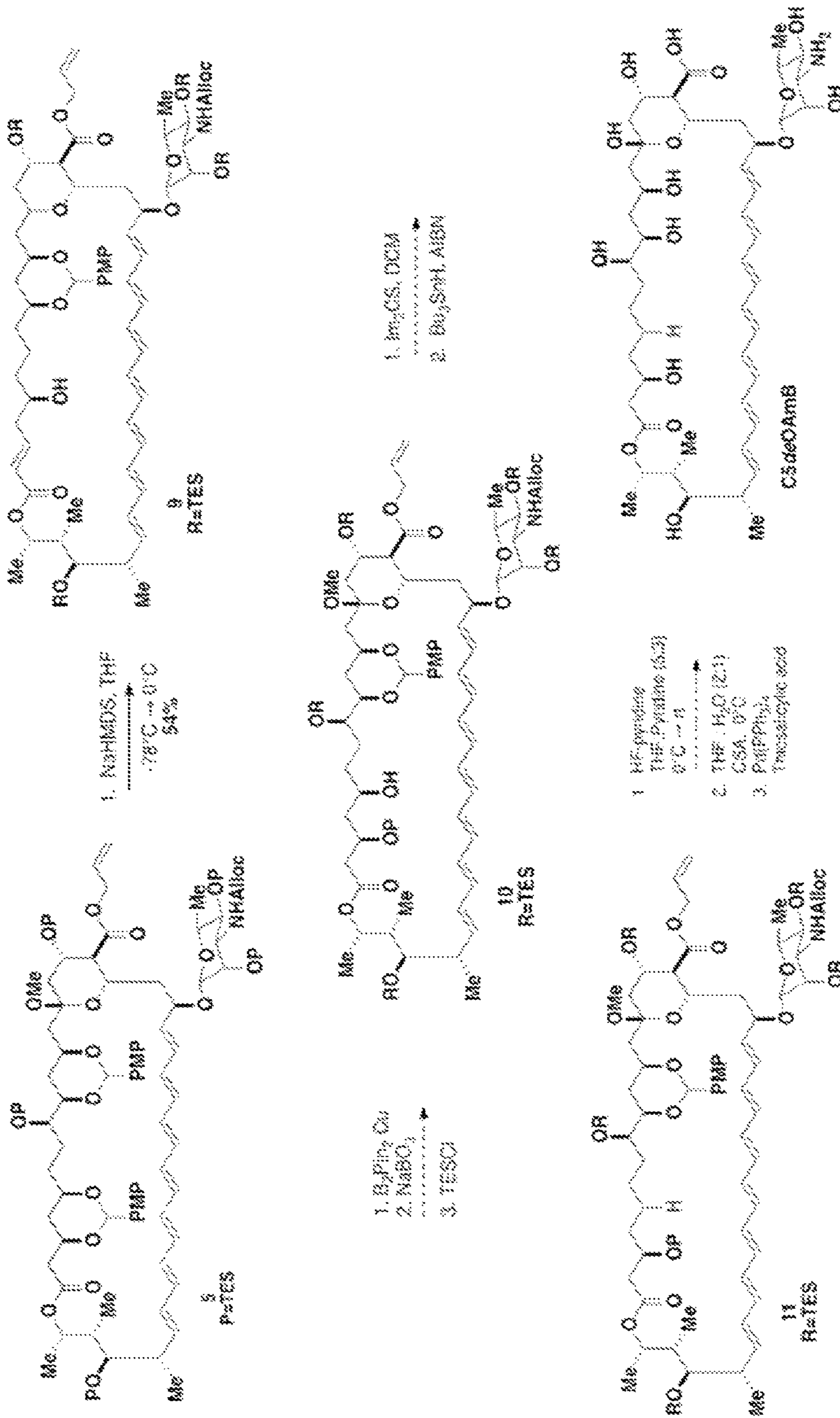
Scheme 6
