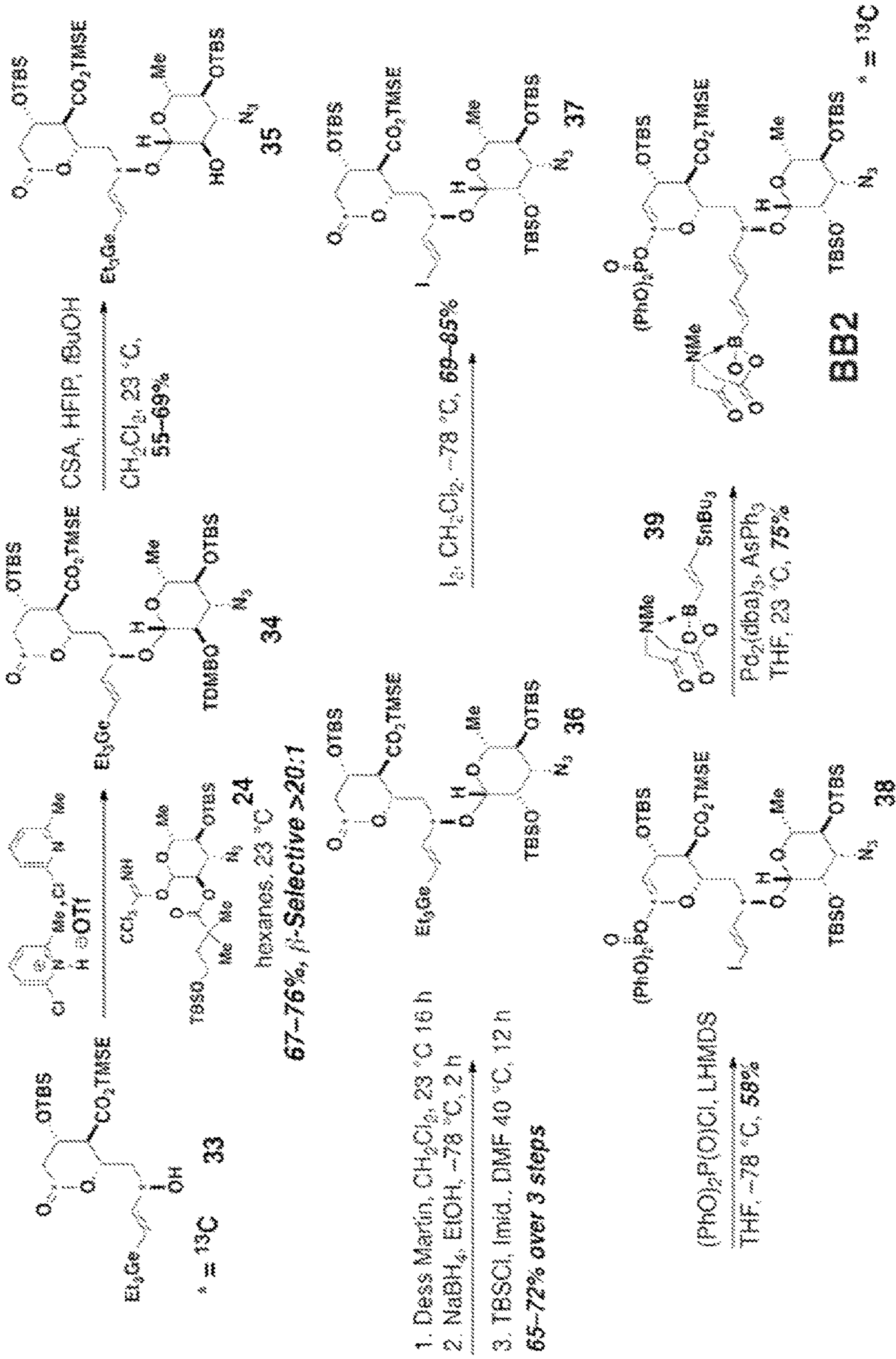
Scheme 10
