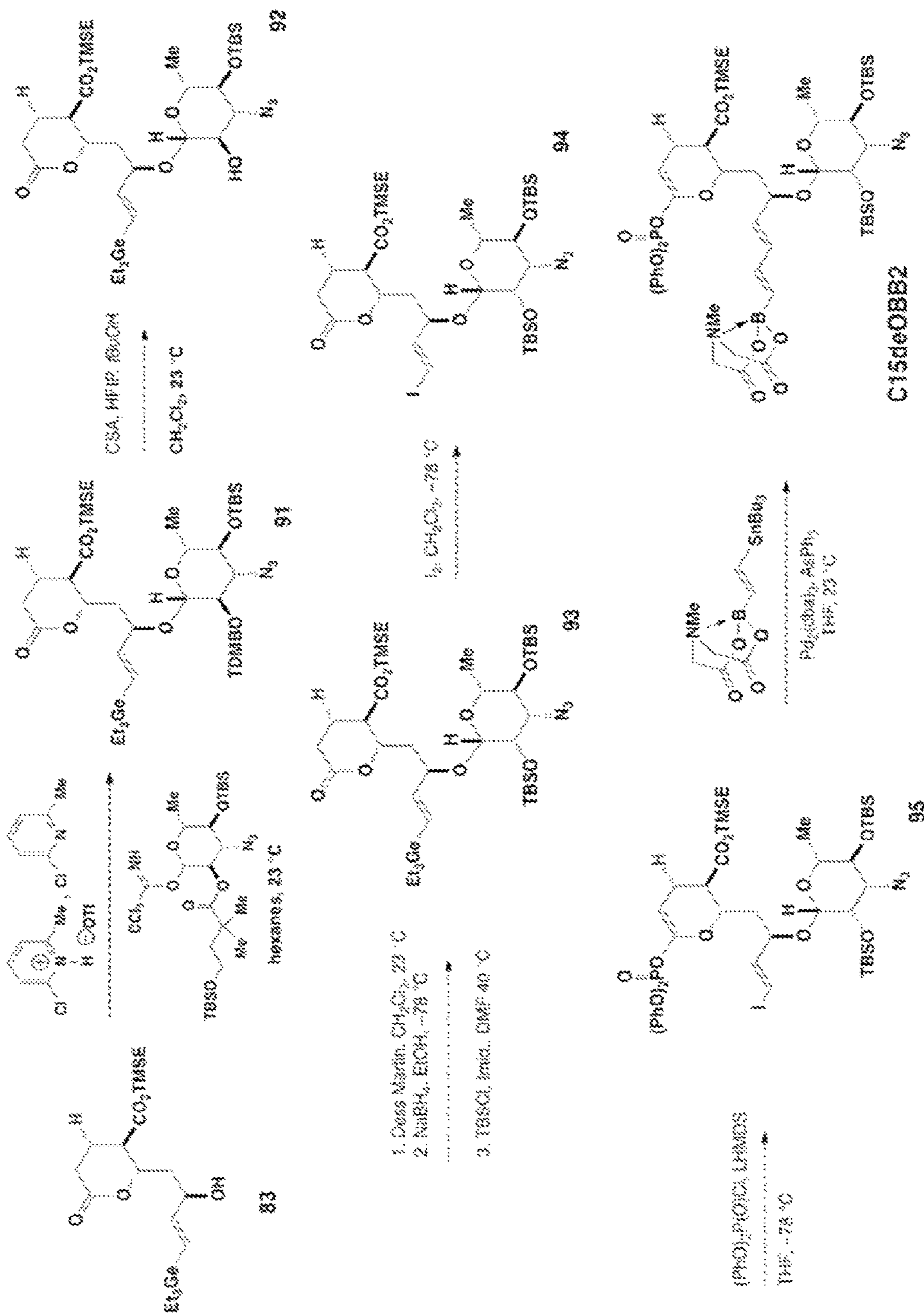
Scheme 23
