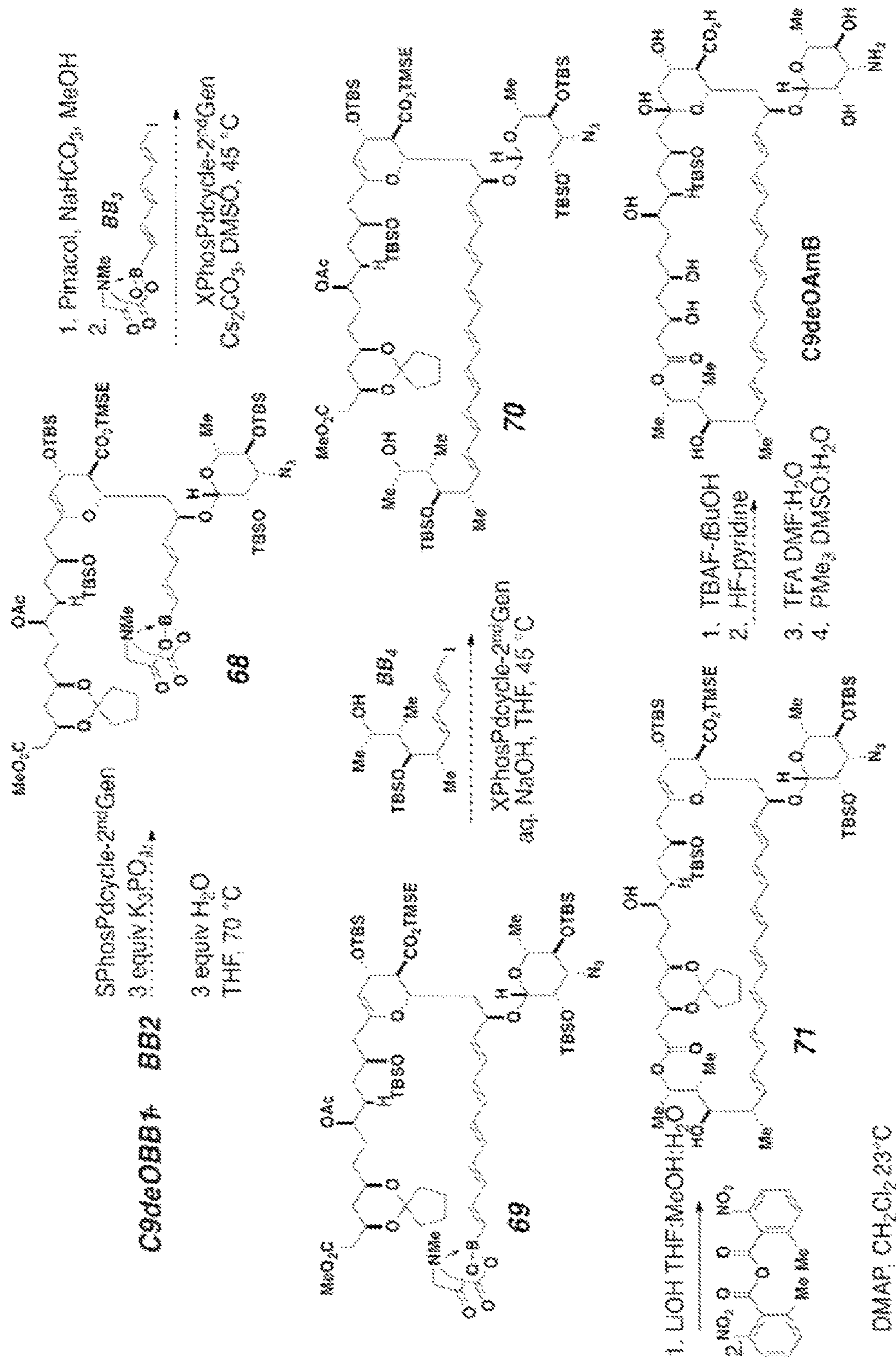
Scheme 18
