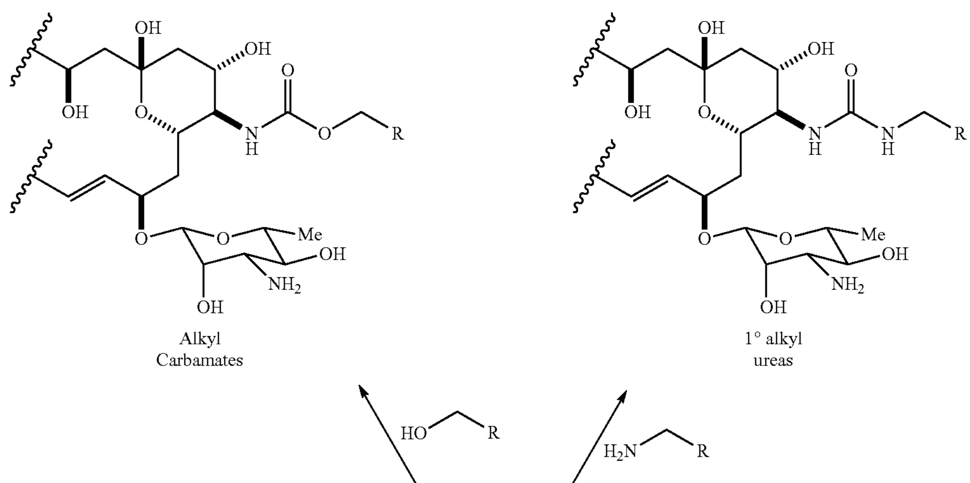
Scheme 2
