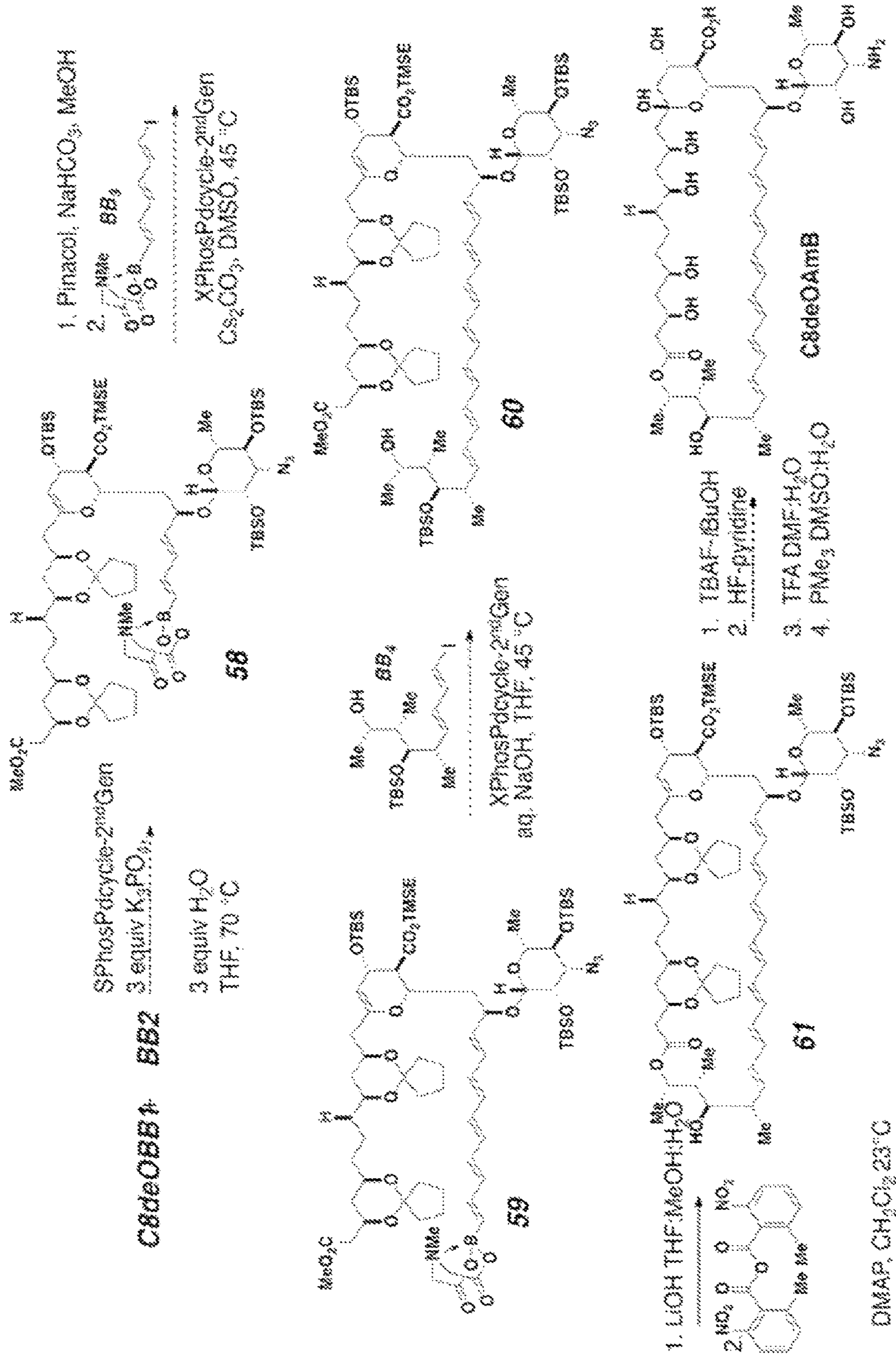
Scheme 16
