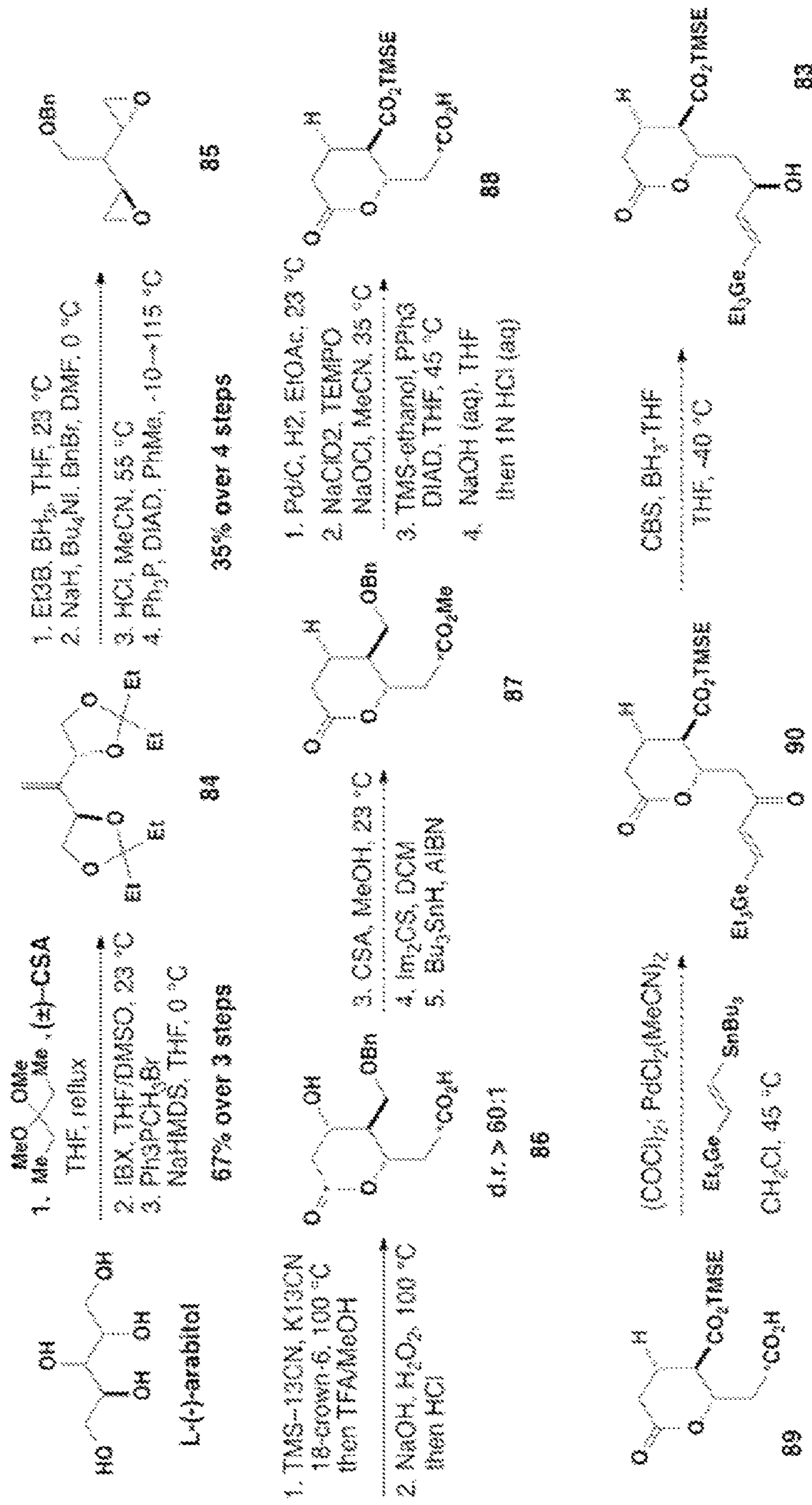
Scheme 22
