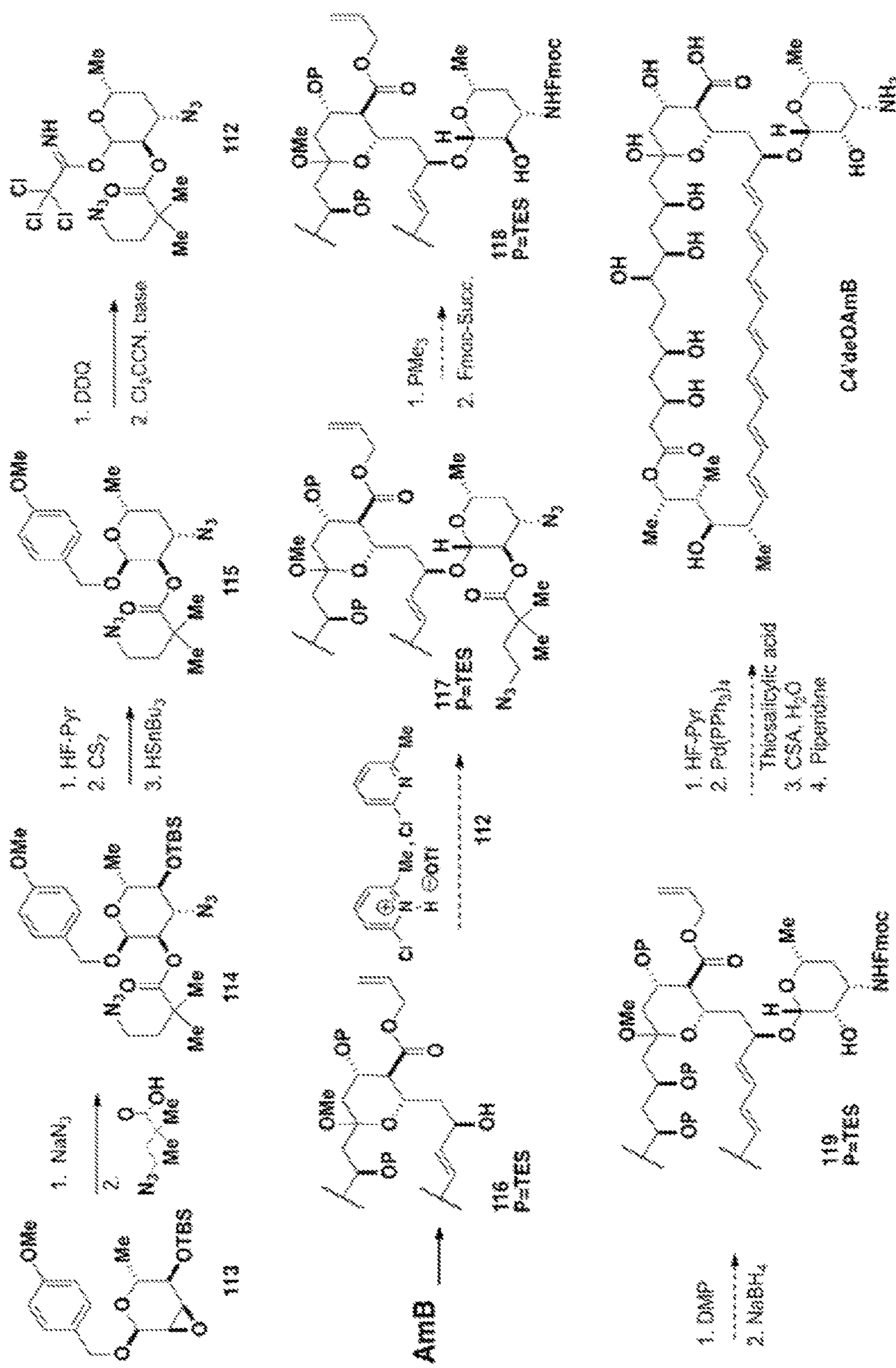
Scheme 27
