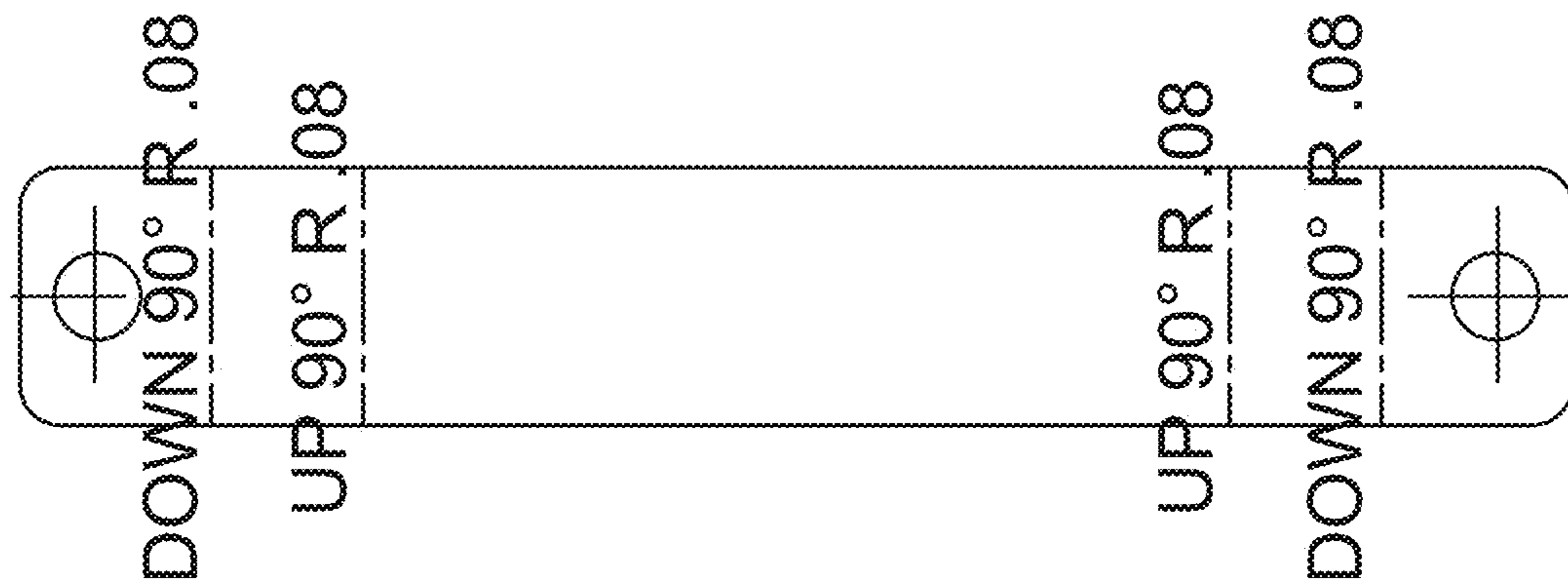
FLAT PATTERN
