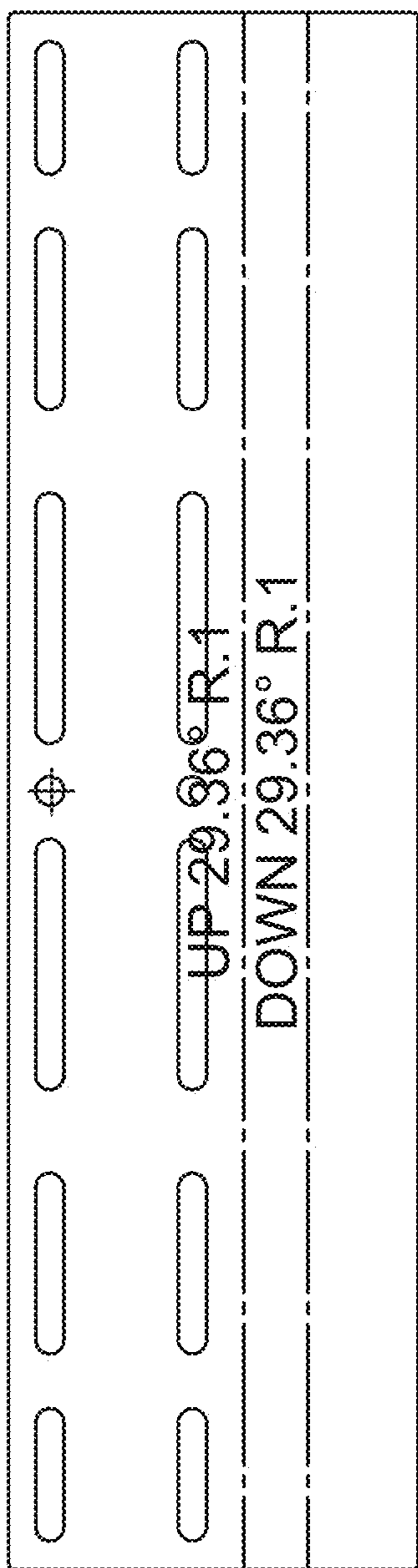
FLAT PATTERN
