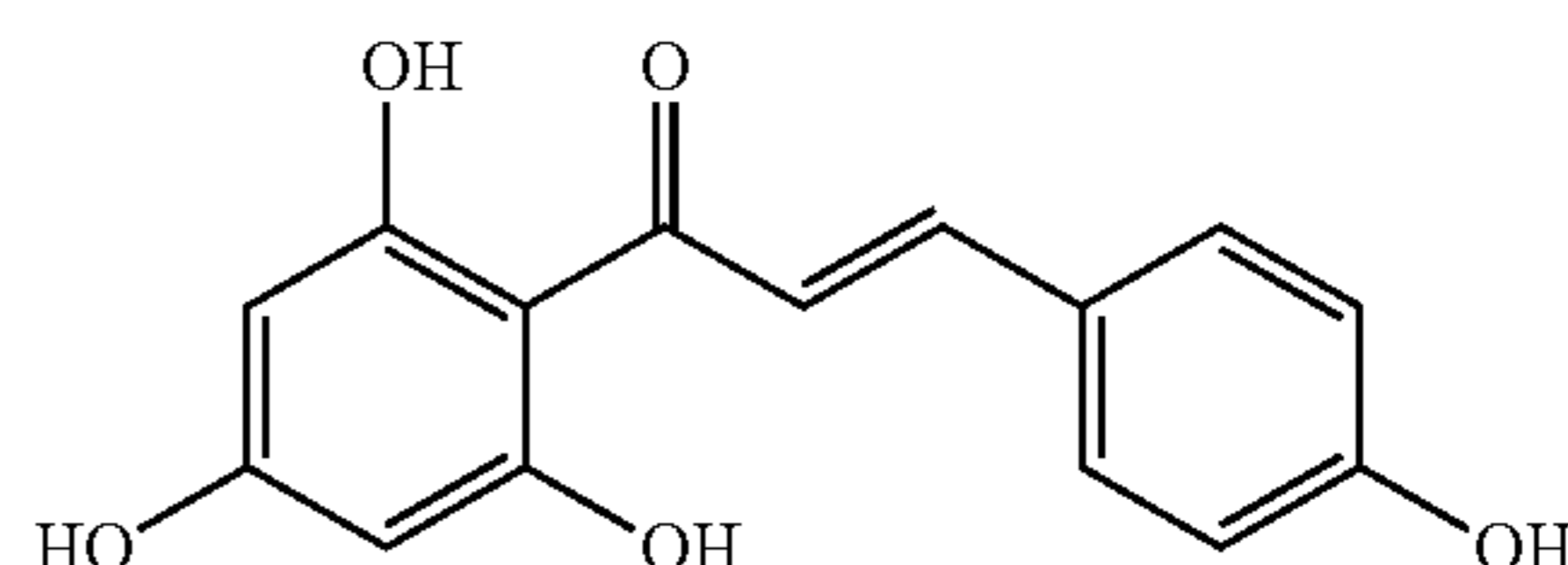
Chalconaringenin
