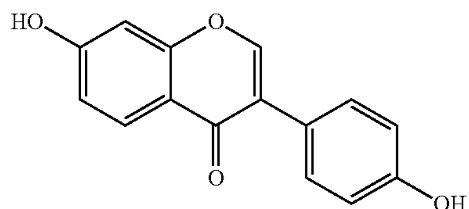
Daidzein
