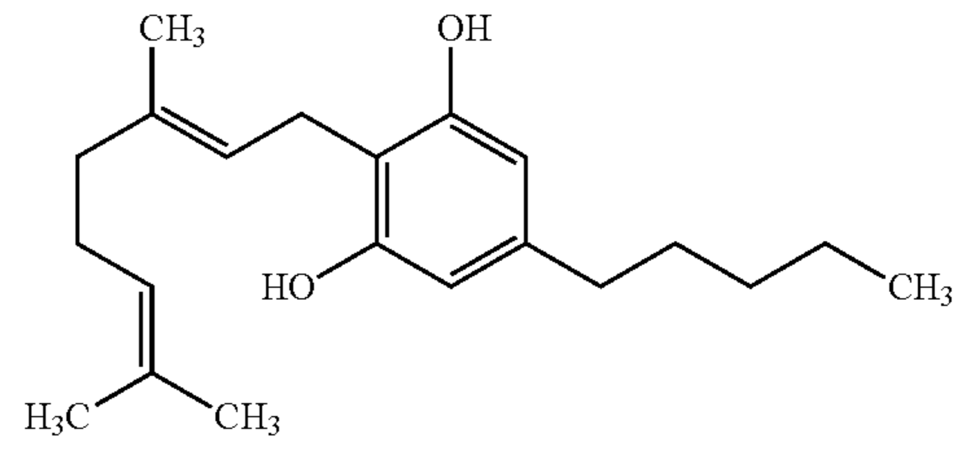
CBG
