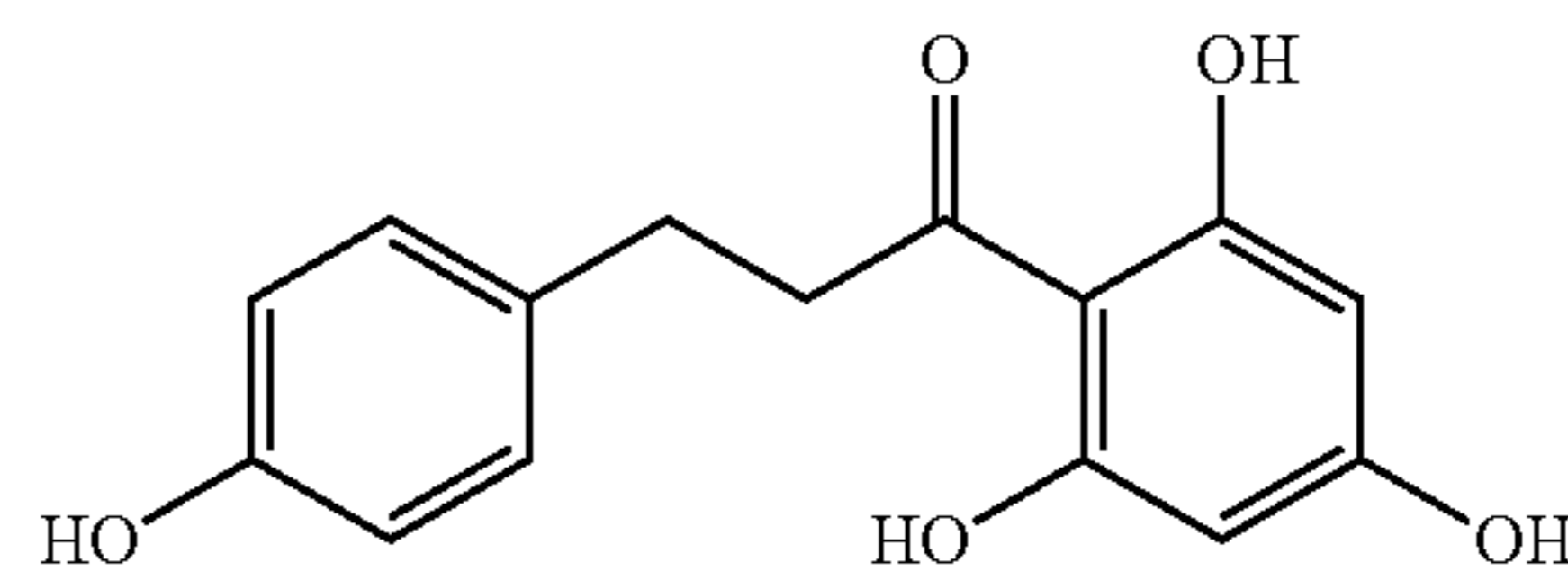
Phloretin
