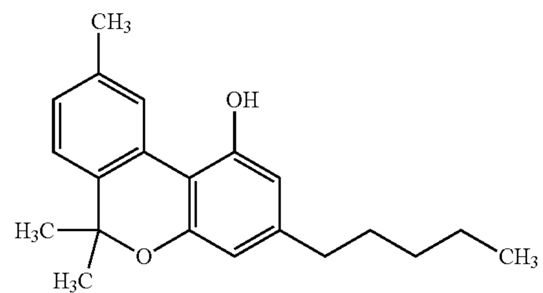
CBN
