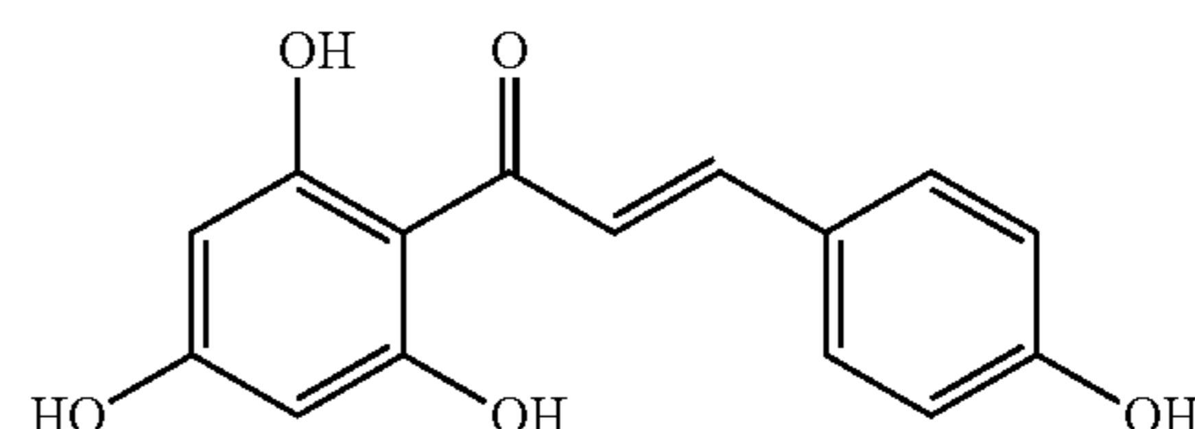
Chalconaringenin
