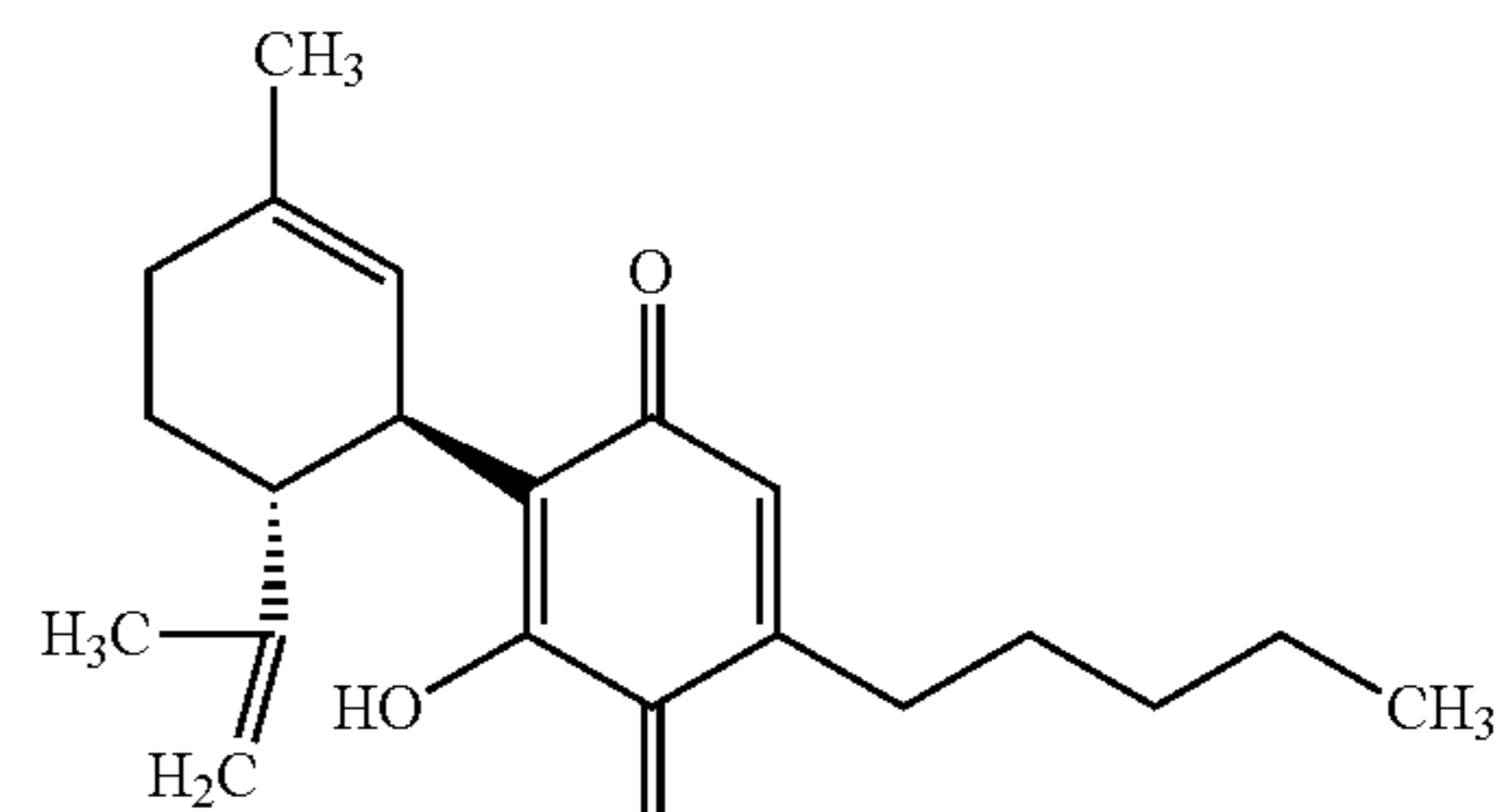
CBQ
