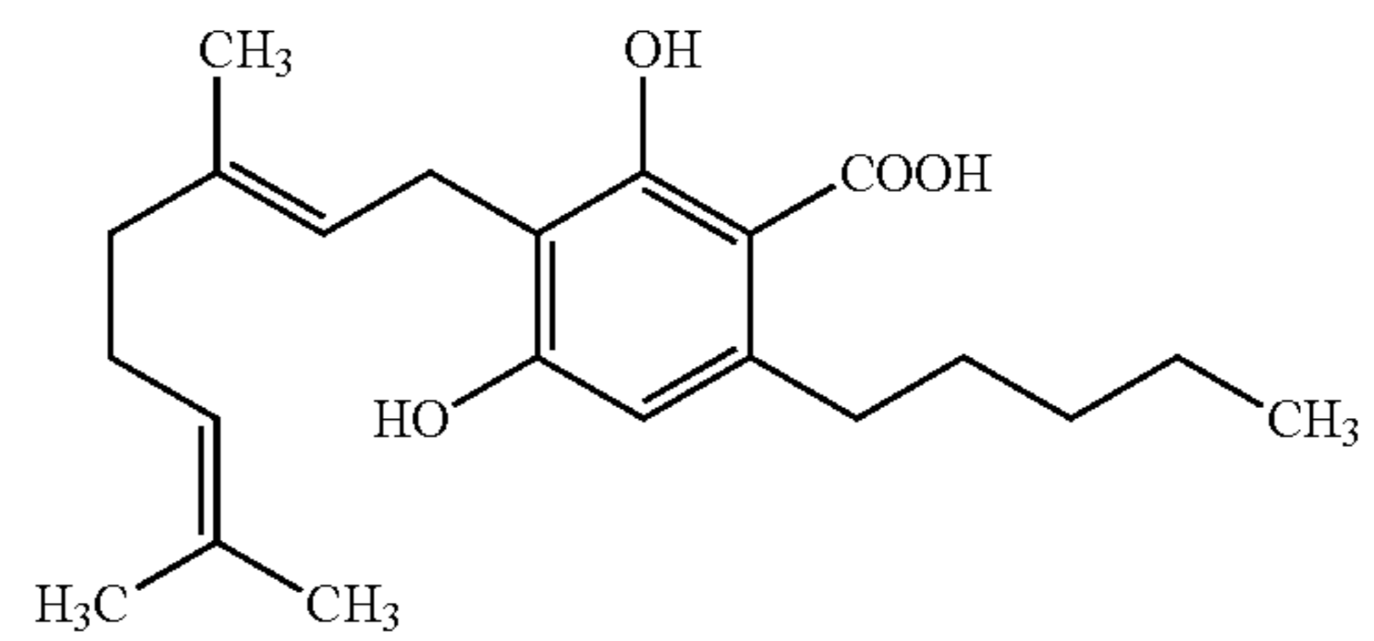
CBGA
