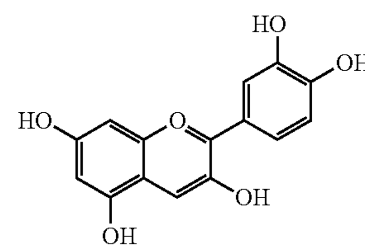
Cyanidin
