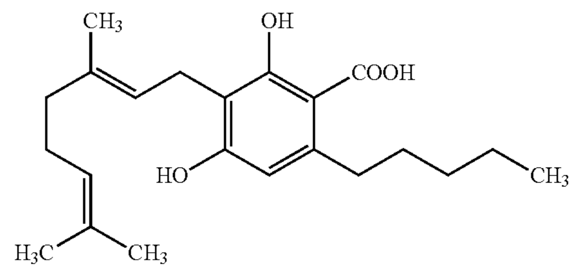
CBGA
