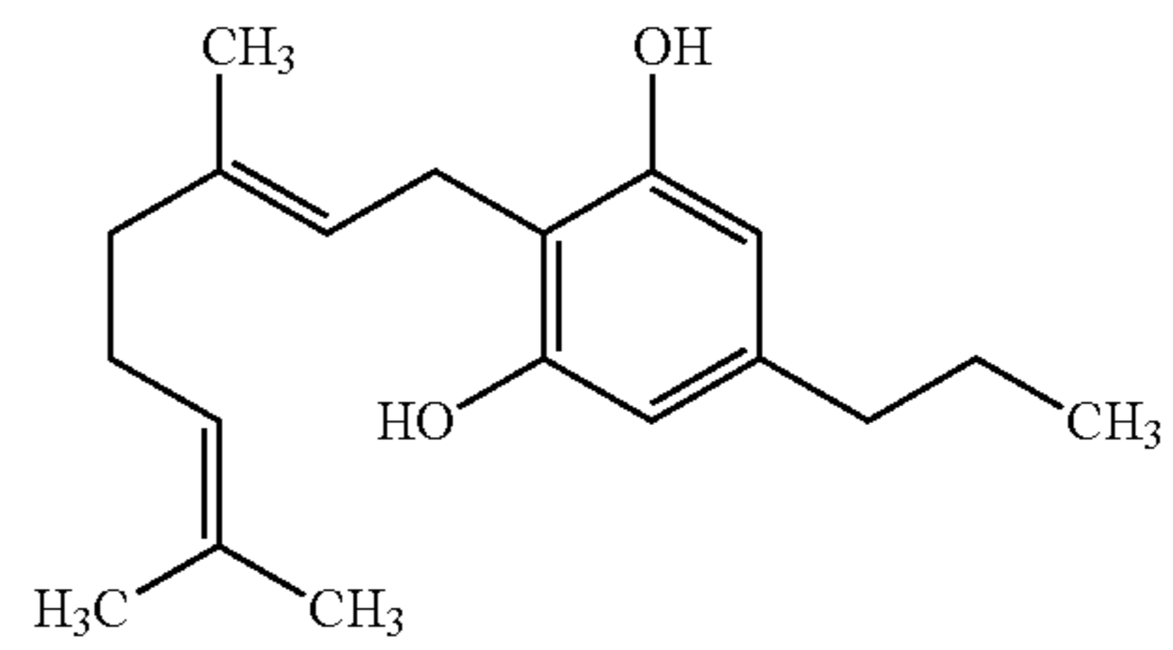
CBGV
