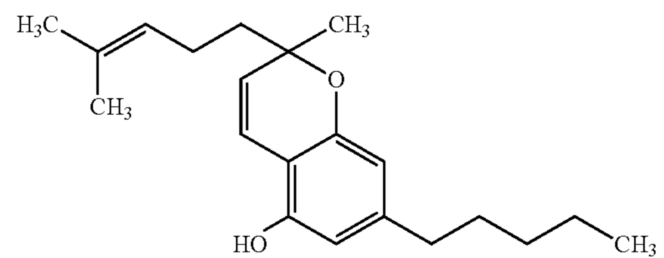
CBC
