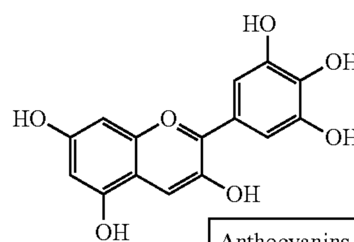
Delphinidin
