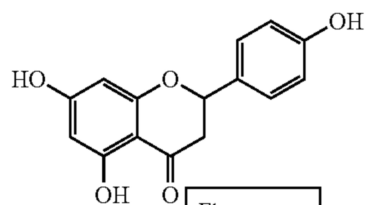
Naringenin
