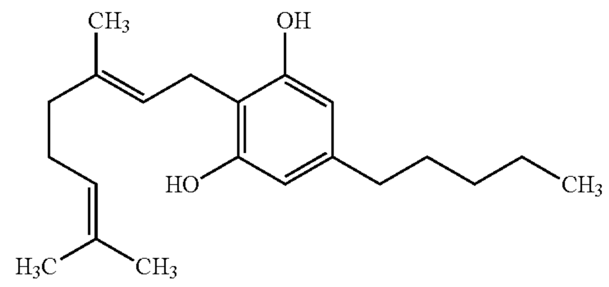
CBG
