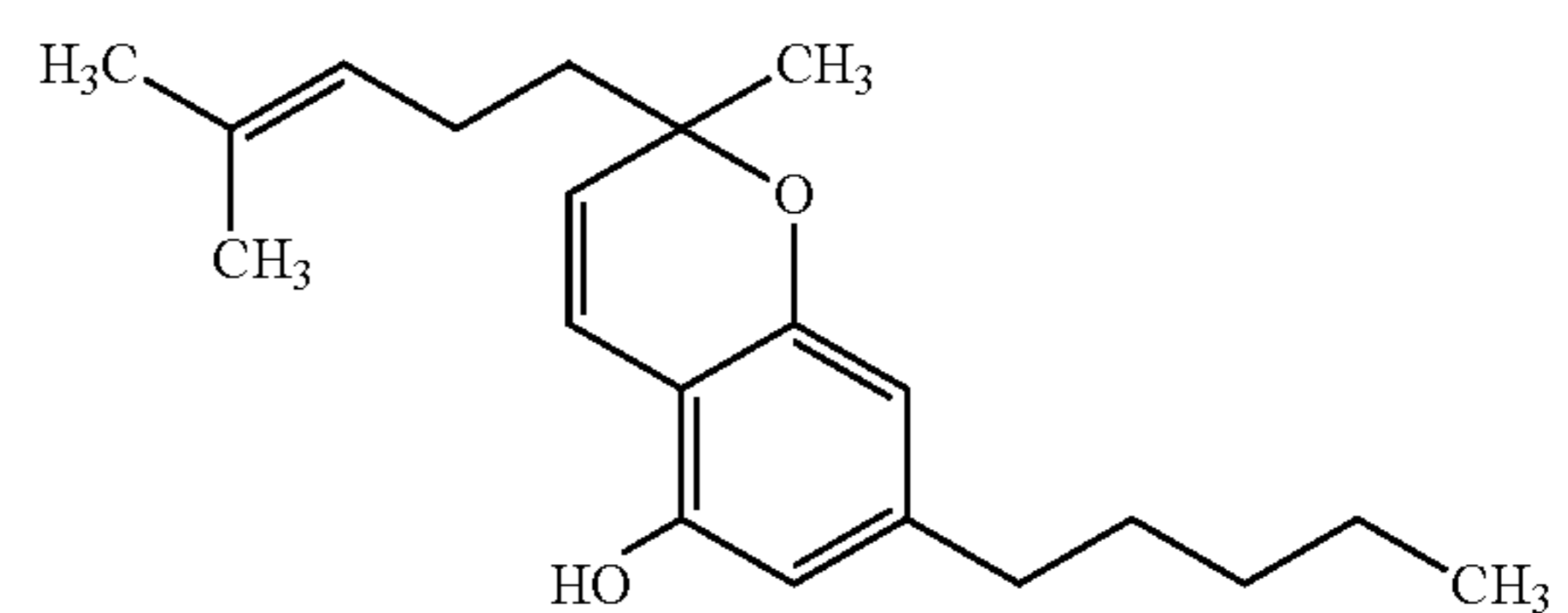
CBC
