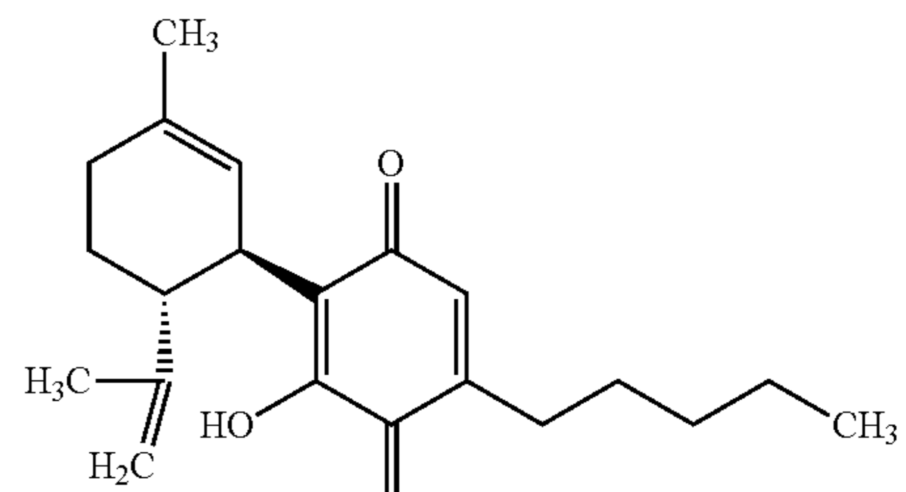
CBQ
