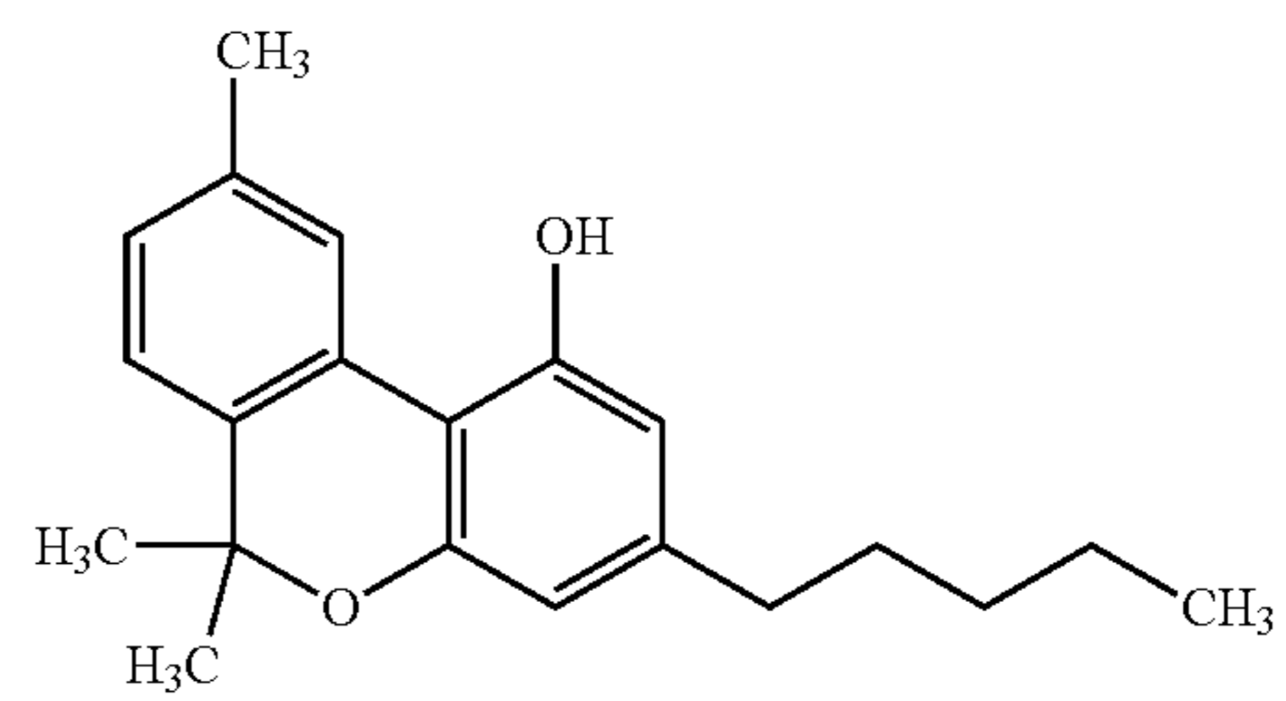
CBN
