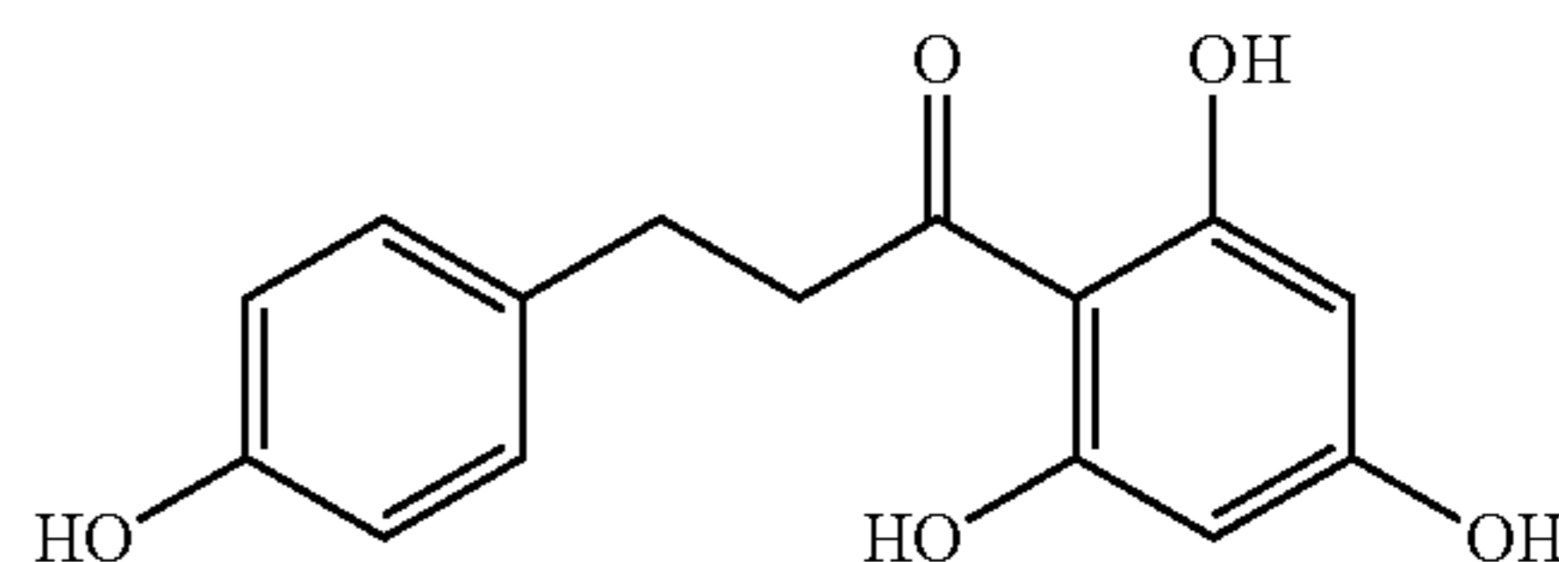
Phloretin
