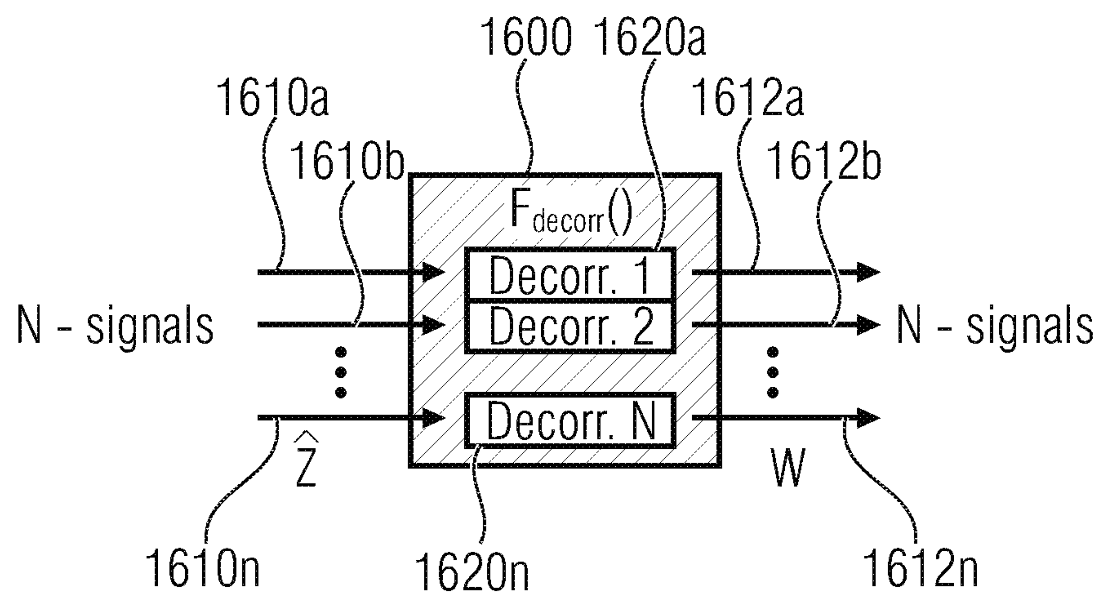
DECORRELATAION UNIT
