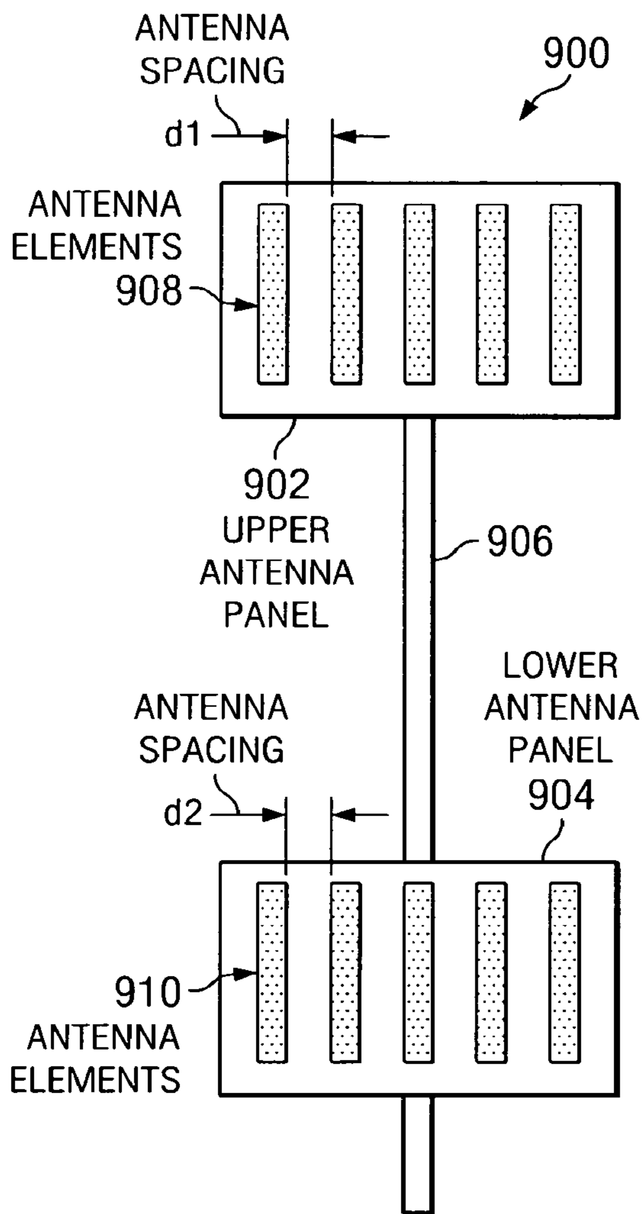
FRONT VIEW
