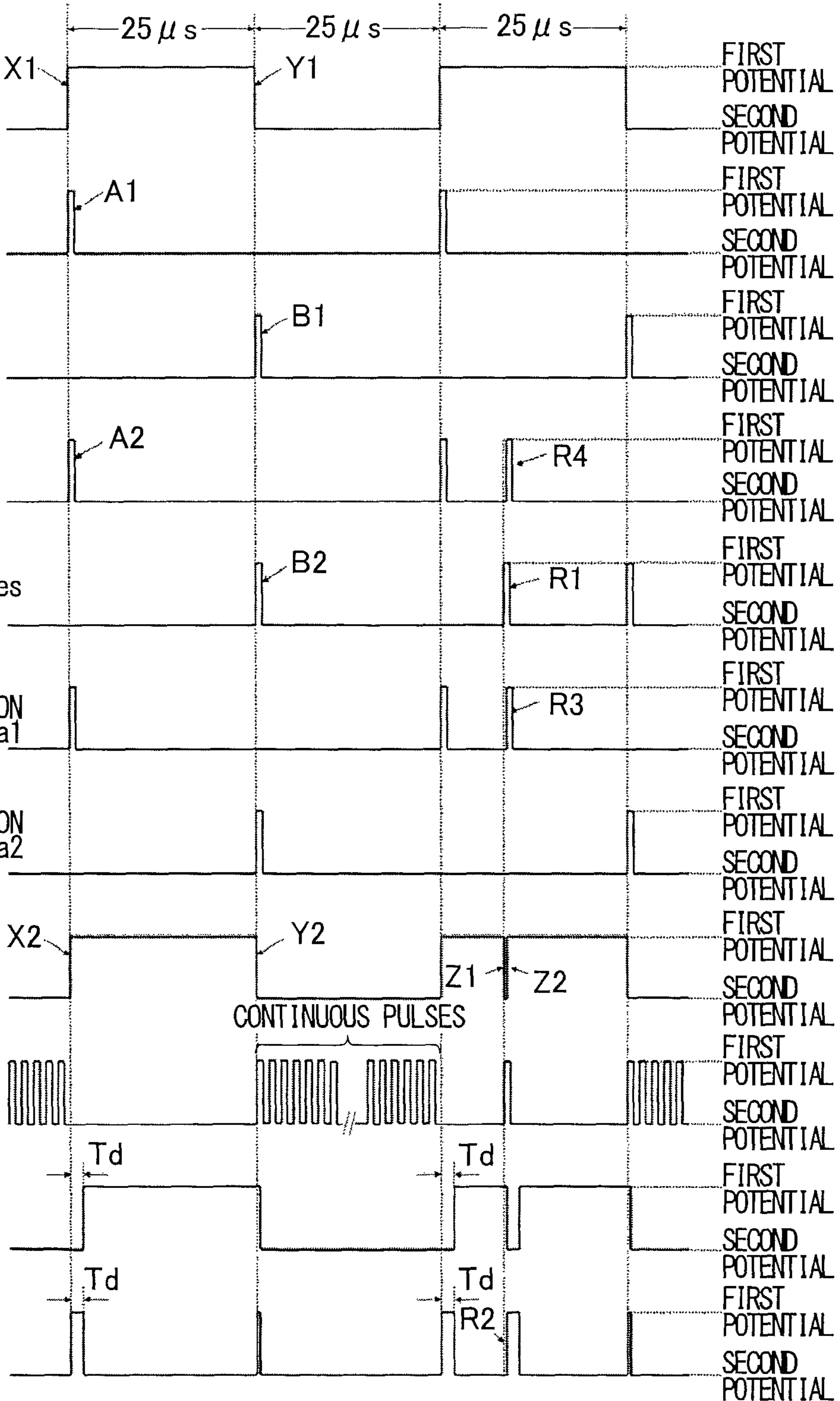
FIG. 17A CONTROL INPUT SIGNAL S_{in}
