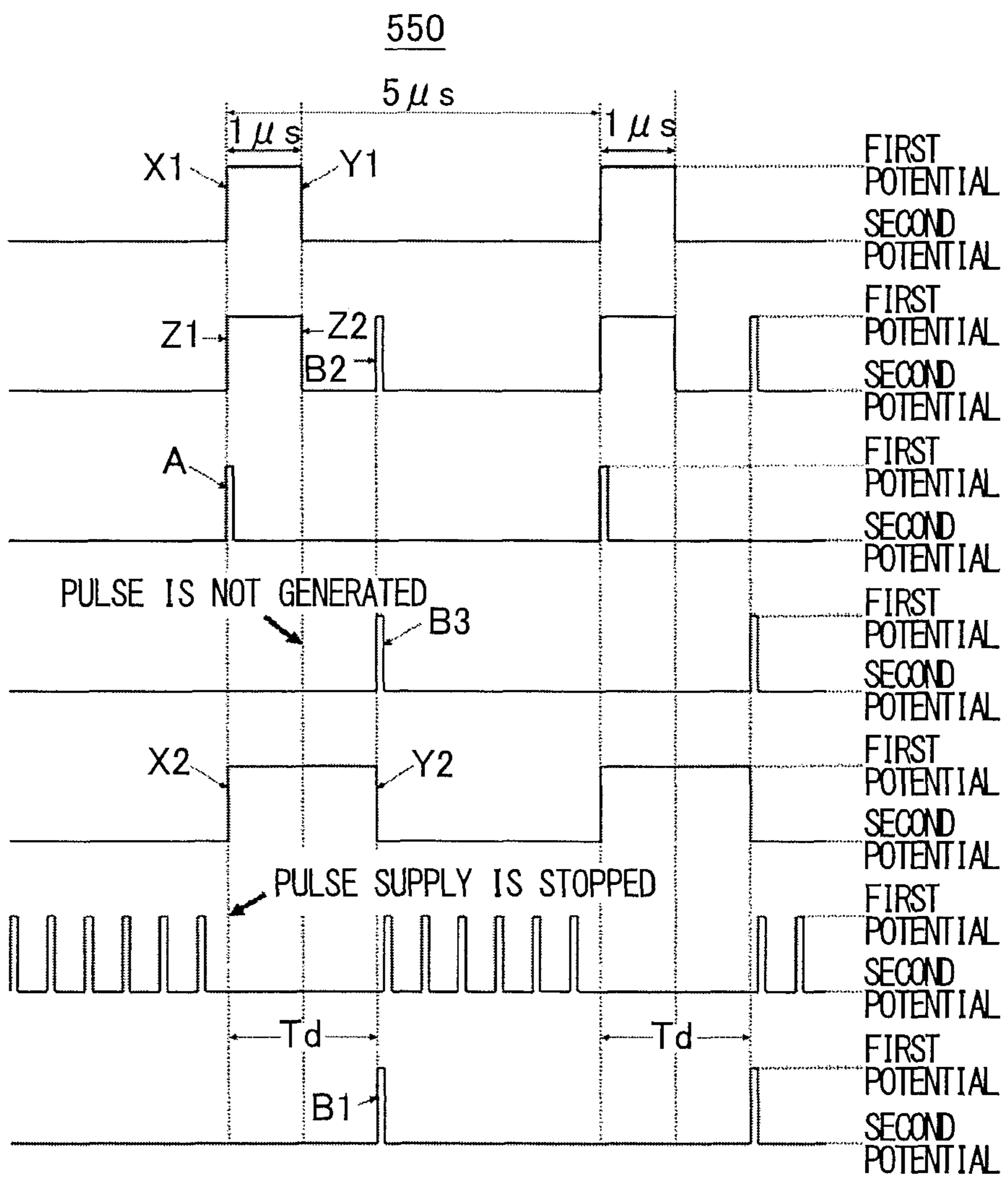
FIG. 7A CONTROL INPUT SIGNAL S_{in}
