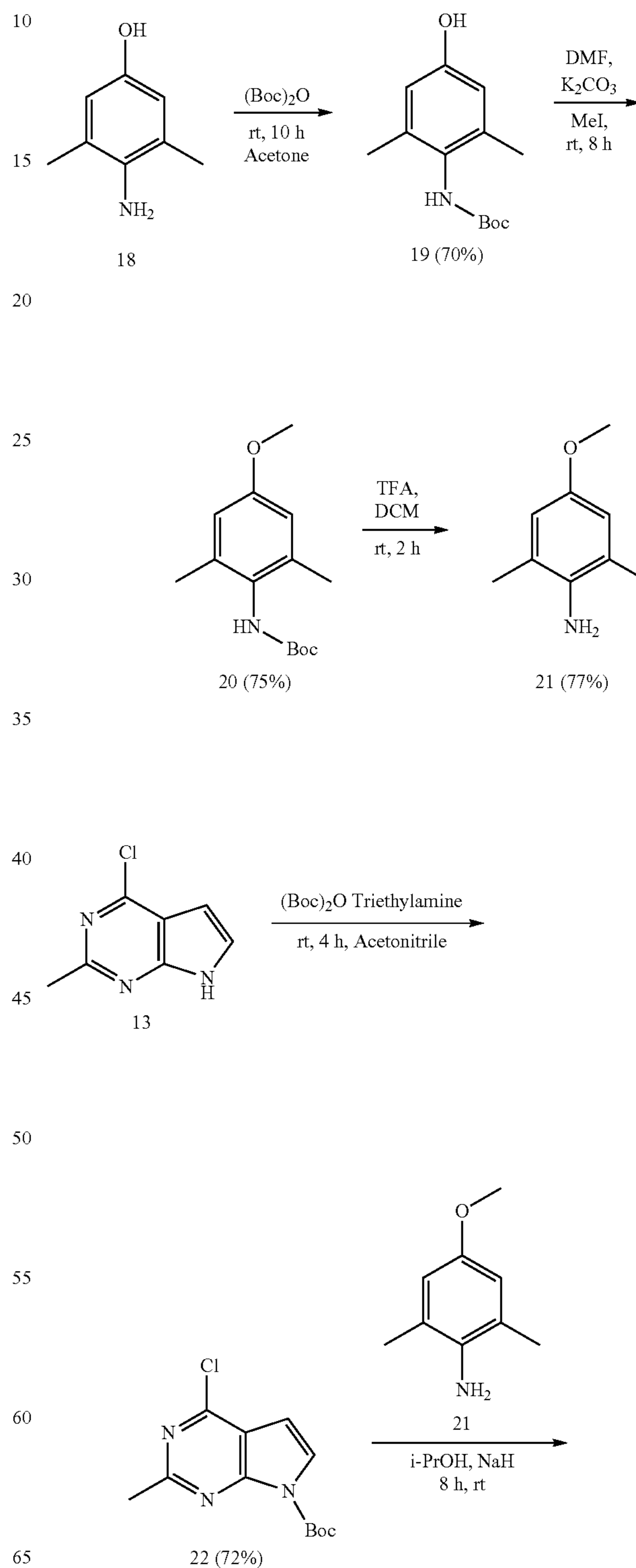
Scheme 2C
