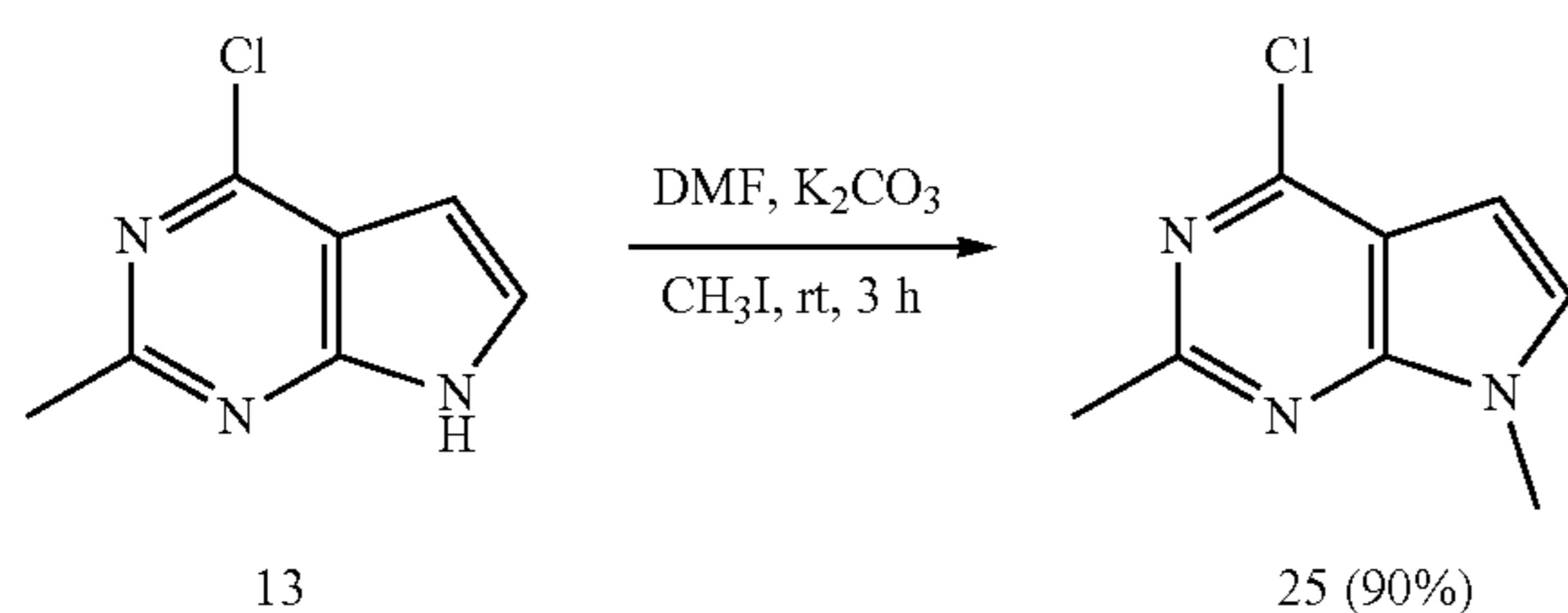
Scheme 3C
