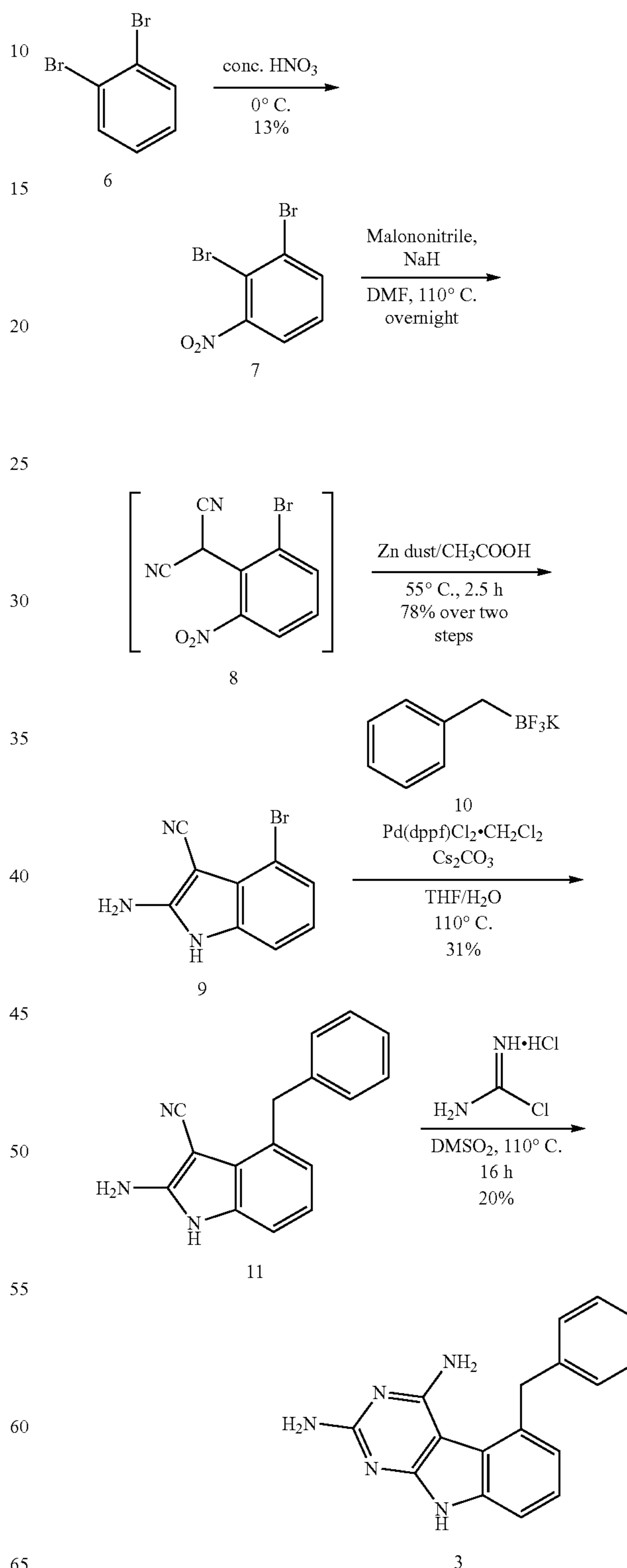
Scheme 1D
