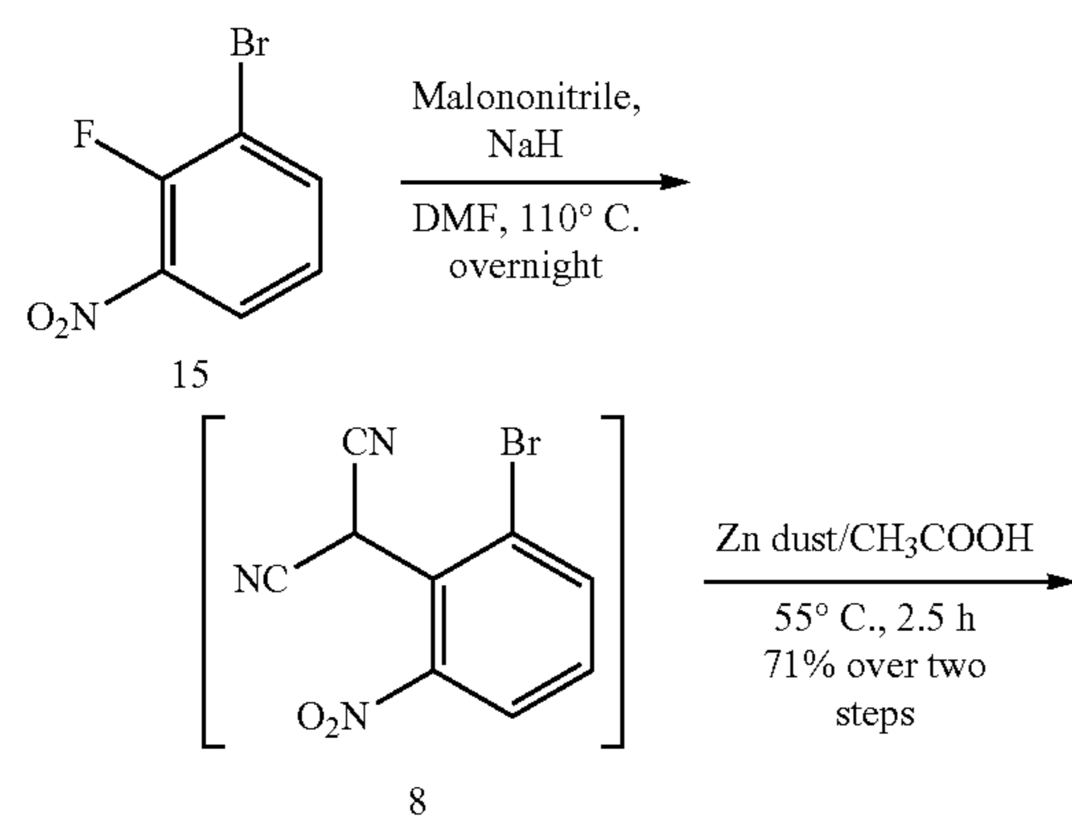
Scheme 3D
