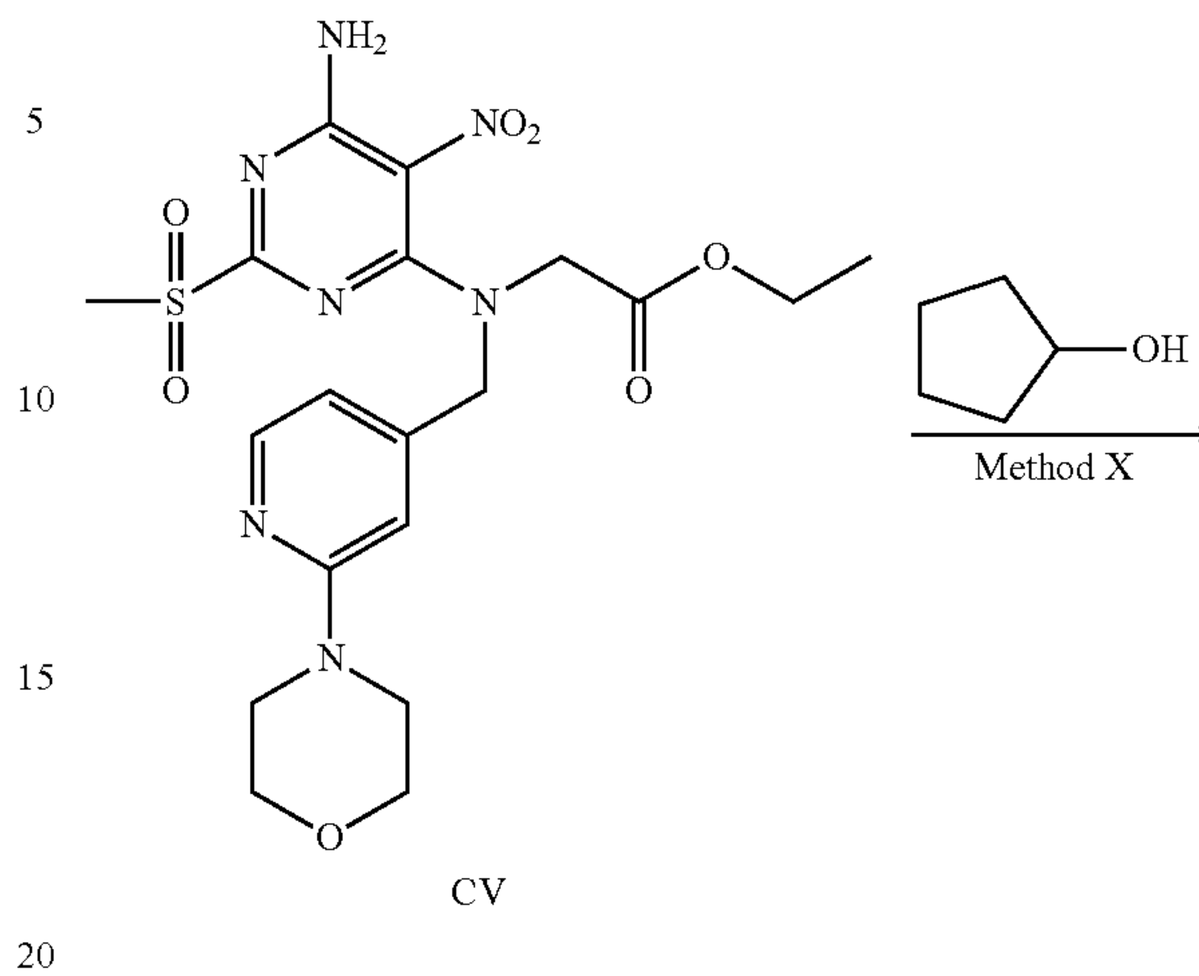
Scheme 58: Example 69, Method X followed by Method XII
