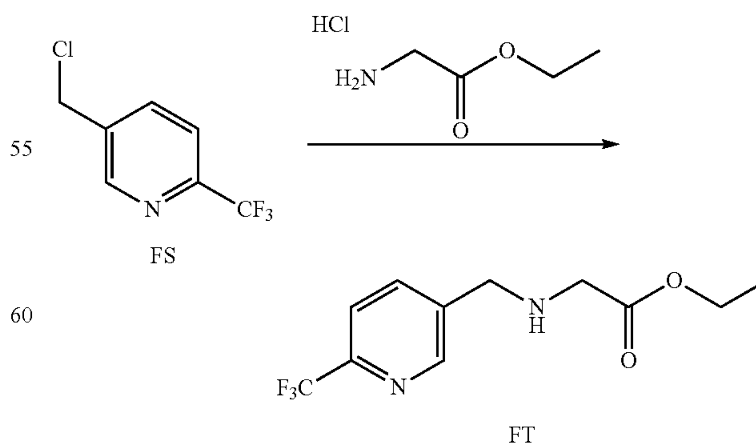
Scheme 103: Prepared Via Method XLXVI:
