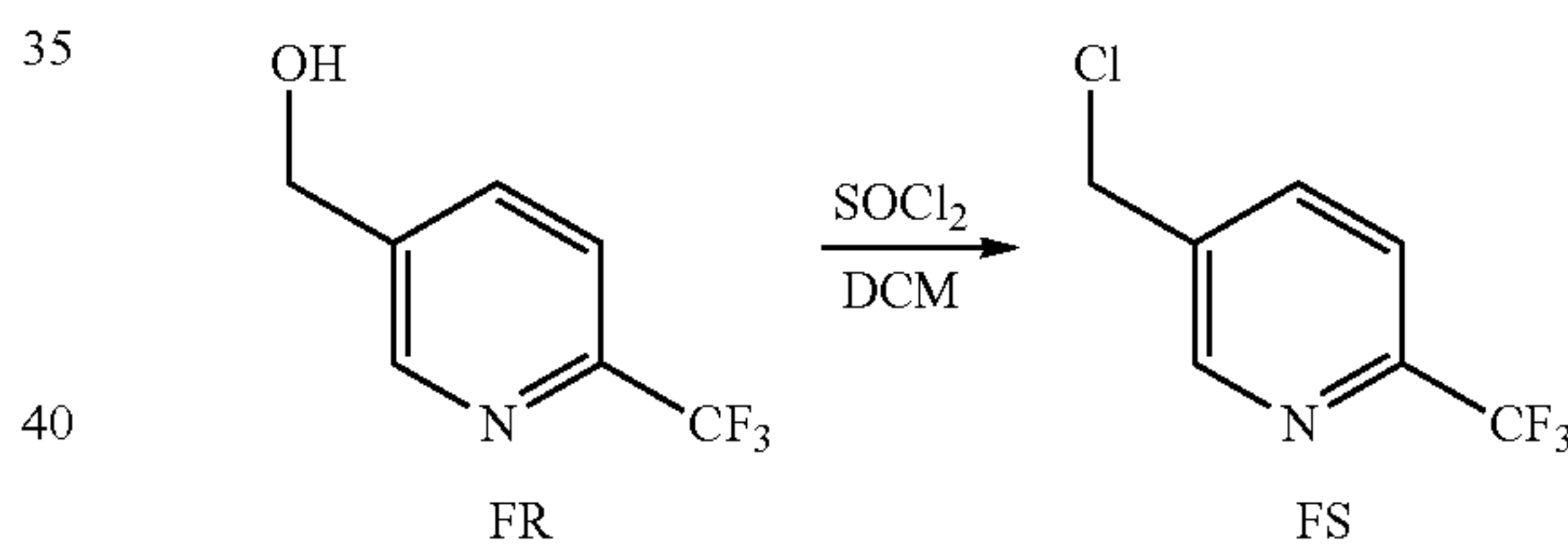
Scheme 102: Prepared Via Method XLXV:
