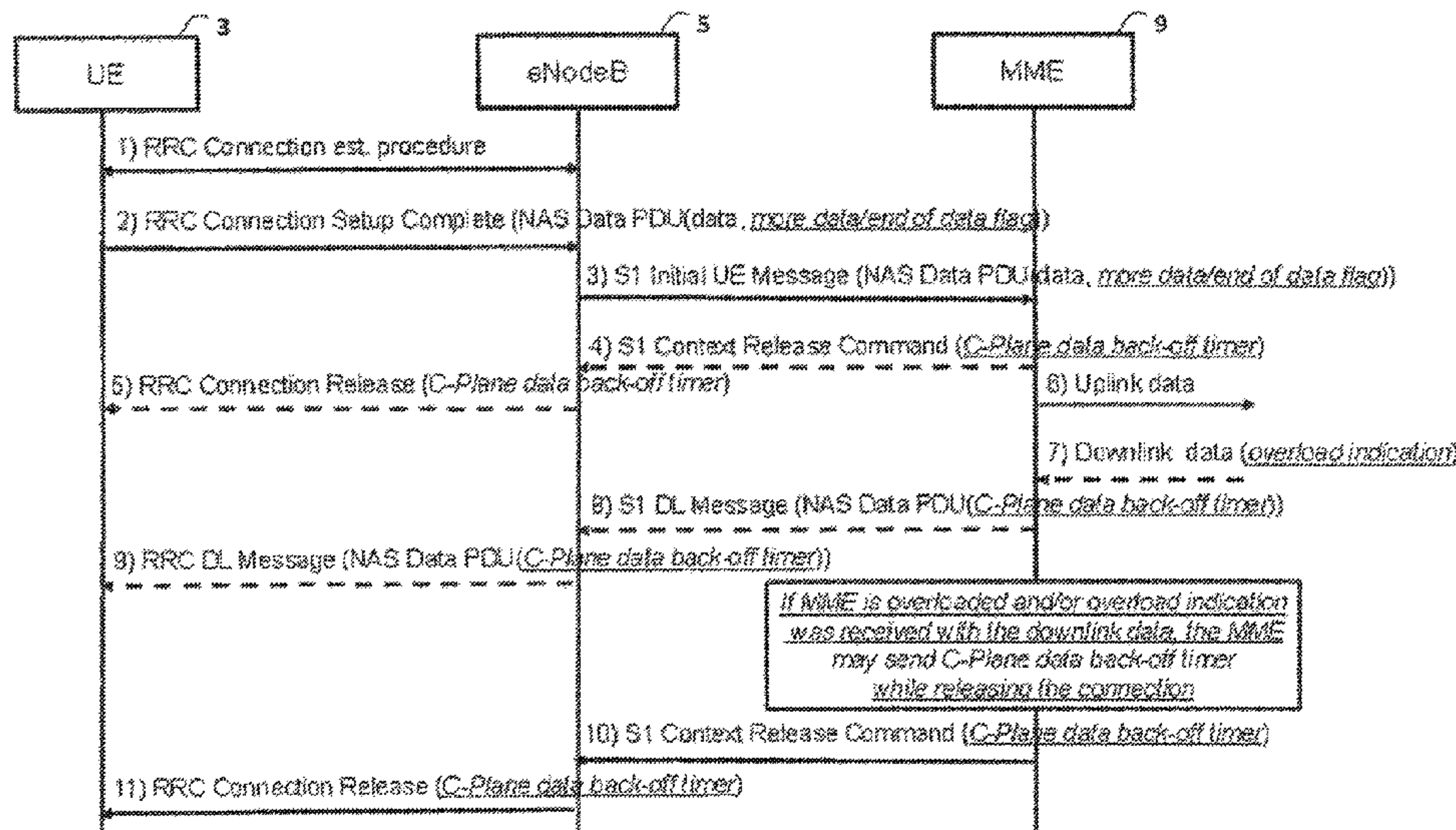
C-Plane data back-off timer while UE is attached for Control Plane CIoT EPS Optimisation
