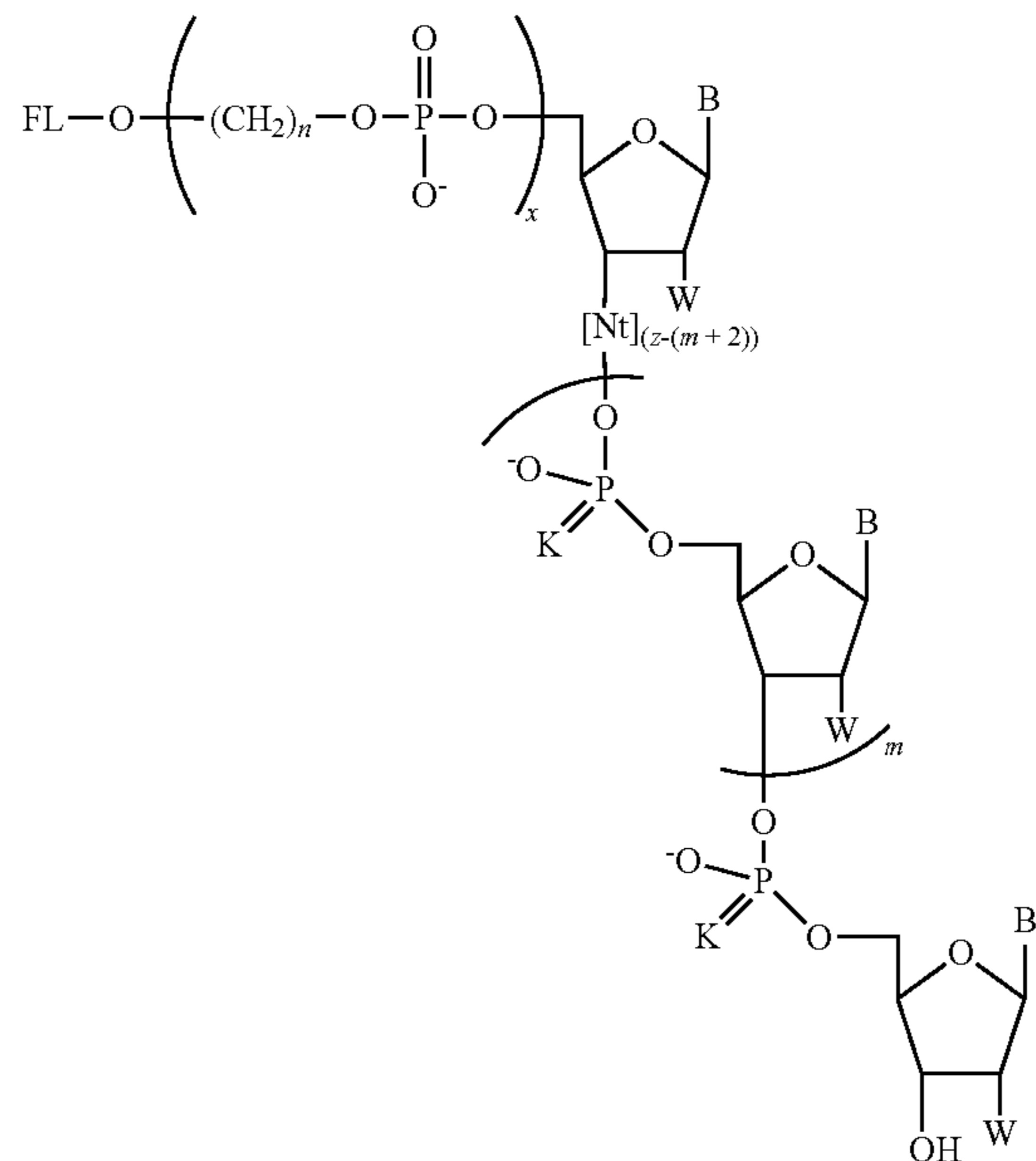
Formula I-D
