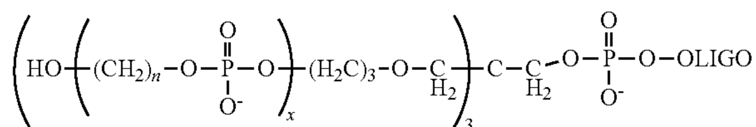
Formula VI-A1
