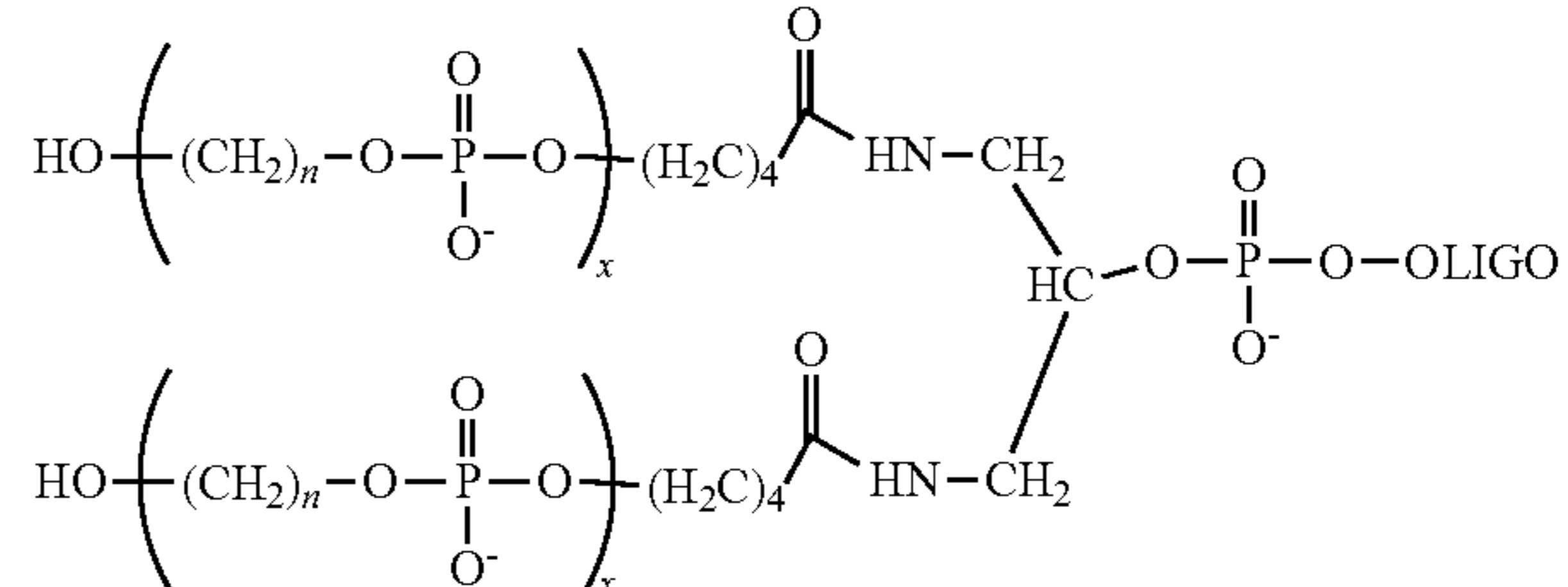
Formula V-A
