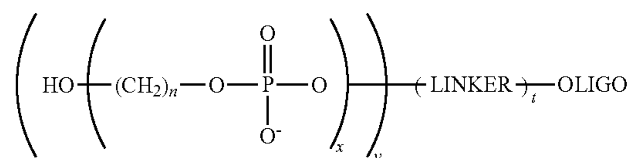
Formula IV
