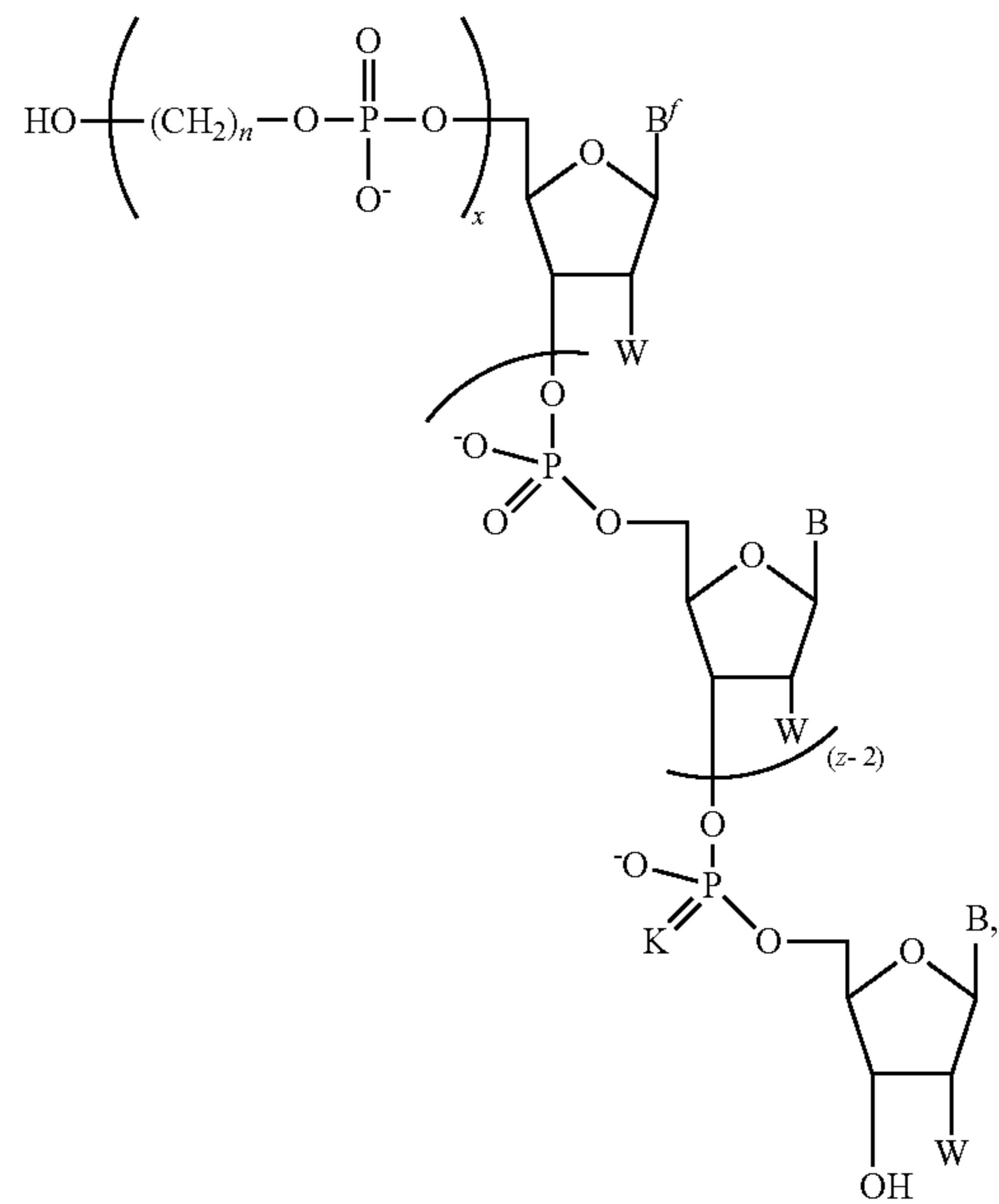
Formula I-E
