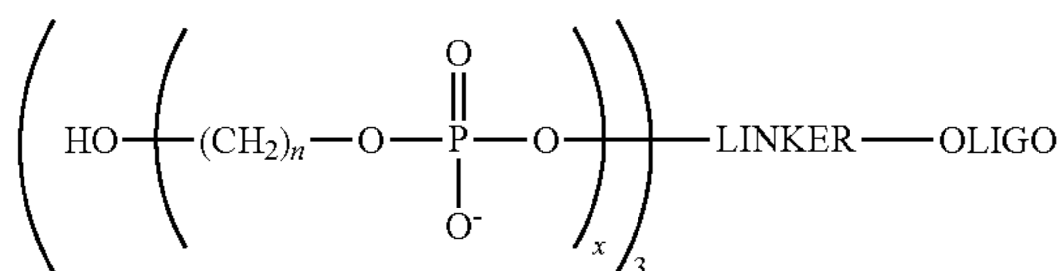
Formula VI
