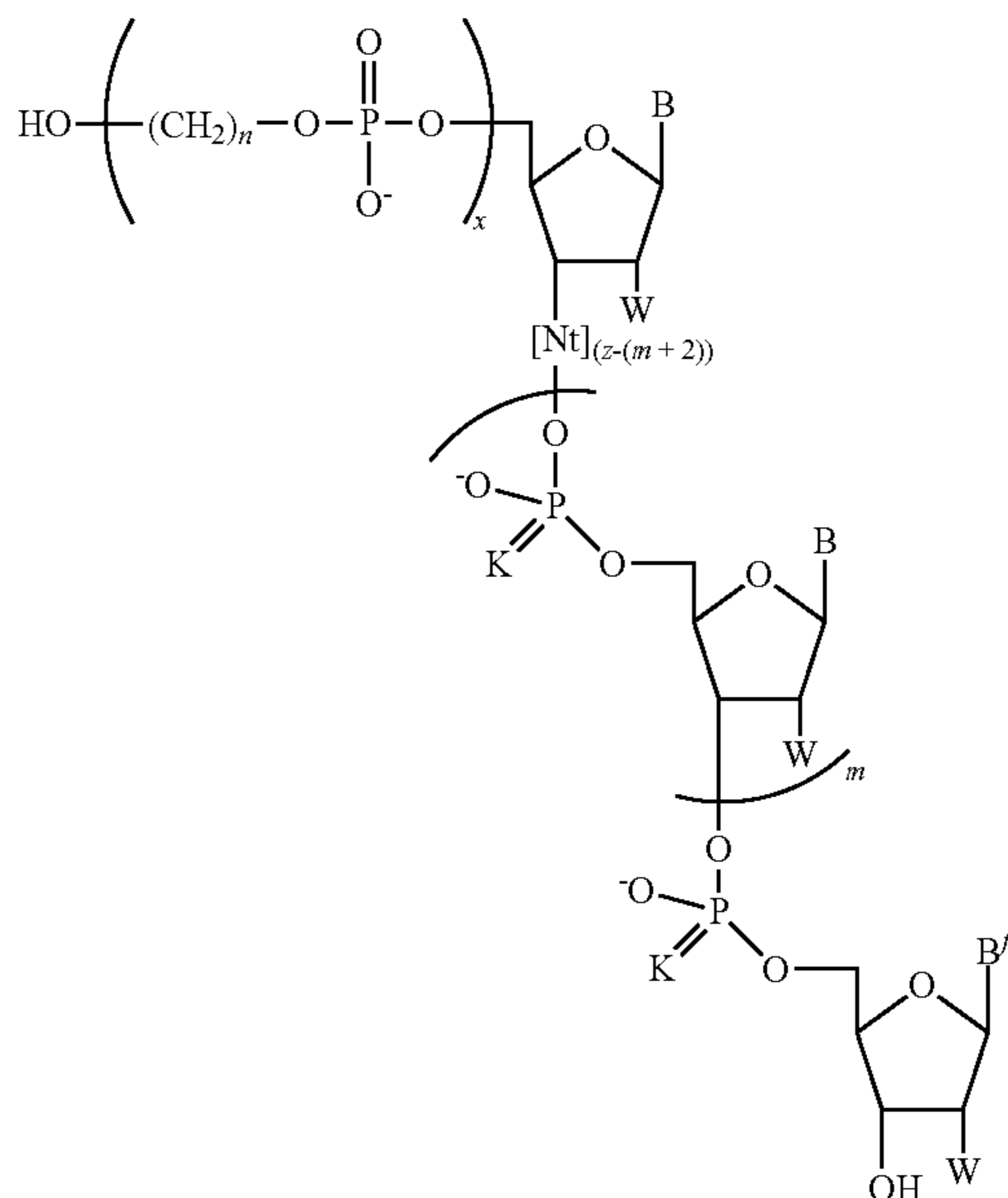
Formula I-B
