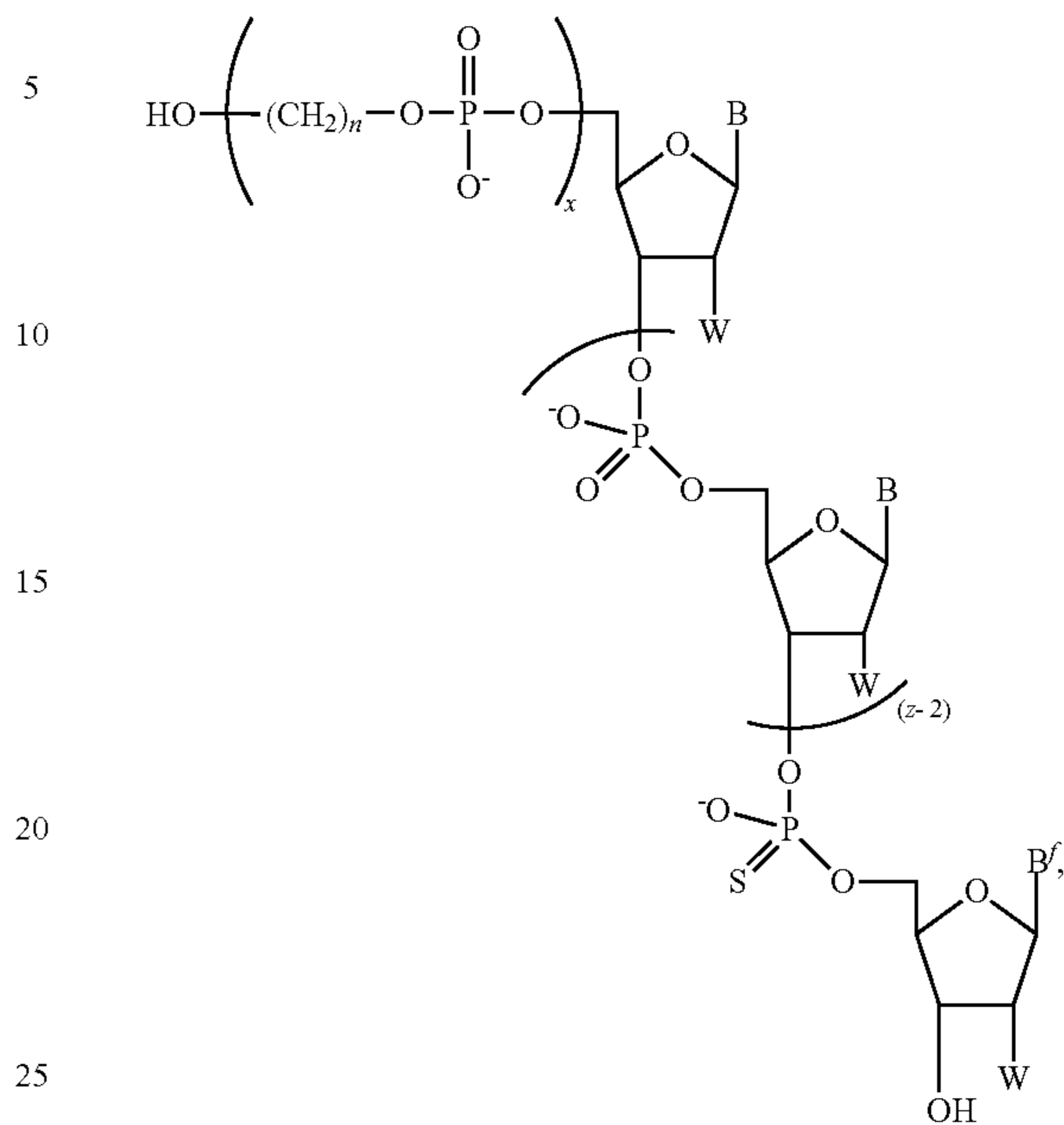
Formula -I-H
