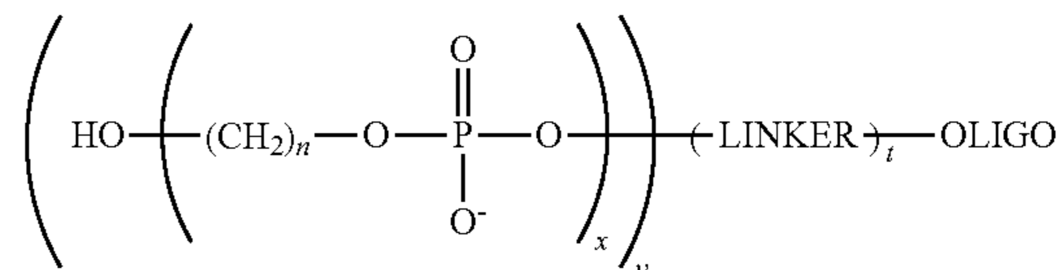
Formula IV
