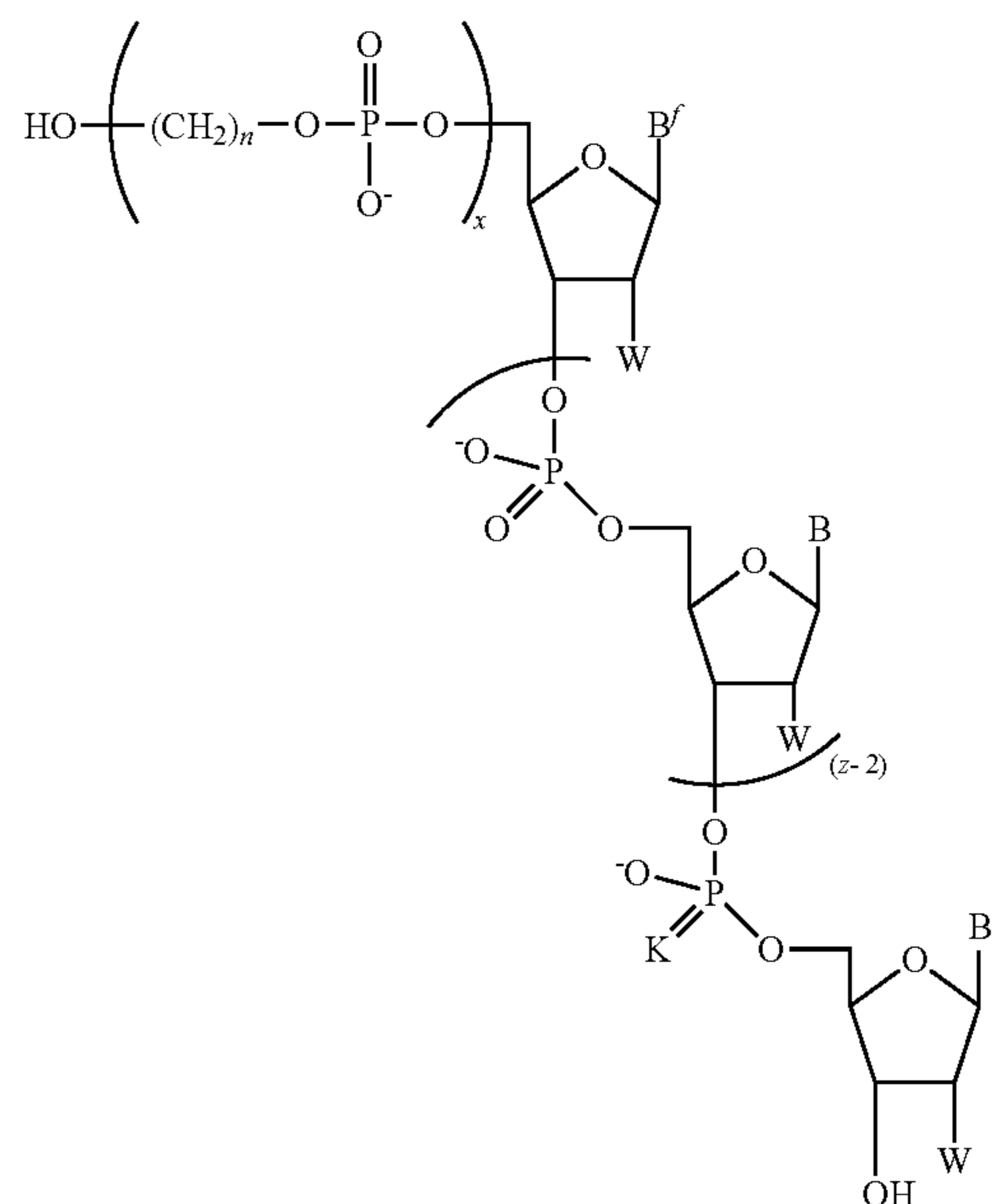
Formula I-E
