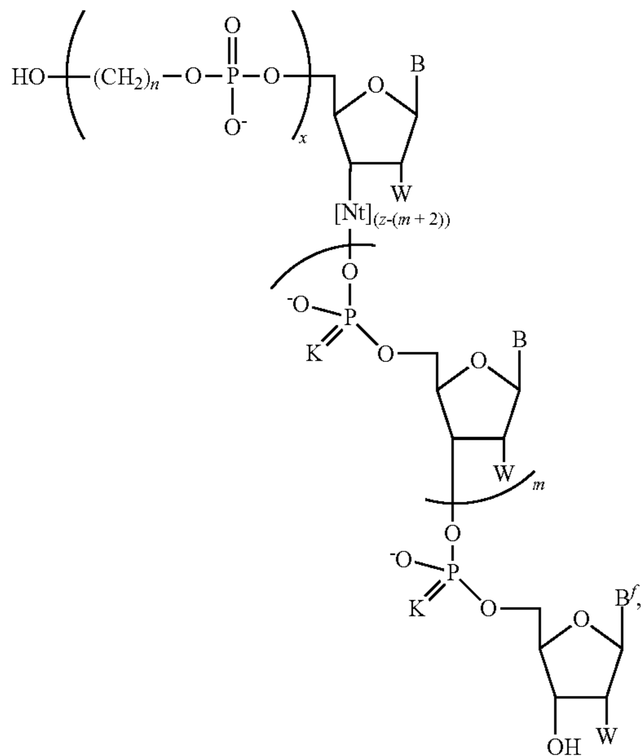
Formula I-C
