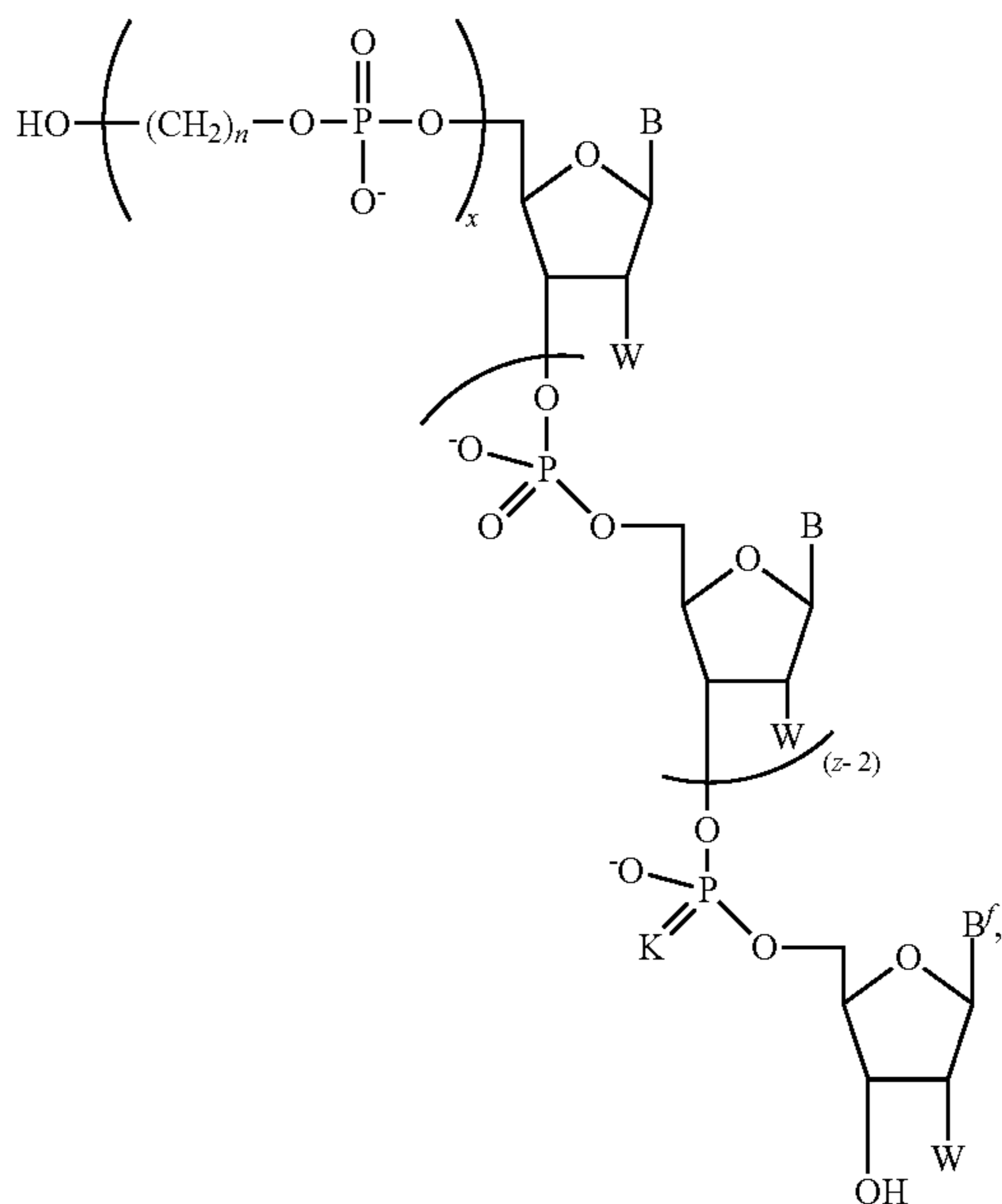
Formula I-F
