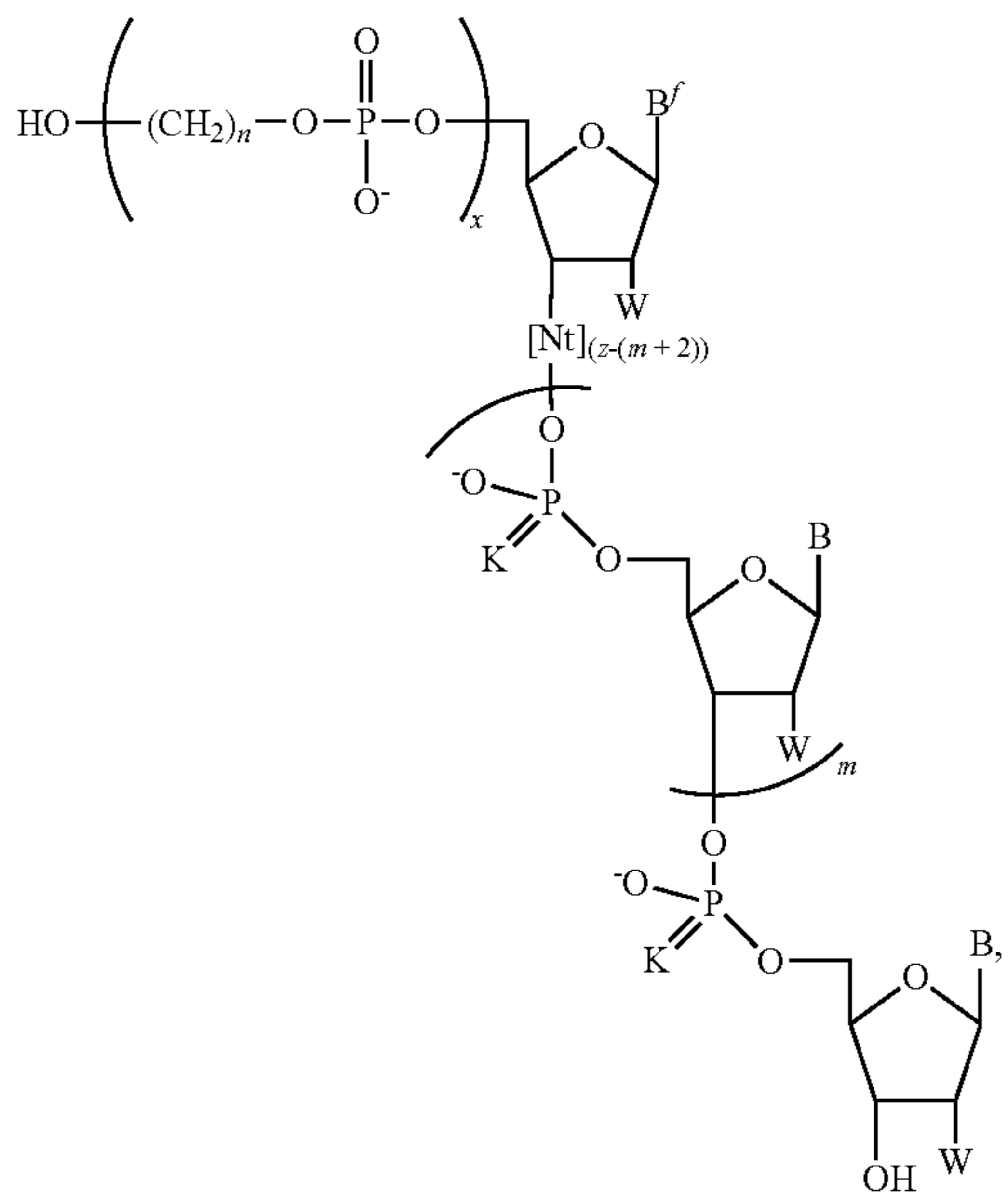
Formula I-C
