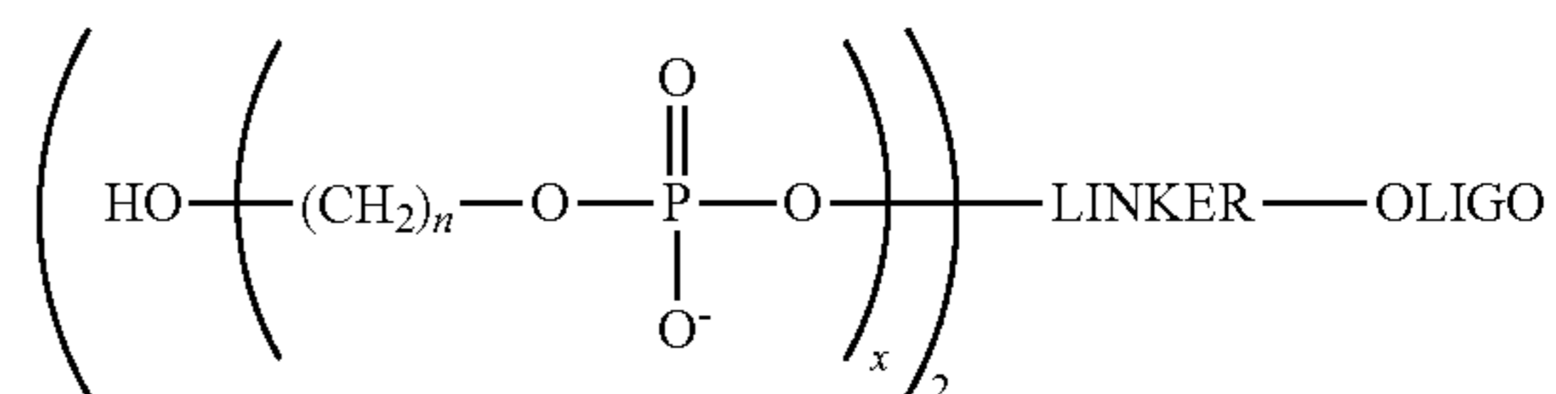
Formula V
