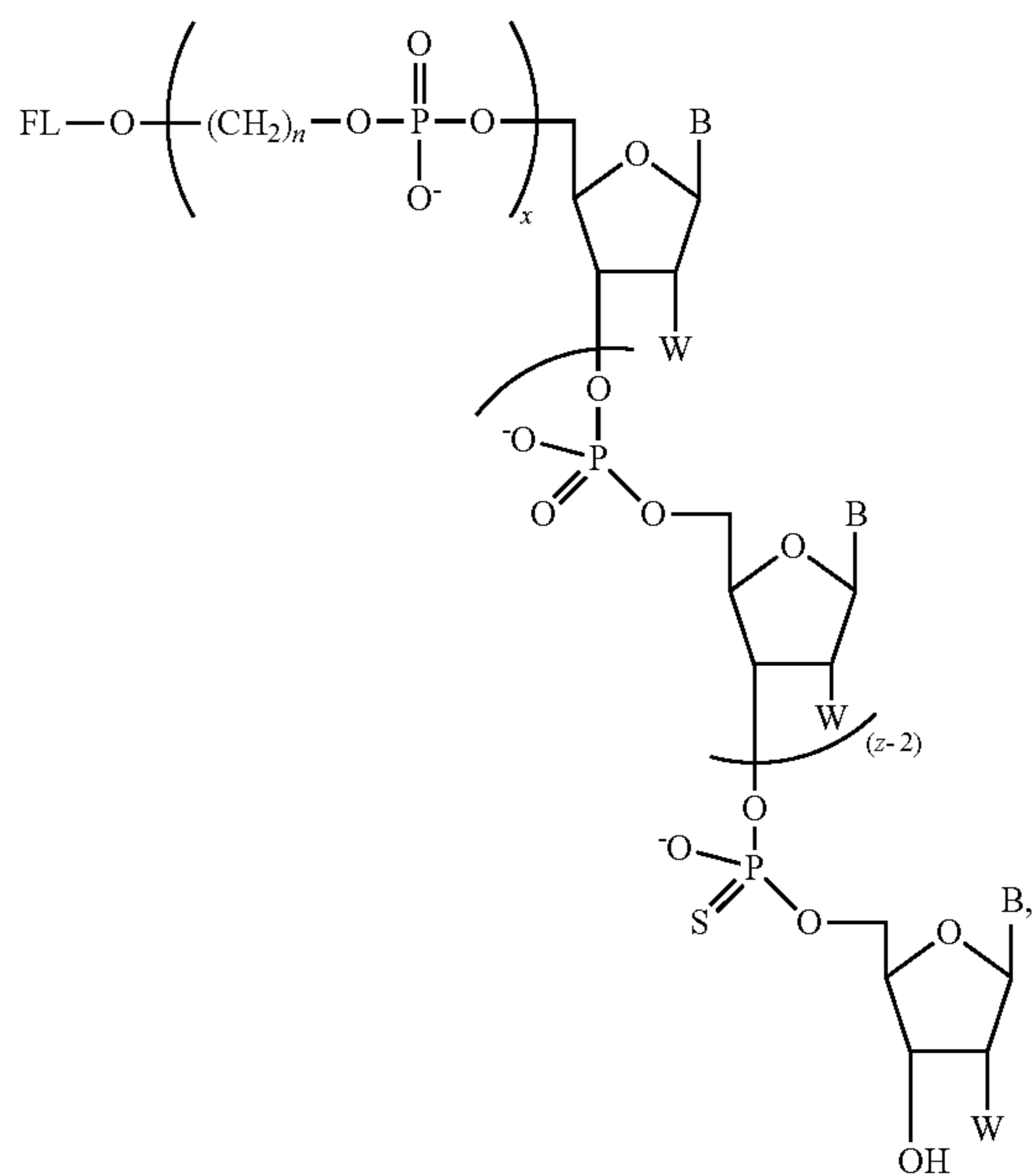
Formula I-J
