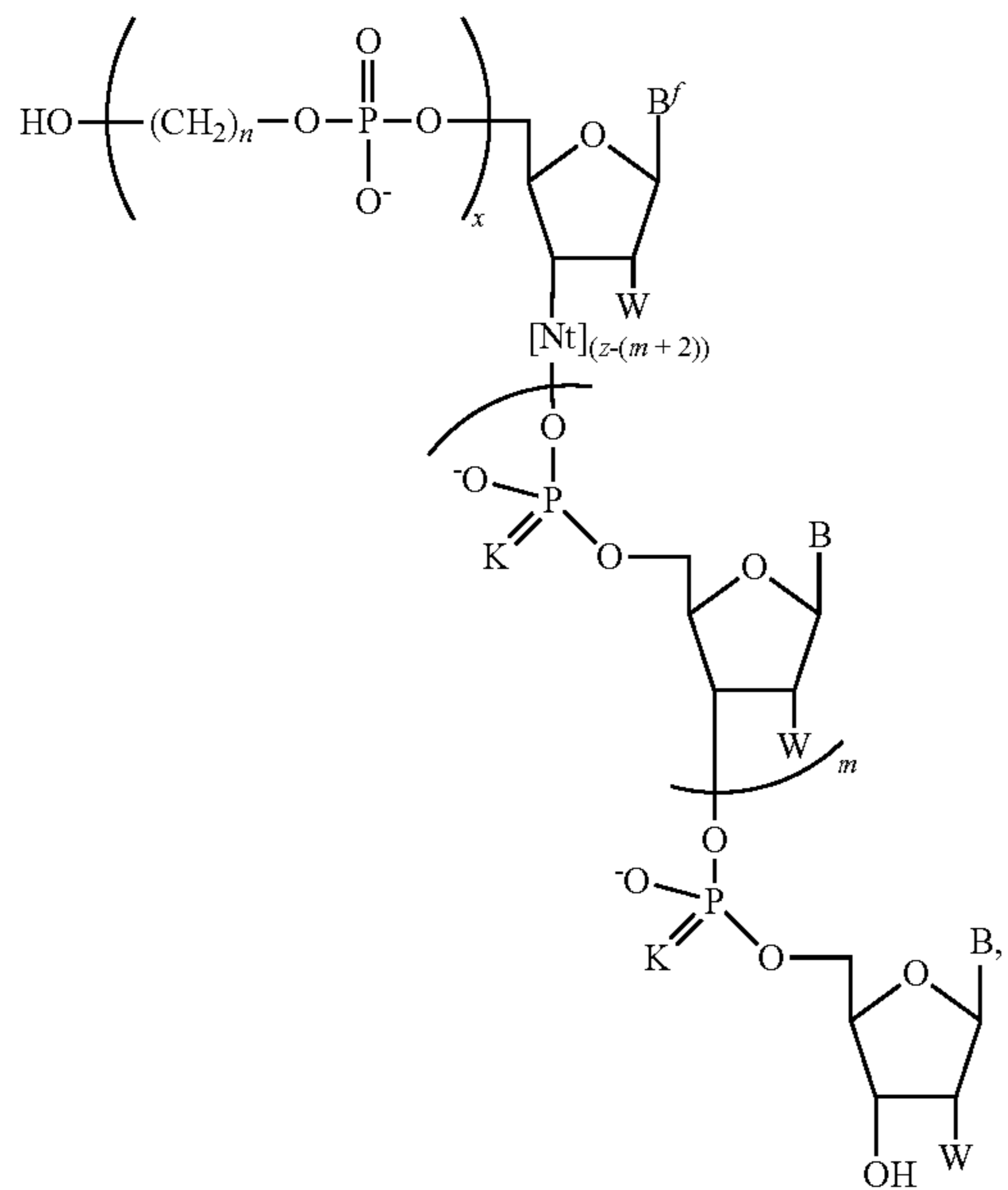
Formula I-C
