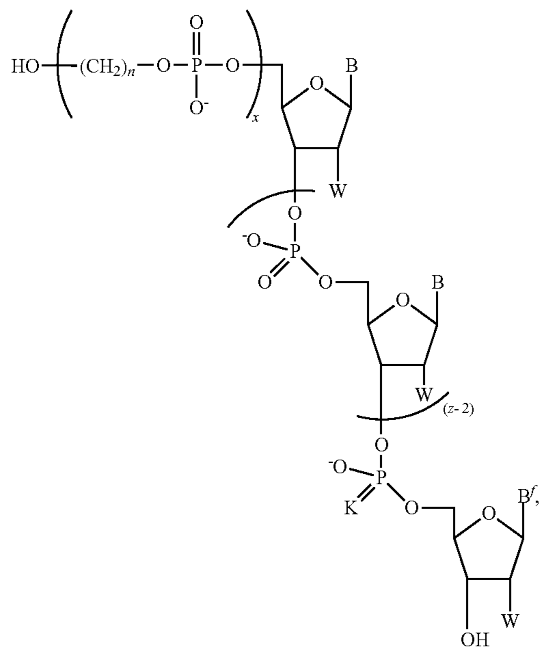
Formula -I-F
