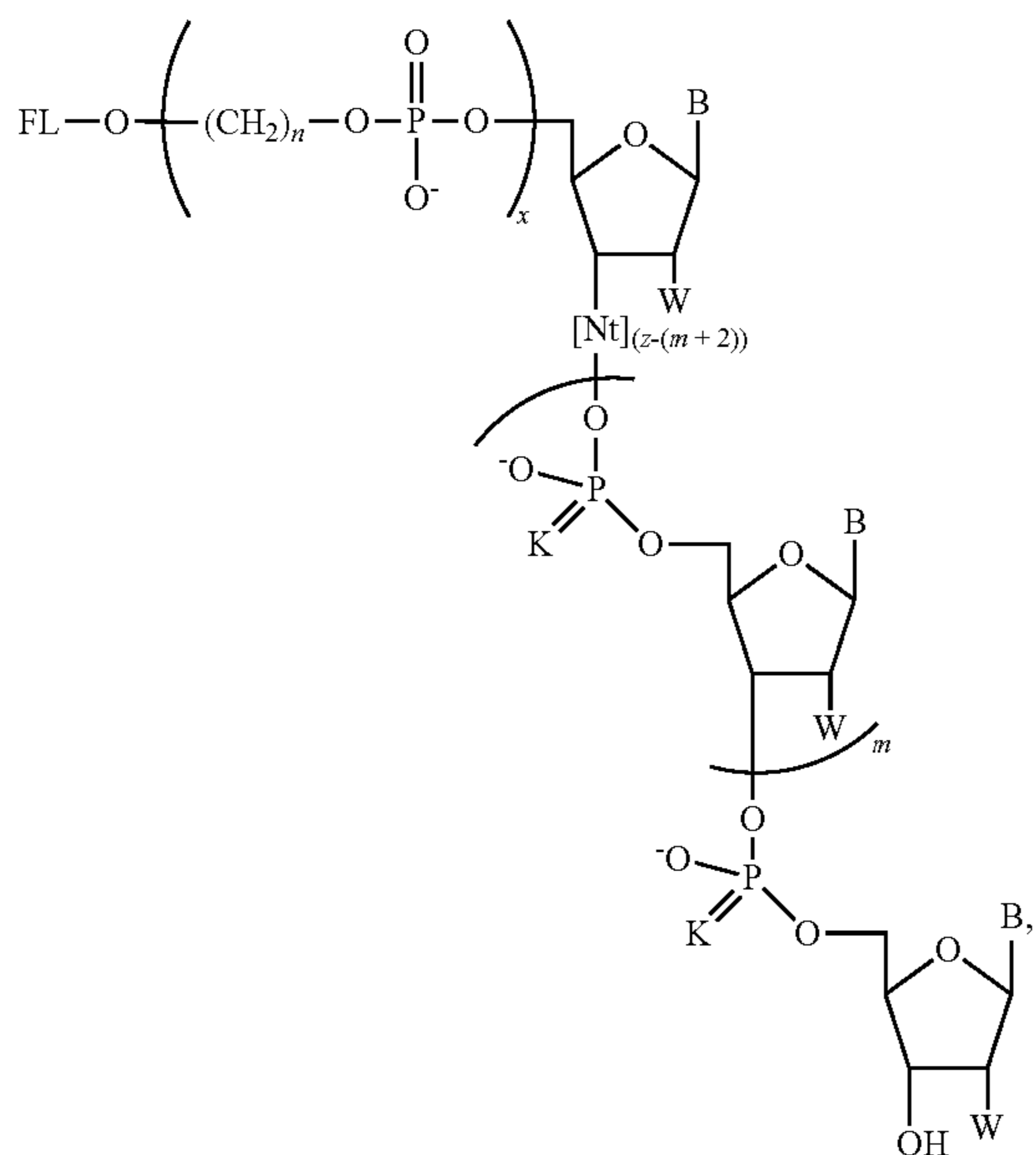
Formula I-D
