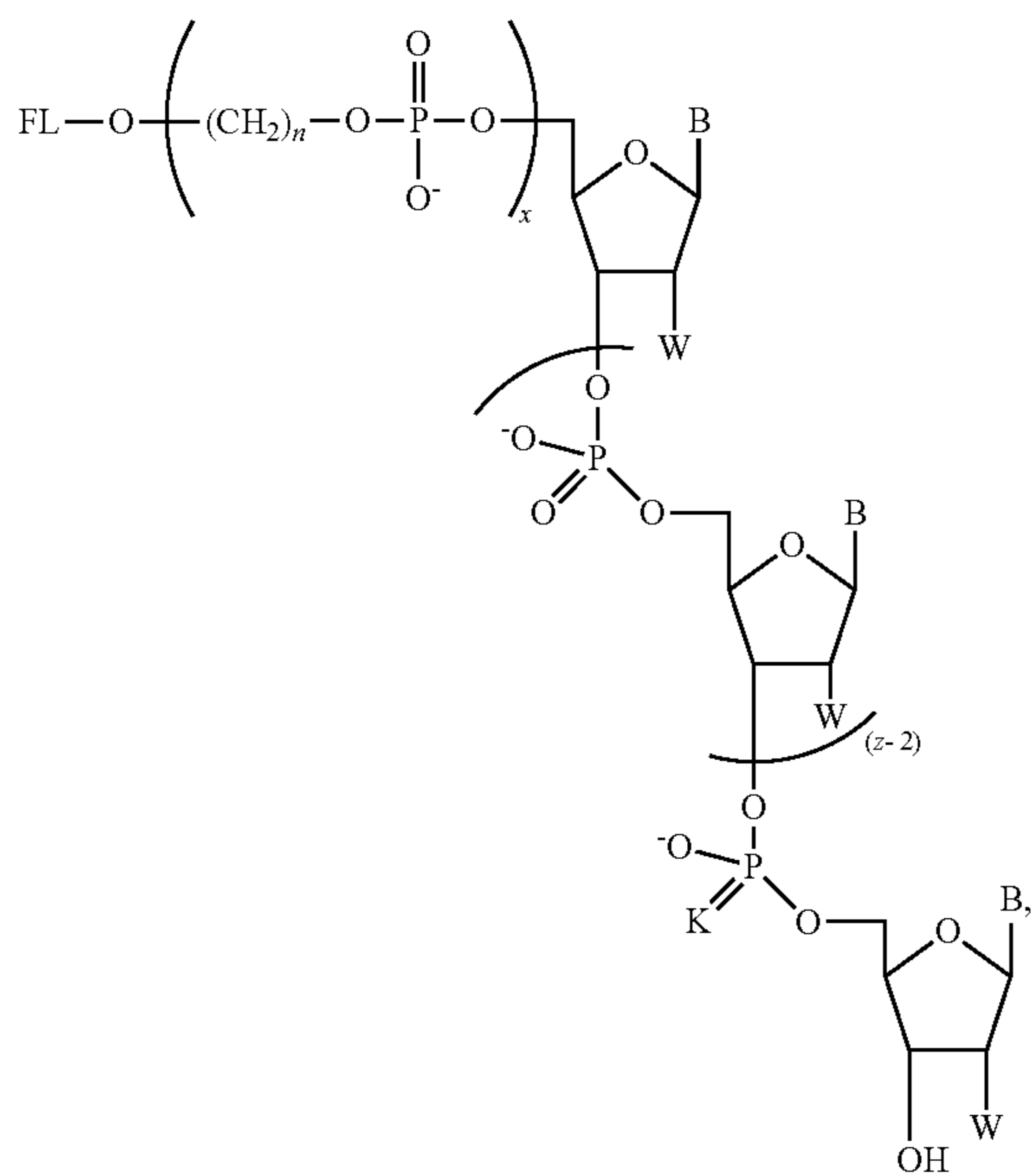
Formula I-G
