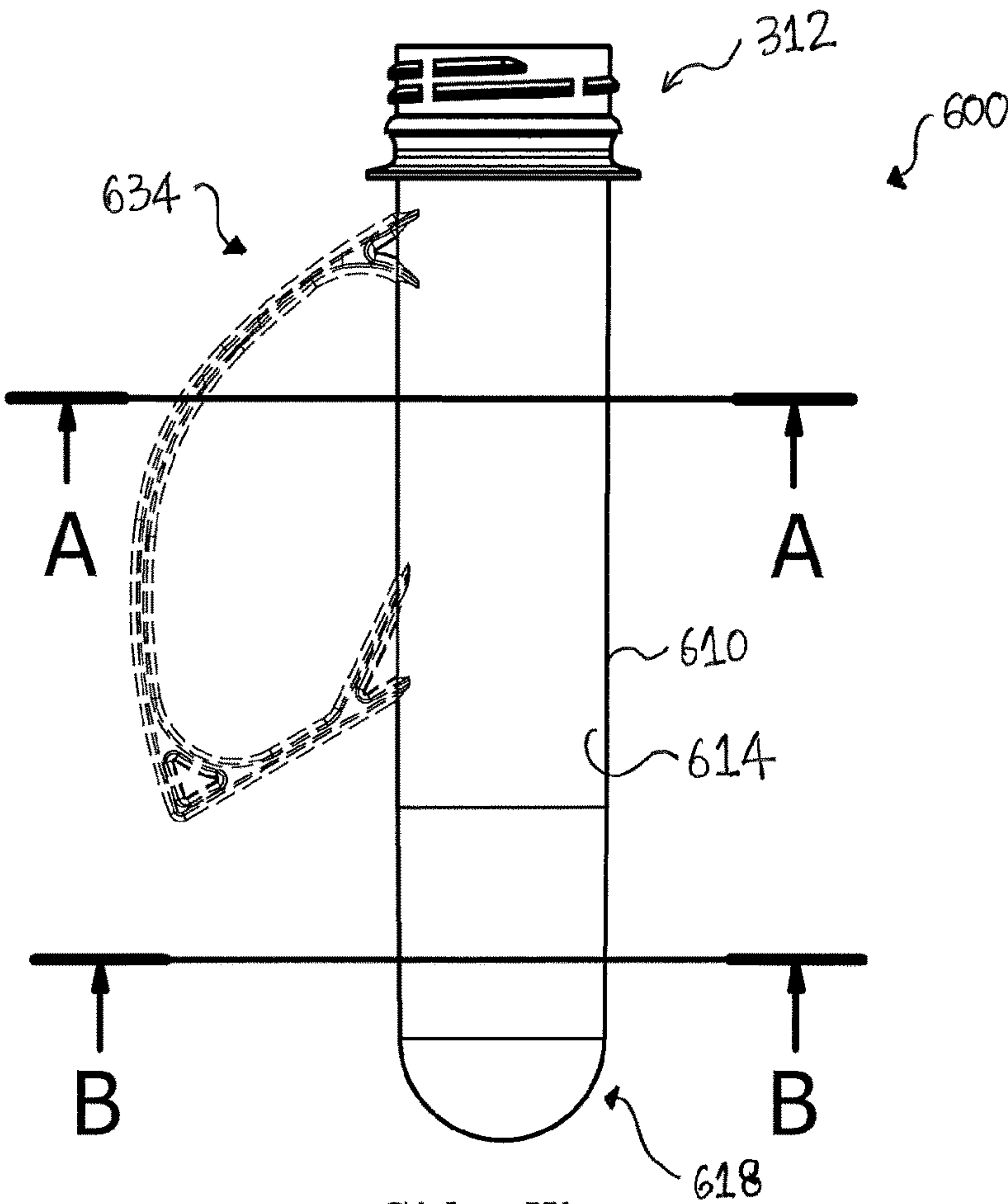
Side View
