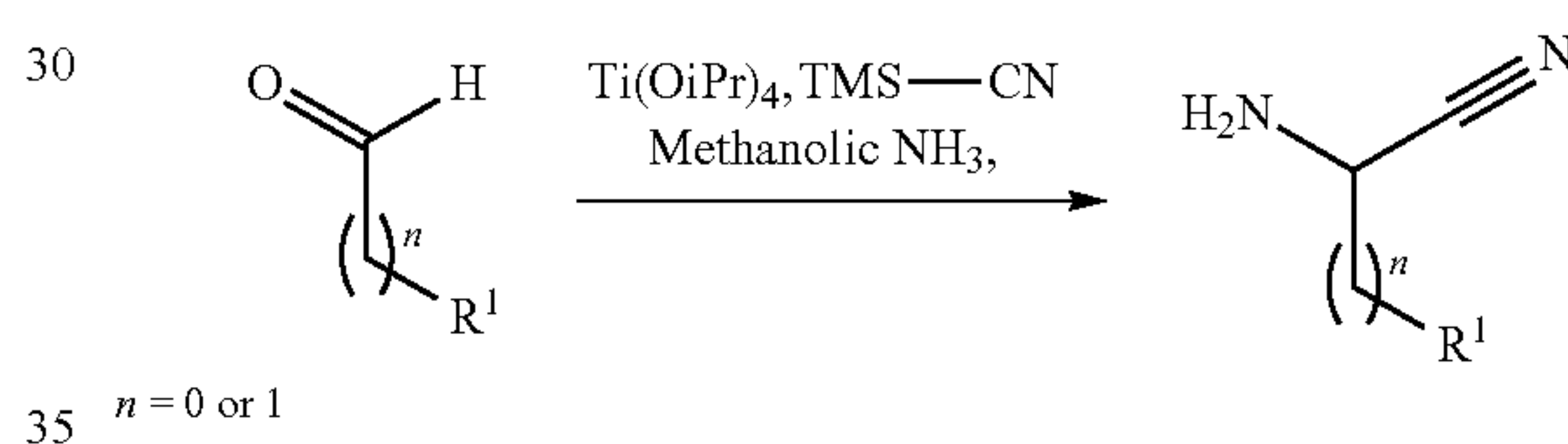
Scheme 16
