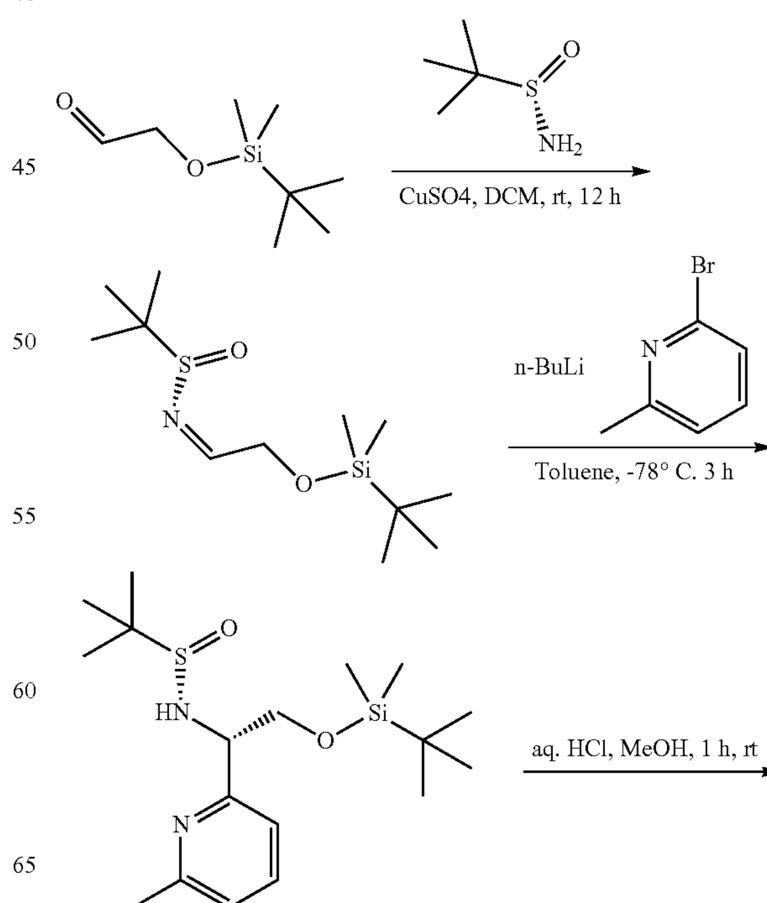
Scheme 17
