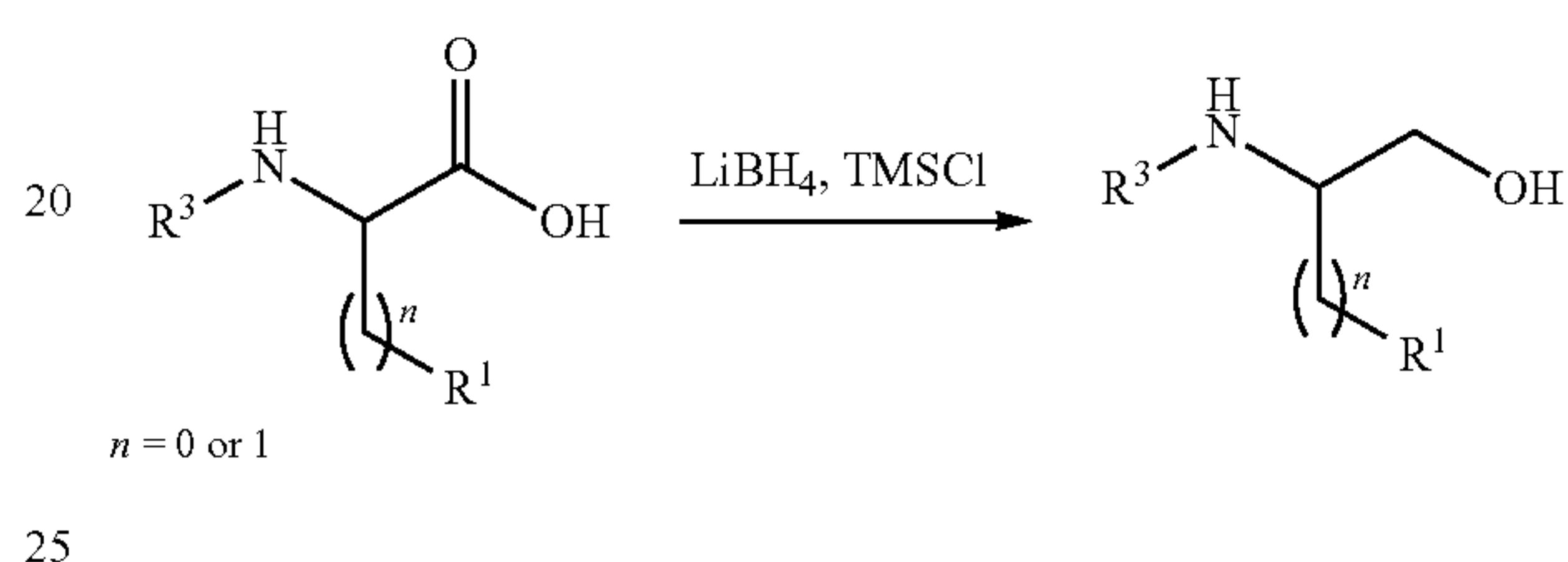
Scheme 15
