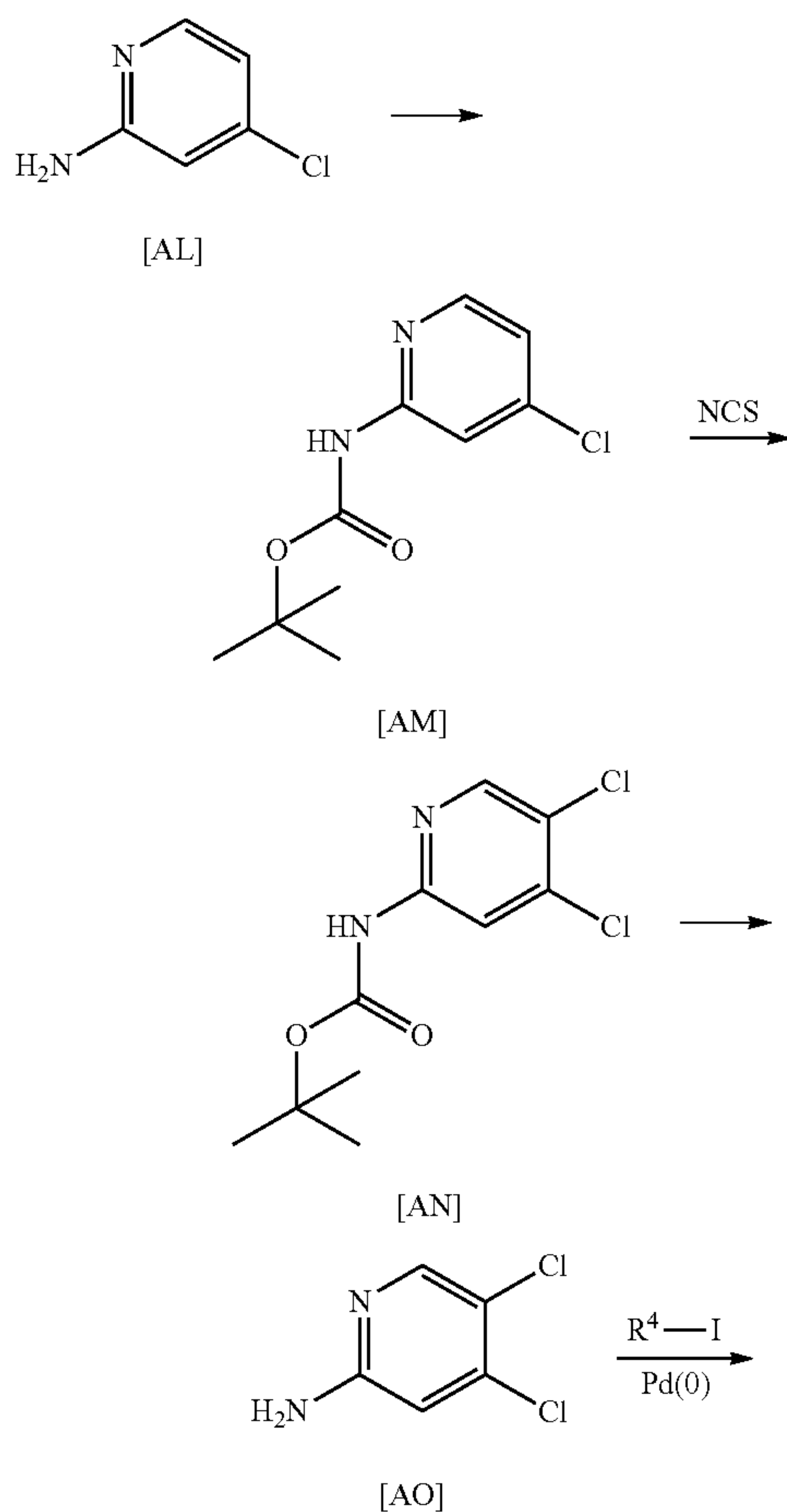
Scheme 10
