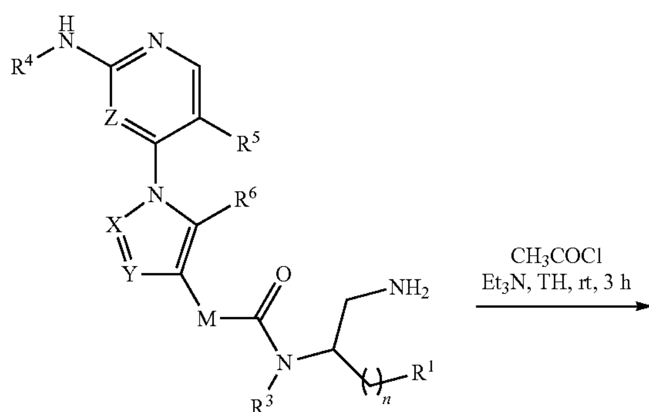
Scheme 19
