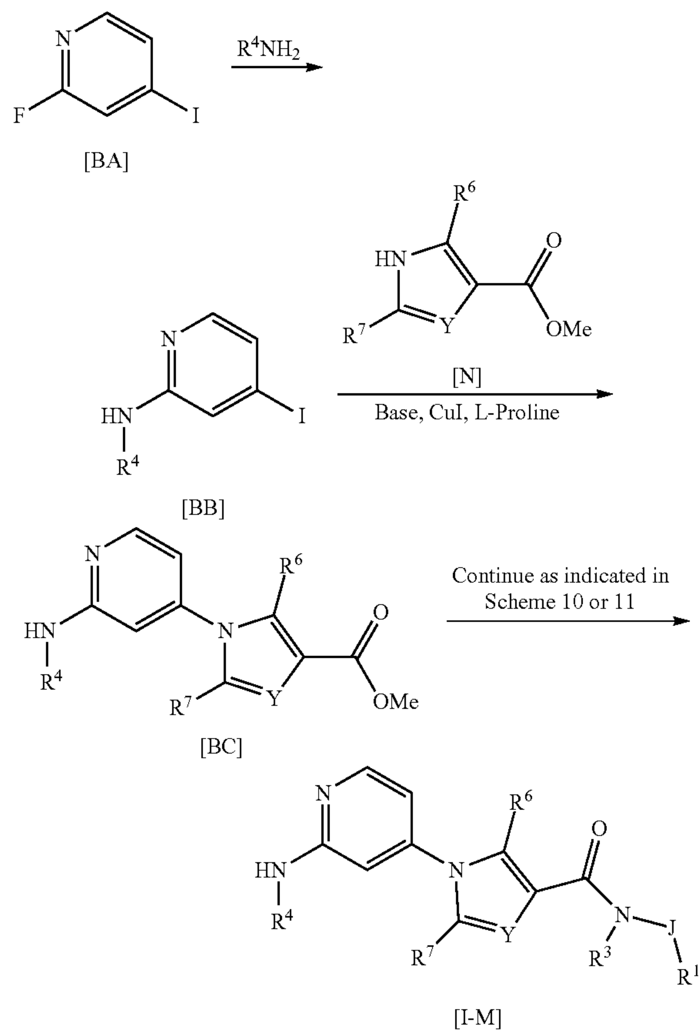
Scheme 13
