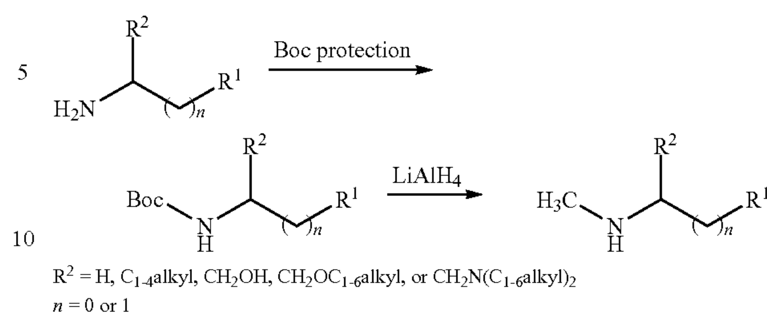
Scheme 14
