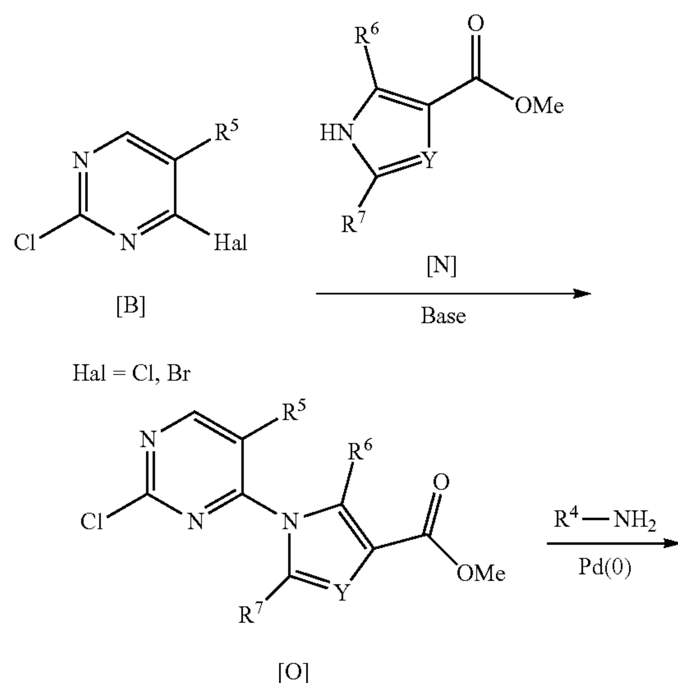
Scheme 4
