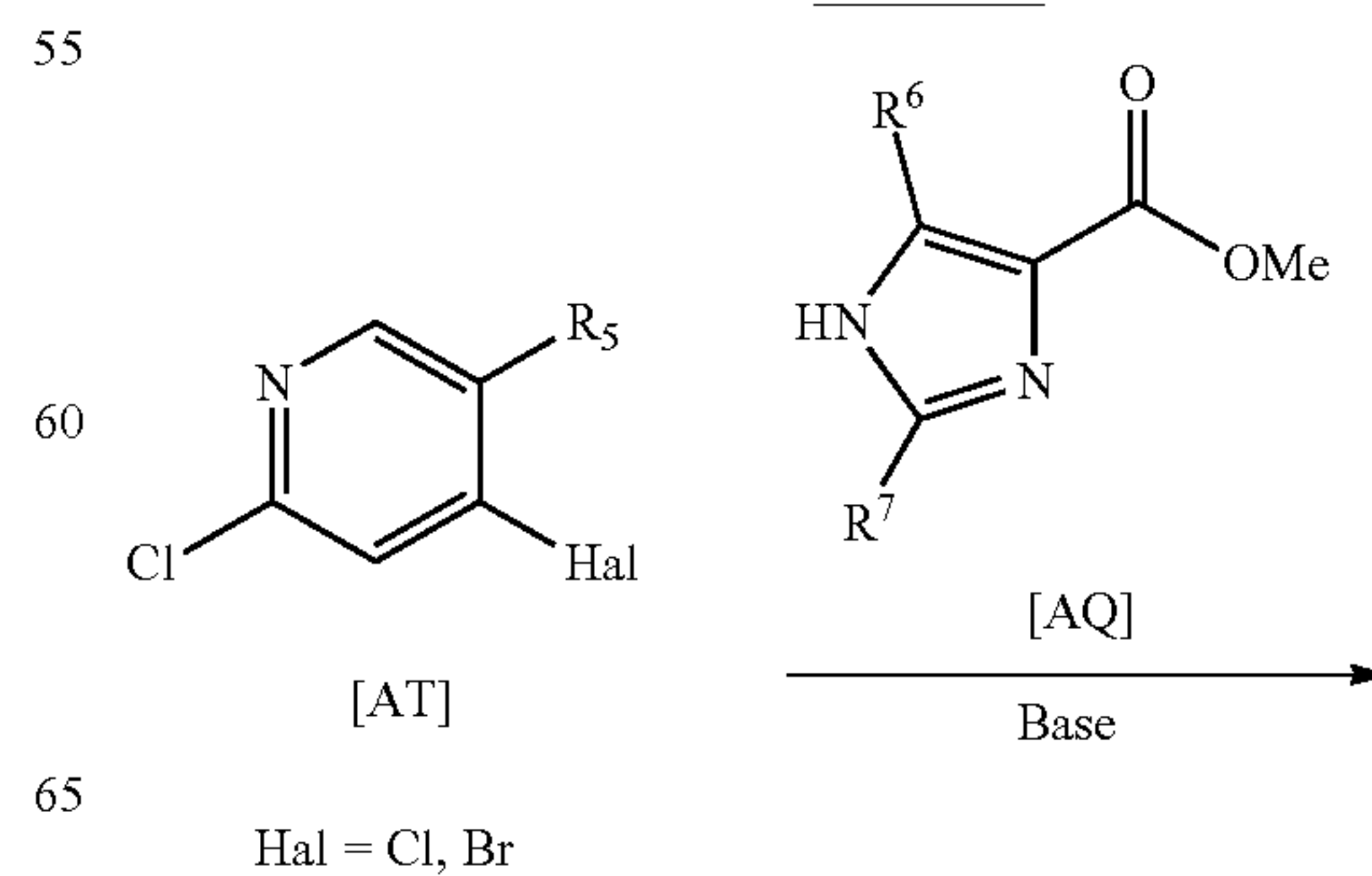
Scheme 11
