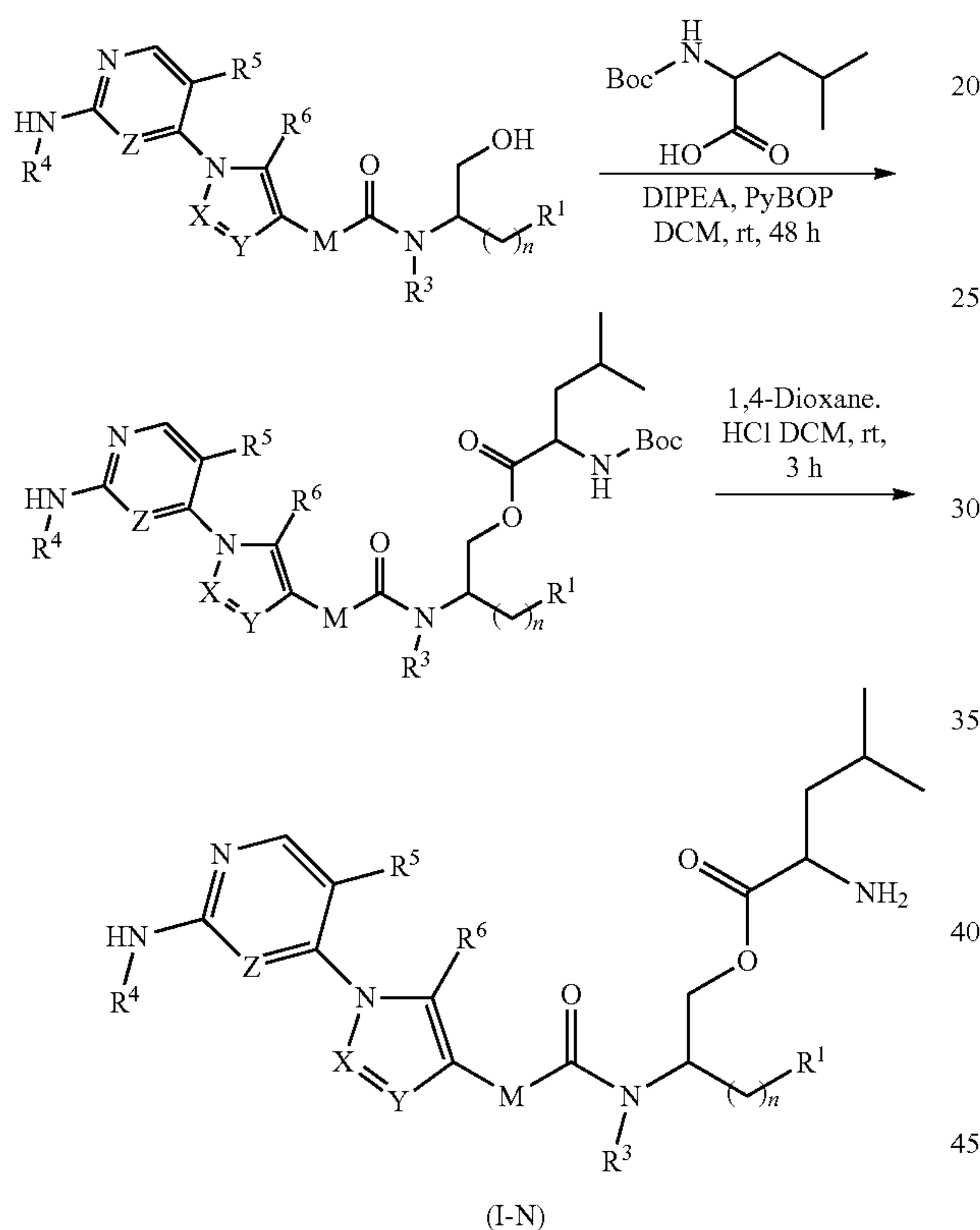
Scheme 18
