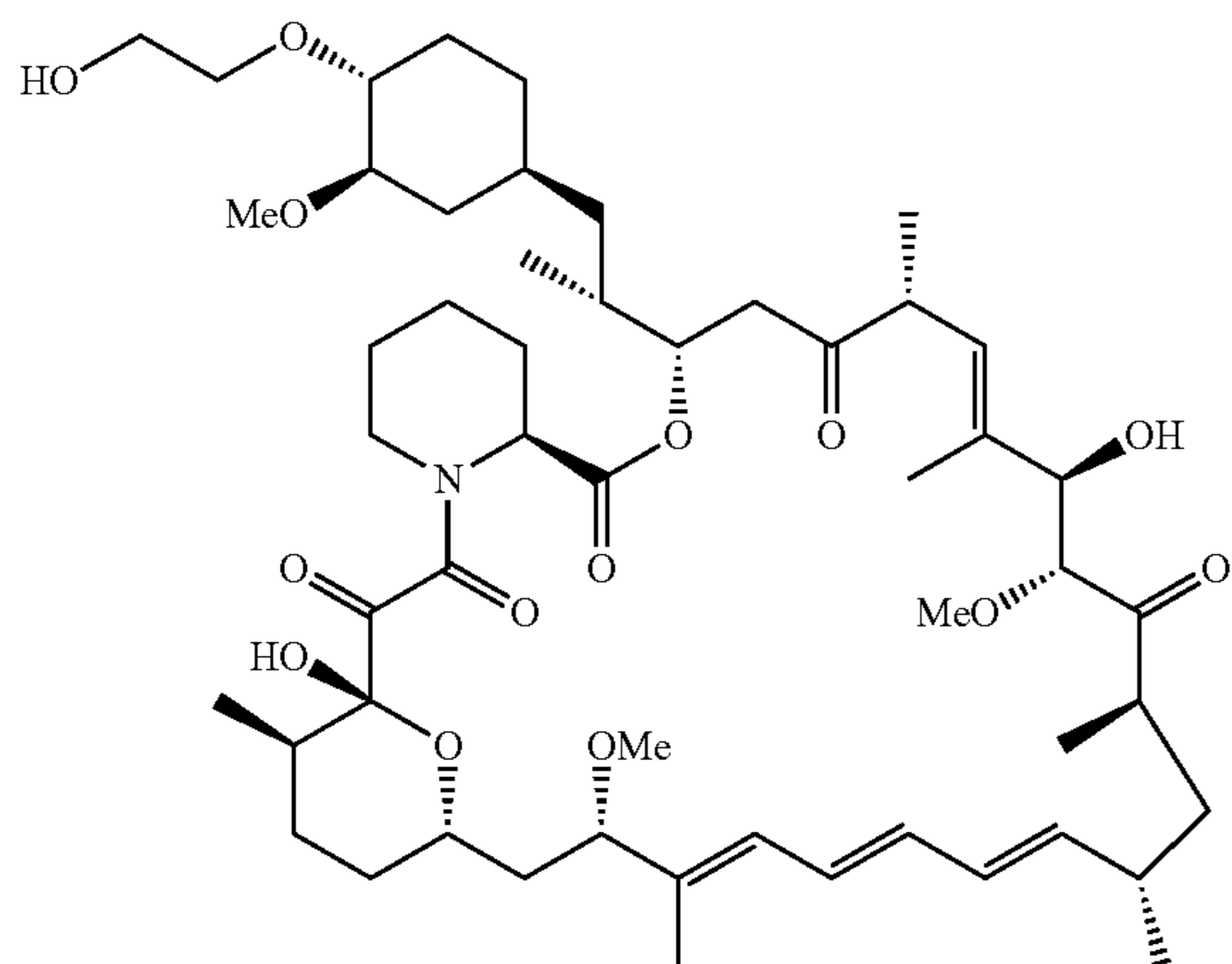
Everolimus (Affinitor)
