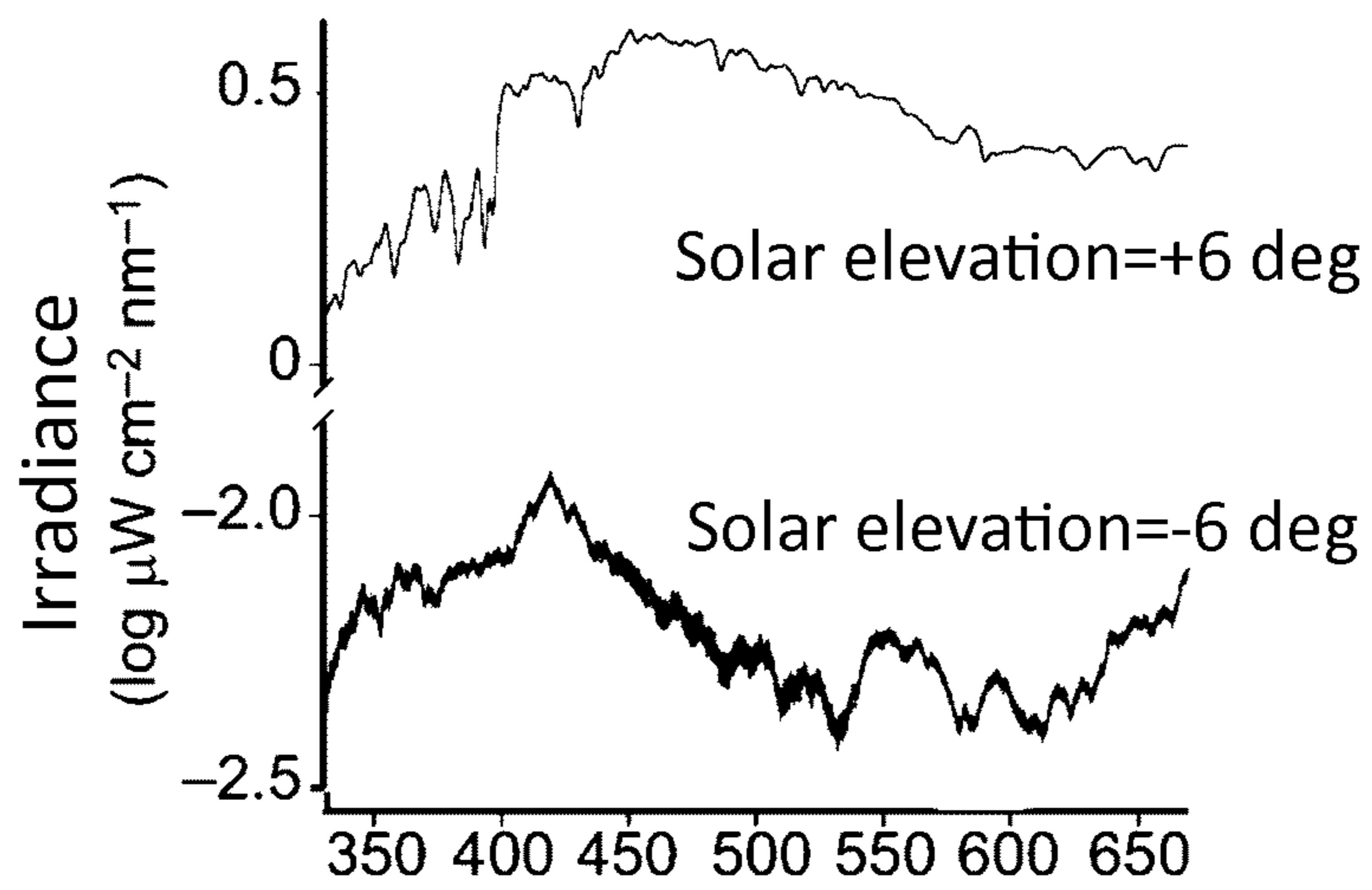
FIG. 3 (Prior art)
