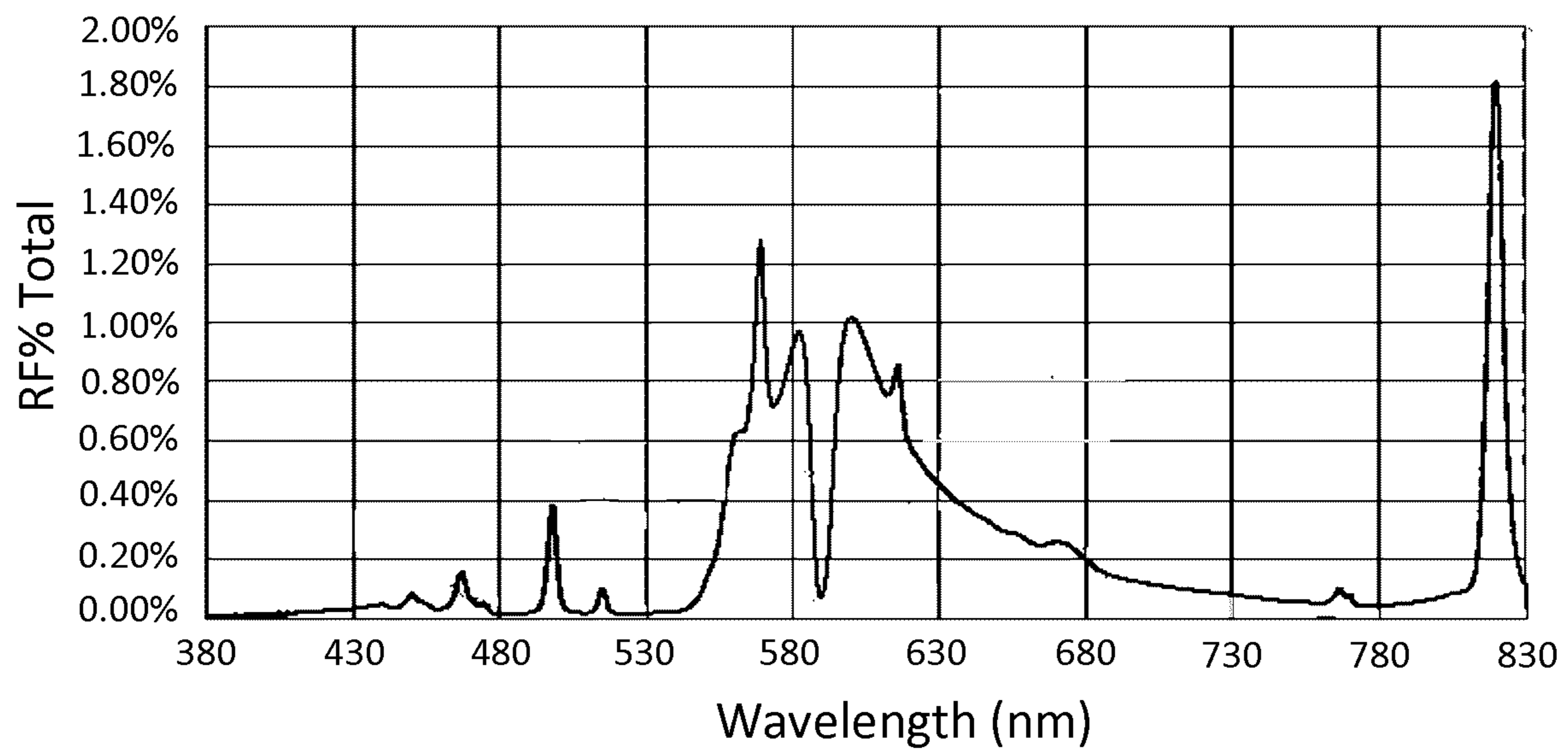
FIG. 4 (Prior art)
