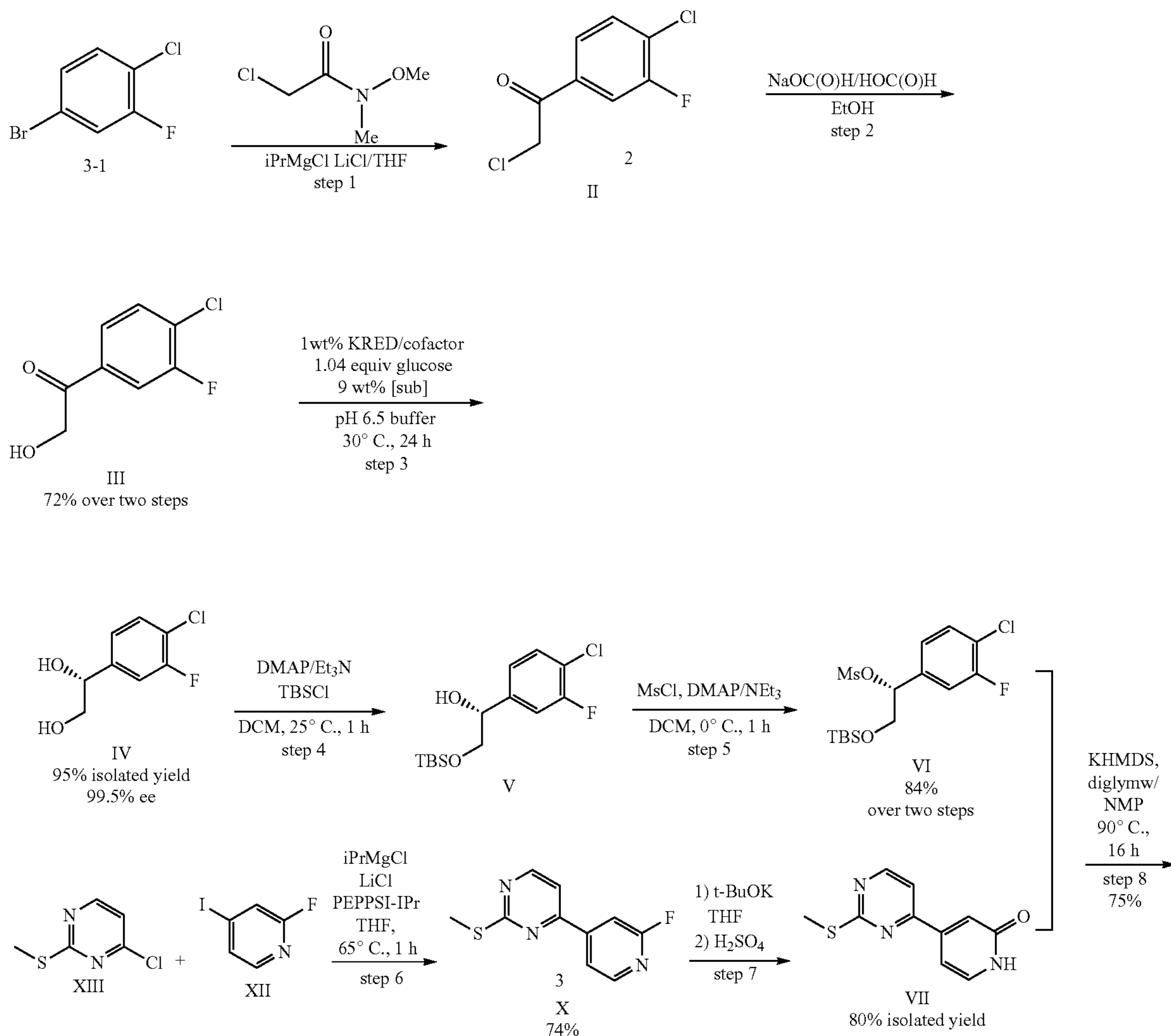
Scheme 2. Improved Process To I
