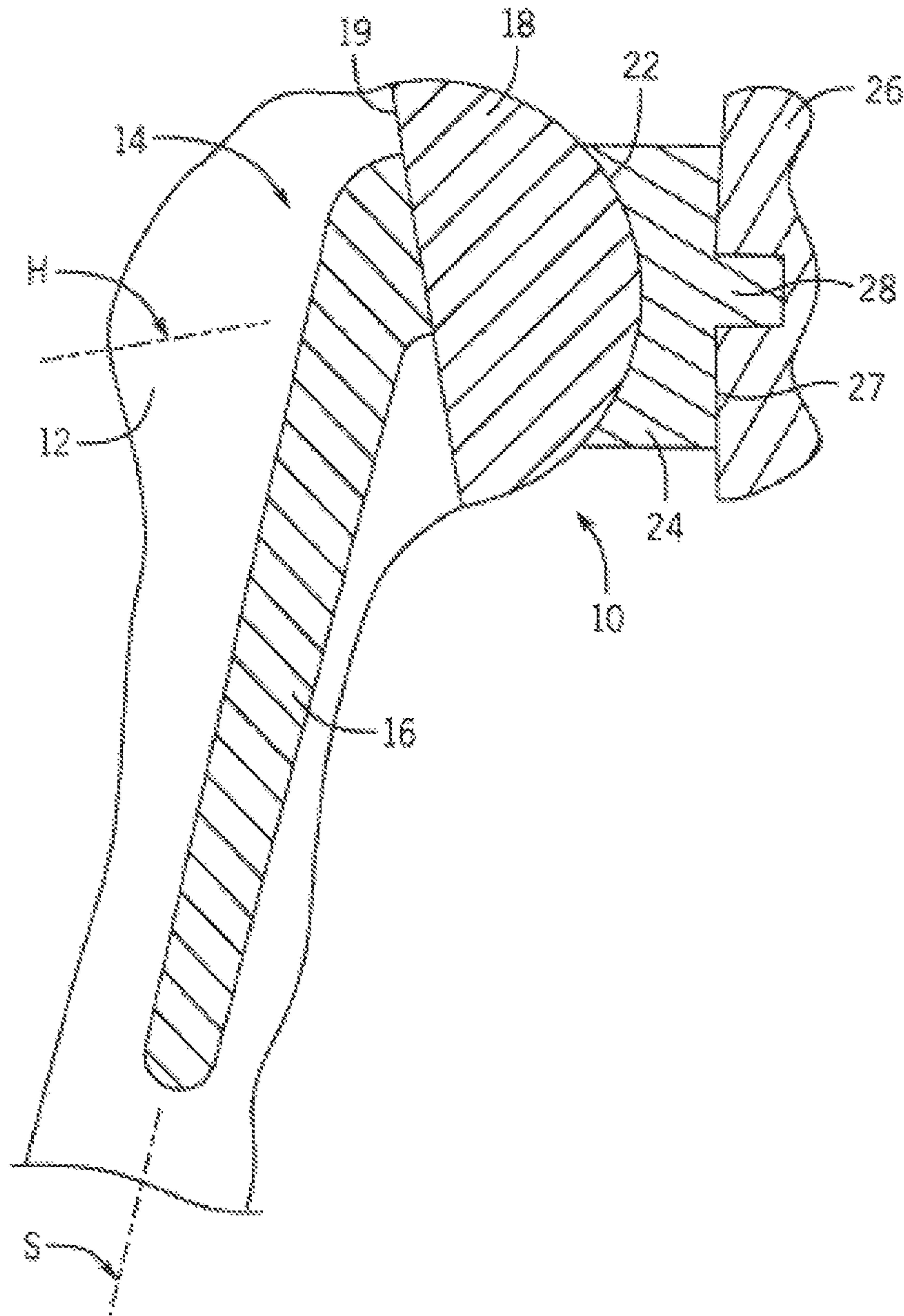
FIG. 1 PRIOR ART
