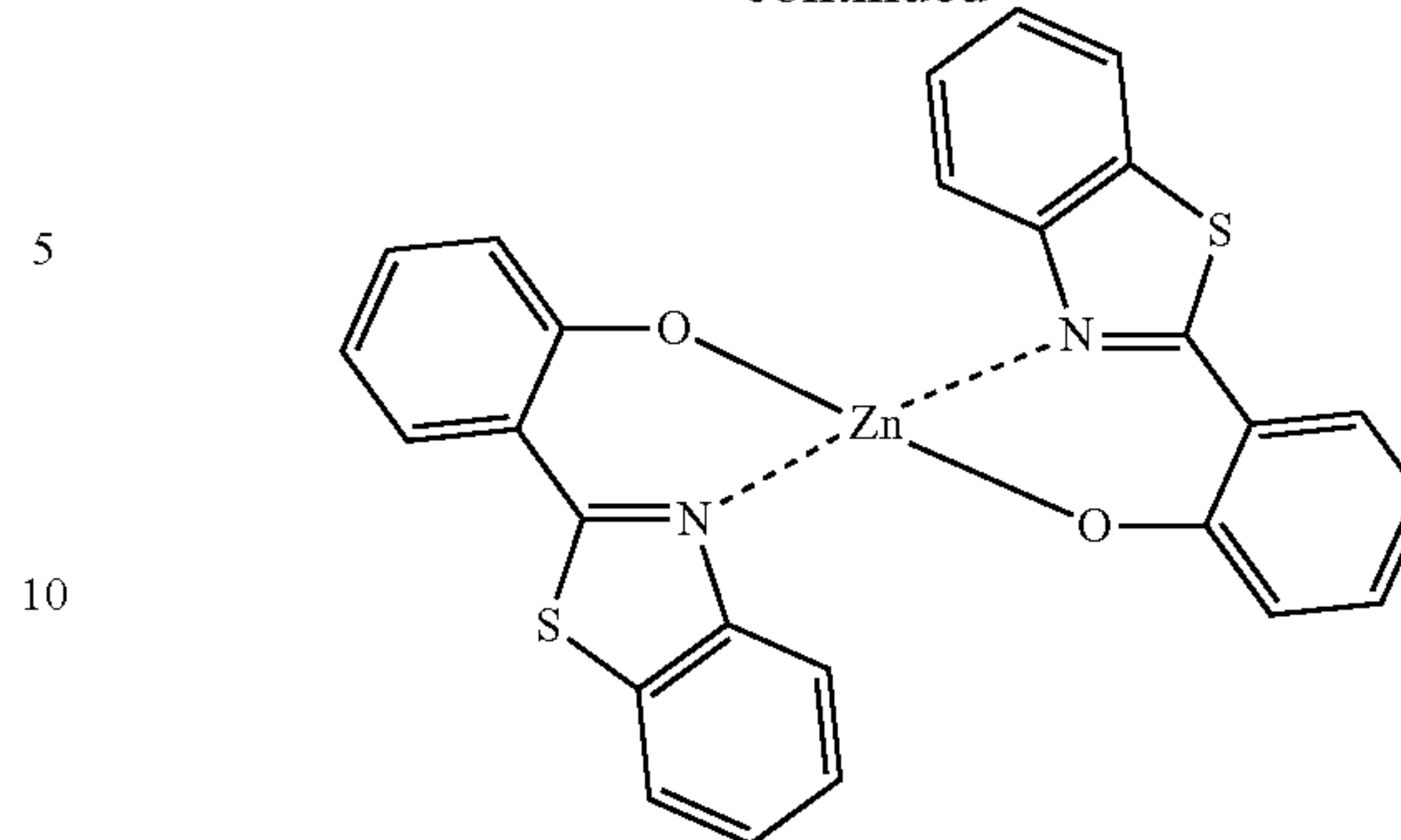
Zn(BTZ) 2
