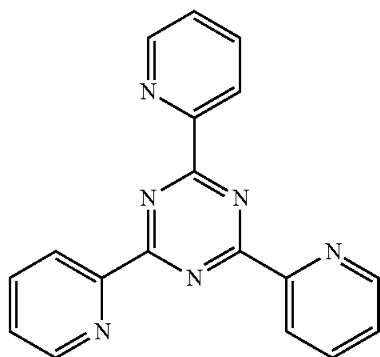
2Py3Tz
